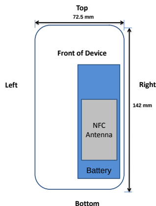
Figure 1-2 DUT Antenna Locations
