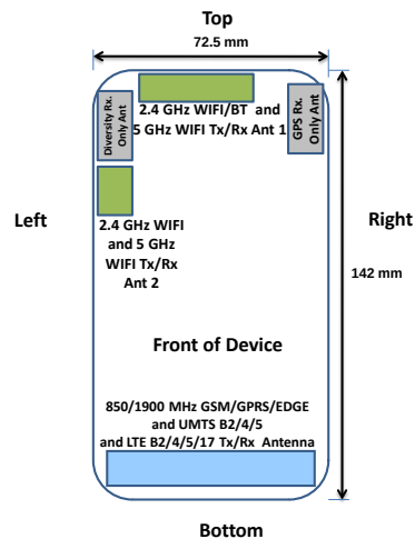
Figure 1-1 DUT Antenna Locations
