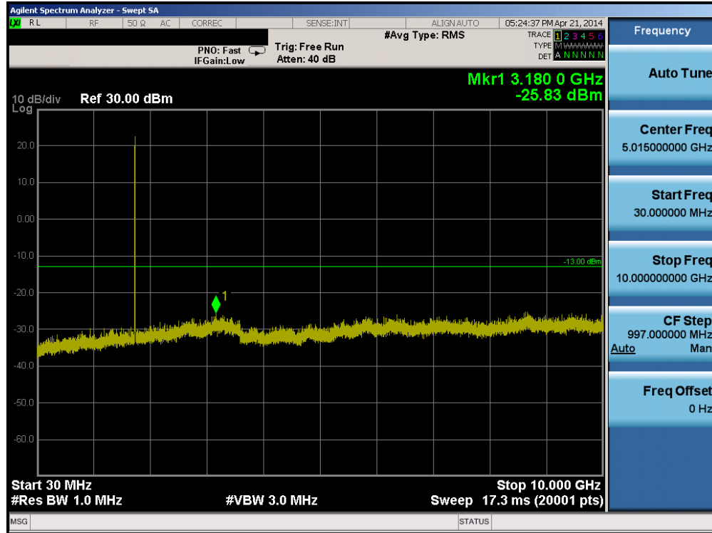
Plot 6-6. Conducted Spurious Plot (AWS WCDMA Mode – Ch. 1862)
