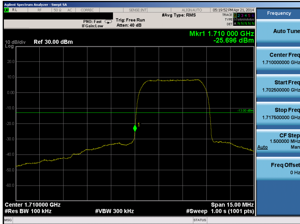
Plot 6-8. Band Edge Plot (AWS WCDMA Mode – Ch. 1312)
