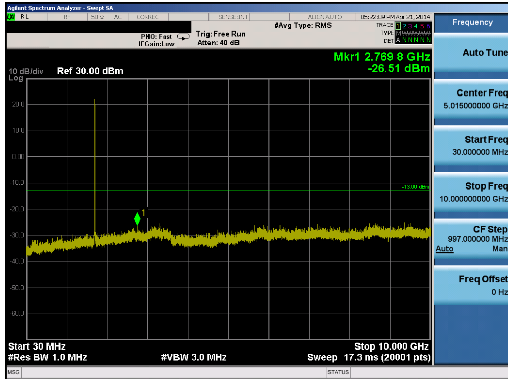
Plot 6-2. Conducted Spurious Plot (AWS WCDMA Mode – Ch. 1312)
