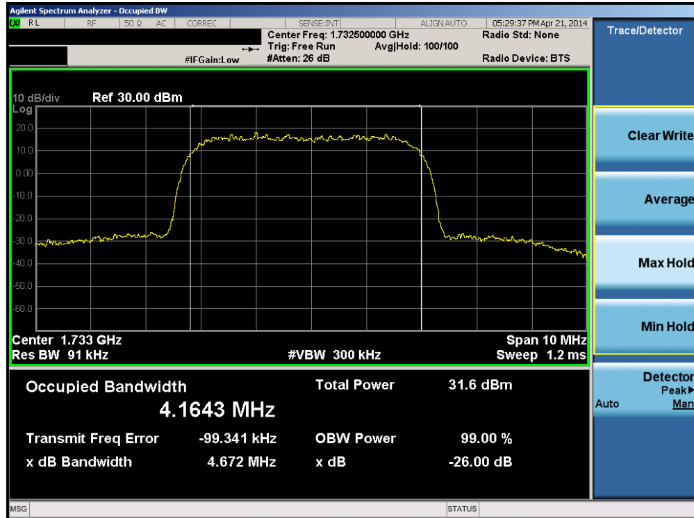
Plot 6-1. Occupied Bandwidth Plot (AWS WCDMA Mode – Ch. 1412)
