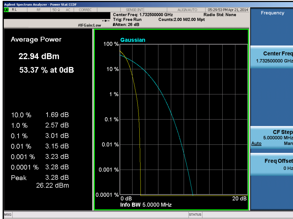
Plot 6-12. Peak-Average Ratio Plot (AWS WCDMA Mode – Ch. 1412)
