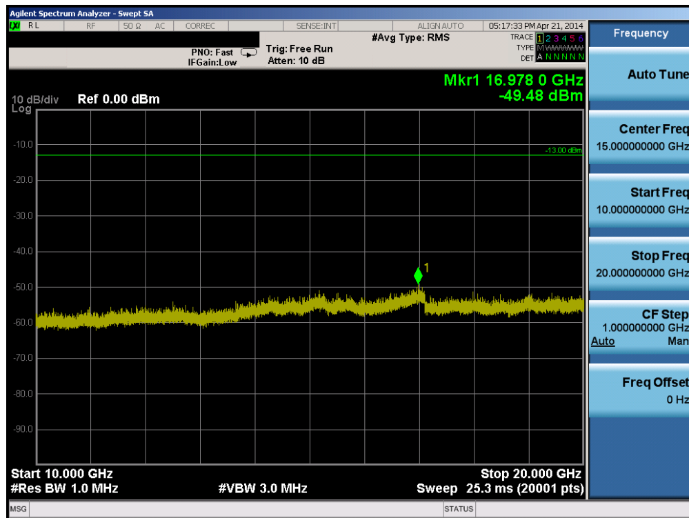
Plot 6-5. Conducted Spurious Plot (AWS WCDMA Mode – Ch. 1412)
