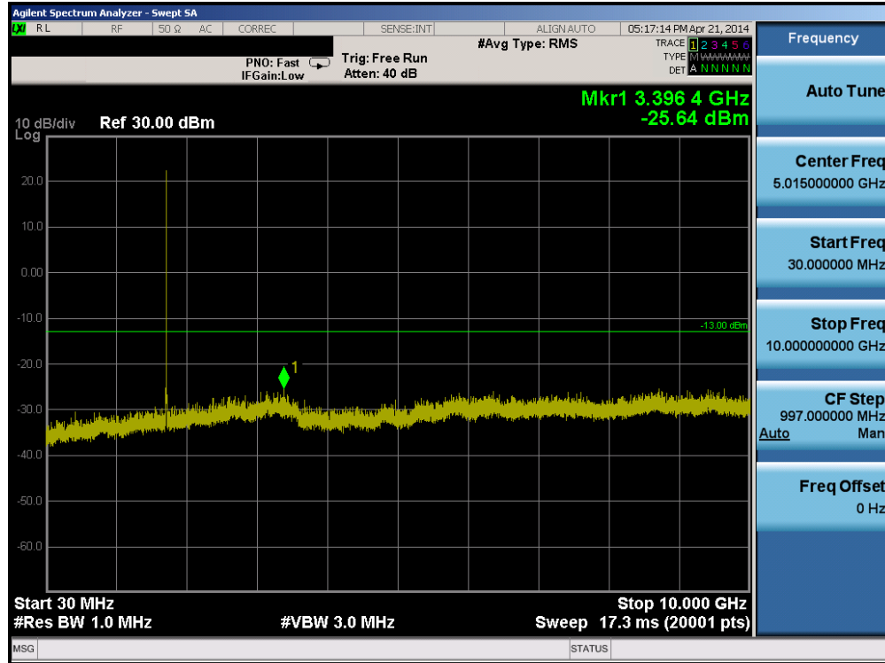
Plot 6-4. Conducted Spurious Plot (AWS WCDMA Mode – Ch. 1412)
