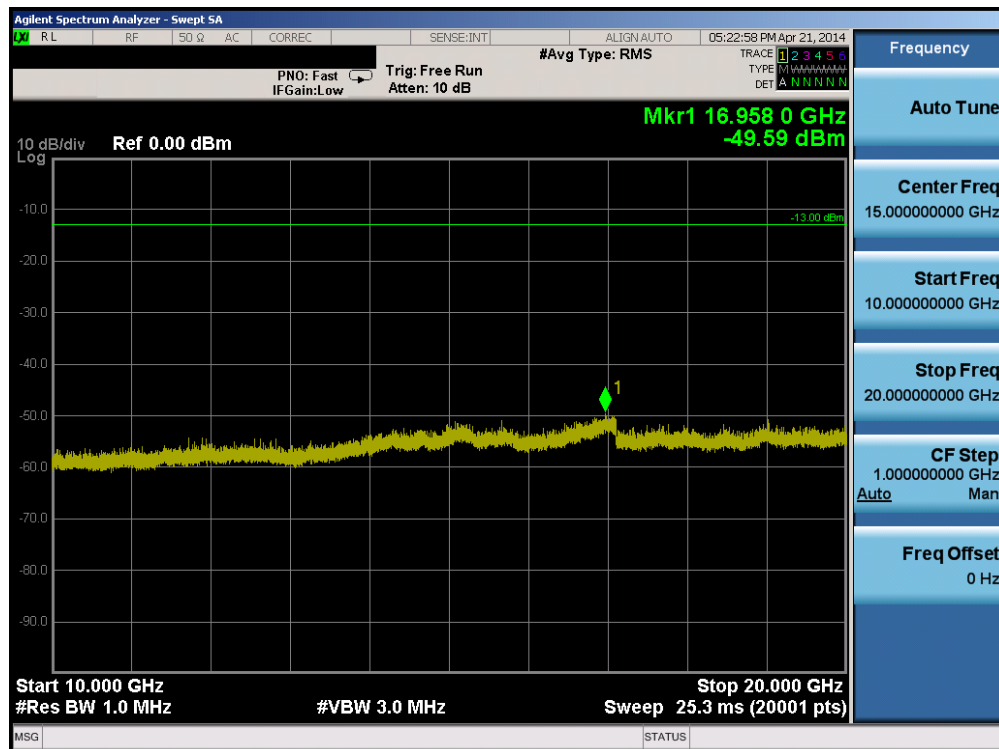
Plot 6-3. Conducted Spurious Plot (AWS WCDMA Mode – Ch. 1312)
