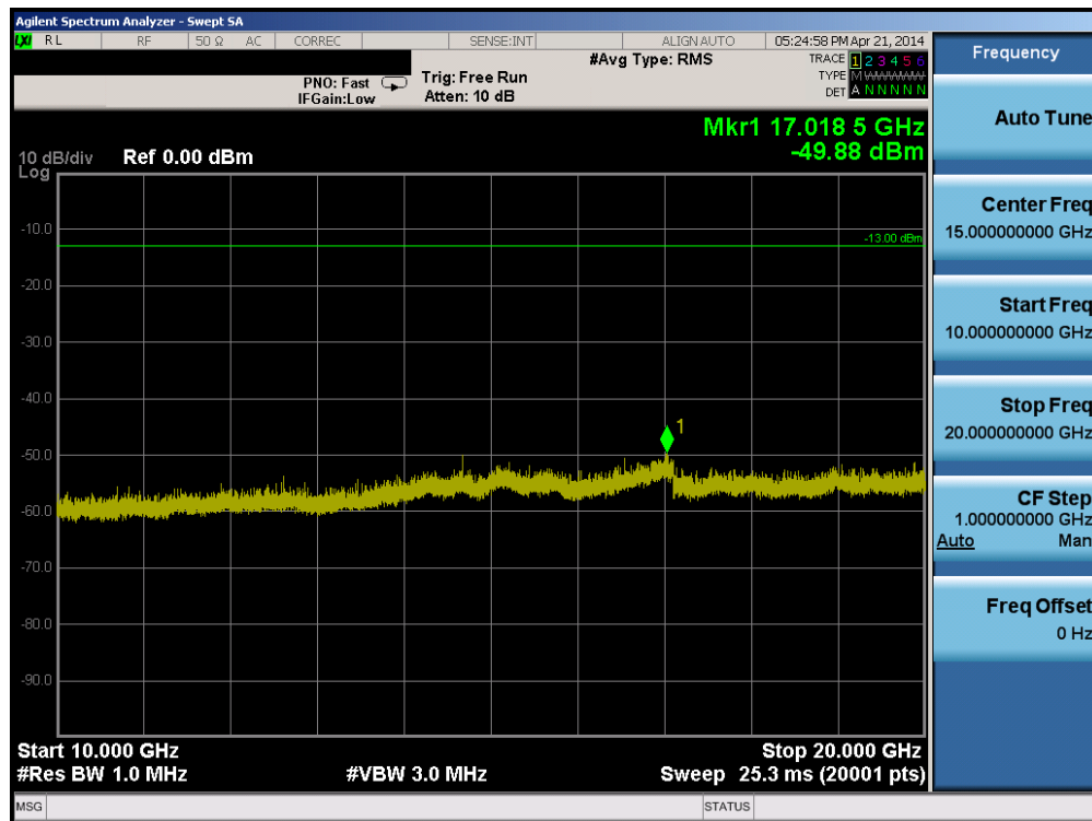
Plot 6-7. Conducted Spurious Plot (AWS WCDMA Mode – Ch. 1862)
