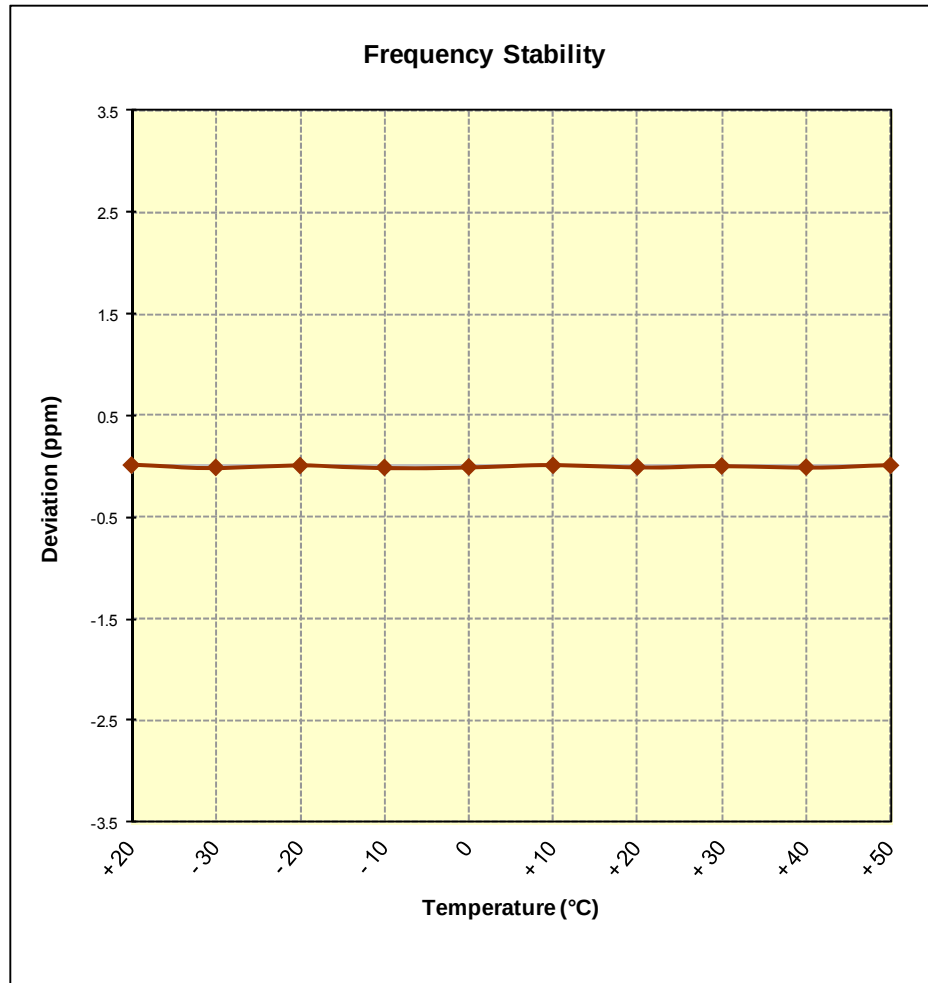
Figure 6-7. Frequency Stability Graph (AWS WCDMA Mode – Ch. 1412)
