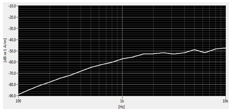
Figure 7-2 Worst-case ABM2 Plot for WD
