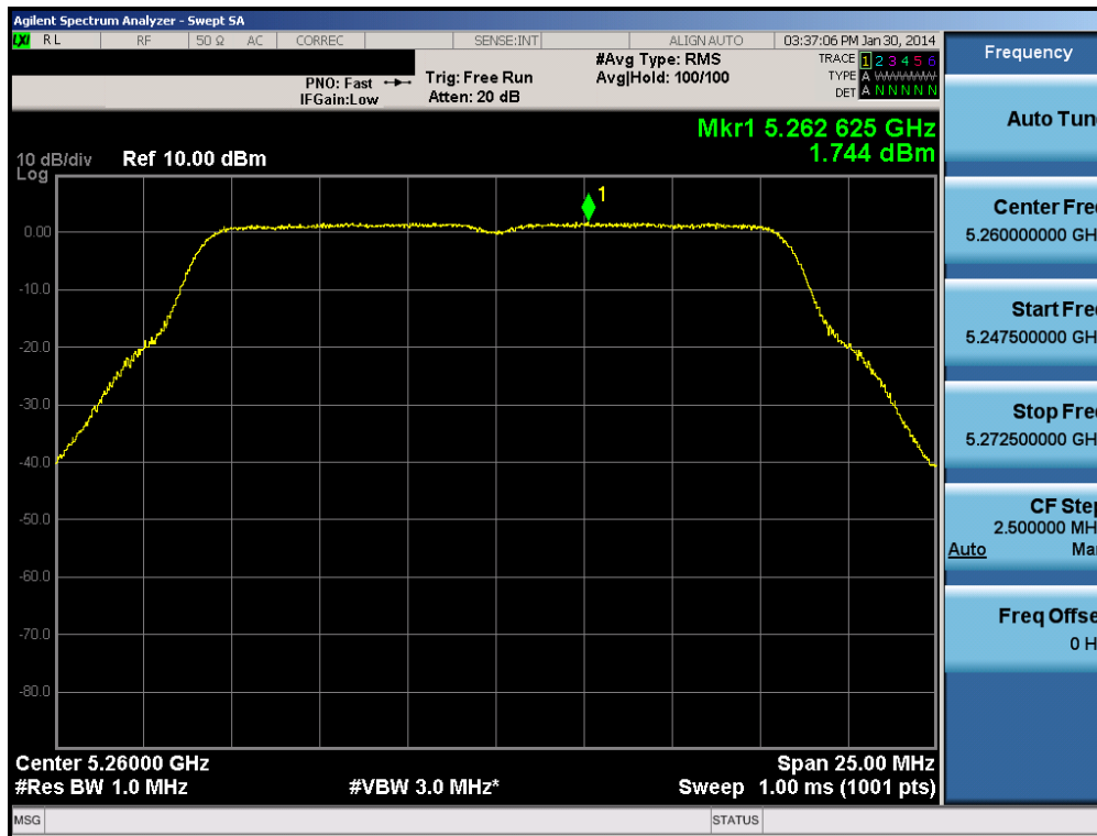
Plot 6-76. Peak Power Spectral Density Plot (802.11a (UNII Band 2A) – Ch. 52)
