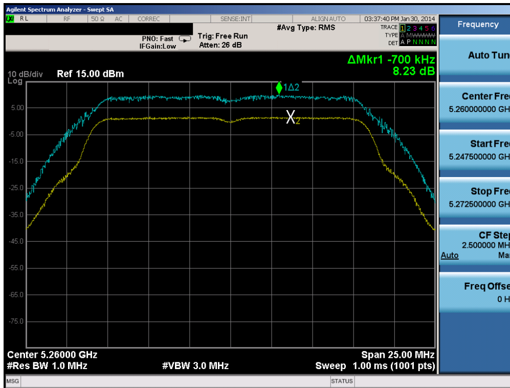
Plot 6-132. Peak Excursion Ratio Plot (802.11a (UNII Band 2A) – Ch. 52)
