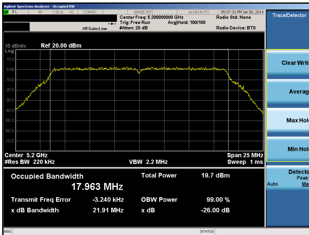
Plot 6-38. 26dB Bandwidth Plot (20MHz BW 802.11n (UNII Band 1) – Ch. 40)
