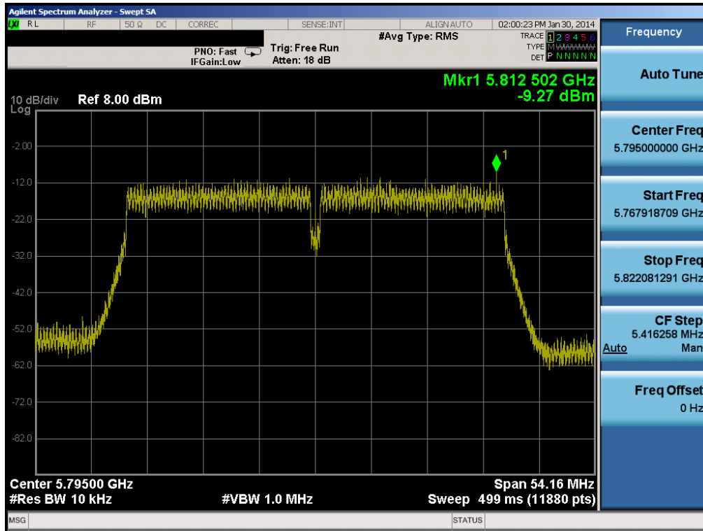
Plot 6-71. 6dB Bandwidth Plot (40MHz BW 802.11n (5.8GHz) – Ch. 159)
