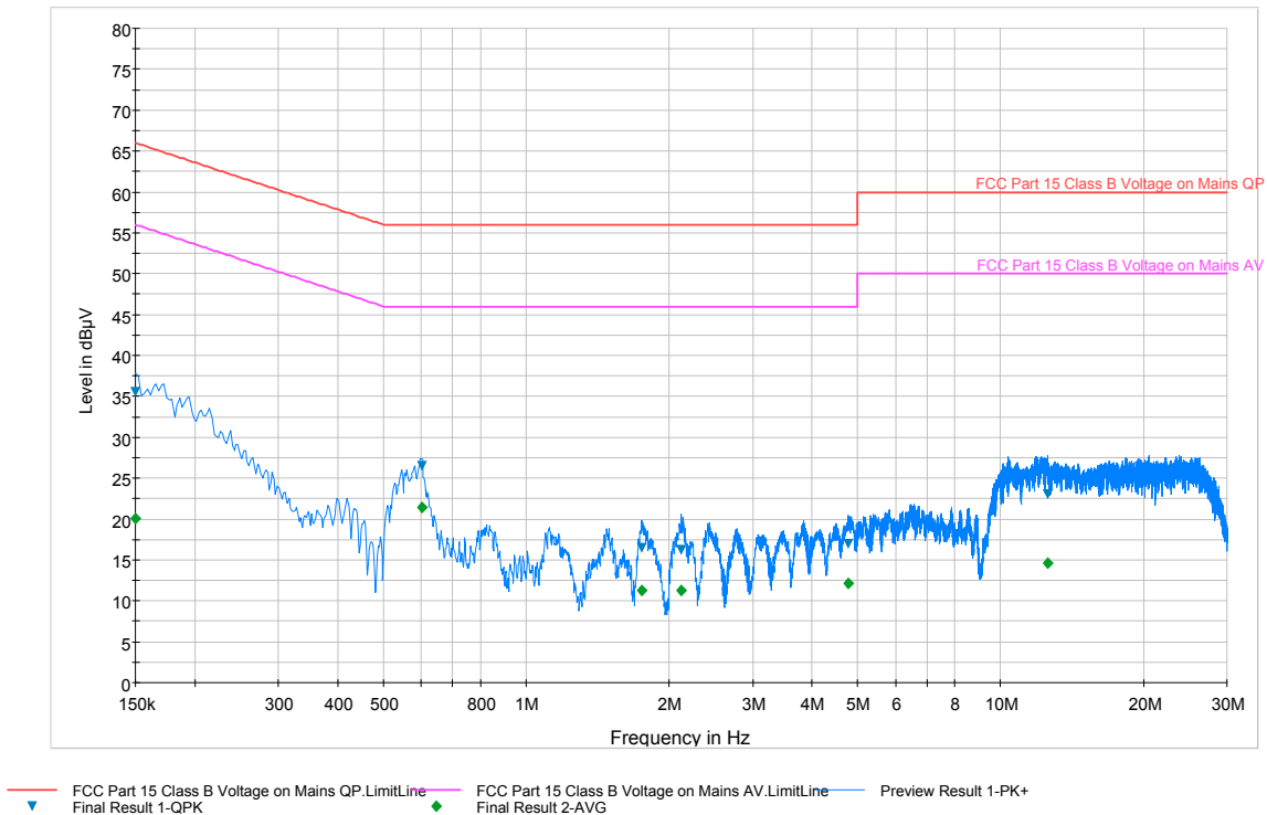
Plot 6-145. Line Conducted Plot with 802.11a (L1)
