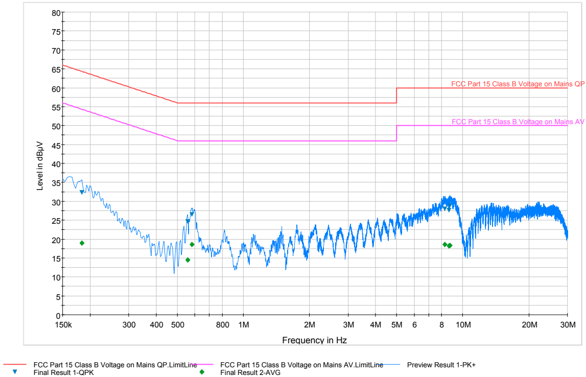
Plot 6-146. Line Conducted Plot with 802.11a (N)
