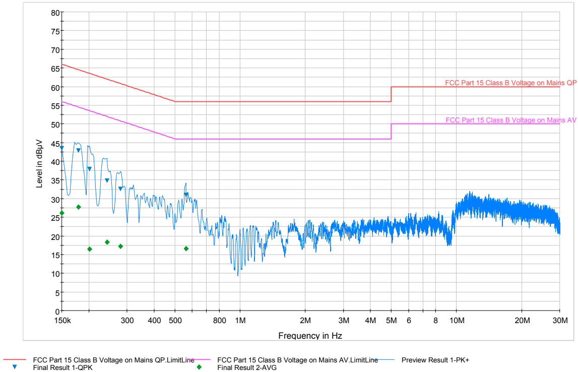
Plot 6-143. Line Conducted Plot with 802.11b (L1)
