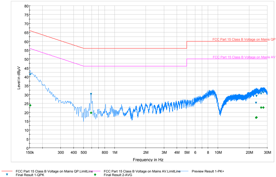
Plot 6-144. Line Conducted Plot with 802.11b (N)
