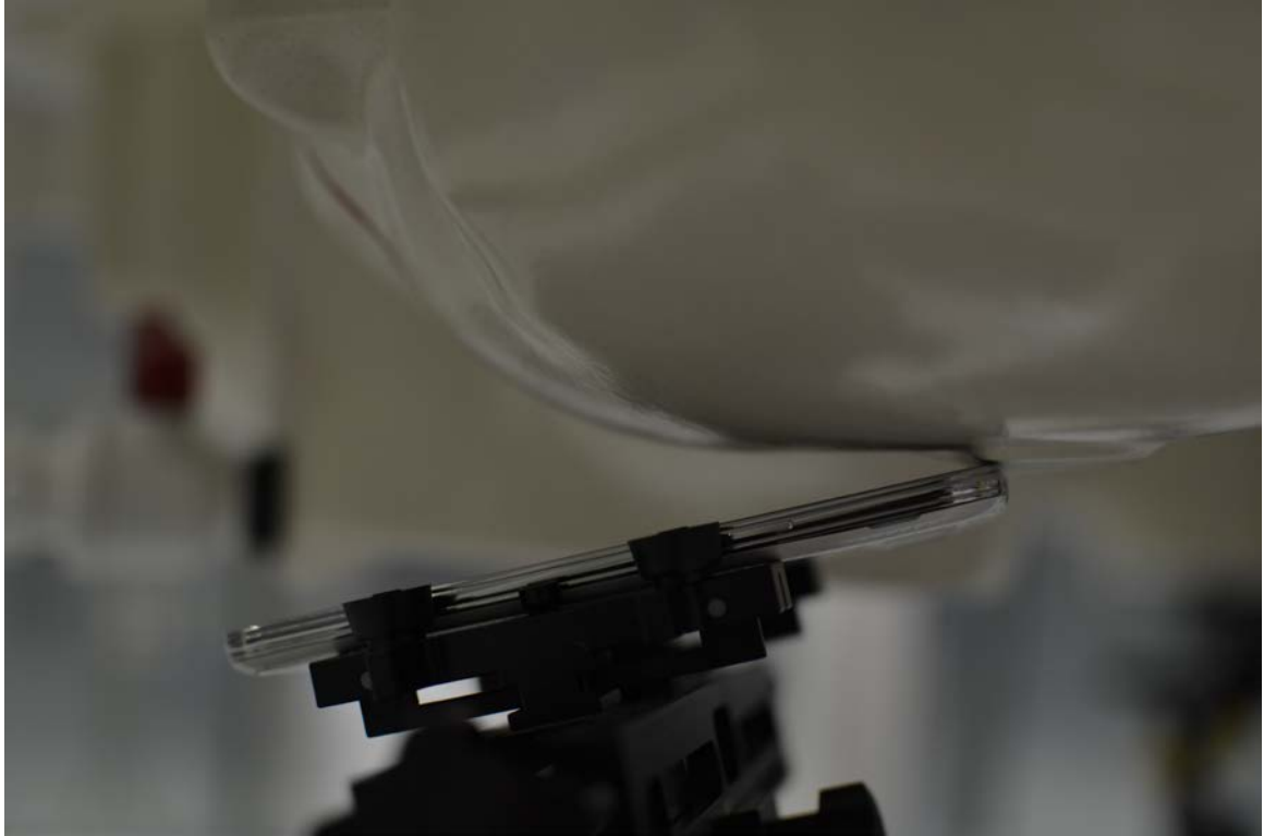
SAR Test Setup Photo 5 – Left Tilt, Standard Battery Cover
