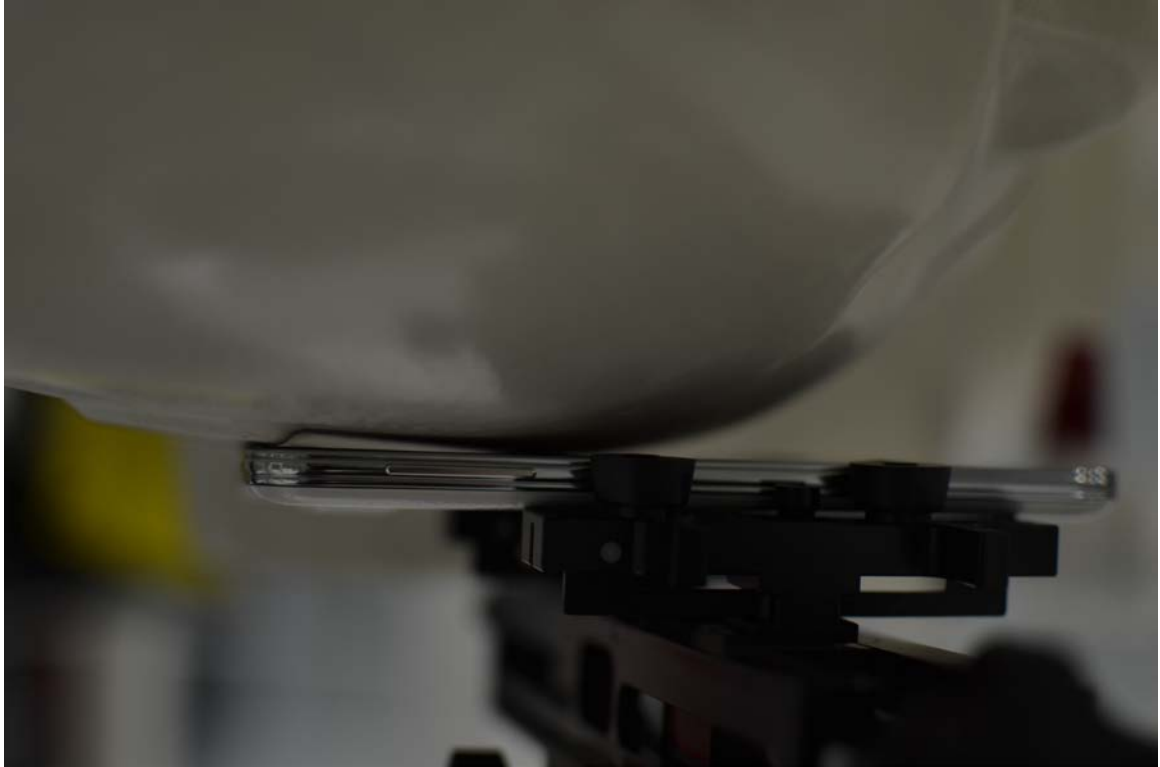
SAR Test Setup Photo 1 – Right Cheek, Standard Battery Cover
