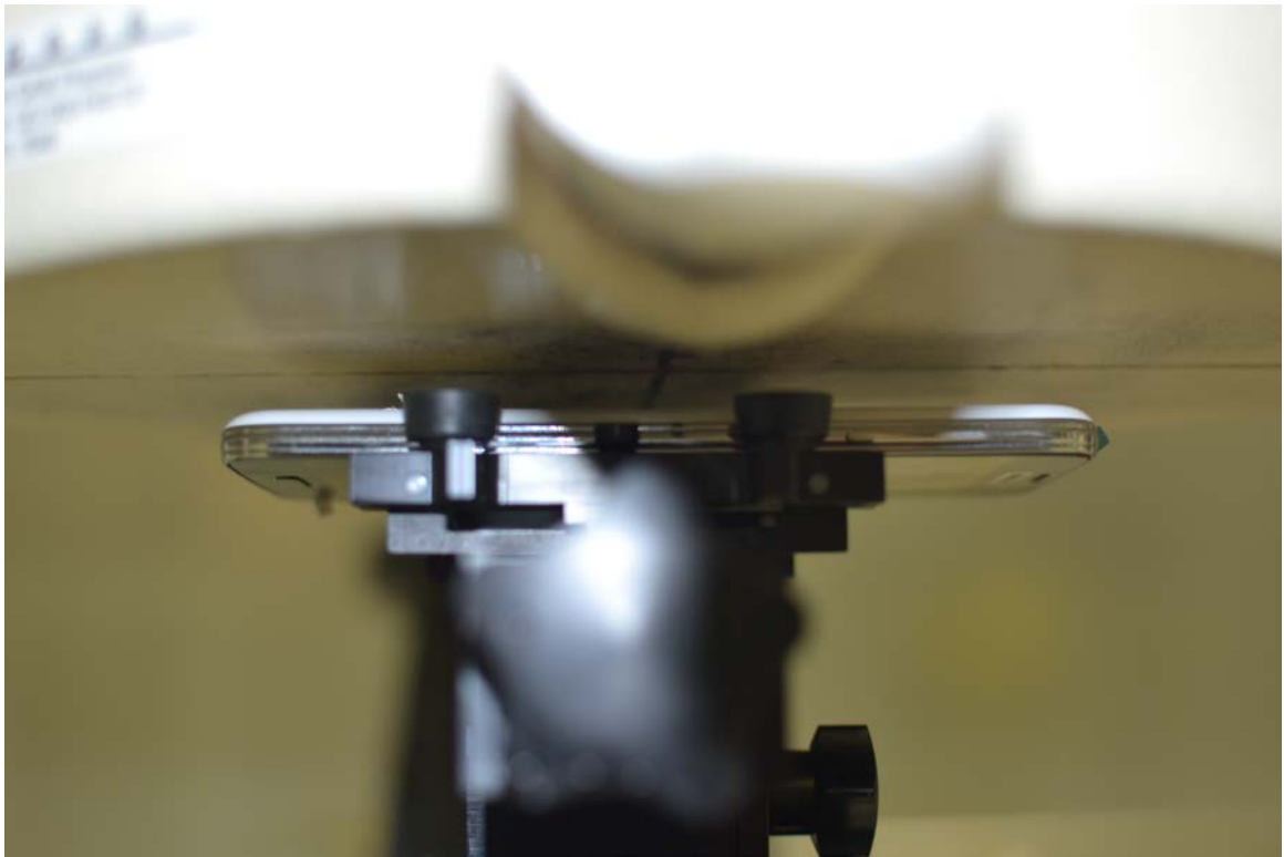
SAR Test Setup Photo 6 – Back Side at 1.0 cm, Standard Battery Cover
