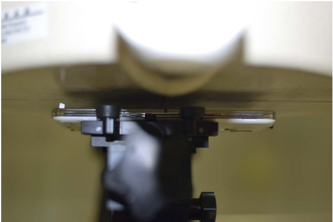
SAR Test Setup Photo 8 – Front Side at 1.0 cm, Standard Battery Cover
