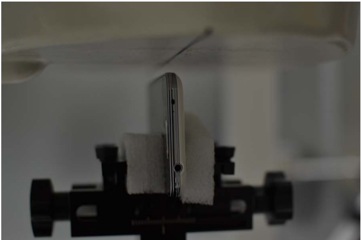
SAR Test Setup Photo 12 – Left Edge at 1.0 cm, Wireless Charging Cover
