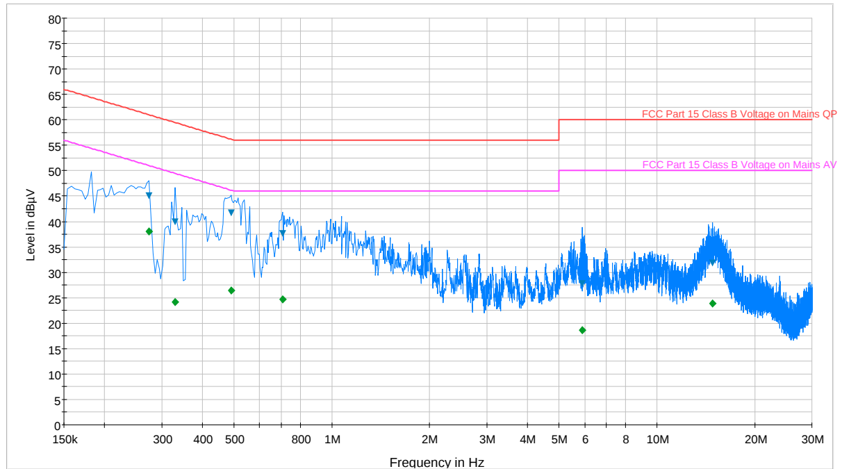
Plot 7-1. Line Conducted Plot (L1)
