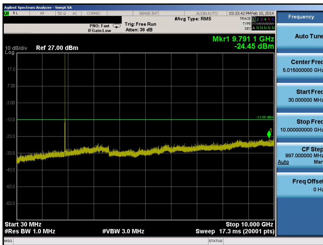
Plot 8-51. Conducted Spurious Plot (10.0MHz QPSK – RB Size 1, RB Offset 0 – High Channel)
