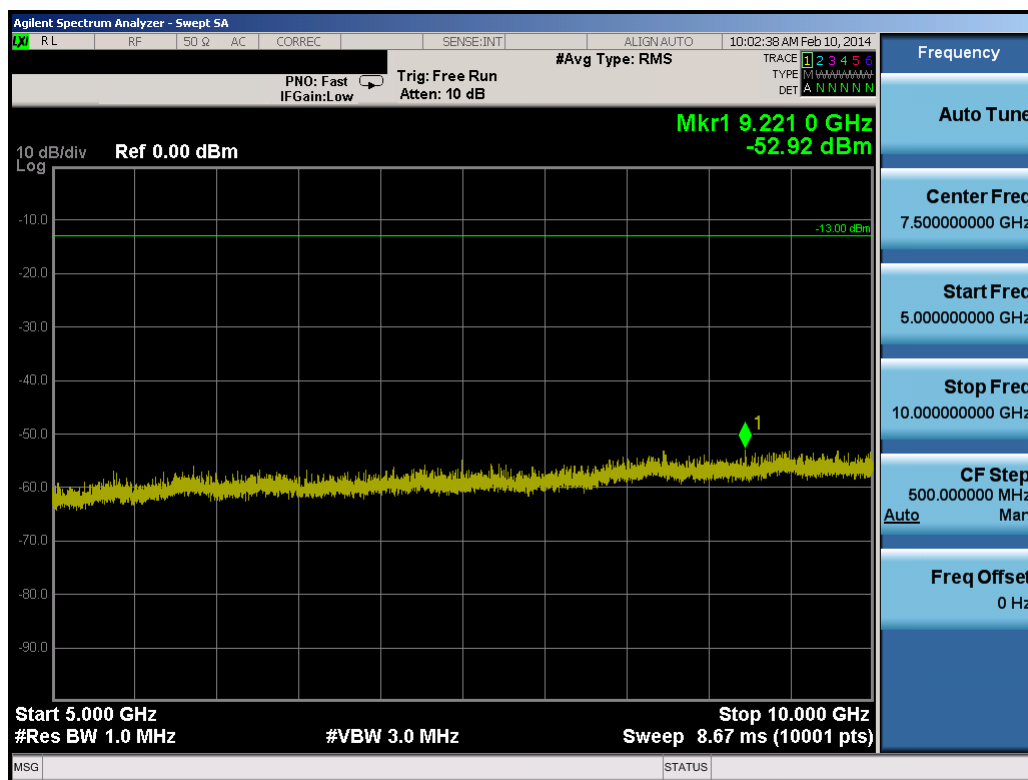
Plot 7-19. Conducted Spurious Plot (3.0MHz QPSK – RB Size 1, RB Offset 0 – High Channel)
