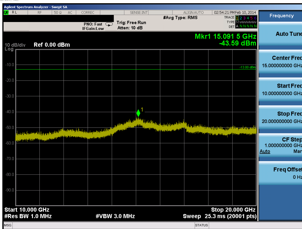
Plot 8-20. Conducted Spurious Plot (3.0MHz QPSK – RB Size 1, RB Offset 0 – Low Channel)
