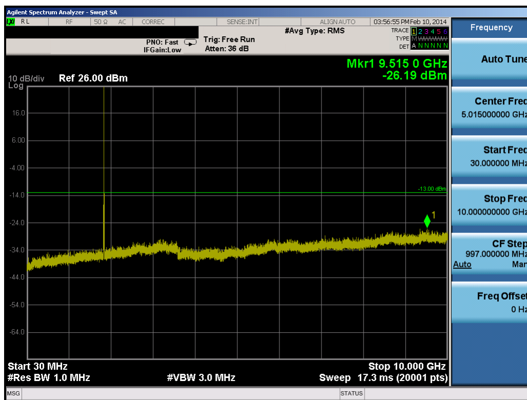
Plot 8-61. Conducted Spurious Plot (15.0MHz QPSK – RB Size 1, RB Offset 0 – Low Channel)
