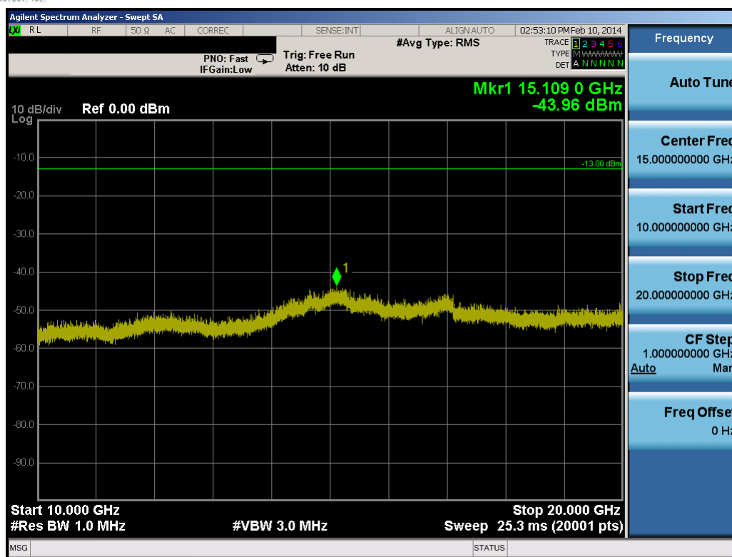
Plot 8-22. Conducted Spurious Plot (3.0MHz QPSK – RB Size 1, RB Offset 0 – Mid Channel)
