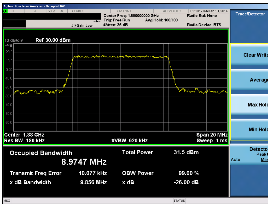
Plot 8-45. Occupied Bandwidth Plot (10.0MHz QPSK – RB Size 50)
