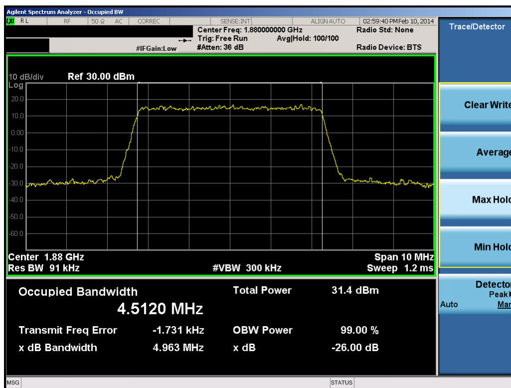
Plot 8-31. Occupied Bandwidth Plot (5.0MHz QPSK – RB Size 25)
