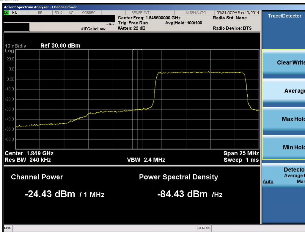
Plot 8-44. Lower Extended Band Edge Plot (10.0MHz QPSK – RB Size 50)
