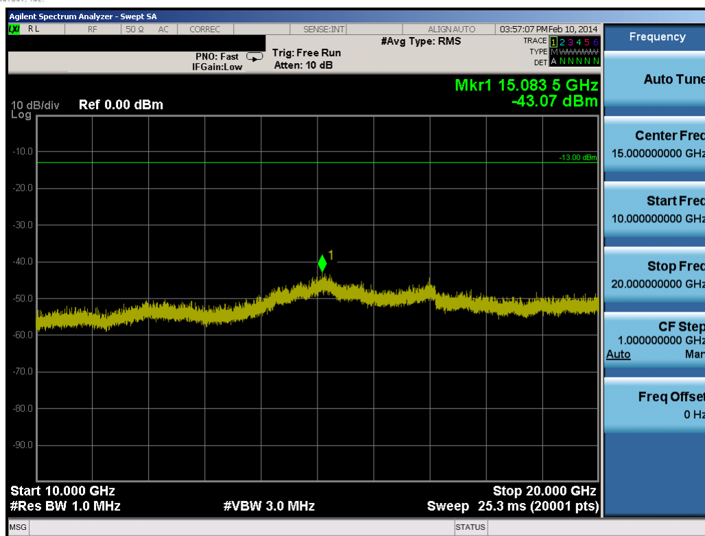
Plot 8-62. Conducted Spurious Plot (15.0MHz QPSK – RB Size 1, RB Offset 0 – Low Channel)
