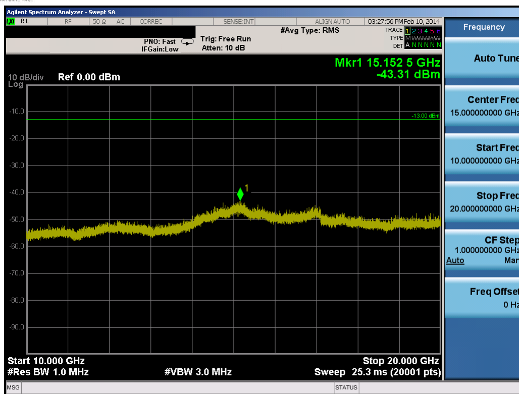
Plot 8-50. Conducted Spurious Plot (10.0MHz QPSK – RB Size 1, RB Offset 0 – Mid Channel)
