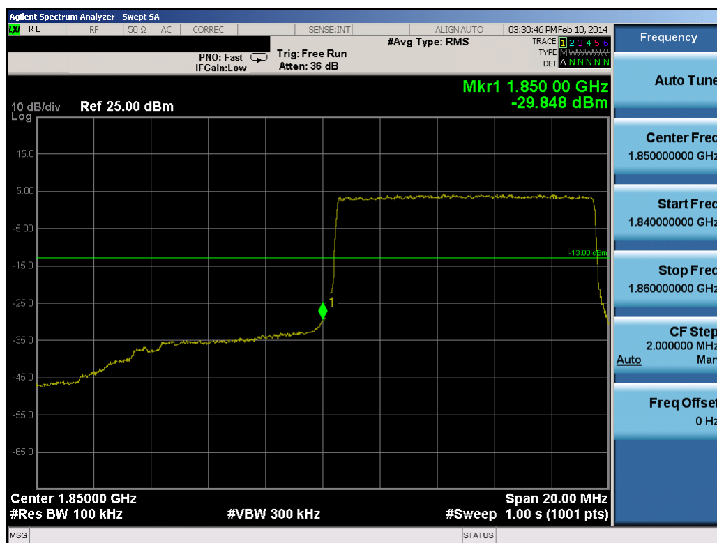
Plot 8-43. Lower Band Edge Plot (10.0MHz QPSK - RB Size 50)
