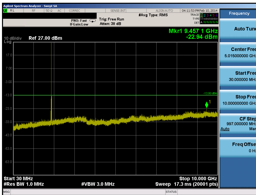
Plot 8-79. Conducted Spurious Plot (20.0MHz QPSK – RB Size 1, RB Offset 0 – High Channel)
