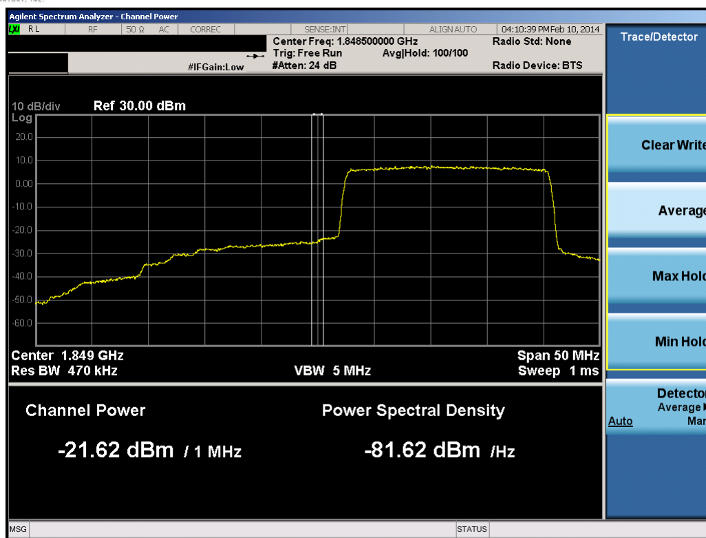
Plot 8-72. Lower Extended Band Edge Plot (20.0MHz QPSK – RB Size 100)
