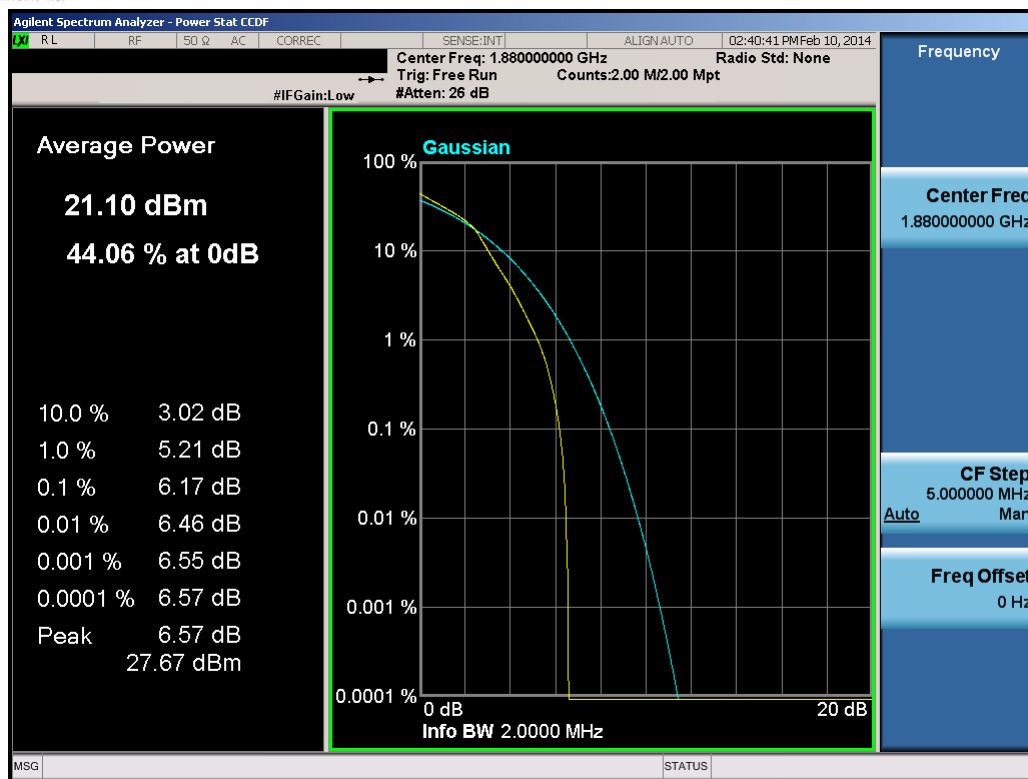
Plot 8-14. PAR Plot (1.4MHz 16-QAM – RB Size 6)
