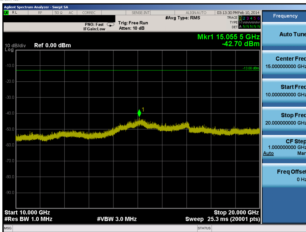
Plot 8-38. Conducted Spurious Plot (5.0MHz QPSK – RB Size 1, RB Offset 0 – High Channel)
