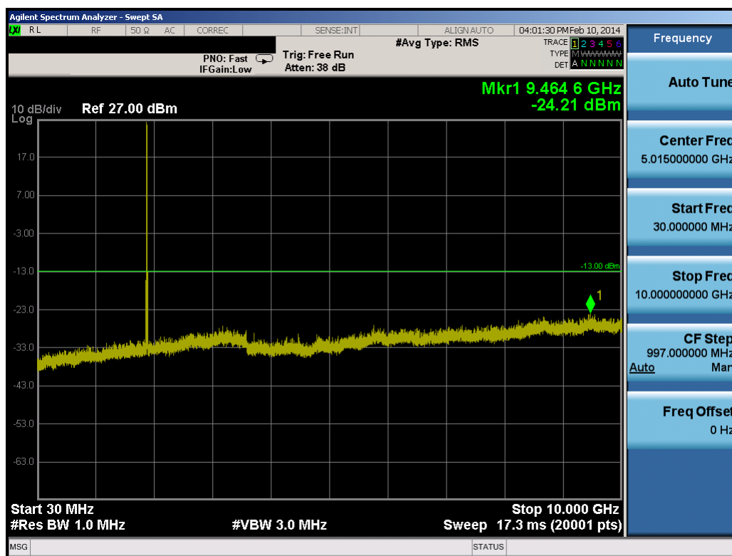
Plot 8-65. Conducted Spurious Plot (15.0MHz QPSK – RB Size 1, RB Offset 0 – High Channel)
