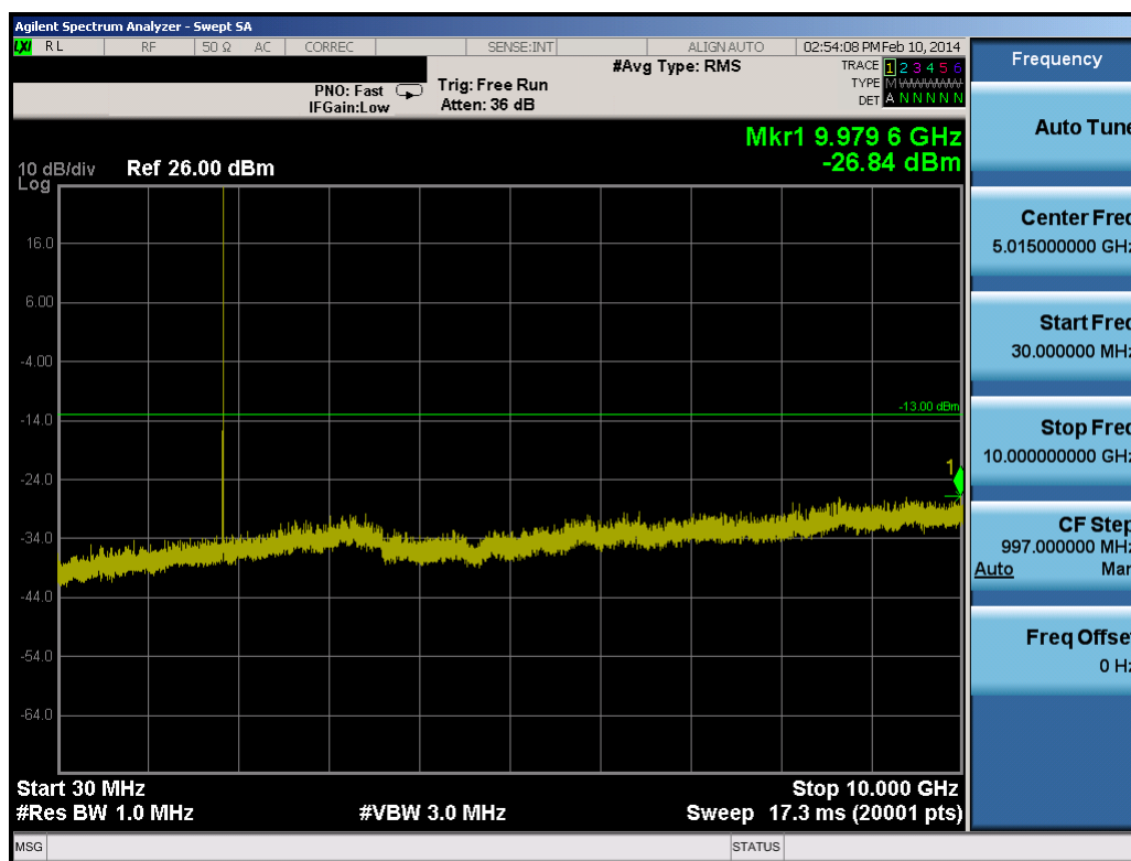
Plot 8-19. Conducted Spurious Plot (3.0MHz QPSK – RB Size 1, RB Offset 0 – Low Channel)
