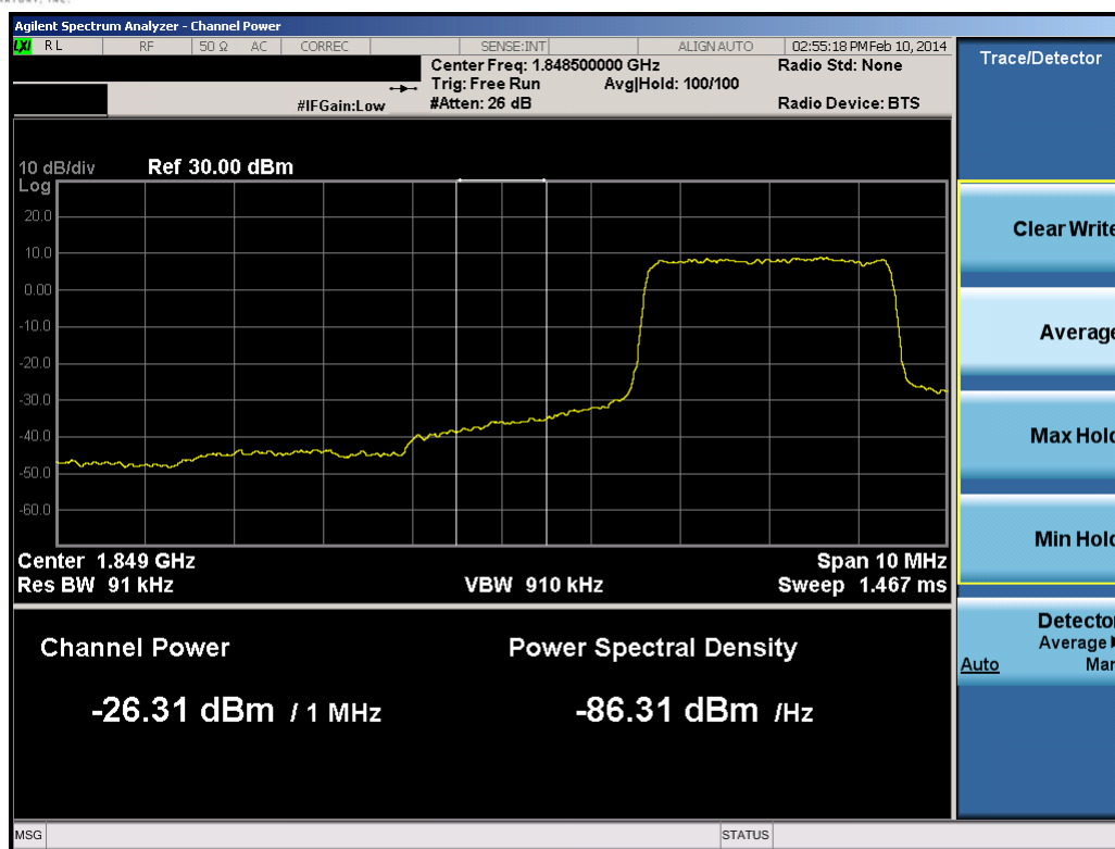
Plot 8-16. Lower Extended Band Edge Plot (3.0MHz QPSK – RB Size 15)
