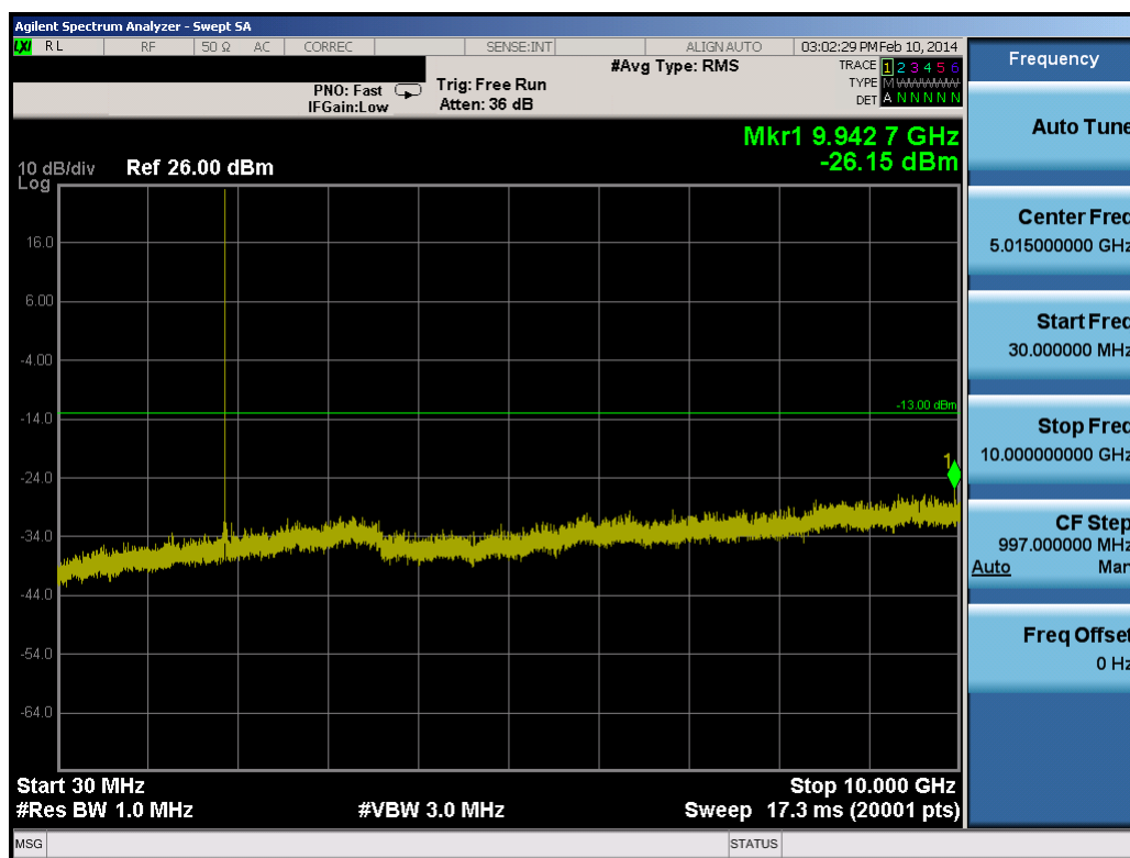
Plot 8-35. Conducted Spurious Plot (5.0MHz QPSK – RB Size 1, RB Offset 0 – Mid Channel)
