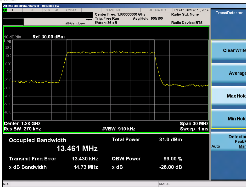
Plot 8-60. Occupied Bandwidth Plot (15.0MHz 16-QAM – RB Size 75)
