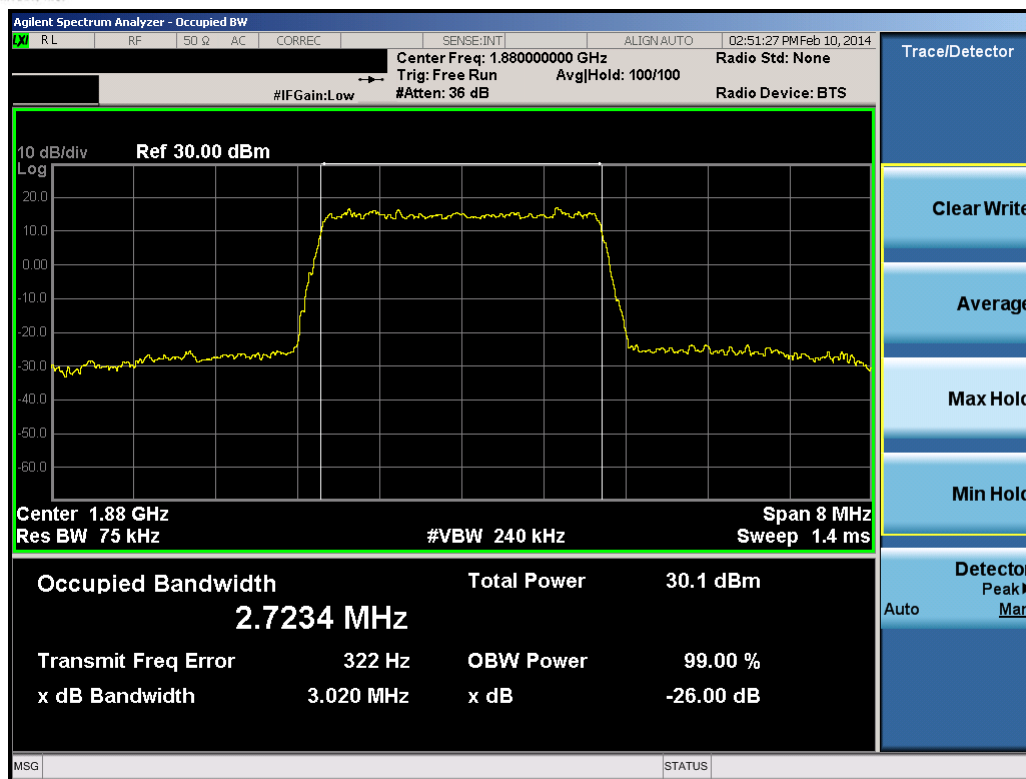
Plot 8-18. Occupied Bandwidth Plot (3.0MHz 16-QAM – RB Size 15)
