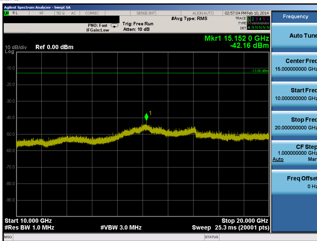
Plot 8-24. Conducted Spurious Plot (3.0MHz QPSK – RB Size 1, RB Offset 0 – High Channel)
