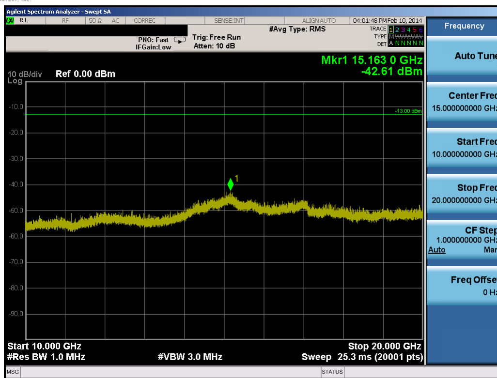
Plot 8-66. Conducted Spurious Plot (15.0MHz QPSK – RB Size 1, RB Offset 0 – High Channel)
