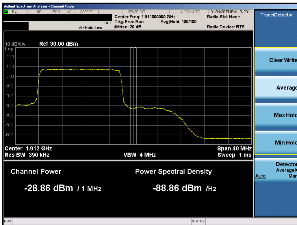
Plot 8-68. Upper Extended Band Edge Plot (15.0MHz QPSK – RB Size 75)
