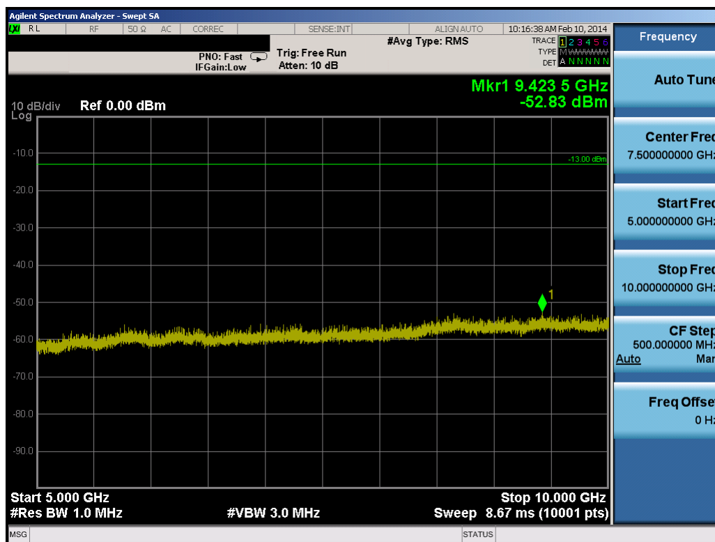
Plot 7-27. Conducted Spurious Plot (5.0MHz QPSK – RB Size 1, RB Offset 0 – Mid Channel)
