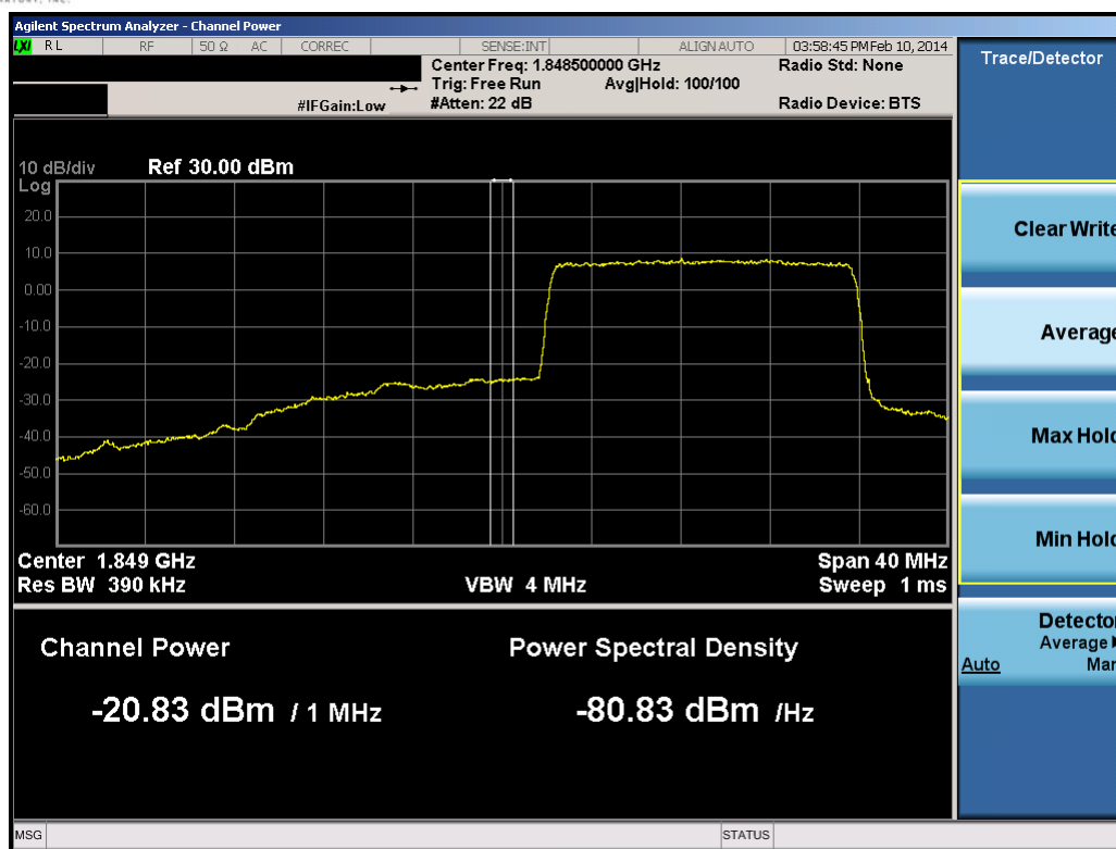
Plot 8-58. Lower Extended Band Edge Plot (15.0MHz QPSK – RB Size 75)
