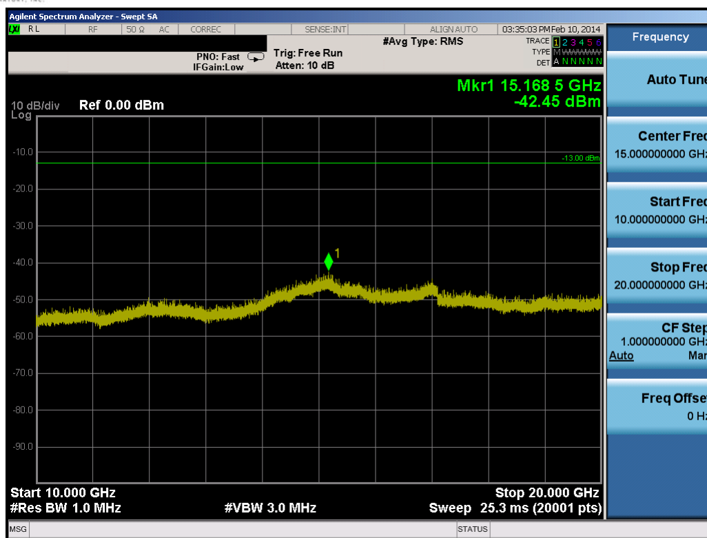
Plot 8-52. Conducted Spurious Plot (10.0MHz QPSK – RB Size 1, RB Offset 0 – High Channel)
