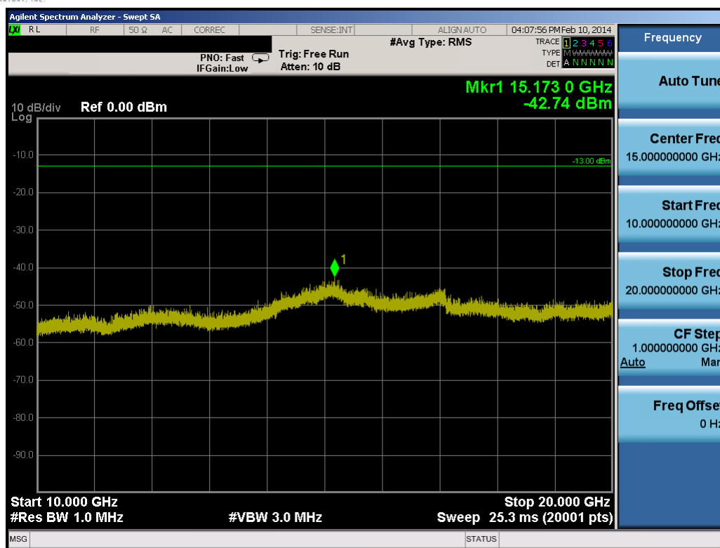
Plot 8-78. Conducted Spurious Plot (20.0MHz QPSK – RB Size 1, RB Offset 0 – Mid Channel)
