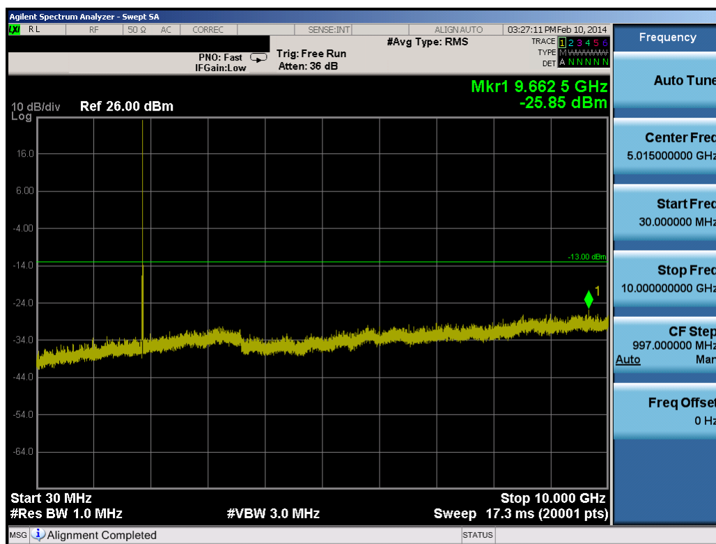
Plot 8-49. Conducted Spurious Plot (10.0MHz QPSK – RB Size 1, RB Offset 0 – Mid Channel)
