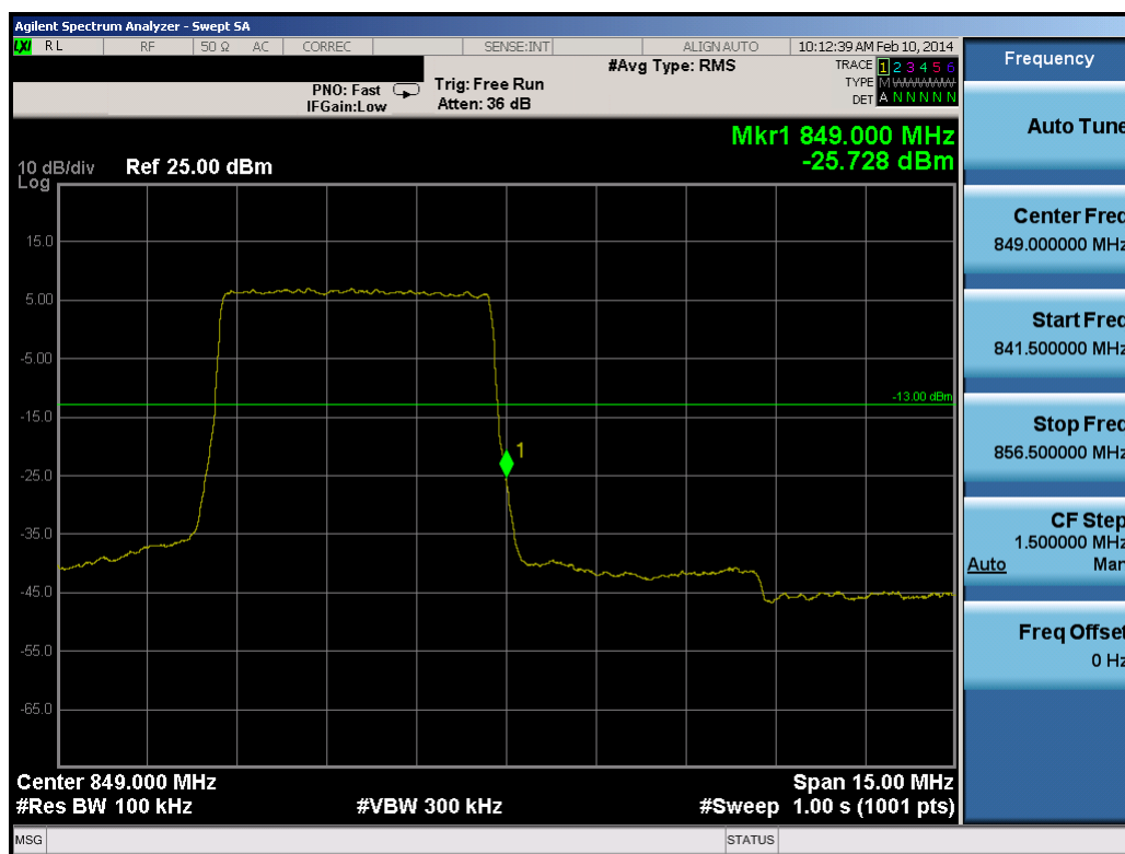
Plot 7-30. Upper Band Edge Plot (5.0MHz QPSK – RB Size 25)
