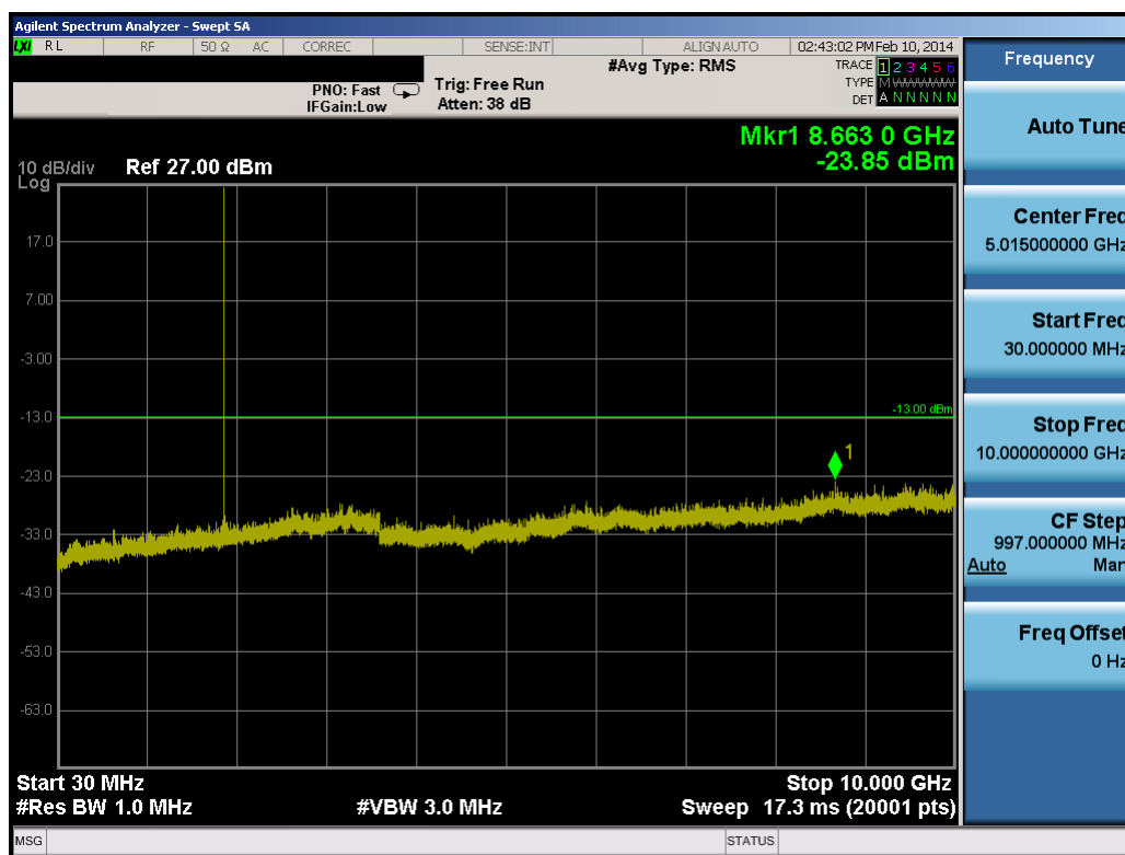
Plot 8-7. Conducted Spurious Plot (1.4MHz QPSK – RB Size 1, RB Offset 0 – Mid Channel)
