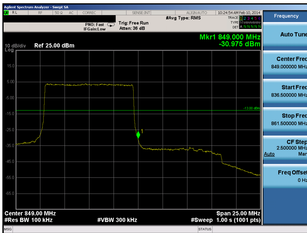
Plot 7-40. Upper Band Edge Plot (10.0MHz QPSK – RB Size 50)
