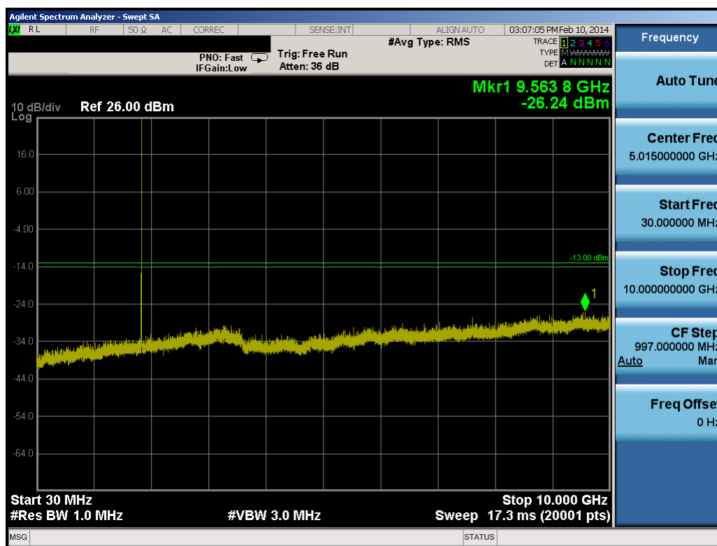
Plot 8-33. Conducted Spurious Plot (5.0MHz QPSK – RB Size 1, RB Offset 0 – Low Channel)
