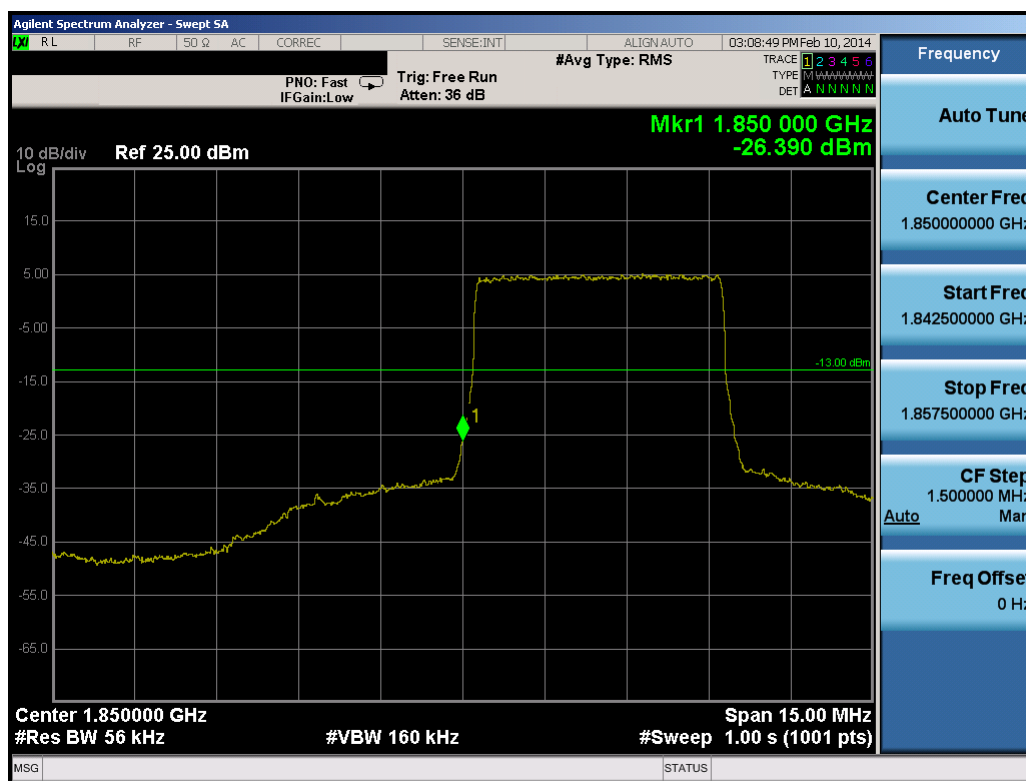
Plot 8-29. Lower Band Edge Plot (5.0MHz QPSK - RB Size 25)
