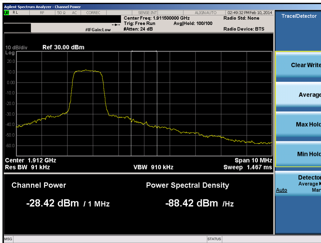
Plot 8-12. Upper Extended Band Edge Plot (1.4MHz QPSK – RB Size 6)
