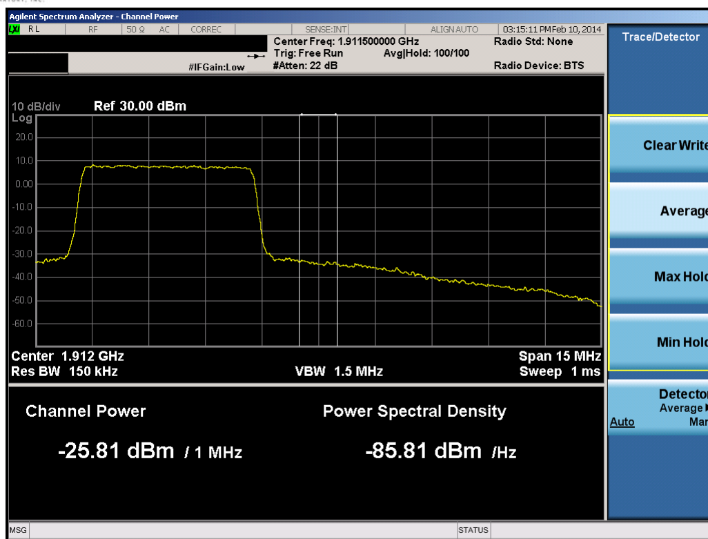
Plot 8-40. Upper Extended Band Edge Plot (5.0MHz QPSK – RB Size 25)
