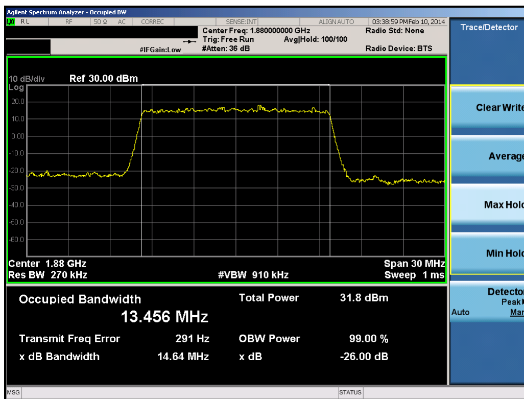
Plot 8-59. Occupied Bandwidth Plot (15.0MHz QPSK – RB Size 75)
