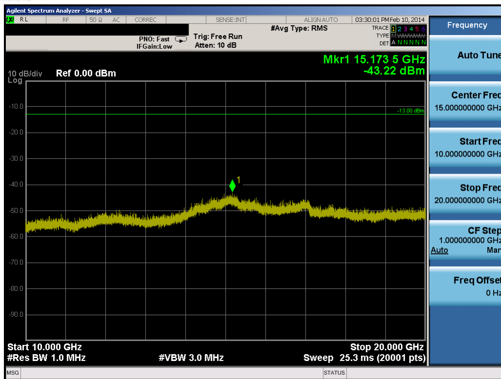
Plot 8-48. Conducted Spurious Plot (10.0MHz QPSK – RB Size 1, RB Offset 0 – Low Channel)
