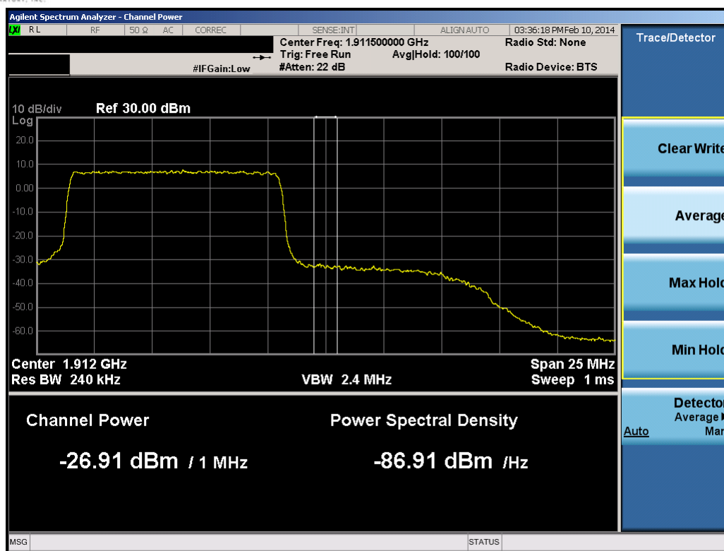
Plot 8-54. Upper Extended Band Edge Plot (10.0MHz QPSK – RB Size 50)
