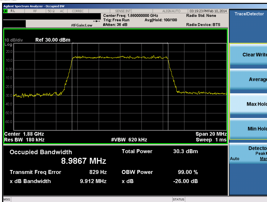
Plot 8-46. Occupied Bandwidth Plot (10.0MHz 16-QAM – RB Size 50)
