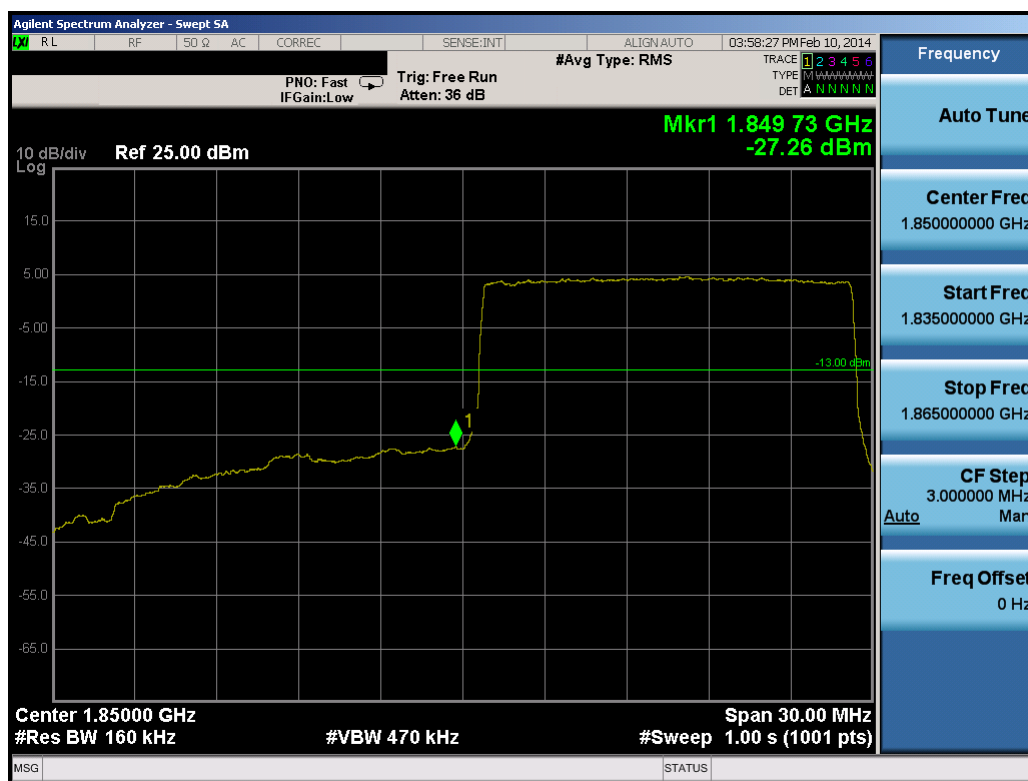
Plot 8-57. Lower Band Edge Plot (15.0MHz QPSK – RB Size 75)
