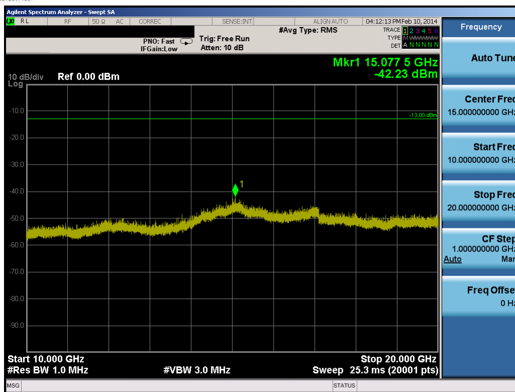
Plot 8-80. Conducted Spurious Plot (20.0MHz QPSK – RB Size 1, RB Offset 0 – High Channel)
