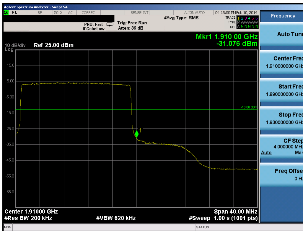
Plot 8-81. Upper Band Edge Plot (20.0MHz QPSK – RB Size 100)
