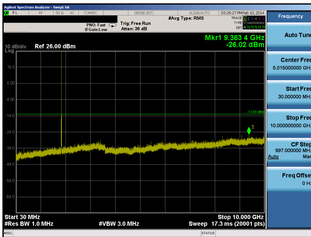
Plot 8-47. Conducted Spurious Plot (10.0MHz QPSK – RB Size 1, RB Offset 0– Low Channel)
