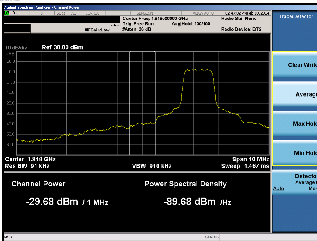
Plot 8-2. Lower Extended Band Edge Plot (1.4MHz QPSK – RB Size 6)
