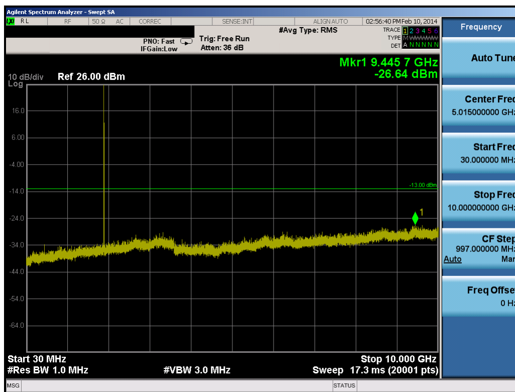
Plot 8-23. Conducted Spurious Plot (3.0MHz QPSK – RB Size 1, RB Offset 0 – High Channel)
