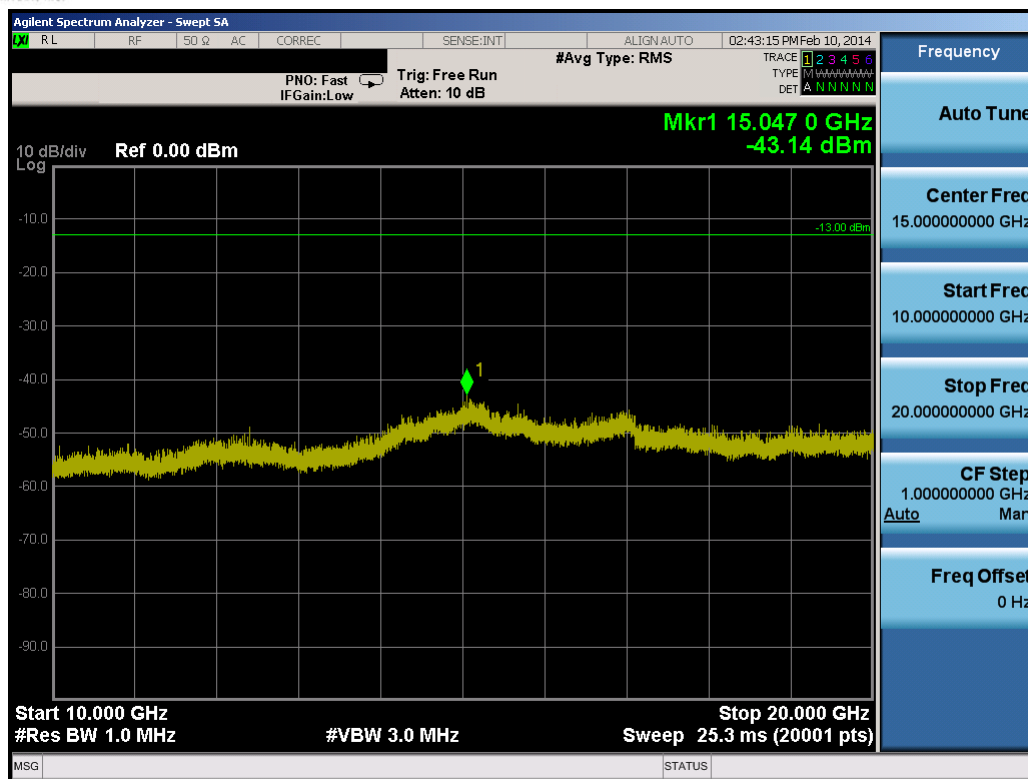
Plot 8-8. Conducted Spurious Plot (1.4MHz QPSK – RB Size 1, RB Offset 0 – Mid Channel)
