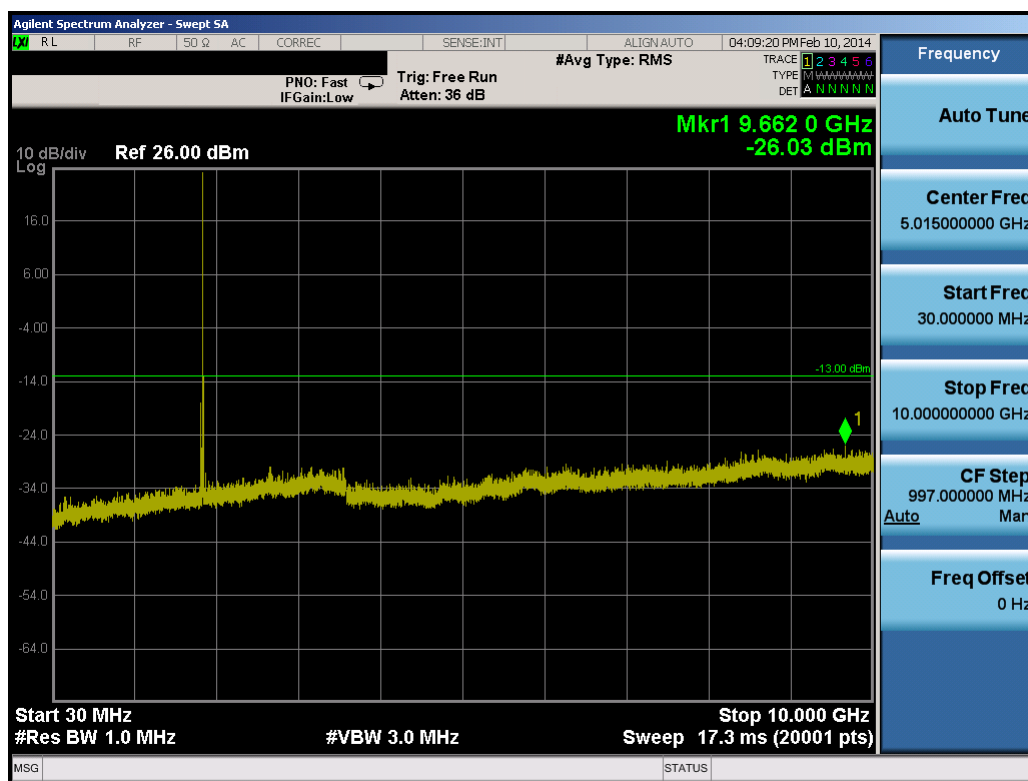
Plot 8-75. Conducted Spurious Plot (20.0MHz QPSK – RB Size 1, RB Offset 0– Low Channel)
