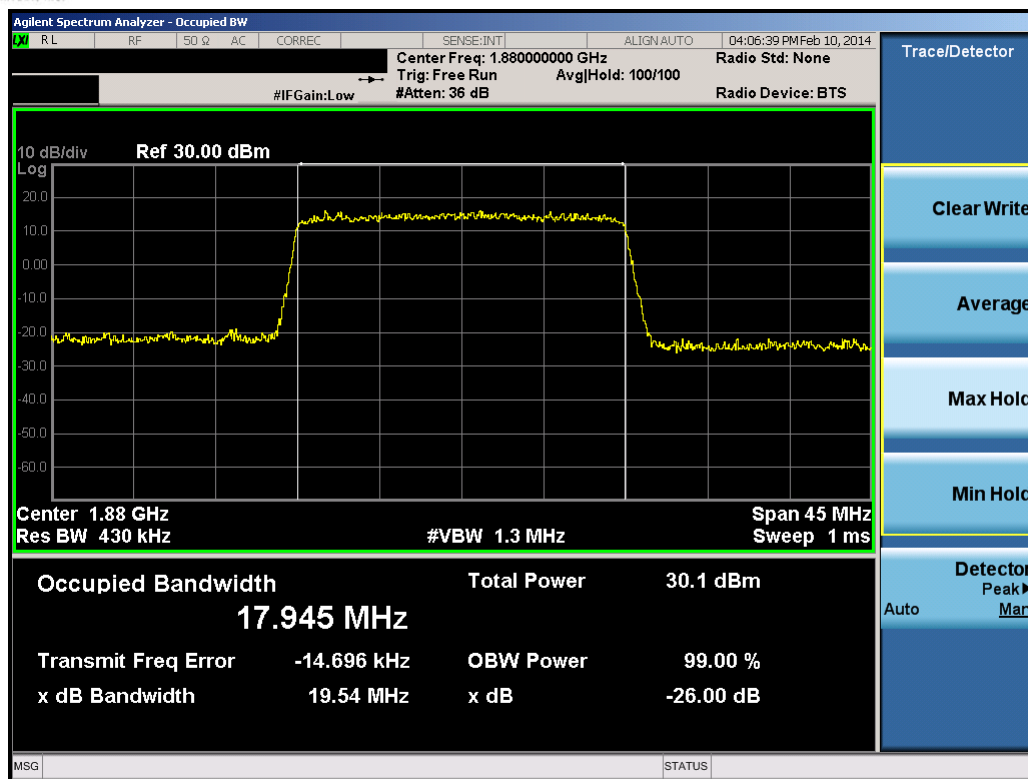
Plot 8-74. Occupied Bandwidth Plot (20.0MHz 16-QAM – RB Size 100)
