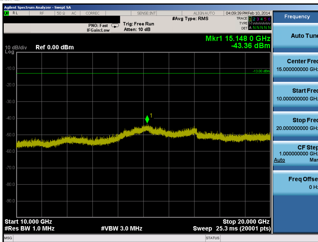
Plot 8-76. Conducted Spurious Plot (20.0MHz QPSK – RB Size 1, RB Offset 0 – Low Channel)
