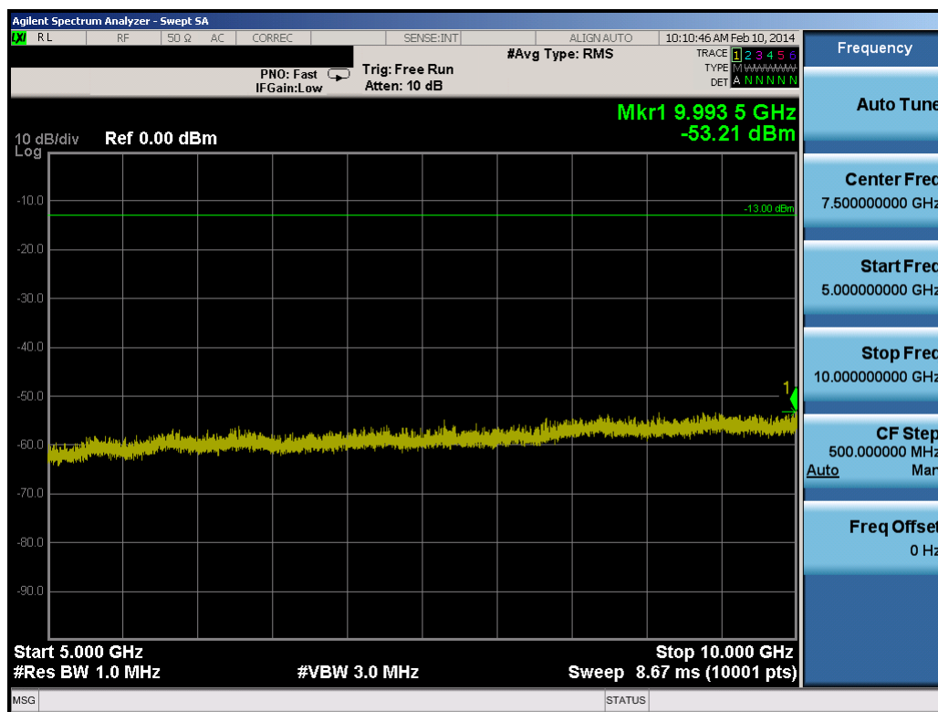
Plot 7-29. Conducted Spurious Plot (5.0MHz QPSK – RB Size 1, RB Offset 0 – High Channel)
