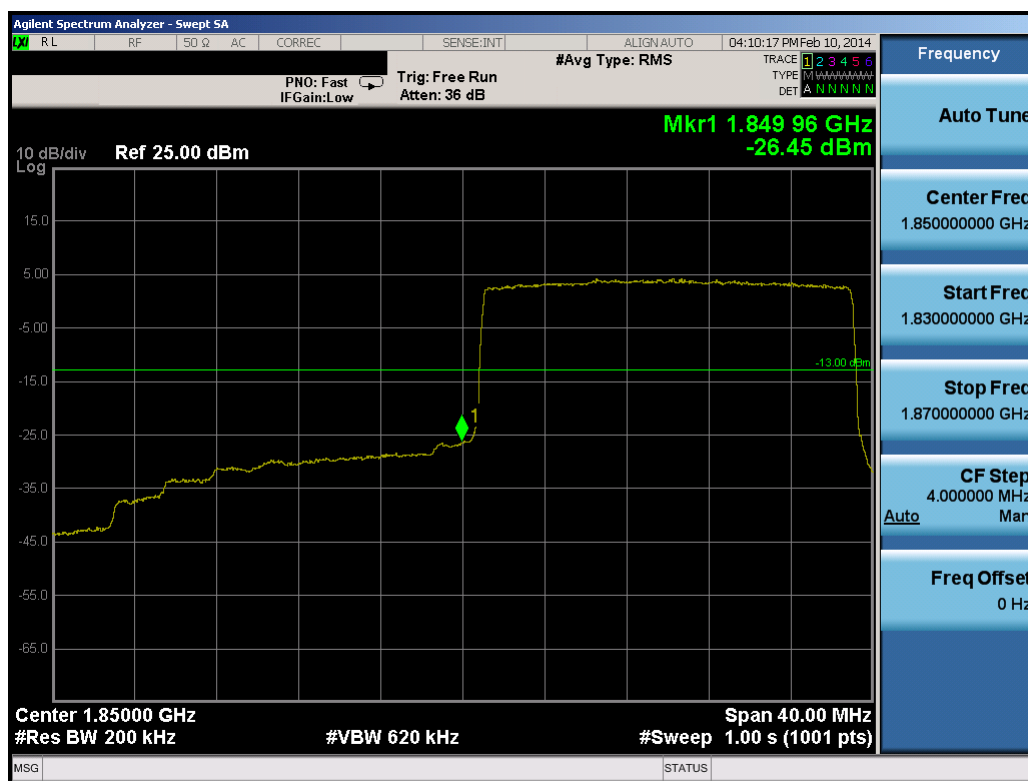
Plot 8-71. Lower Band Edge Plot (20.0MHz QPSK – RB Size 100)
