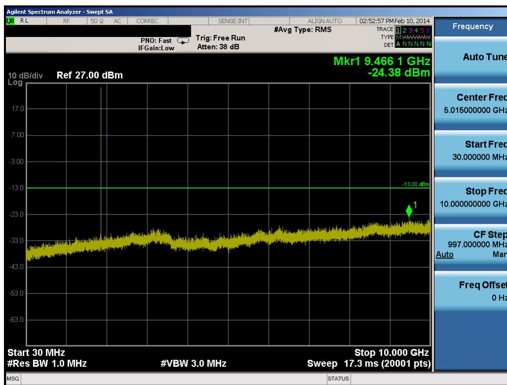
Plot 8-21. Conducted Spurious Plot (3.0MHz QPSK – RB Size 1, RB Offset 0 – Mid Channel)
