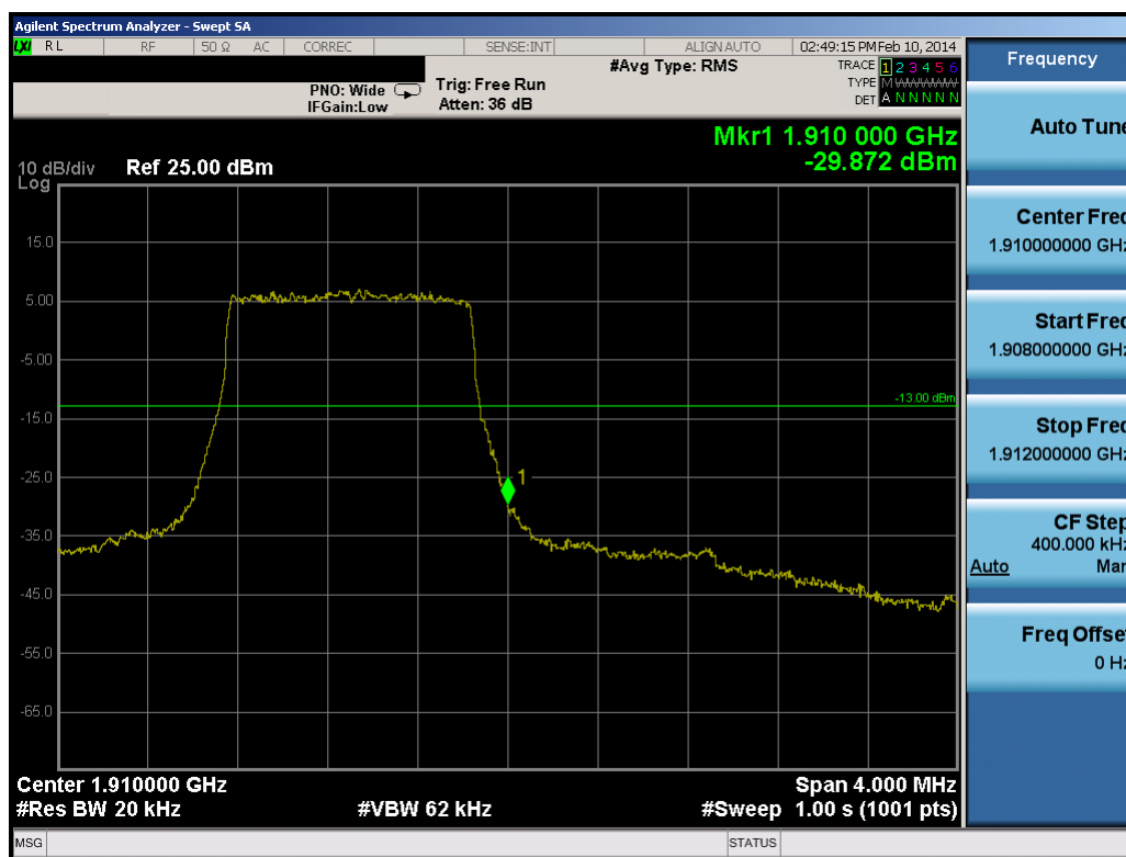
Plot 8-11. Upper Band Edge Plot (1.4MHz QPSK – RB Size 6)
