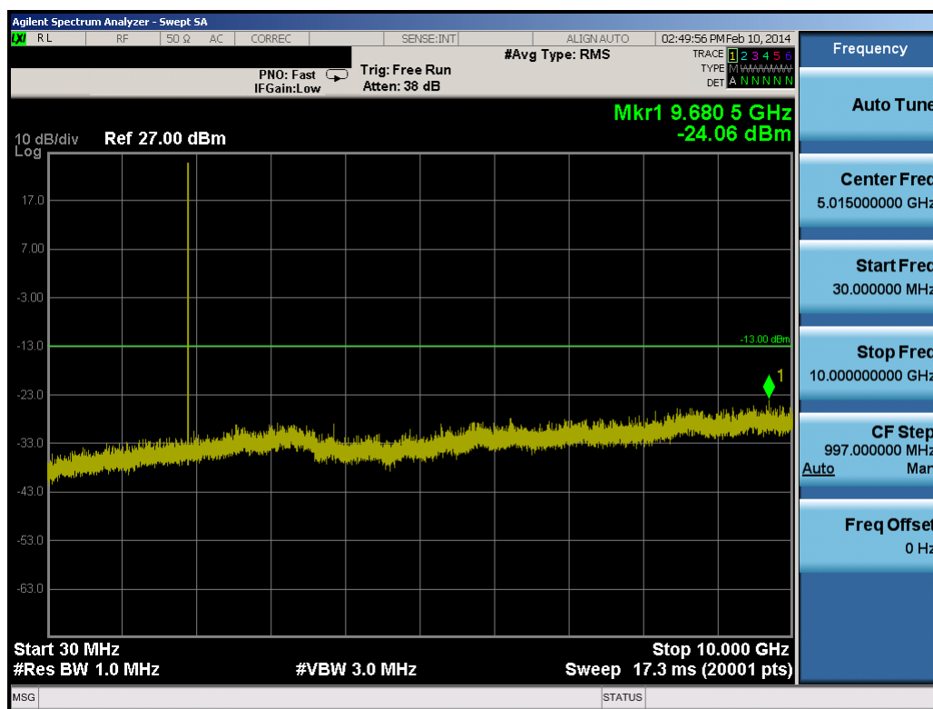
Plot 8-9. Conducted Spurious Plot (1.4MHz QPSK – RB Size 1, RB Offset 0 – High Channel)
