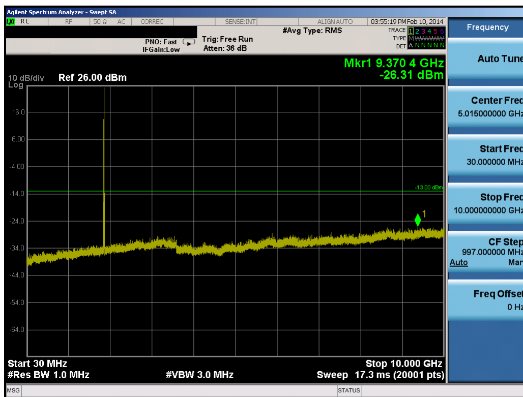
Plot 8-63. Conducted Spurious Plot (15.0MHz QPSK – RB Size 1, RB Offset 0 – Mid Channel)
