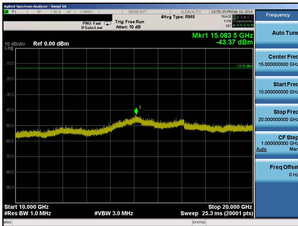
Plot 8-64. Conducted Spurious Plot (15.0MHz QPSK – RB Size 1, RB Offset 0 – Mid Channel)
