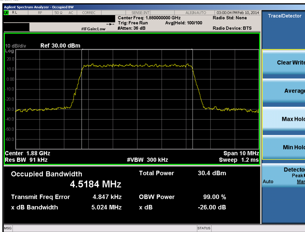
Plot 8-32. Occupied Bandwidth Plot (5.0MHz 16-QAM – RB Size 25)
