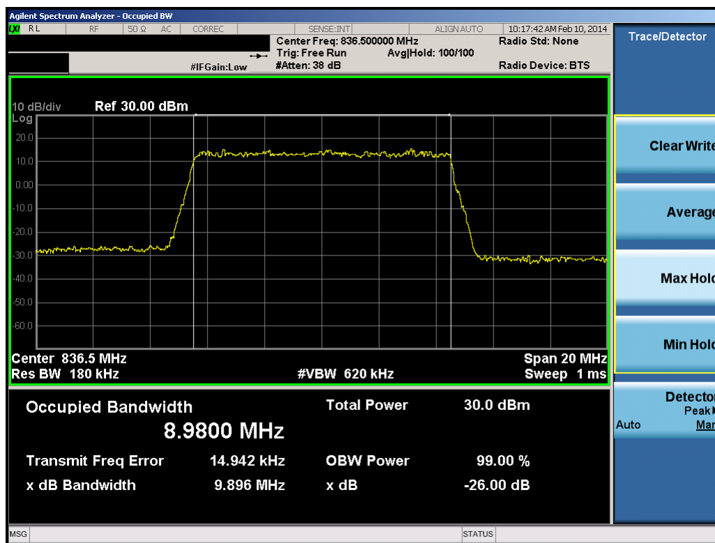
Plot 7-33. Occupied Bandwidth Plot (10.0MHz 16-QAM – RB Size 50)
