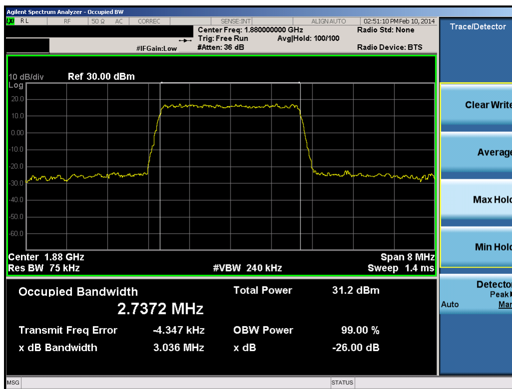
Plot 8-17. Occupied Bandwidth Plot (3.0MHz QPSK – RB Size 15)
