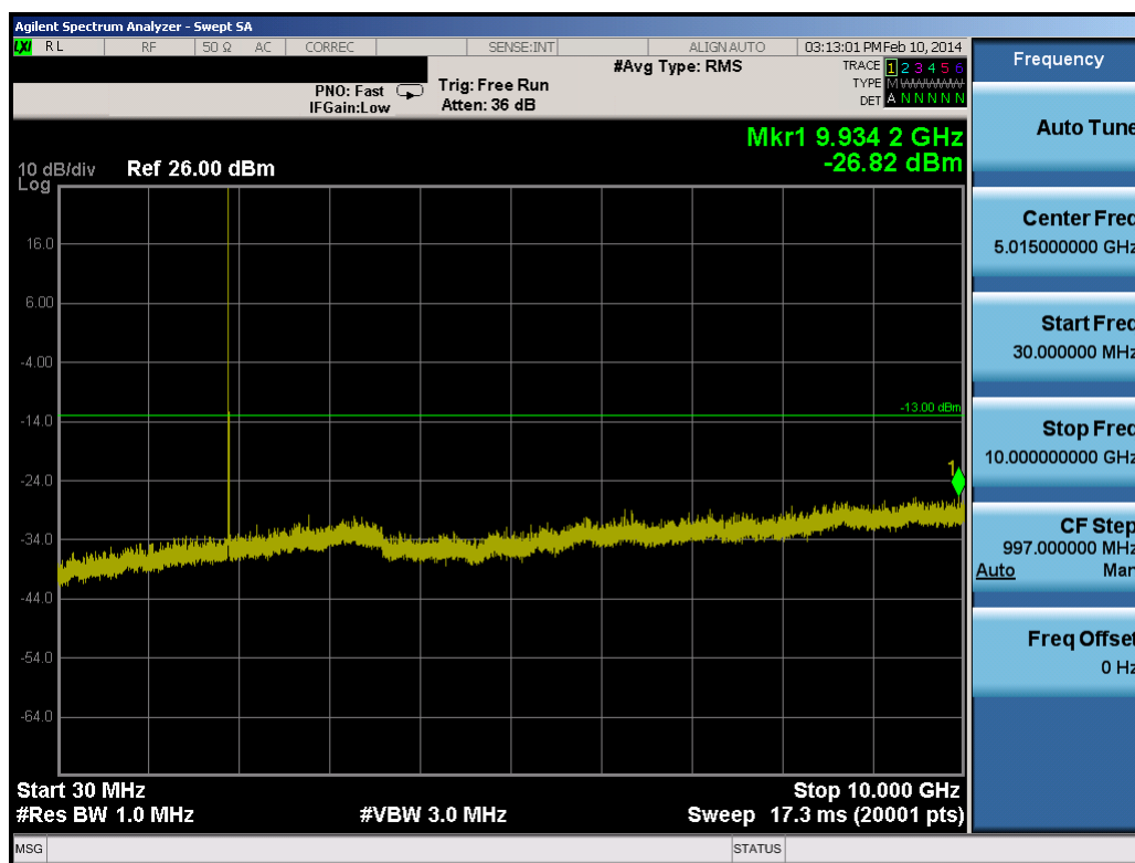
Plot 8-37. Conducted Spurious Plot (5.0MHz QPSK – RB Size 1, RB Offset 0 – High Channel)
