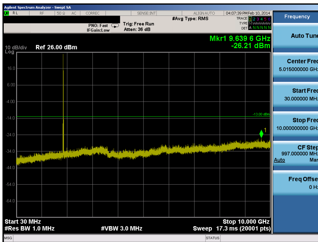
Plot 8-77. Conducted Spurious Plot (20.0MHz QPSK – RB Size 1, RB Offset 0 – Mid Channel)
