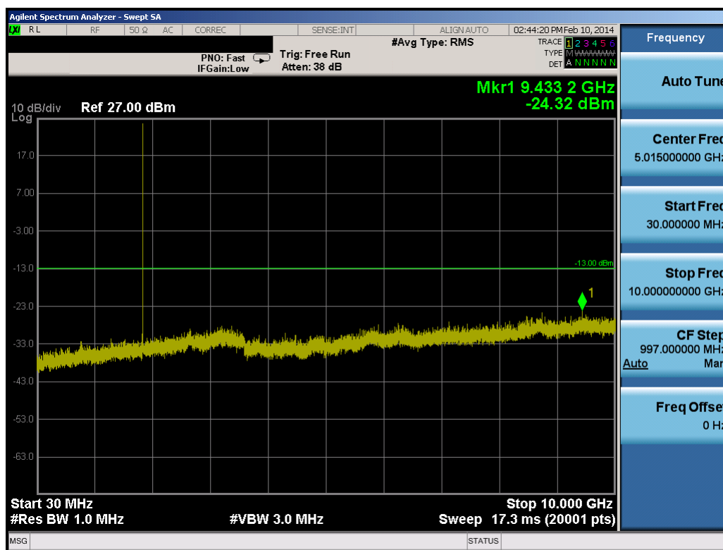
Plot 8-5. Conducted Spurious Plot (1.4MHz QPSK – RB Size 1, RB Offset 0 – Low Channel)
