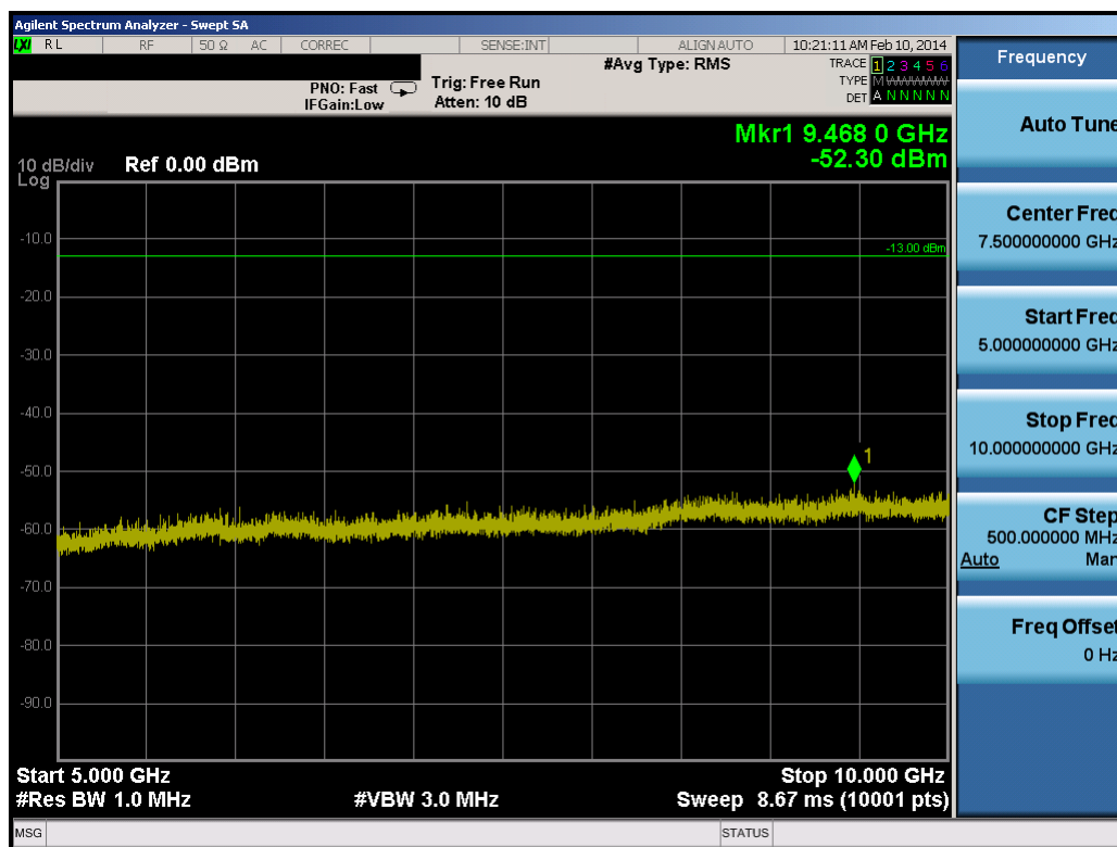
Plot 7-35. Conducted Spurious Plot (10.0MHz QPSK – RB Size 1, RB Offset 0 – Low Channel)
