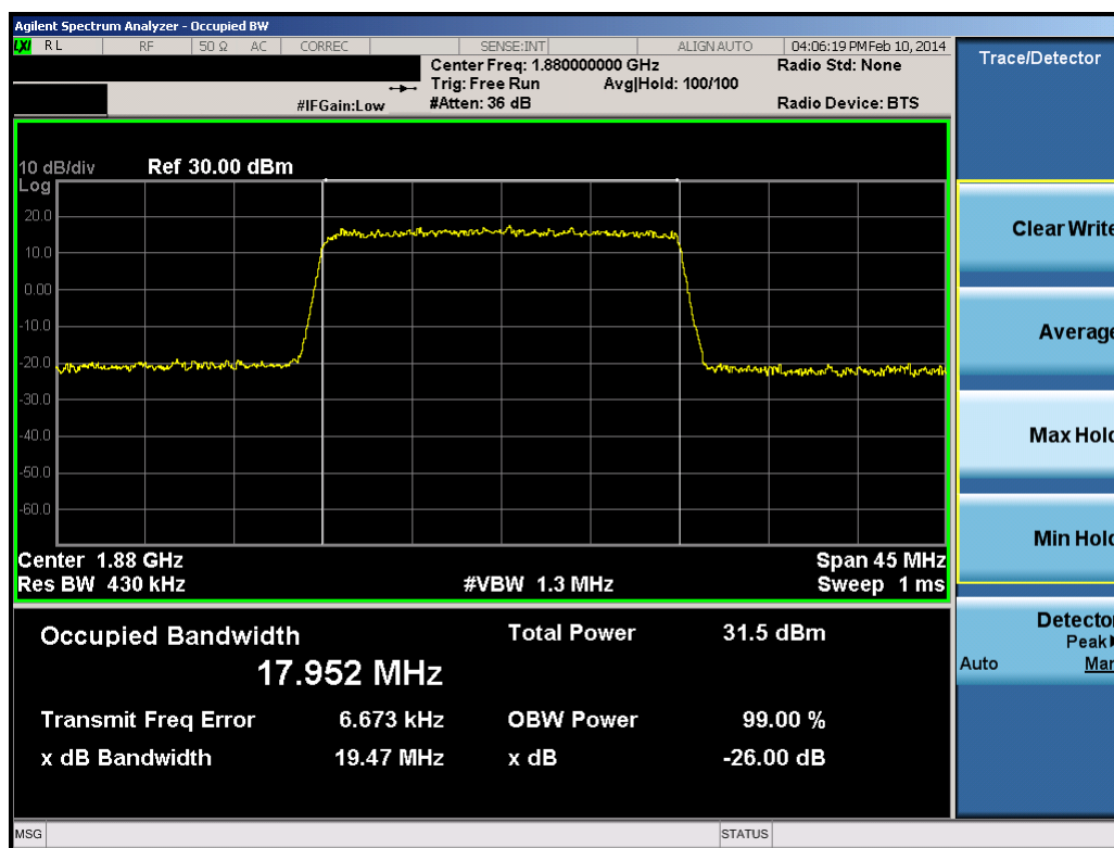
Plot 8-73. Occupied Bandwidth Plot (20.0MHz QPSK – RB Size 100)
