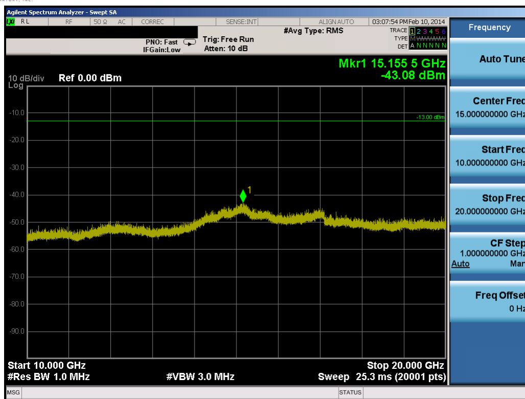
Plot 8-34. Conducted Spurious Plot (5.0MHz QPSK – RB Size 1, RB Offset 0 – Low Channel)
