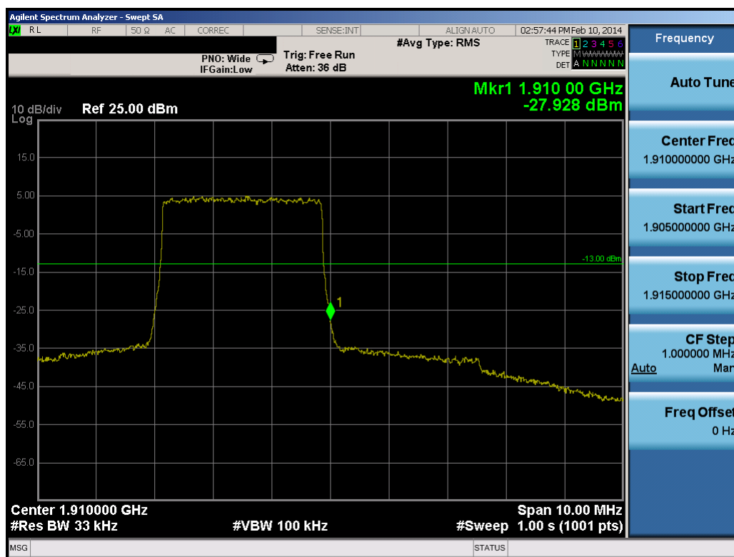
Plot 8-25. Upper Band Edge Plot (3.0MHz QPSK – RB Size 15)
