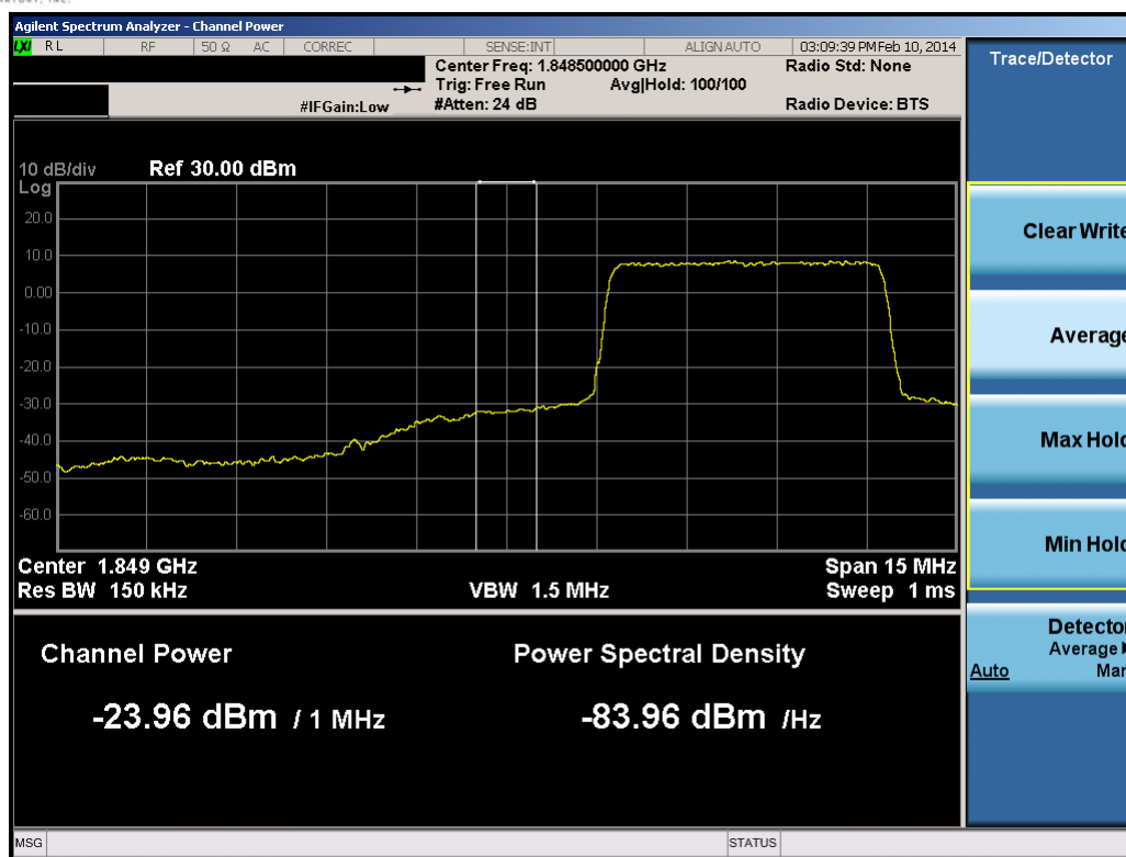
Plot 8-30. Lower Extended Band Edge Plot (5.0MHz QPSK – RB Size 25)
