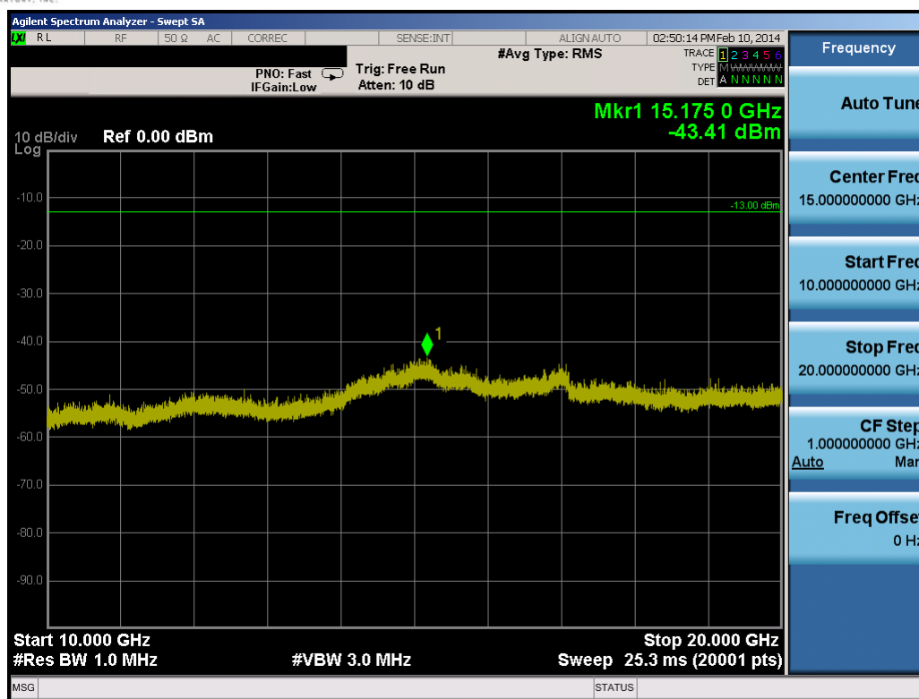
Plot 8-10. Conducted Spurious Plot (1.4MHz QPSK – RB Size 1, RB Offset 0 – High Channel)
