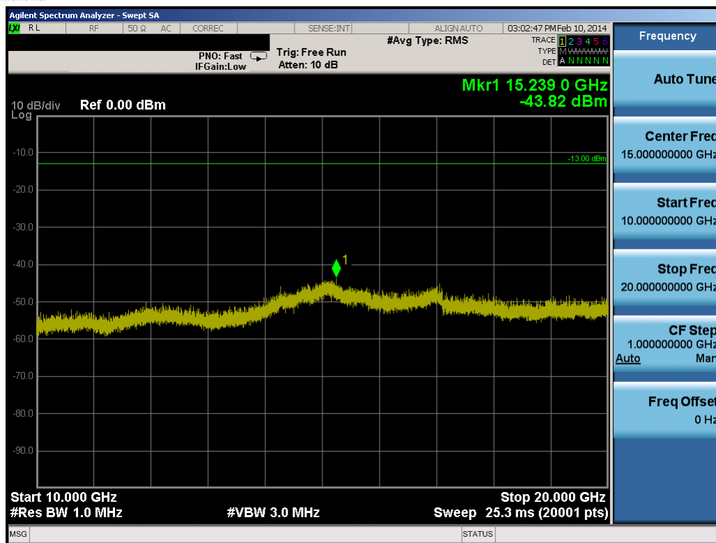
Plot 8-36. Conducted Spurious Plot (5.0MHz QPSK – RB Size 1, RB Offset 0 – Mid Channel)
