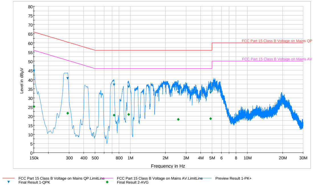
Plot 6-203. Line Conducted Plot with 802.11a UNII Band 2C (L1)
