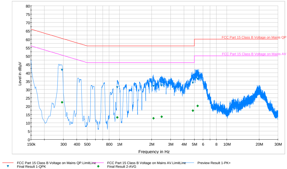
Plot 6-202. Line Conducted Plot with 802.11a UNII Band 2A (N)
