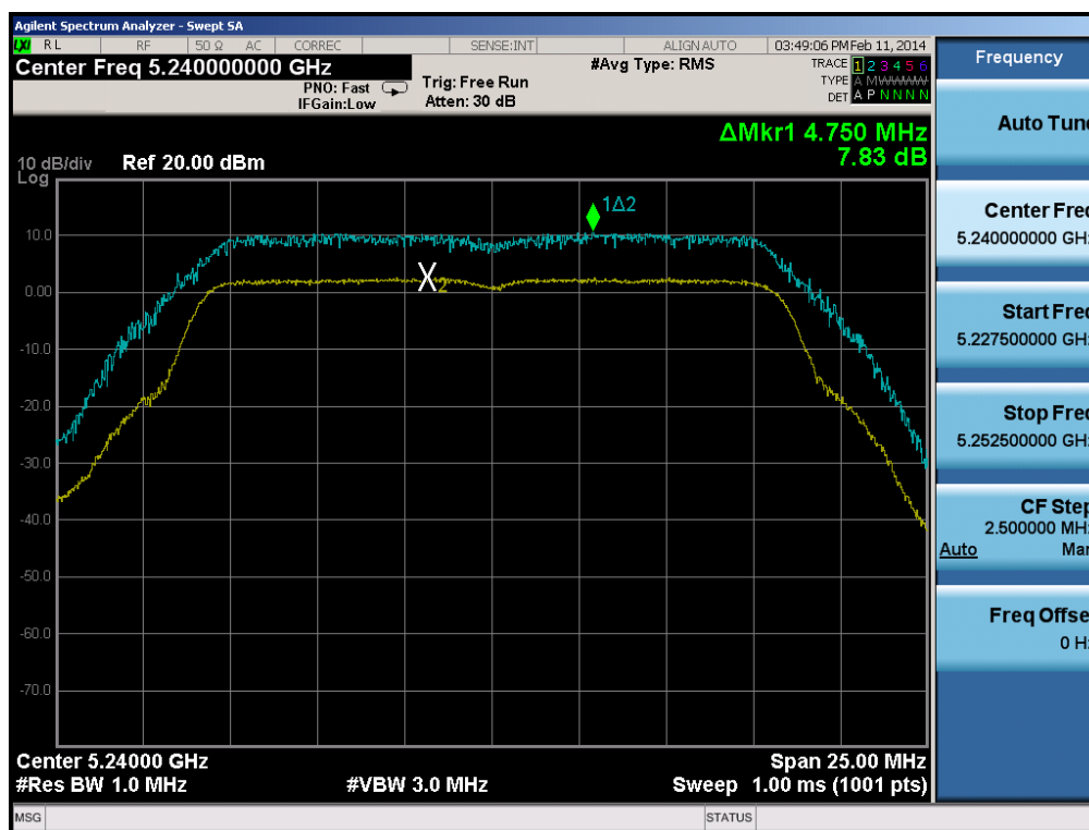
Plot 6-135. Peak Excursion Ratio Plot (802.11a (UNII Band 1) – Ch. 48)
