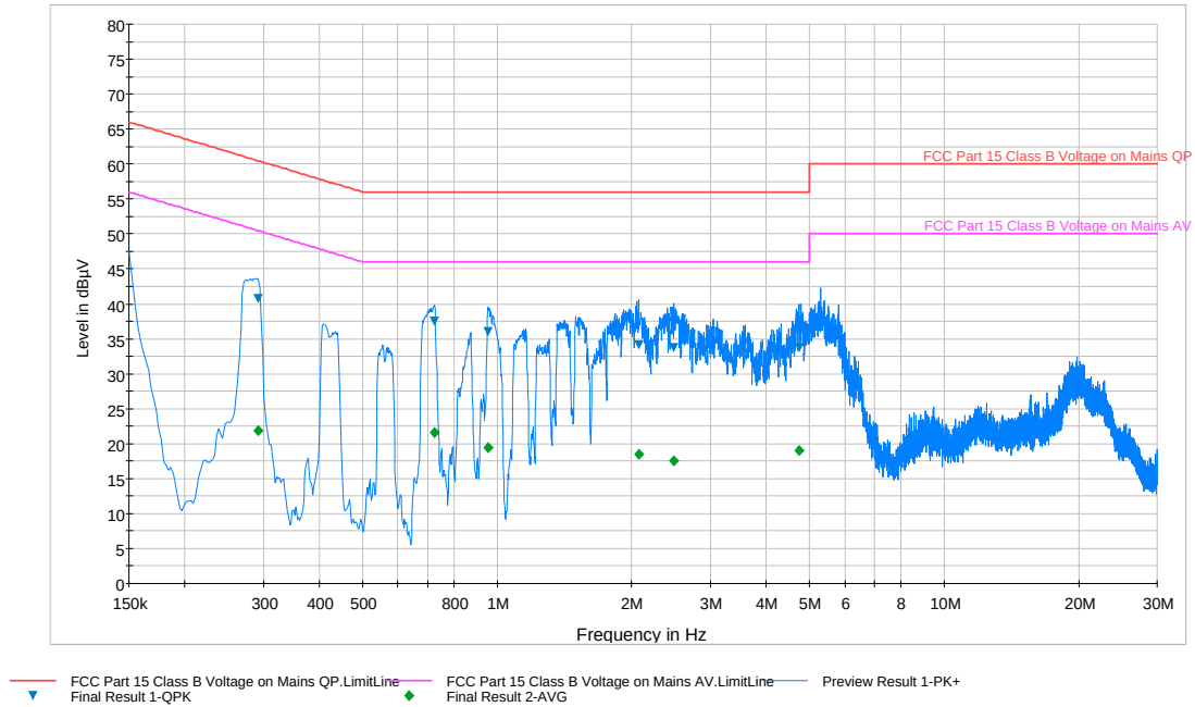
Plot 6-199. Line Conducted Plot with 802.11a UNII Band 1 (L1)
