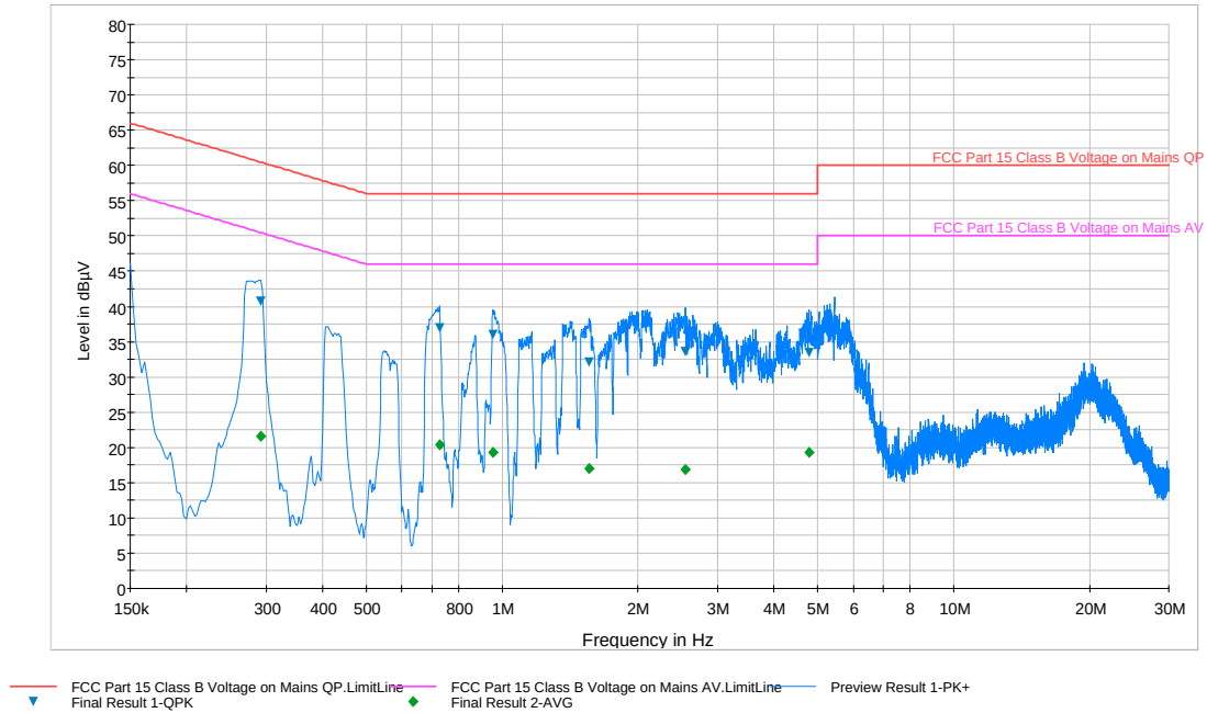
Plot 6-201. Line Conducted Plot with 802.11a UNII Band 2A (L1)
