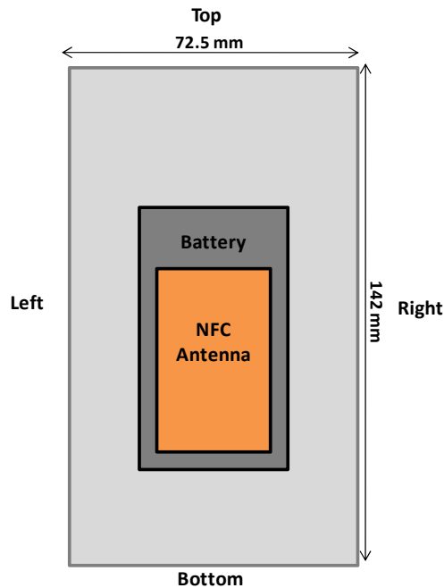
Figure 1-2 DUT Antenna Locations
