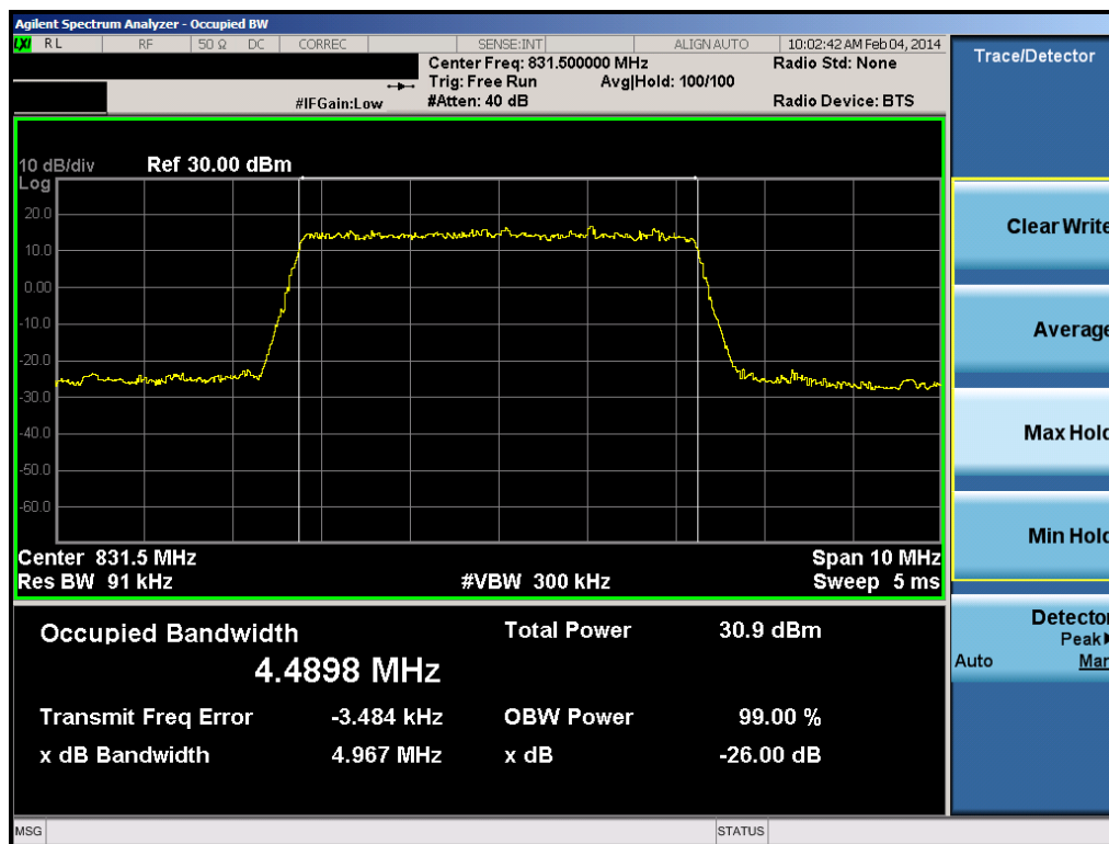
Plot 7-10. Occupied Bandwidth Plot (5.0MHz QPSK – RB Size 25)
