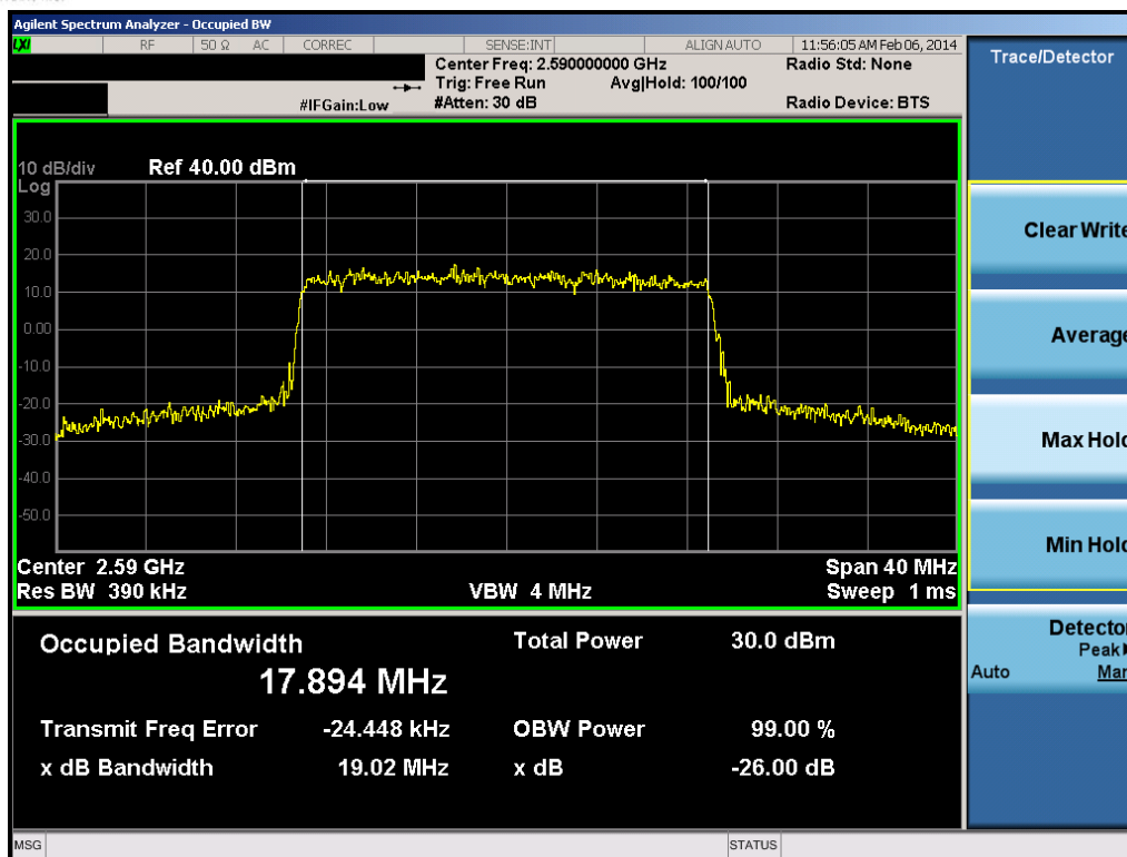
Plot 9-23. Occupied Bandwidth Plot (20.0MHz QPSK – RB Size 100)
