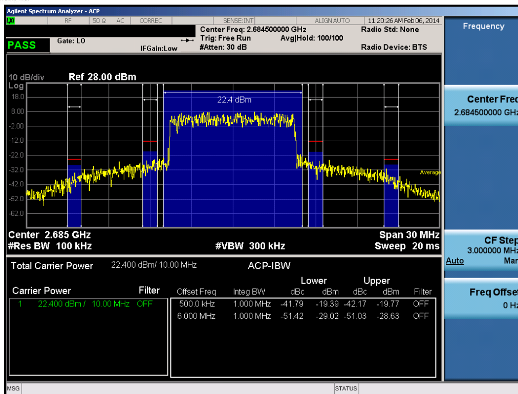
Plot 9-3. High Adjacent Channel Band Edge Plot (10.0MHz QPSK – RB Size 50)
