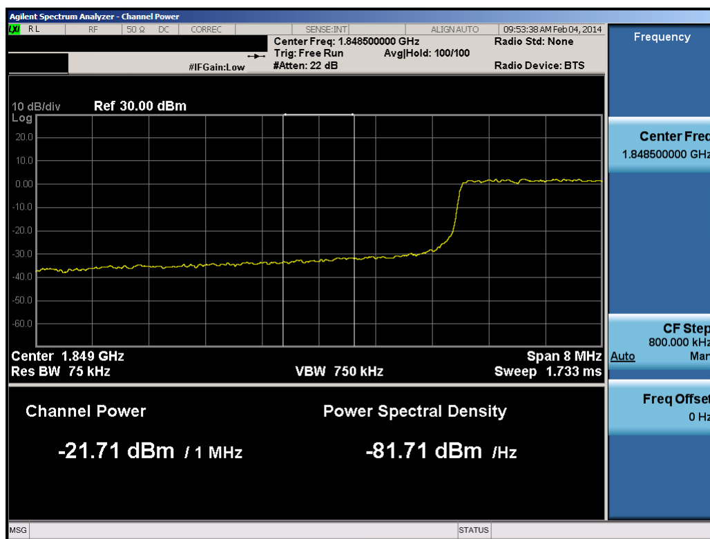
Plot 8-24. Lower Extended Band Edge Plot (10.0MHz QPSK – RB Size 50)
