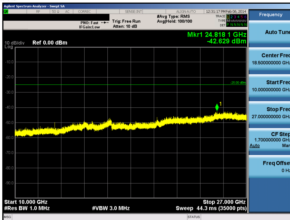
Plot 9-11. Conducted Spurious Plot (10.0MHz QPSK – RB Size 1, RB Offset 0 – Mid Channel)
