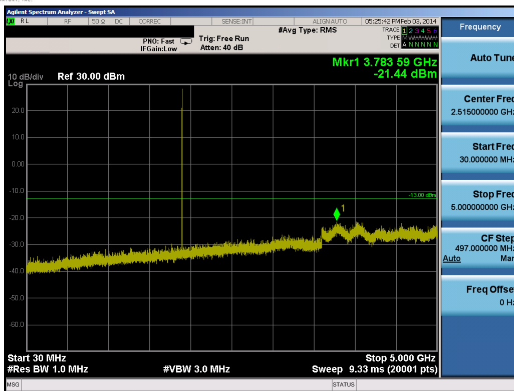
Plot 8-9. Conducted Spurious Plot (3.0MHz QPSK – RB Size 1, RB Offset 0 – High Channel)
