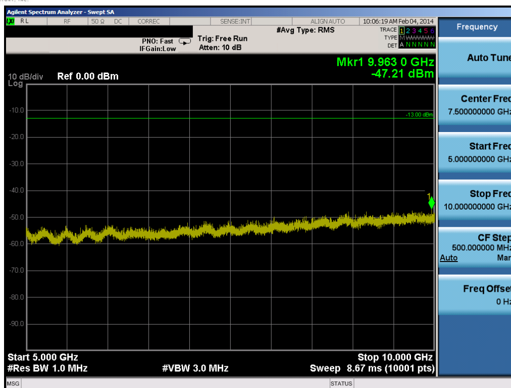
Plot 7-13. Conducted Spurious Plot (5.0MHz QPSK – RB Size 1, RB Offset 0 – Low Channel)
