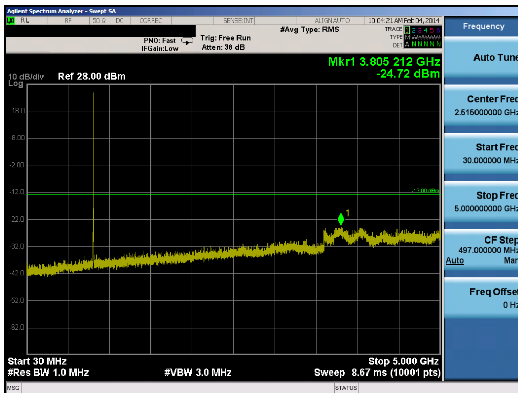
Plot 7-14. Conducted Spurious Plot (5.0MHz QPSK – RB Size 1, RB Offset 0 – Mid Channel)
