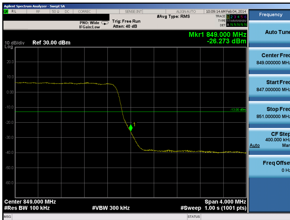
Plot 7-18. Upper Band Edge Plot (5.0MHz QPSK – RB Size 25)
