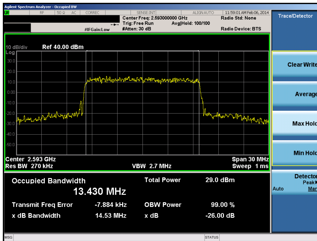
Plot 9-18. Occupied Bandwidth Plot (15.0MHz QPSK – RB Size 75)
