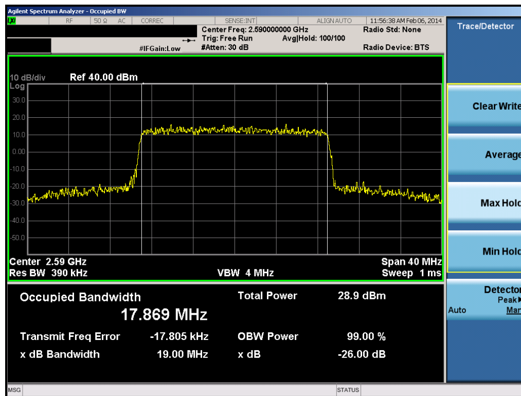
Plot 9-24. Occupied Bandwidth Plot (20.0MHz 16-QAM – RB Size 100)
