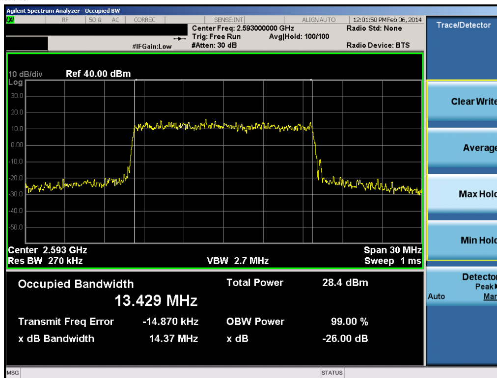
Plot 9-19. Occupied Bandwidth Plot (15.0MHz 16-QAM – RB Size 75)
