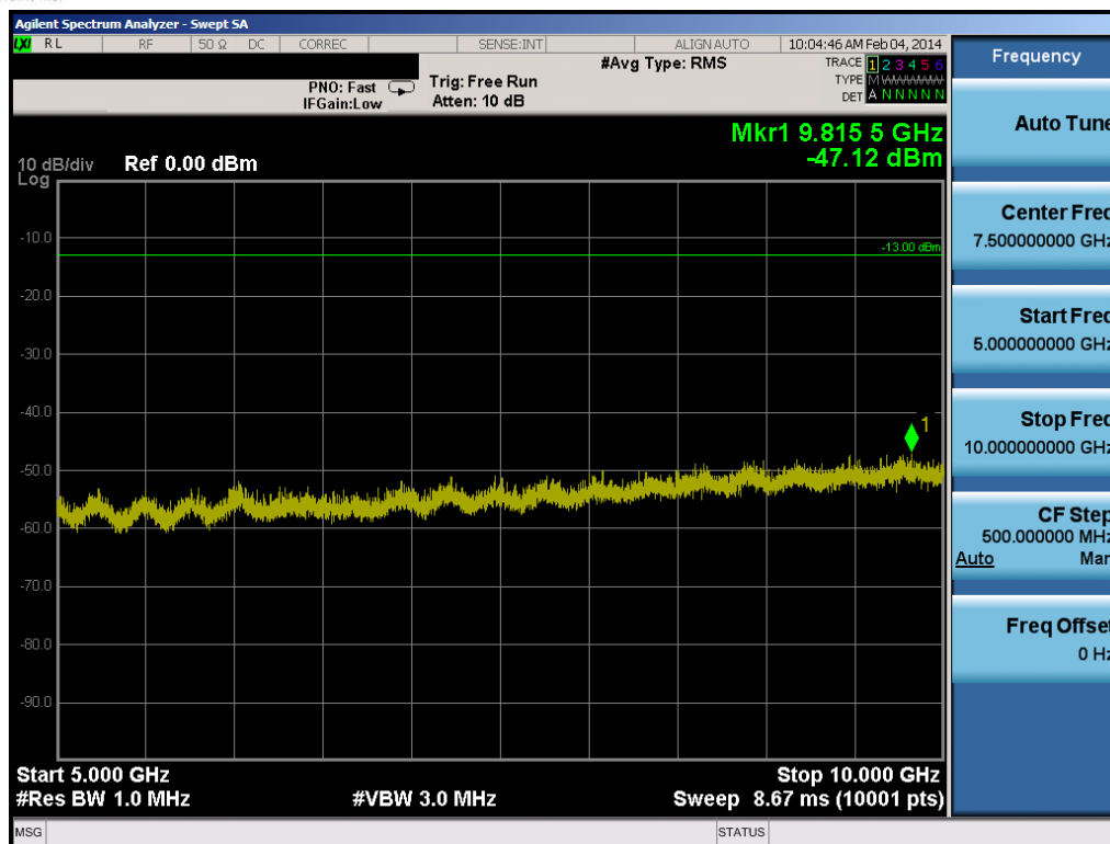
Plot 7-15. Conducted Spurious Plot (5.0MHz QPSK – RB Size 1, RB Offset 0 – Mid Channel)
