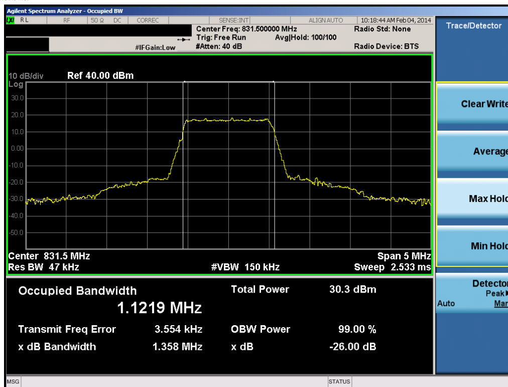
Plot 7-3. Occupied Bandwidth Plot (1.4MHz 16-QAM – RB Size 6)
