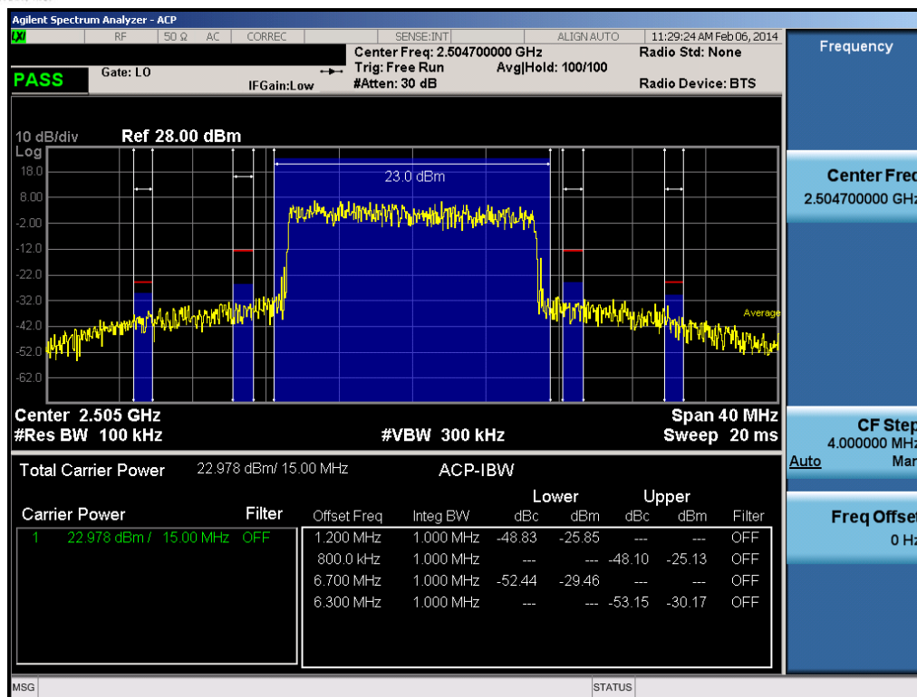
Plot 9-15. Low Adjacent Channel Band Edge Plot (15.0MHz QPSK – RB Size 75)
