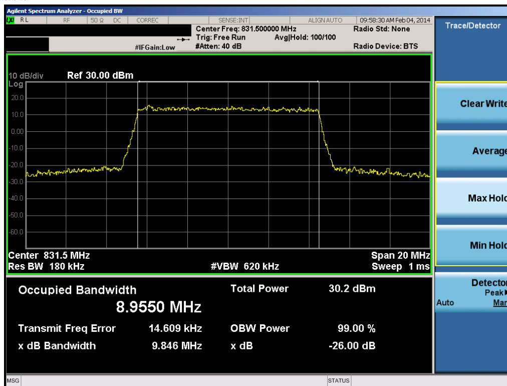
Plot 7-21. Occupied Bandwidth Plot (10.0MHz 16-QAM – RB Size 50)
