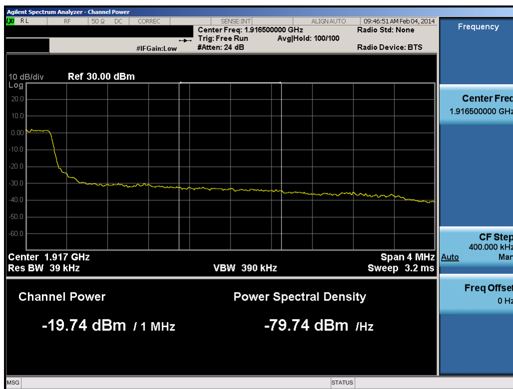
Plot 8-20. Upper Extended Band Edge Plot (5.0MHz QPSK – RB Size 25)
