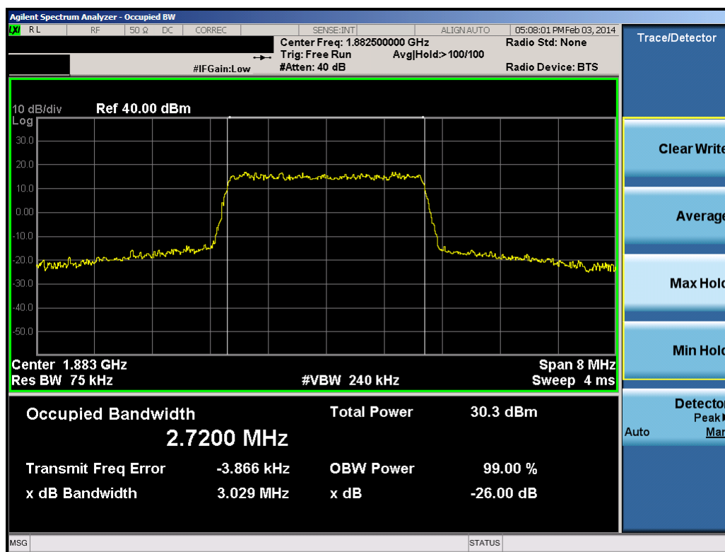
Plot 8-4. Occupied Bandwidth Plot (3.0MHz 16-QAM – RB Size 15)
