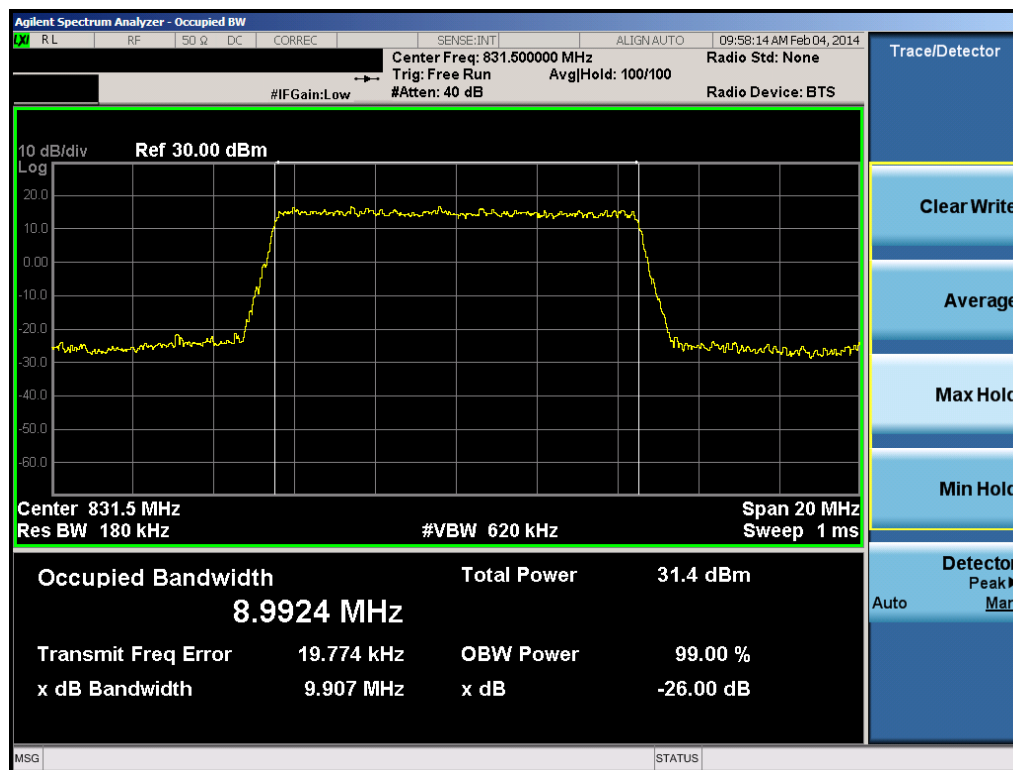
Plot 7-20. Occupied Bandwidth Plot (10.0MHz QPSK – RB Size 50)
