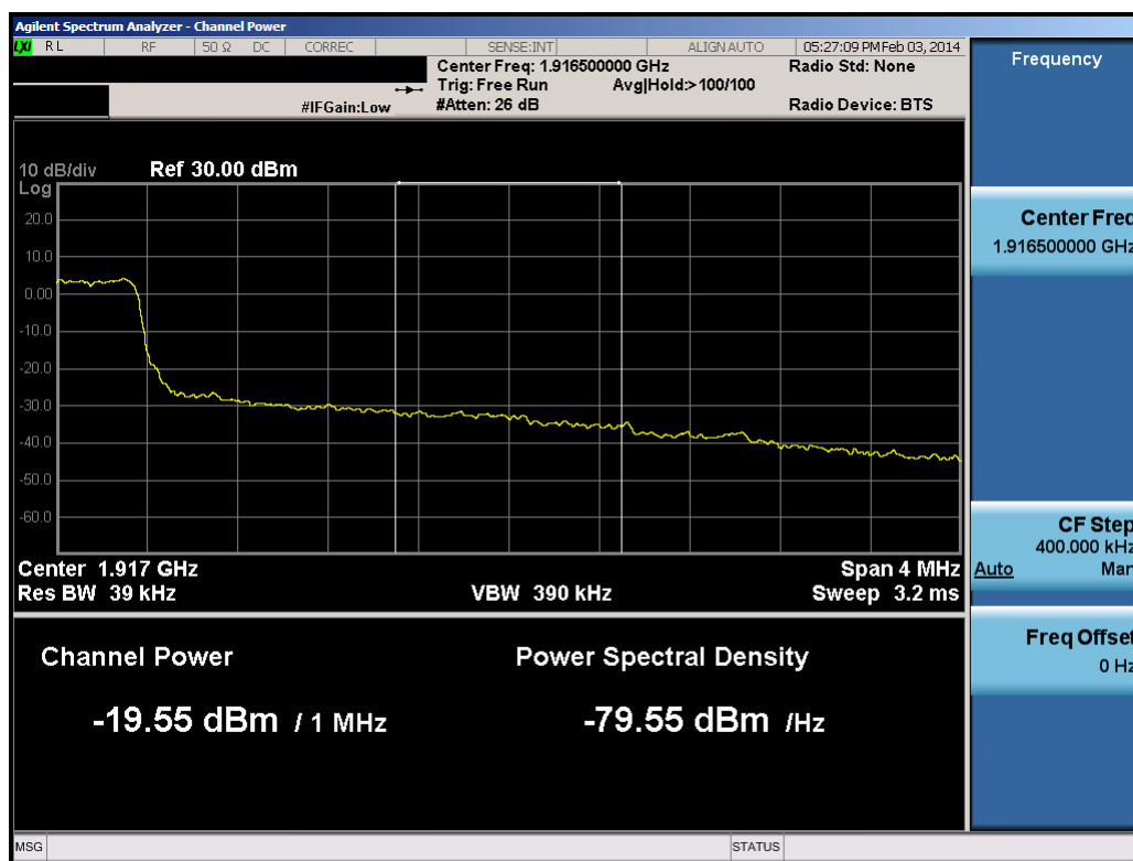
Plot 8-12. Upper Extended Band Edge Plot (3.0MHz QPSK – RB Size 15)
