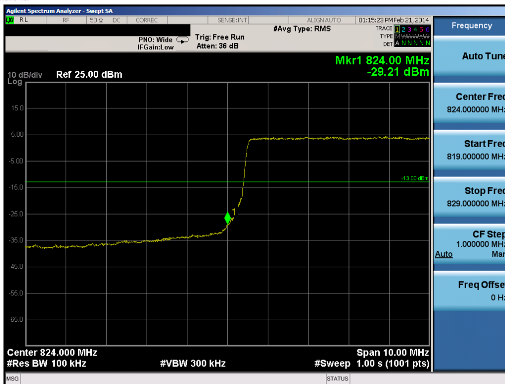
Plot 7-19. Lower Band Edge Plot (10.0MHz QPSK – RB Size 50)
