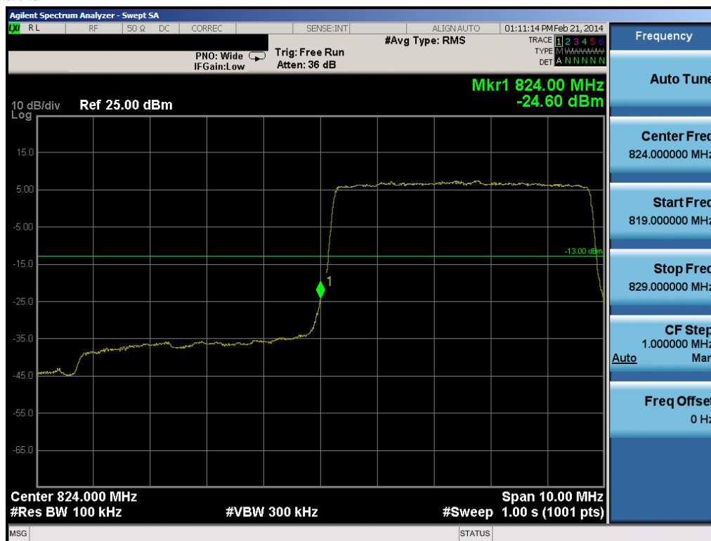
Plot 7-9. Lower Band Edge Plot (5.0MHz QPSK – RB Size 25)
