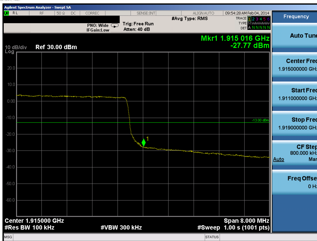
Plot 8-27. Upper Band Edge Plot (10.0MHz QPSK – RB Size 50)
