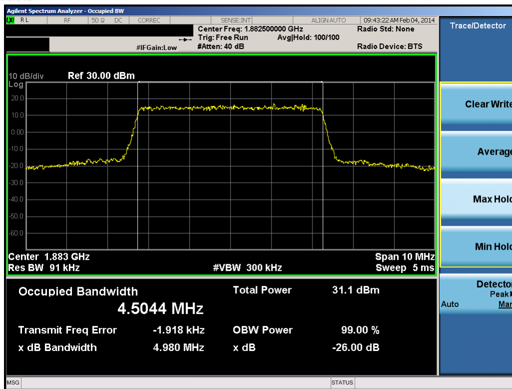
Plot 8-17. Occupied Bandwidth Plot (5.0MHz QPSK – RB Size 25)
