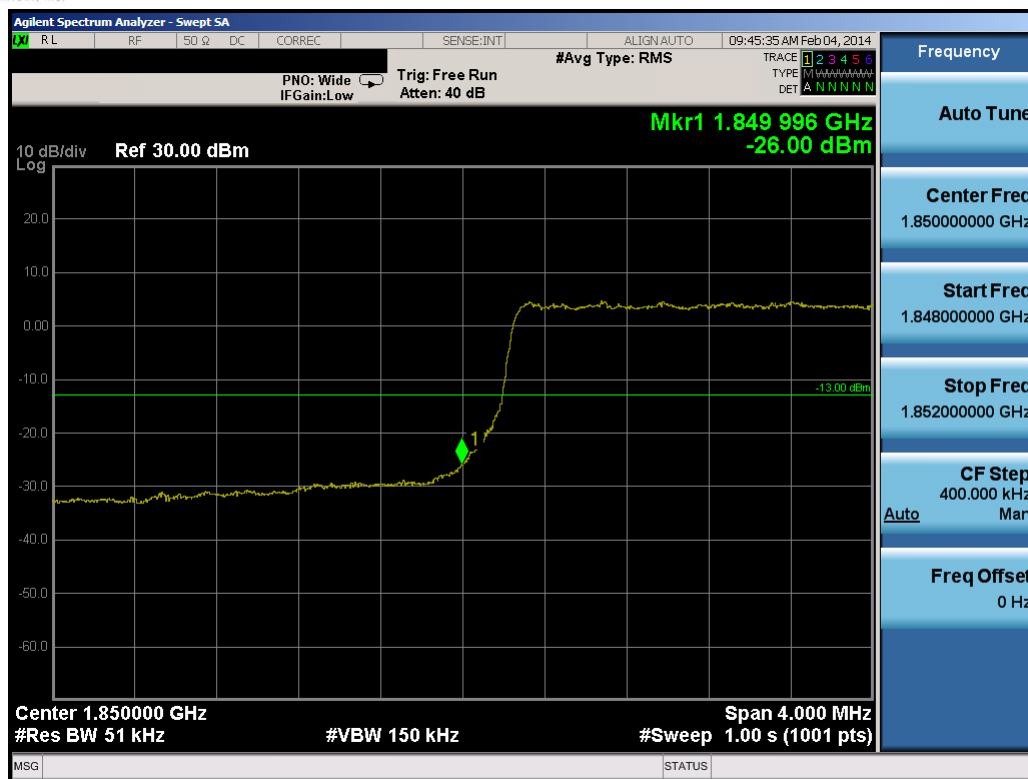
Plot 8-15. Lower Band Edge Plot (5.0MHz QPSK – RB Size 25)
