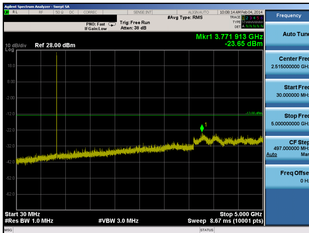
Plot 7-16. Conducted Spurious Plot (5.0MHz QPSK – RB Size 1, RB Offset 0 – High Channel)
