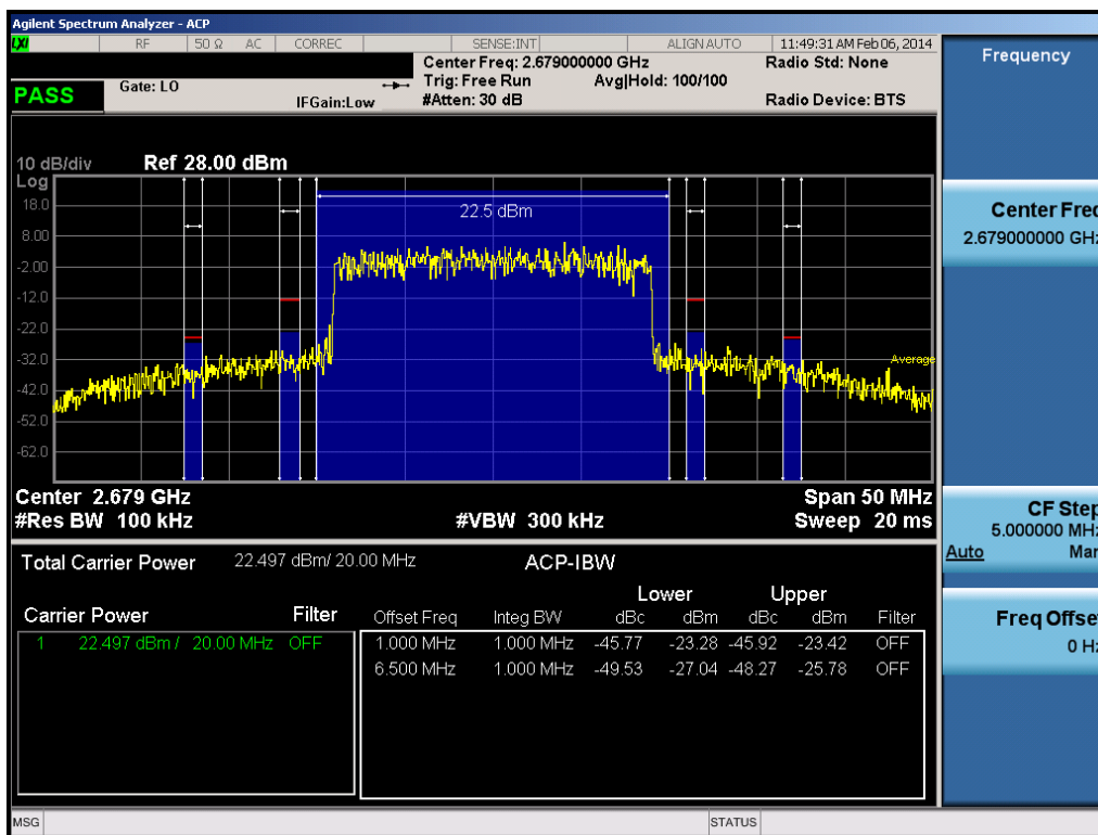
Plot 9-22. High Adjacent Channel Band Edge Plot (20.0MHz QPSK – RB Size 100)
