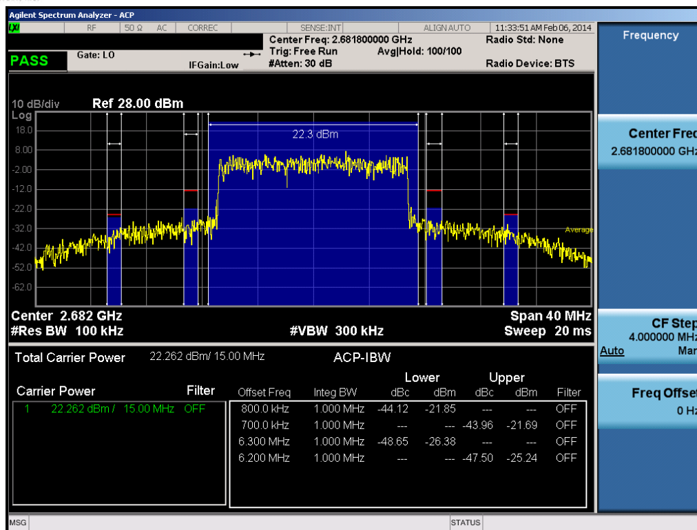
Plot 9-17. High Adjacent Channel Band Edge Plot (15.0MHz QPSK – RB Size 75)
