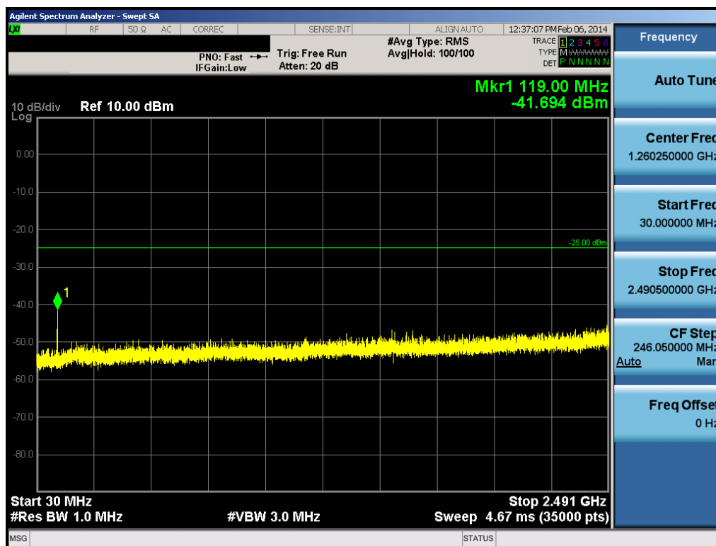
Plot 9-12. Conducted Spurious Plot (10.0MHz QPSK – RB Size 1, RB Offset 0 – High Channel)
