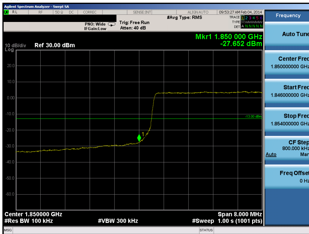
Plot 8-23. Lower Band Edge Plot (10.0MHz QPSK – RB Size 50)
