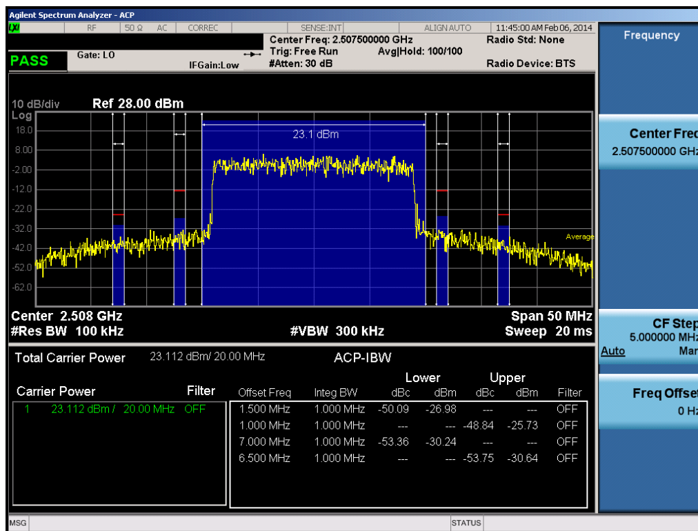
Plot 9-20. Low Adjacent Channel Band Edge Plot (20.0MHz QPSK – RB Size 100)
