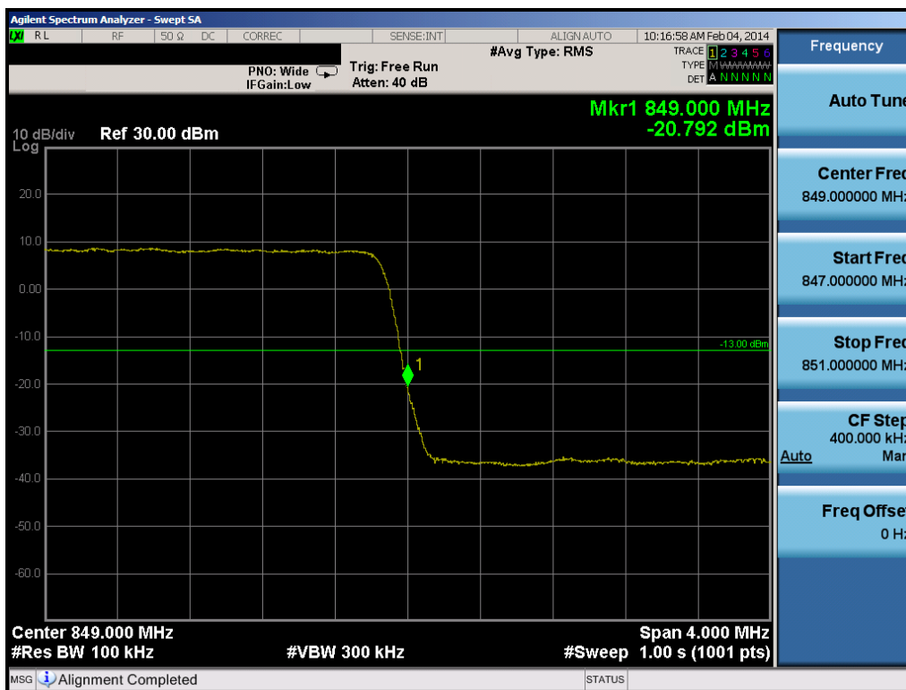
Plot 7-8. Upper Band Edge Plot (3.0MHz QPSK – RB Size 15)
