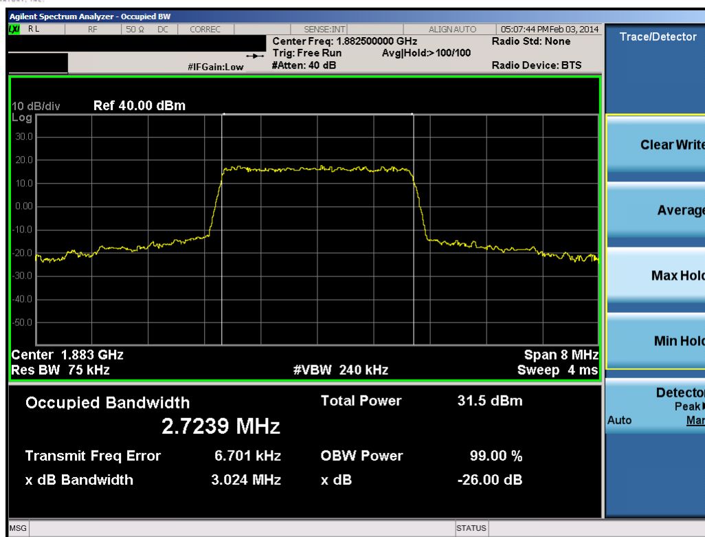
Plot 8-3. Occupied Bandwidth Plot (3.0MHz QPSK – RB Size 15)
