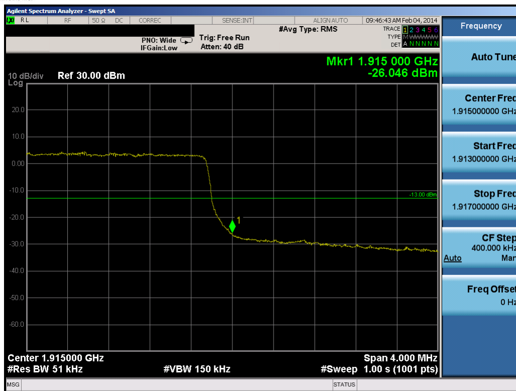
Plot 8-19. Upper Band Edge Plot (5.0MHz QPSK – RB Size 25)
