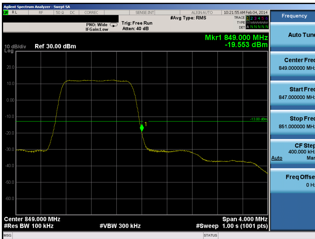
Plot 7-4. Upper Band Edge Plot (1.4MHz QPSK – RB Size 6)
