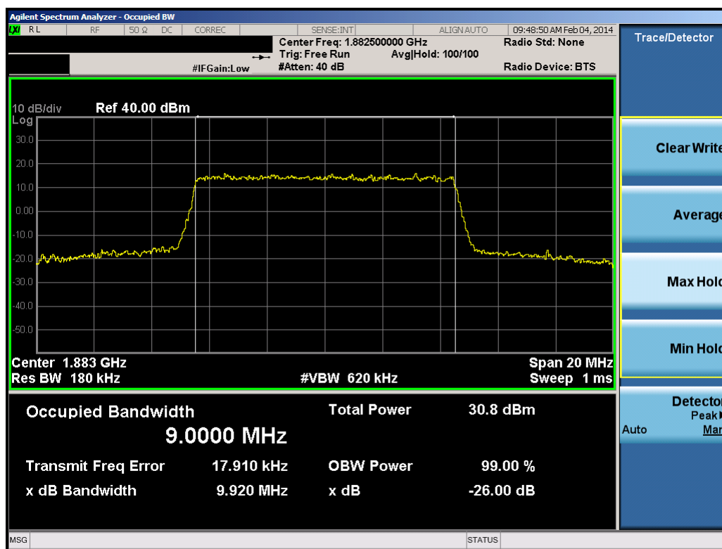
Plot 8-26. Occupied Bandwidth Plot (10.0MHz 16-QAM – RB Size 50)
