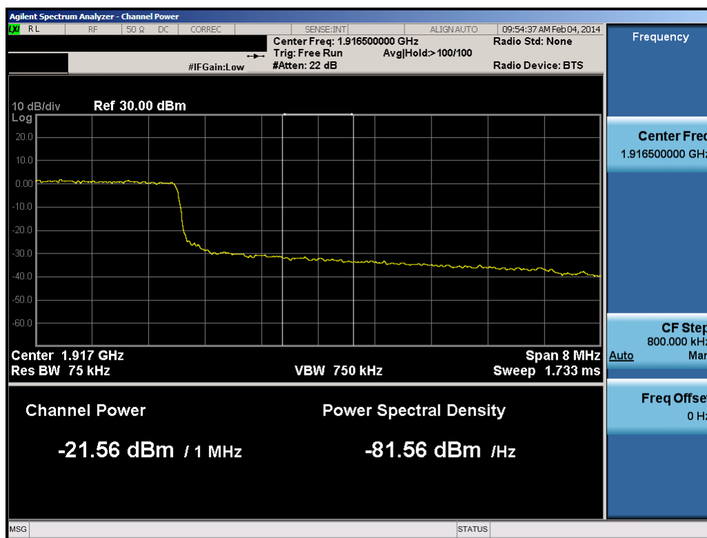
Plot 8-28. Upper Extended Band Edge Plot (10.0MHz QPSK – RB Size 50)
