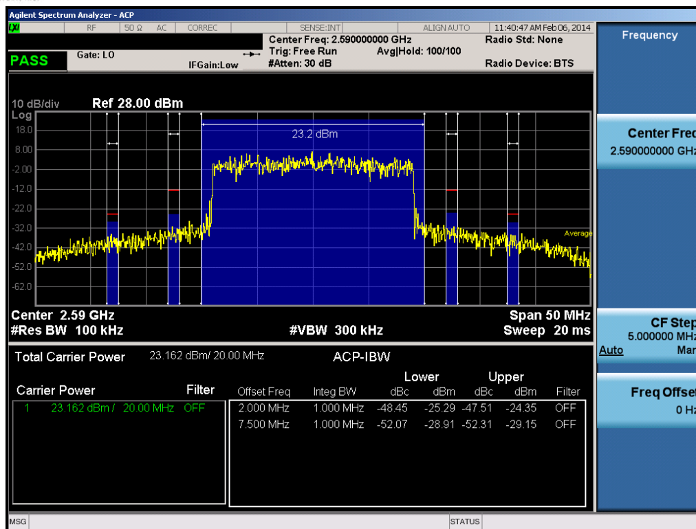
Plot 9-21. Mid Adjacent Channel Band Edge Plot (20.0MHz QPSK – RB Size 100)
