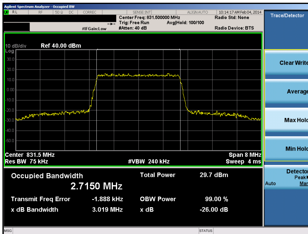
Plot 7-7. Occupied Bandwidth Plot (3.0MHz 16-QAM – RB Size 15)
