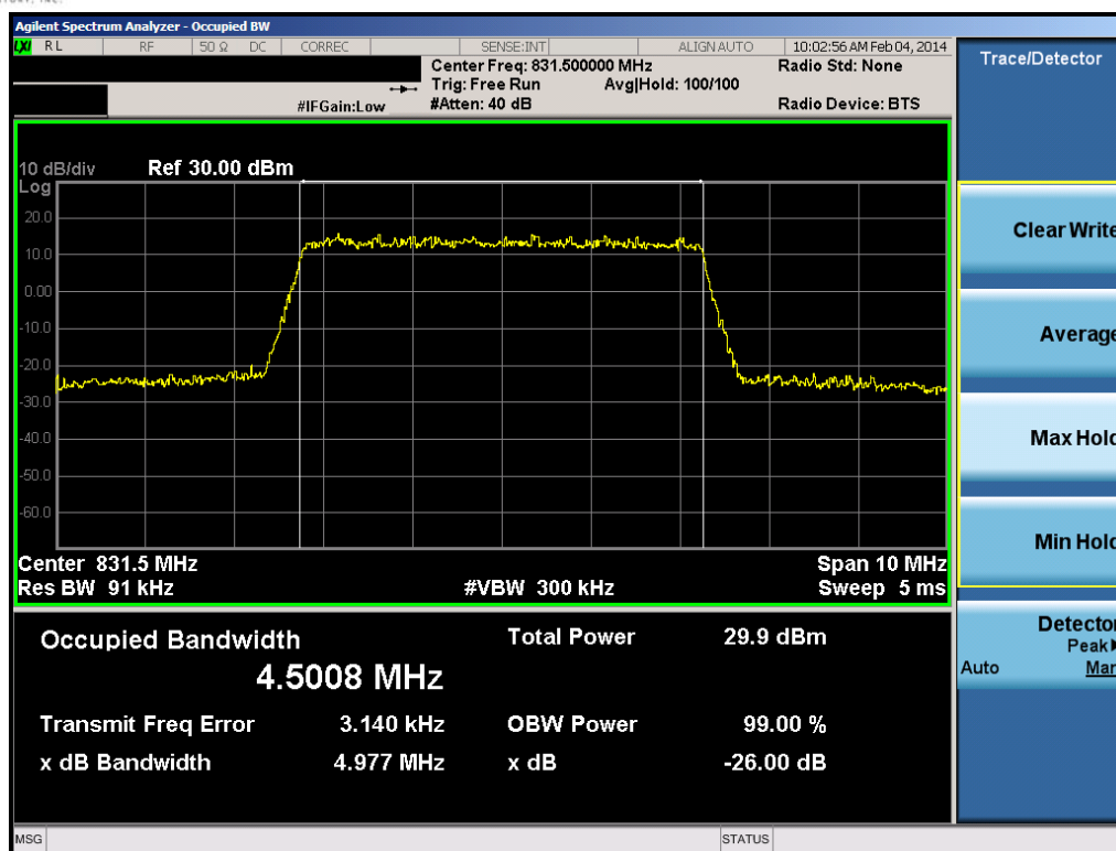
Plot 7-11. Occupied Bandwidth Plot (5.0MHz 16-QAM – RB Size 25)
