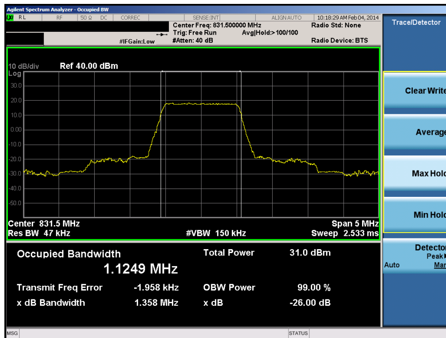
Plot 7-2. Occupied Bandwidth Plot (1.4MHz QPSK – RB Size 6)
