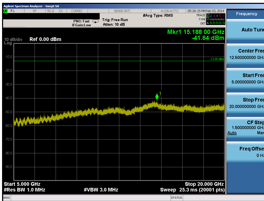
Plot 8-10. Conducted Spurious Plot (3.0MHz QPSK – RB Size 1, RB Offset 0 – High Channel)
