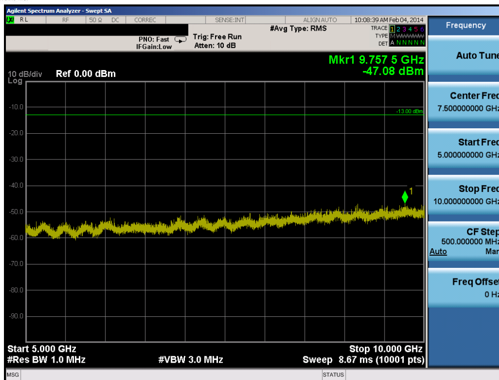
Plot 7-17. Conducted Spurious Plot (5.0MHz QPSK – RB Size 1, RB Offset 0 – High Channel)
