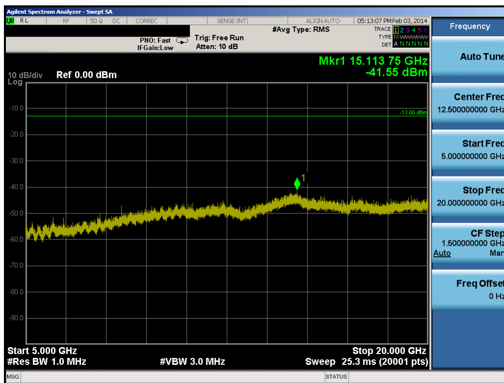
Plot 8-8. Conducted Spurious Plot (3.0MHz QPSK – RB Size 1, RB Offset 0 – Mid Channel)
