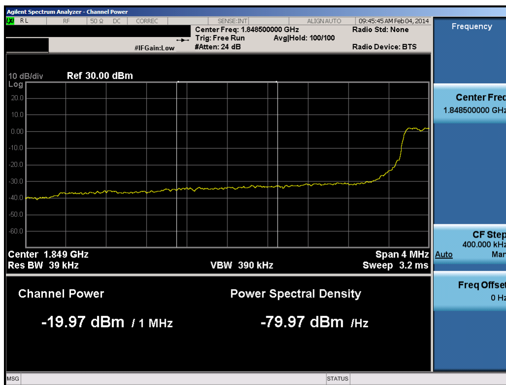
Plot 8-16. Lower Extended Band Edge Plot (5.0MHz QPSK – RB Size 25)
