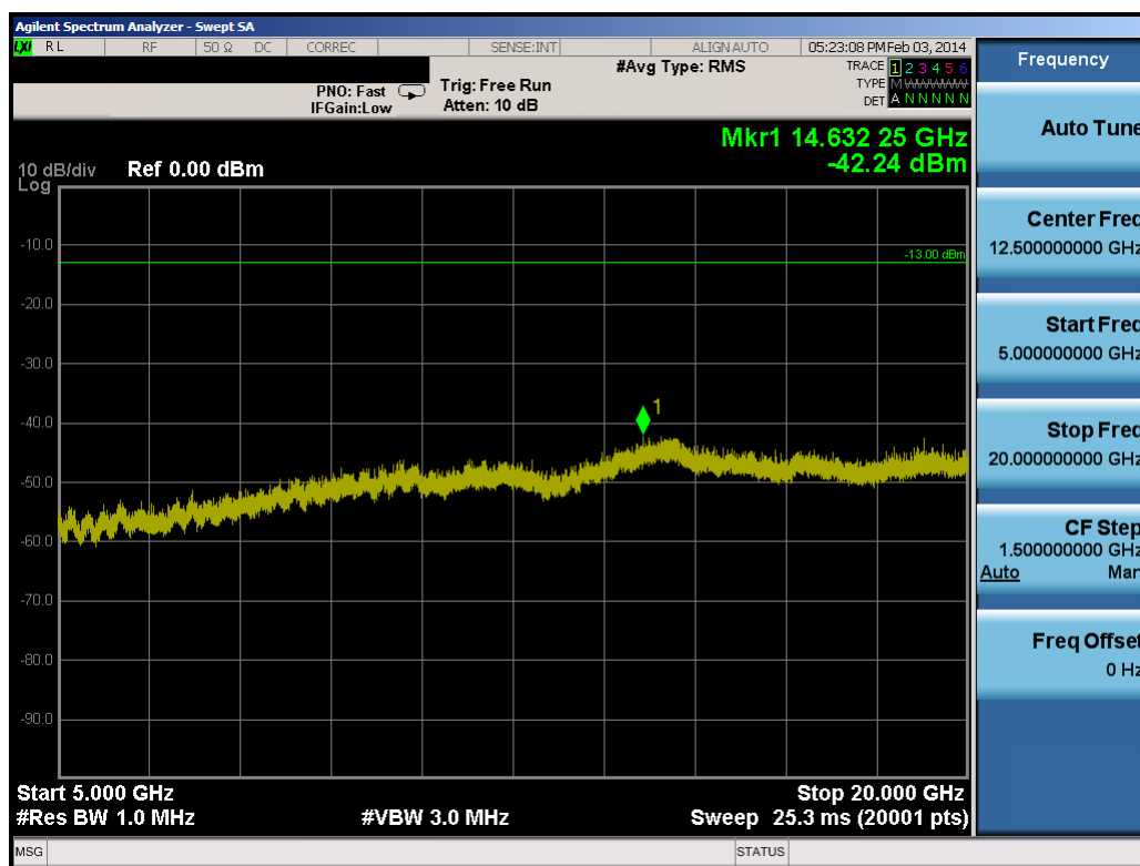
Plot 8-6. Conducted Spurious Plot (3.0MHz QPSK – RB Size 1, RB Offset 0 – Low Channel)
