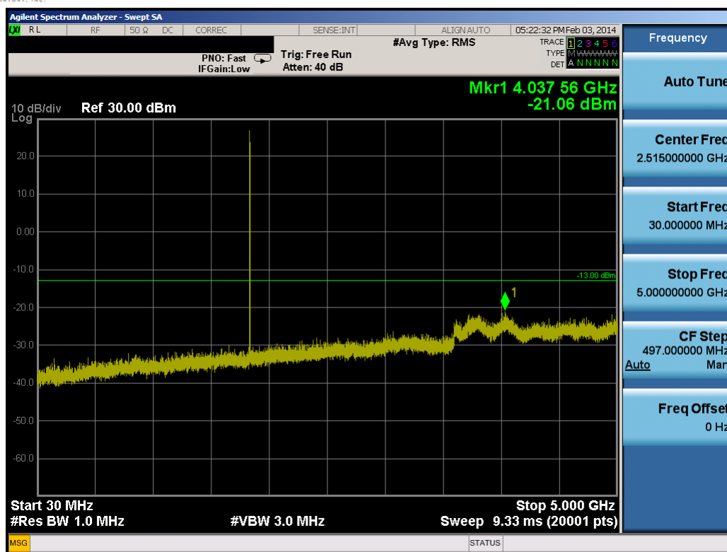
Plot 8-5. Conducted Spurious Plot (3.0MHz QPSK – RB Size 1, RB Offset 0 – Low Channel)
