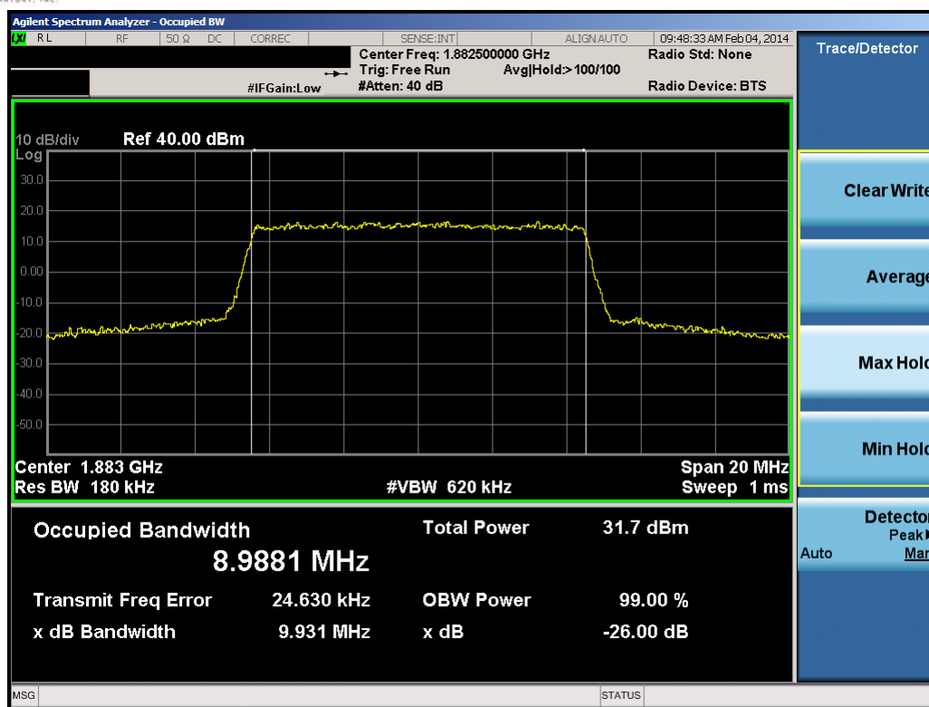
Plot 8-25. Occupied Bandwidth Plot (10.0MHz QPSK – RB Size 50)
