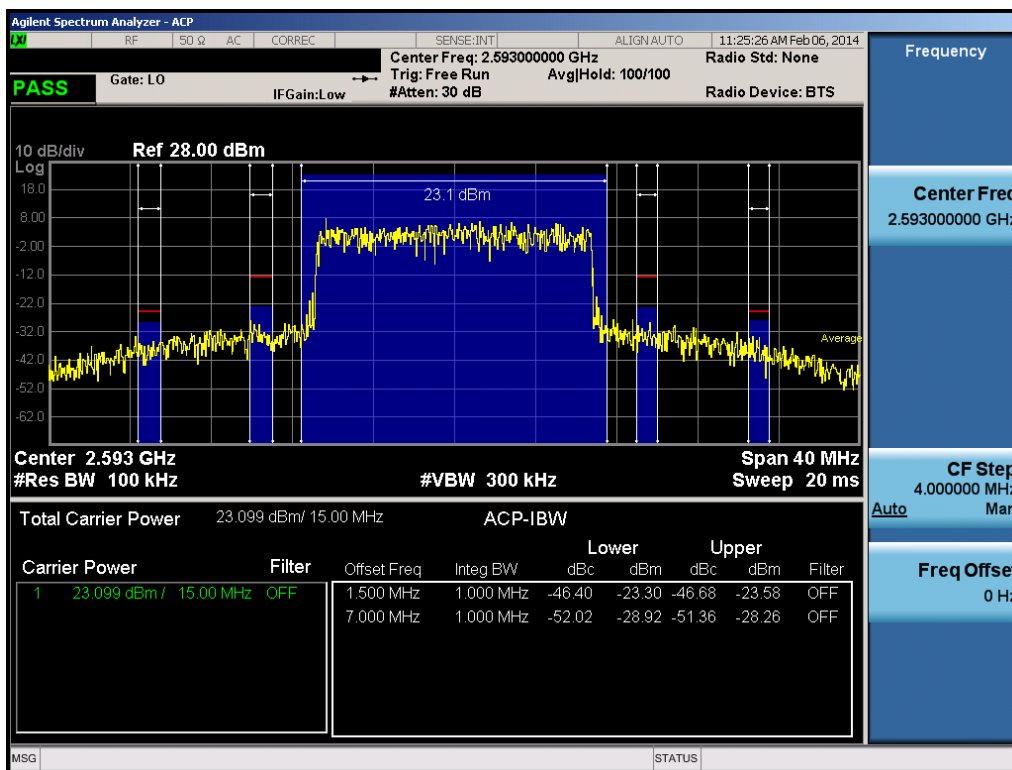
Plot 9-16. Mid Adjacent Channel Band Edge Plot (15.0MHz QPSK – RB Size 75)
