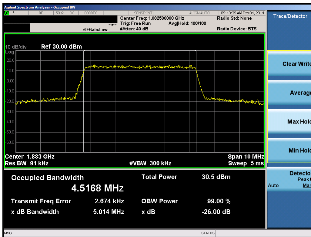
Plot 8-18. Occupied Bandwidth Plot (5.0MHz 16-QAM – RB Size 25)
