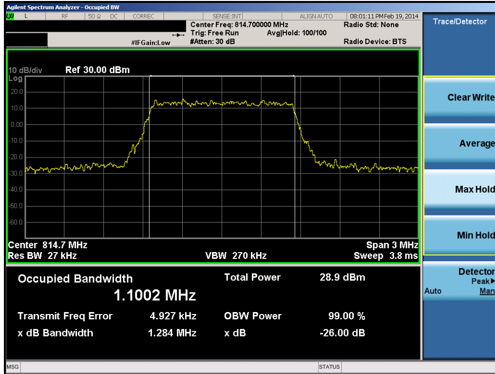
Plot 8-5. Occupied Bandwidth Plot (1.4MHz QPSK – RB Size 6 – Low Channel)
