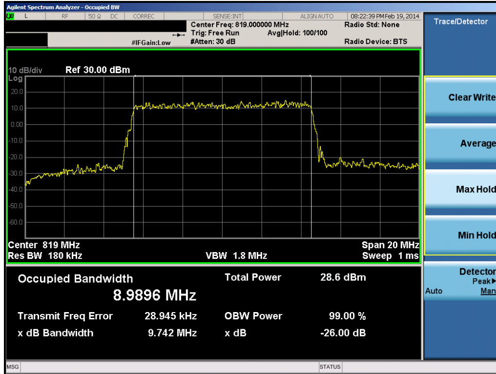
Plot 8-19. Occupied Bandwidth Plot (10MHz QPSK – RB Size 50)
