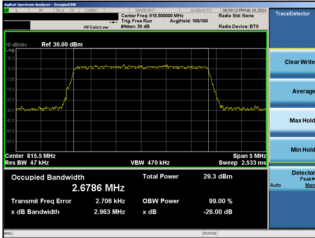
Plot 8-11. Occupied Bandwidth Plot (3MHz QPSK – RB Size 15 – Low Channel)
