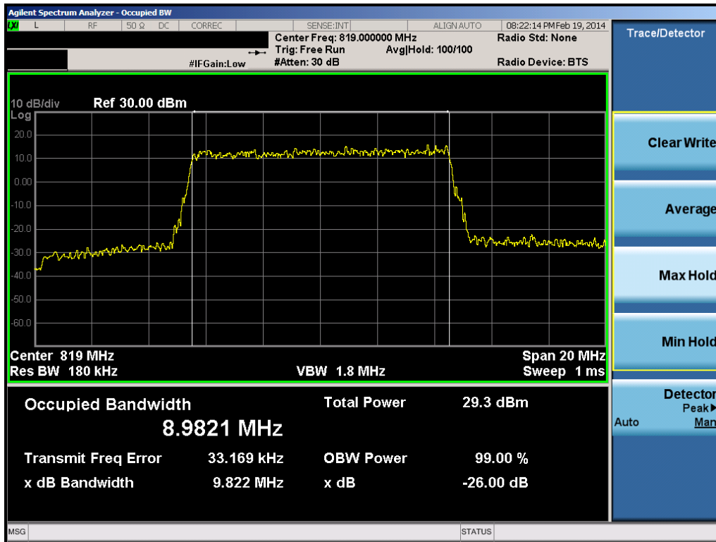
Plot 8-18. Occupied Bandwidth Plot (10MHz QPSK – RB Size 50)
