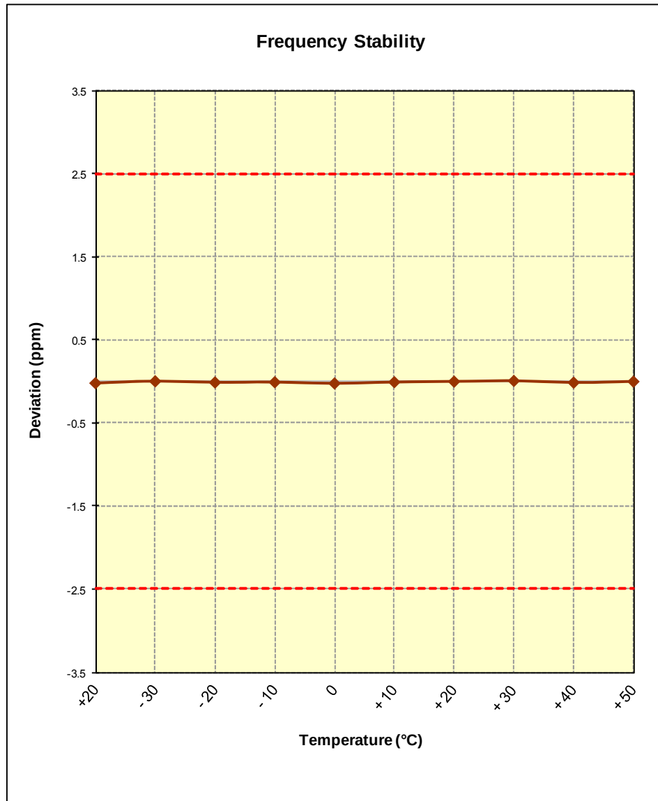
Figure 6-1. Frequency Stability Graph (Ch. 684)
