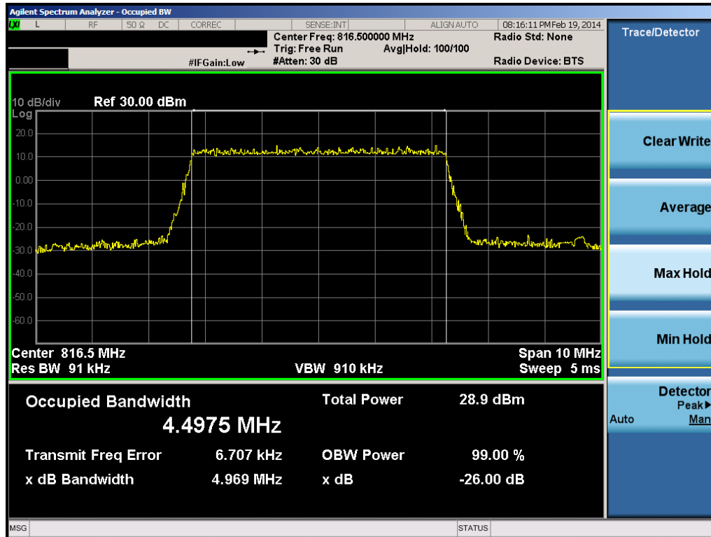
Plot 8-15. Occupied Bandwidth Plot (5MHz QPSK – RB Size 25 – Low Channel)
