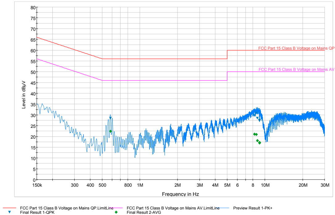
Plot 6-47. Line-Conducted Test Plot (N)
