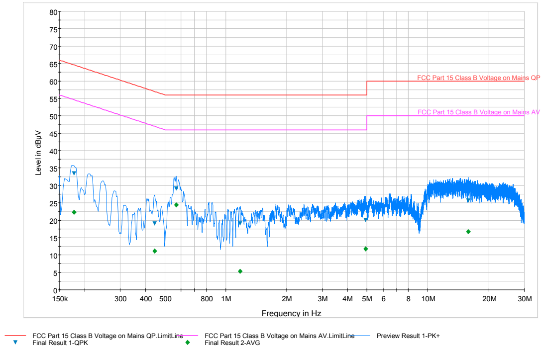
Plot 6-46. Line-Conducted Test Plot (L1)
