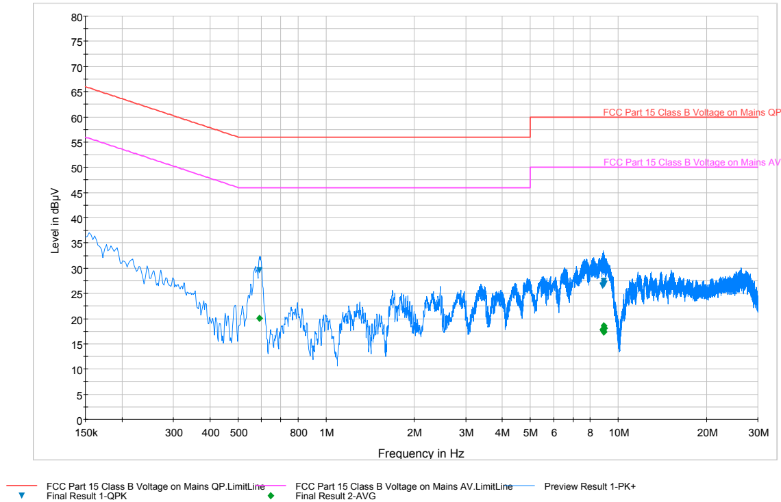
Plot 6-9. Line-Conducted Test Plot (N)
