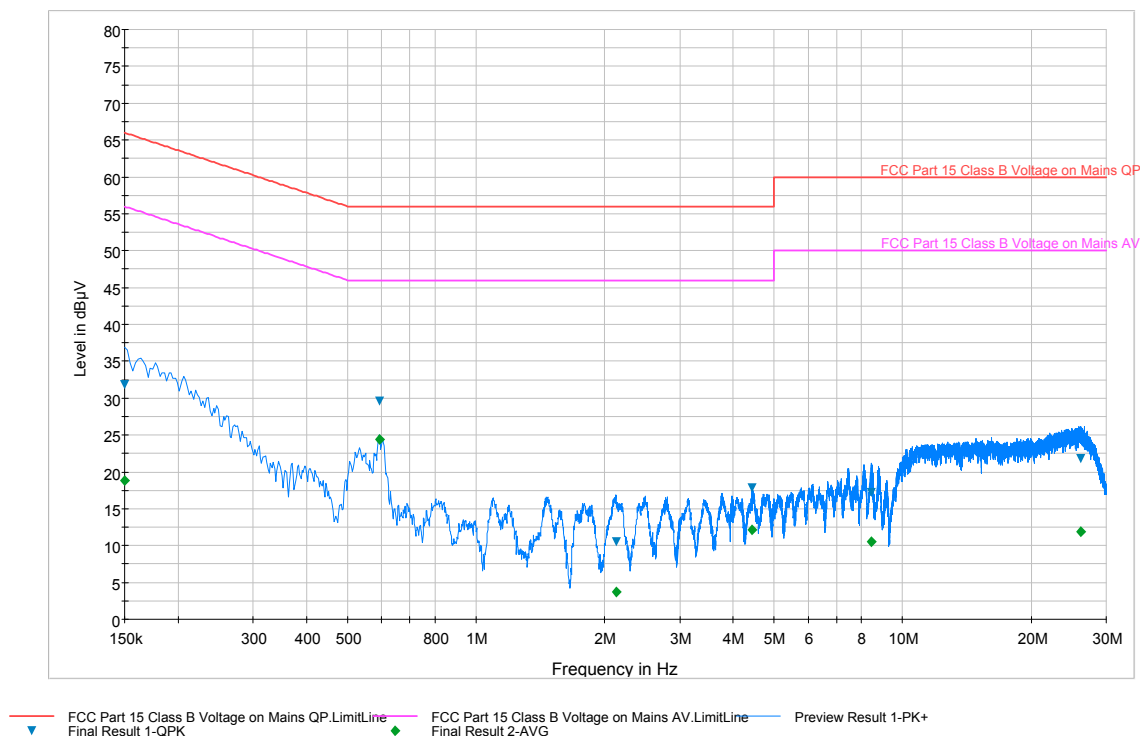
Plot 6-8. Line-Conducted Test Plot (L1)
