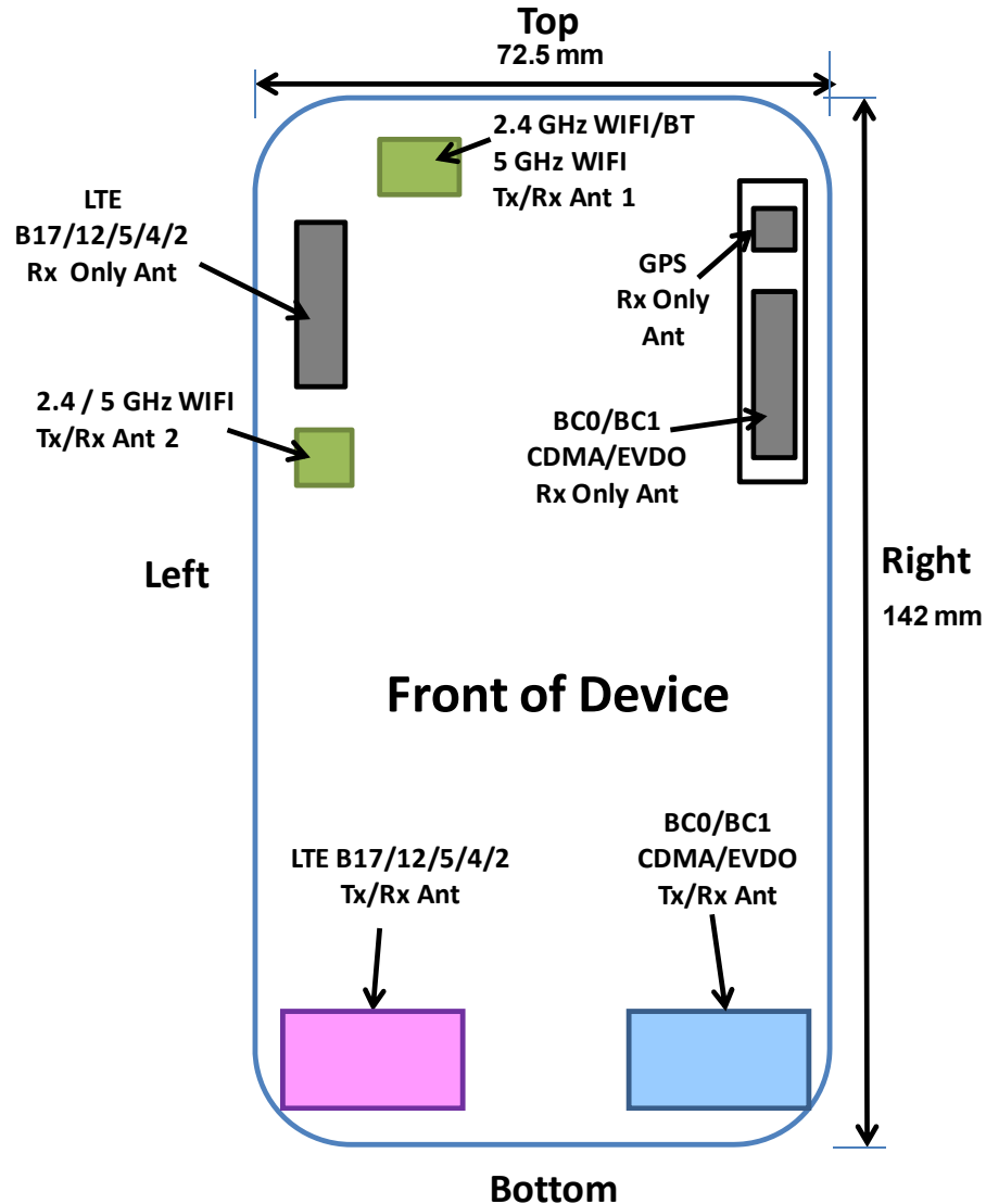
Figure 1-1 DUT Antenna Locations
