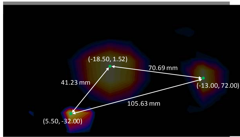
Figure 12-1 Peak SAR Locations of Cell. CDMA, LTE Band 2, and 5 GHz WLAN Antenna 1
