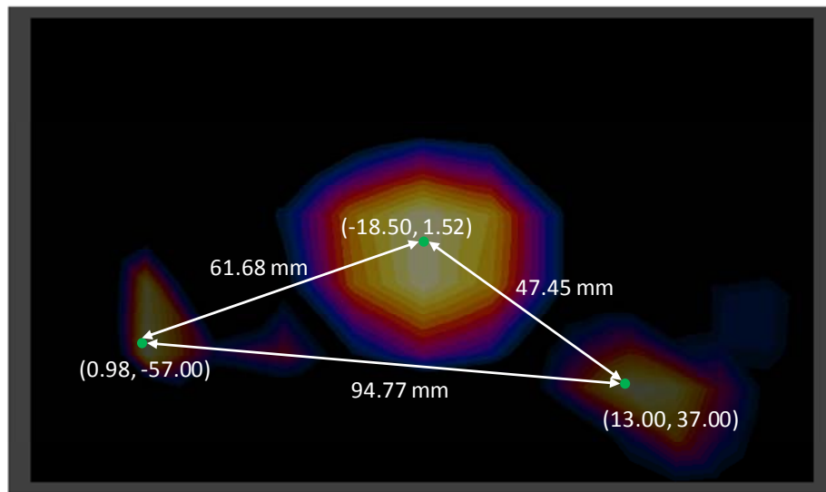
Figure 12-4 Peak SAR Locations of Cell. CDMA, LTE Band 4, and 5 GHz WLAN Antenna 2
