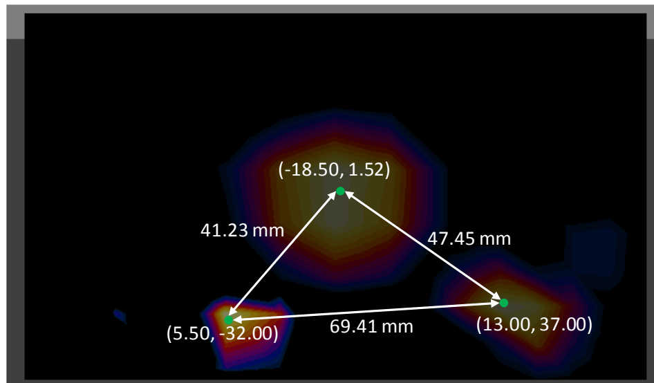
Figure 12-3 Peak SAR Locations of Cell. CDMA, LTE Band 2, and 5 GHz WLAN Antenna 2
