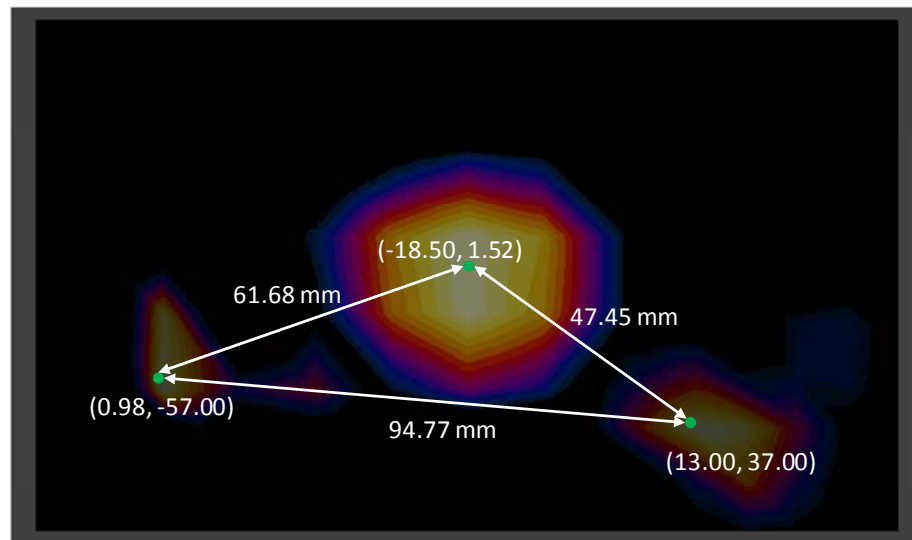
Figure 12-2 Peak SAR Locations of Cell. CDMA, LTE Band 4, and 5 GHz WLAN Antenna 2
