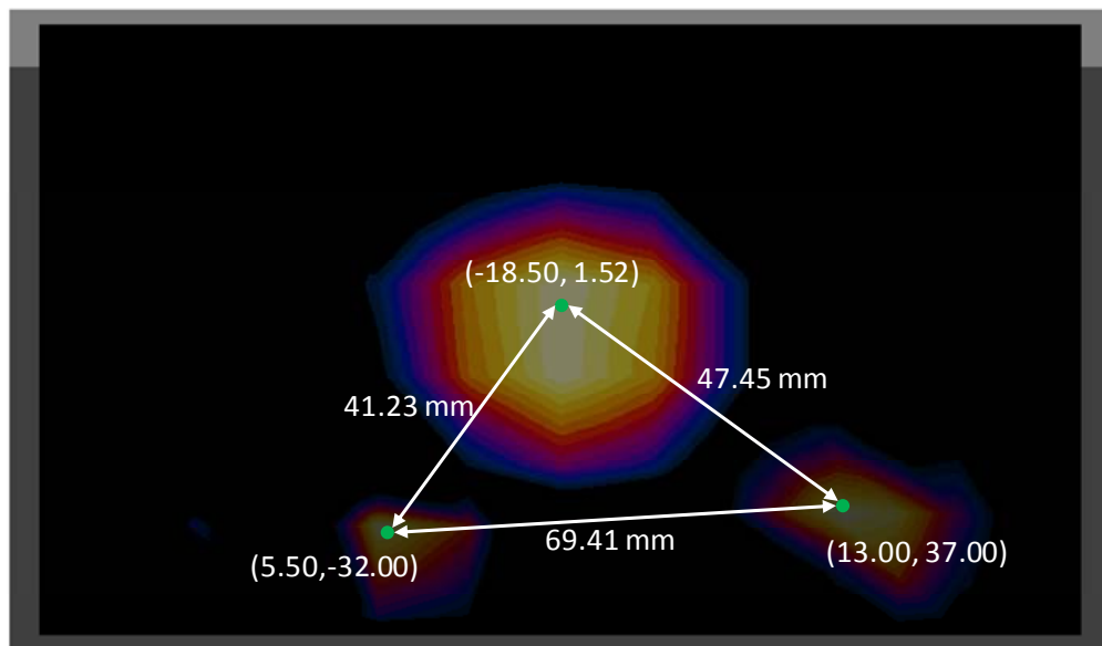
Figure 12-5 Peak SAR Locations of Cell. CDMA, LTE Band 2, and 5 GHz WLAN Antenna 2
