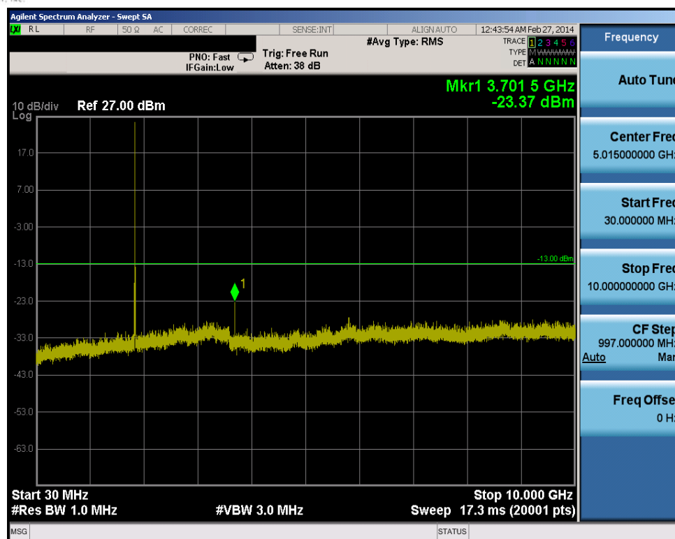
Plot 10-13. Conducted Spurious Plot (10.0MHz QPSK – RB Size 1, RB Offset 0– Low Channel)
