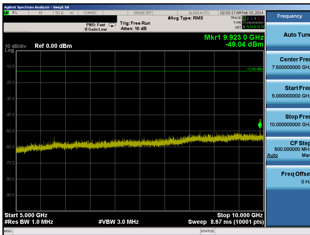
Plot 8-23. Conducted Spurious Plot (10.0MHz QPSK – RB Size 1, RB Offset 0 – Low Channel)
