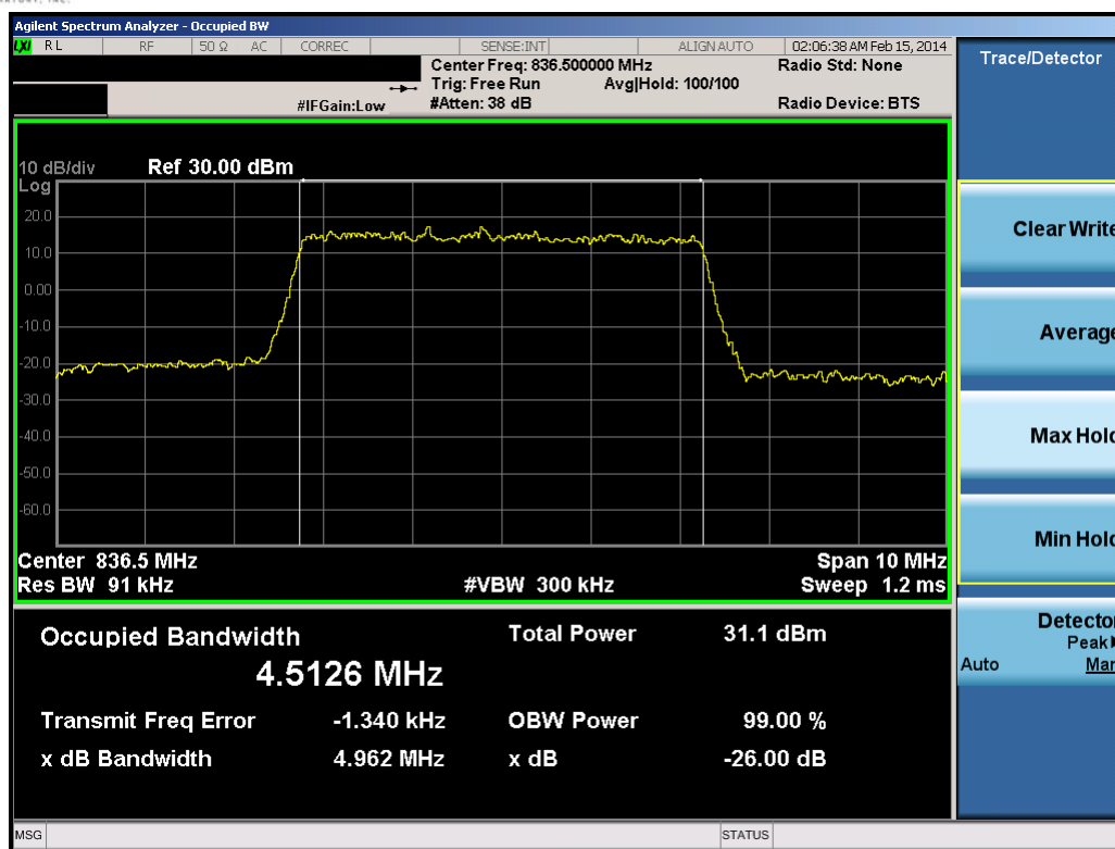
Plot 8-10. Occupied Bandwidth Plot (5.0MHz QPSK – RB Size 25)
