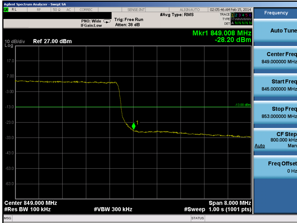
Plot 8-28. Upper Band Edge Plot (10.0MHz QPSK – RB Size 50)
