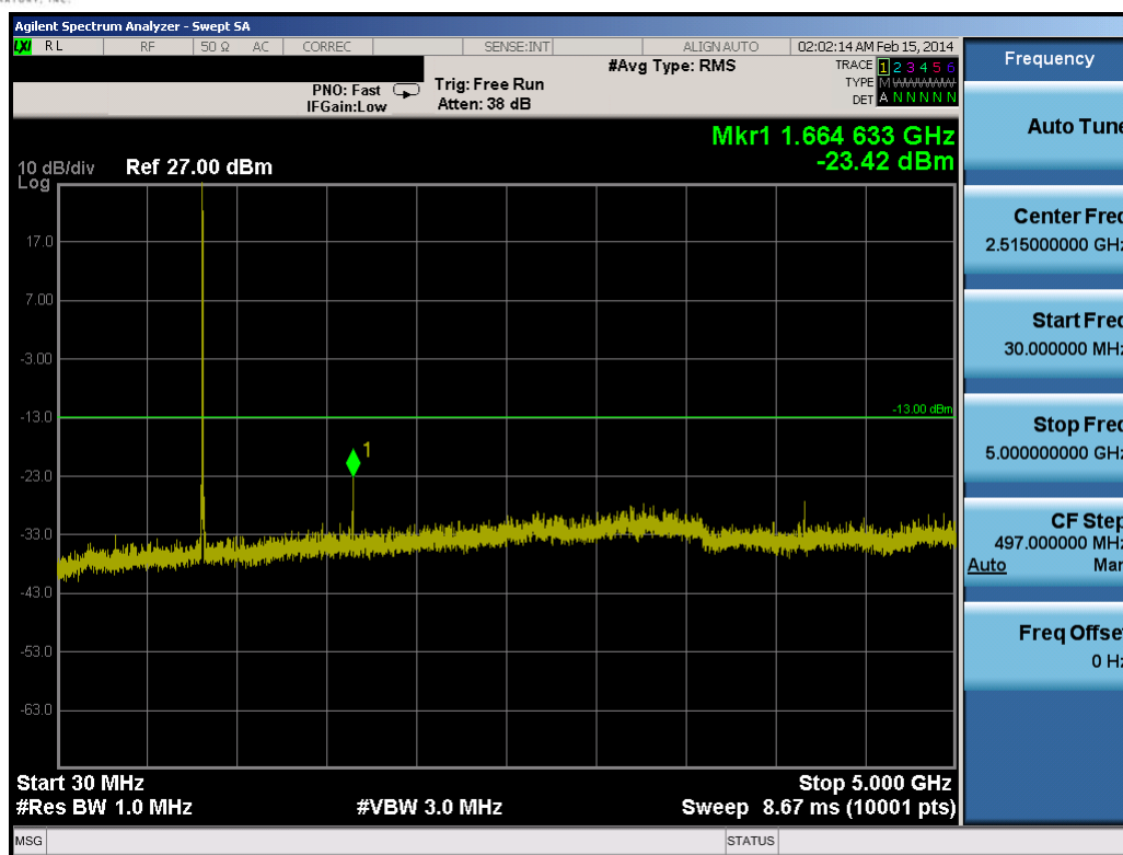
Plot 8-24. Conducted Spurious Plot (10.0MHz QPSK – RB Size 1, RB Offset 0 – Mid Channel)
