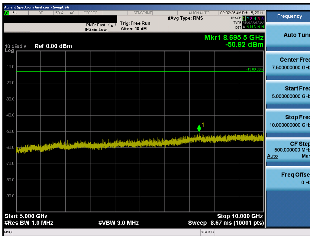
Plot 8-25. Conducted Spurious Plot (10.0MHz QPSK – RB Size 1, RB Offset 0 – Mid Channel)
