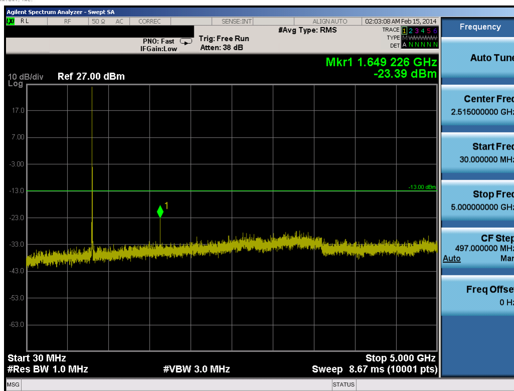
Plot 8-22. Conducted Spurious Plot (10.0MHz QPSK – RB Size 1, RB Offset 0– Low Channel)
