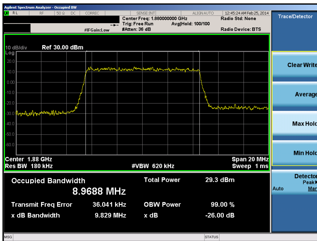
Plot 10-12. Occupied Bandwidth Plot (10.0MHz 16-QAM – RB Size 50)
