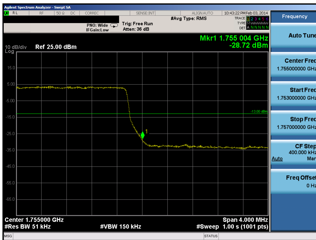
Plot 9-5. Upper Band Edge Plot (5.0MHz QPSK – RB Size 25)
