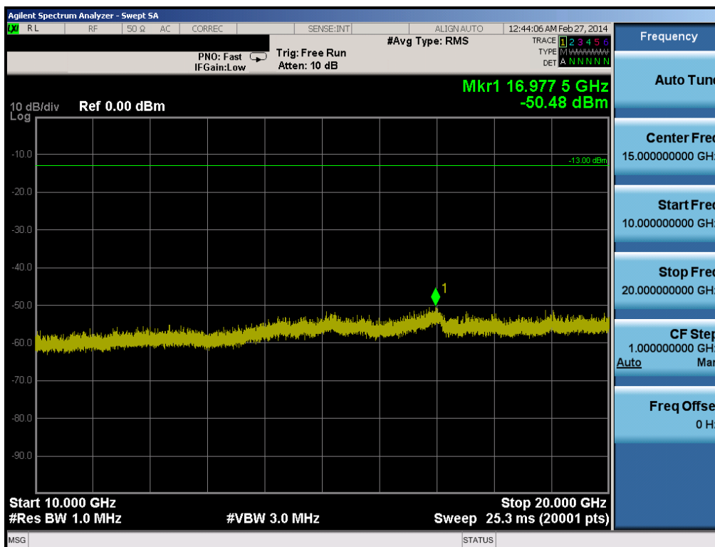
Plot 10-14. Conducted Spurious Plot (10.0MHz QPSK – RB Size 1, RB Offset 0 – Low Channel)
