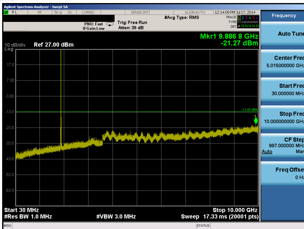
Plot 6-25. Conducted Spurious Plot (Band 2 – 15.0MHz QPSK – RB Size 1, RB Offset 0 – High Channel)
