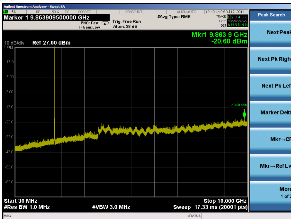
Plot 6-11. Conducted Spurious Plot (Band 4 – 15.0MHz QPSK – RB Size 1, RB Offset 0 – Mid Channel)
