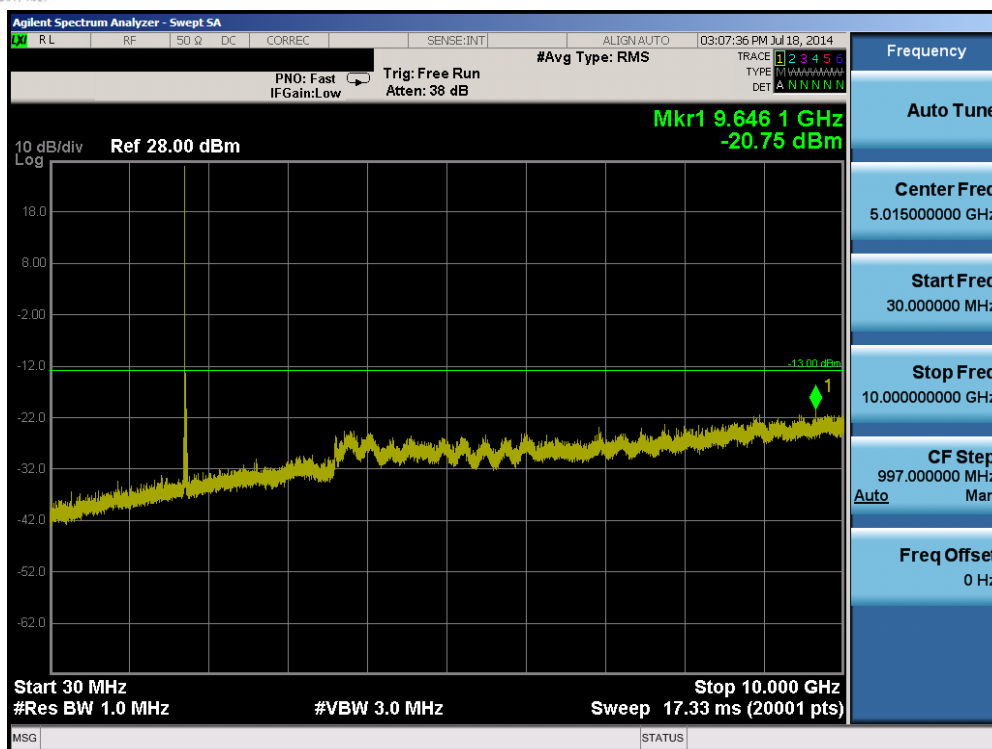
Plot 6-17. Conducted Spurious Plot (Band 4 – 20.0MHz QPSK – RB Size 1, RB Offset 0 – Mid Channel)
