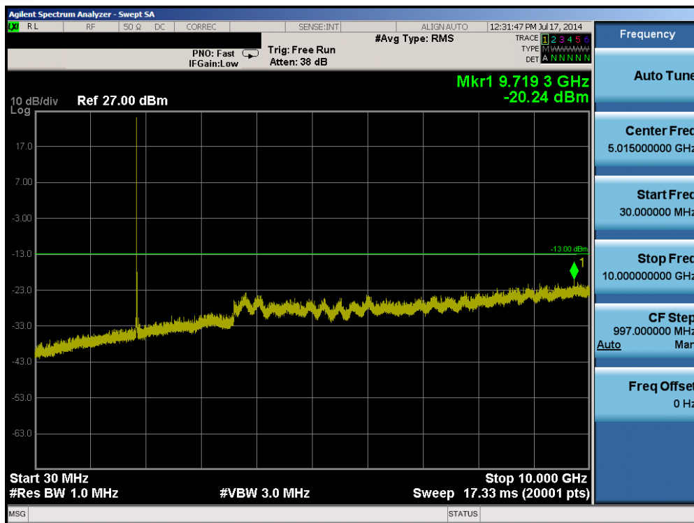
Plot 6-27. Conducted Spurious Plot (Band 2 – 20.0MHz QPSK – RB Size 1, RB Offset 0– Low Channel)
