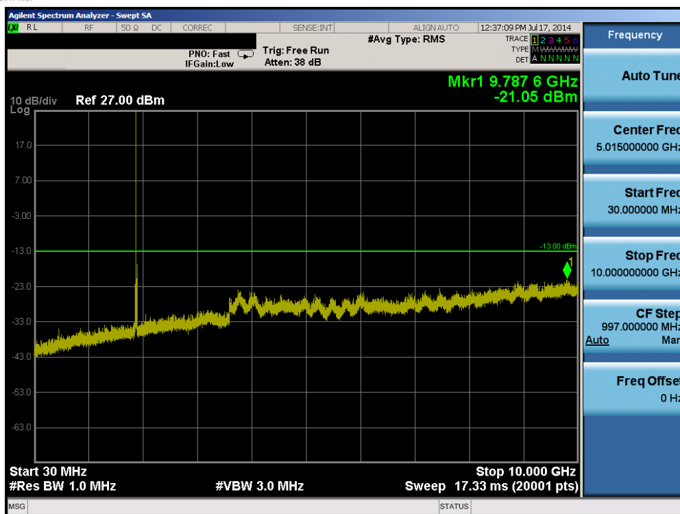
Plot 6-31. Conducted Spurious Plot (Band 2 – 20.0MHz QPSK – RB Size 1, RB Offset 0 – High Channel)
