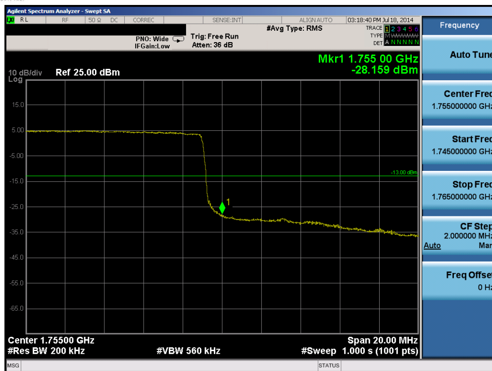
Plot 6-39. Upper Band Edge Plot (Band 4 – 20.0MHz QPSK – RB Size 100)
