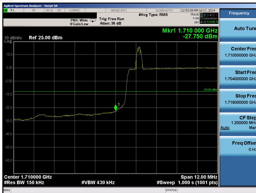
Plot 6-33. Lower Band Edge Plot (Band 4 – 15.0MHz QPSK – RB Size 75)
