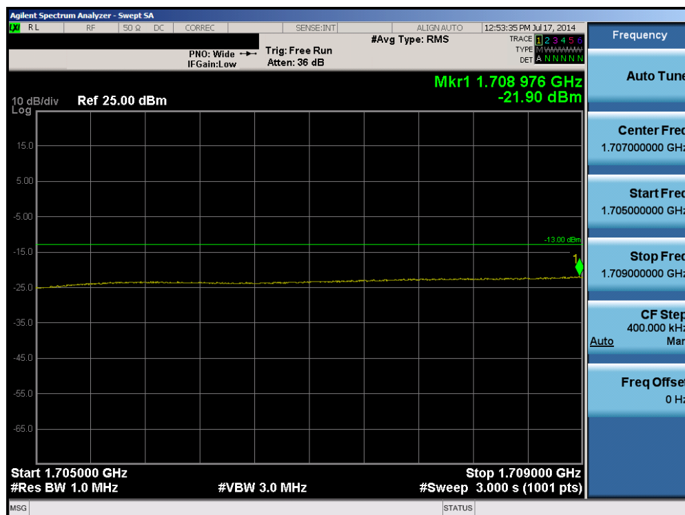
Plot 6-34. Lower Extended Band Edge Plot (Band 4 – 15.0MHz QPSK – RB Size 75)
