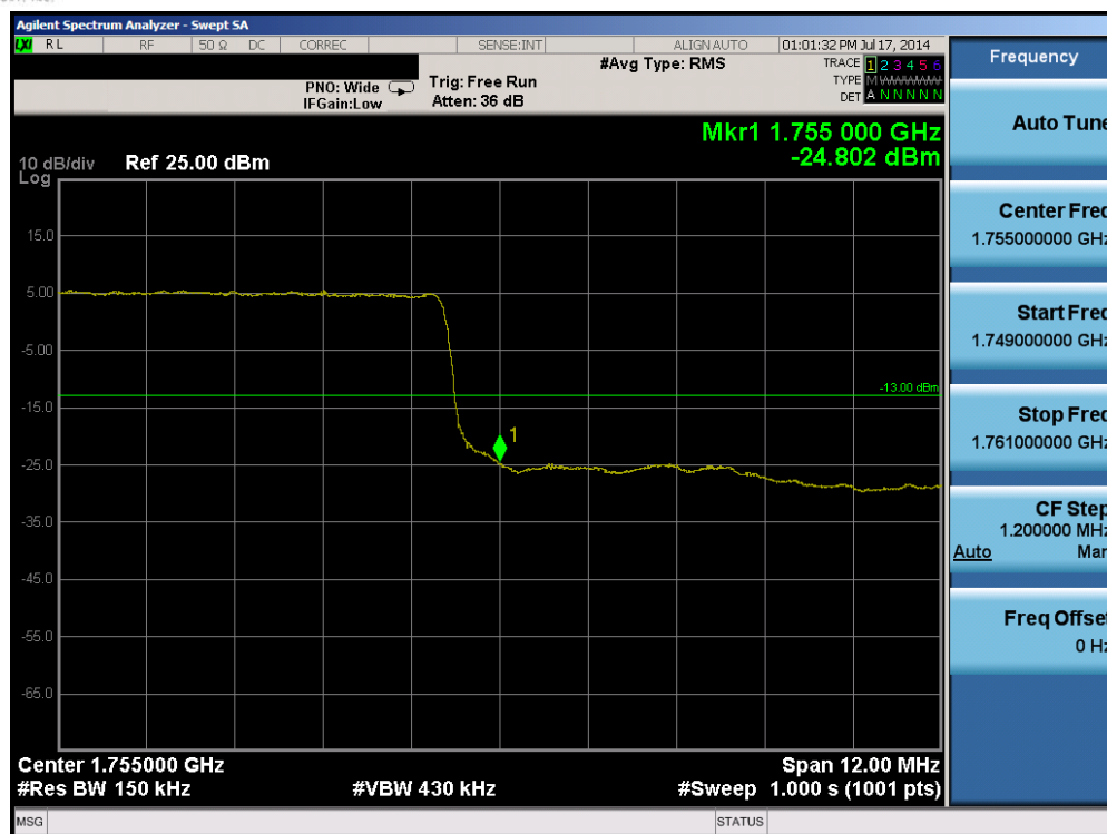
Plot 6-35. Upper Band Edge Plot (Band 4 – 15.0MHz QPSK – RB Size 75)
