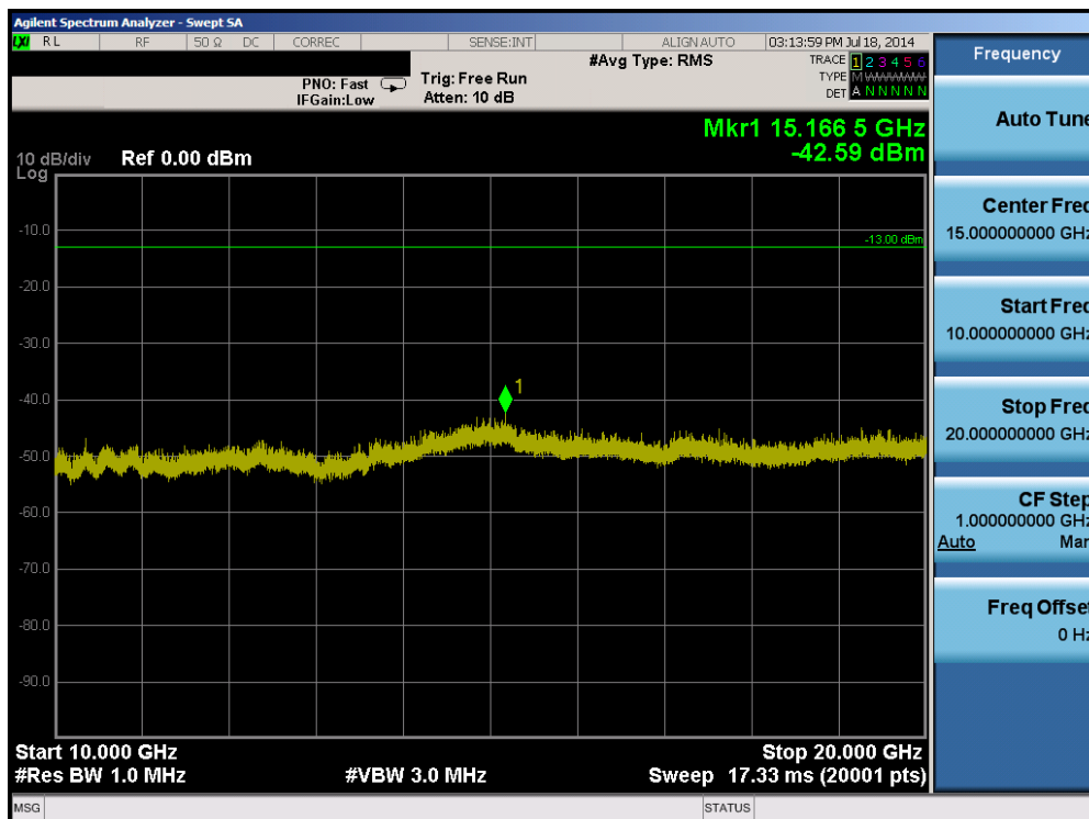
Plot 6-20. Conducted Spurious Plot (Band 4 – 20.0MHz QPSK – RB Size 1, RB Offset 0 – High Channel)
