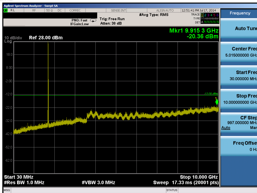
Plot 6-9. Conducted Spurious Plot (Band 4 – 15.0MHz QPSK – RB Size 1, RB Offset 0 – Low Channel)
