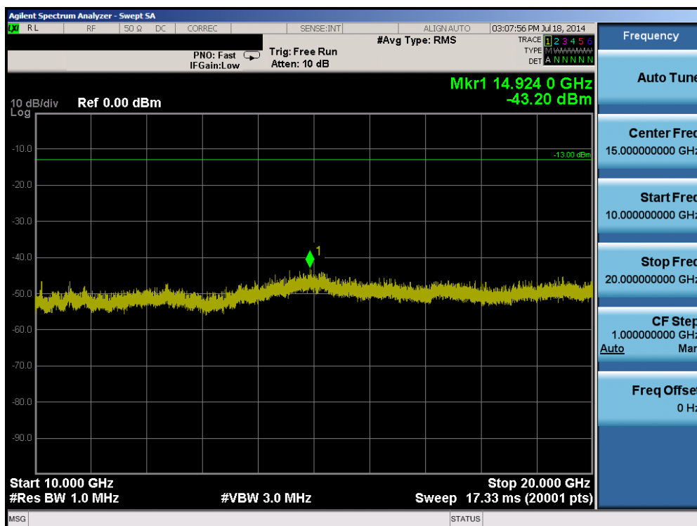
Plot 6-18. Conducted Spurious Plot (Band 4 – 20.0MHz QPSK – RB Size 1, RB Offset 0 – Mid Channel)
