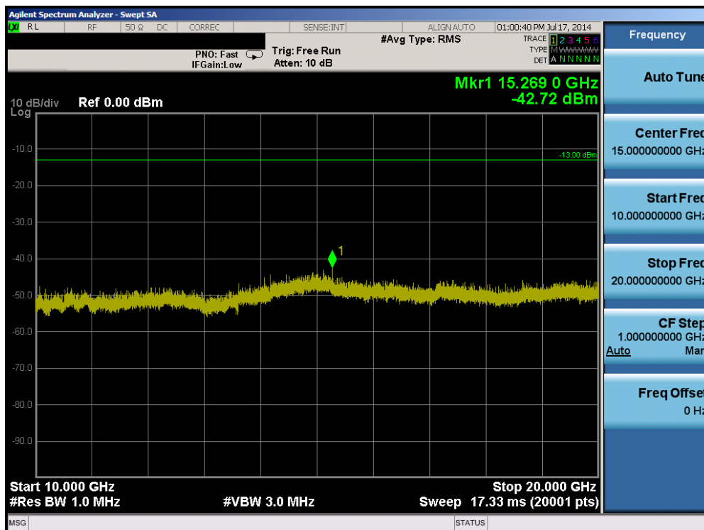
Plot 6-14. Conducted Spurious Plot (Band 4 – 15.0MHz QPSK – RB Size 1, RB Offset 0 – High Channel)
