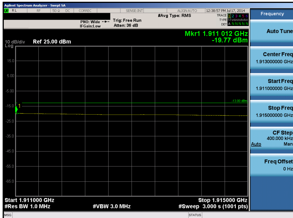
Plot 6-48. Upper Extended Band Edge Plot (Band 2 – 20.0MHz QPSK – RB Size 100)
