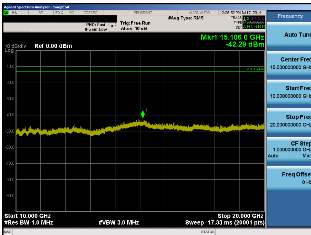
Plot 6-30. Conducted Spurious Plot (Band 2 – 20.0MHz QPSK – RB Size 1, RB Offset 0 – Mid Channel)
