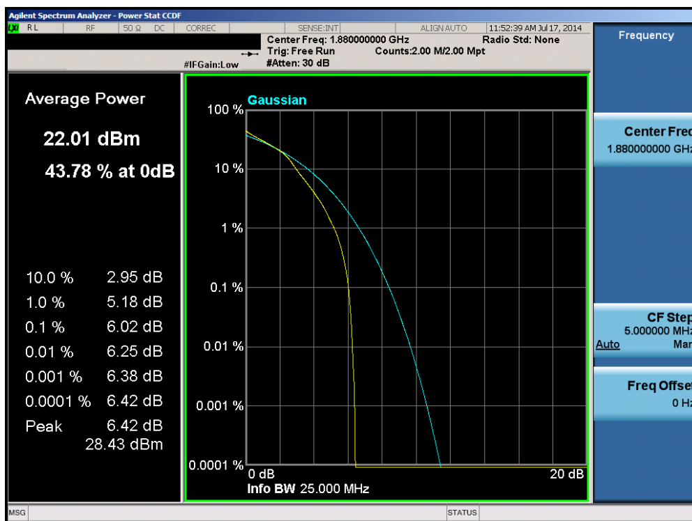
Plot 6-50. PAR Plot (Band 2 – 15.0MHz 16-QAM – RB Size 75)
