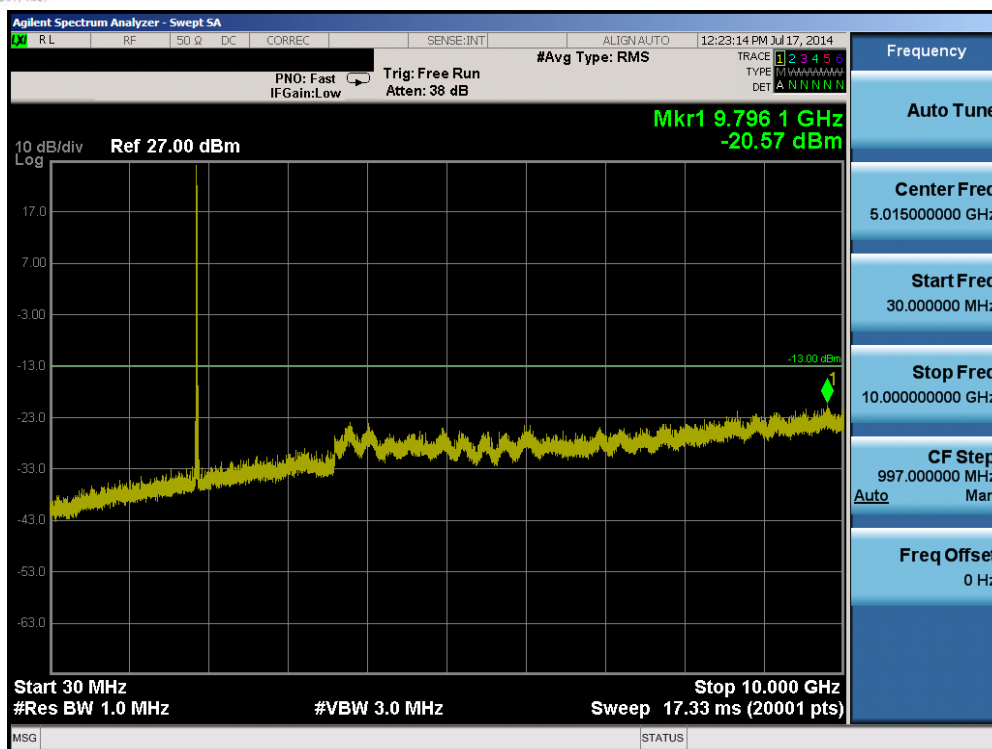
Plot 6-29. Conducted Spurious Plot (Band 2 – 20.0MHz QPSK – RB Size 1, RB Offset 0 – Mid Channel)
