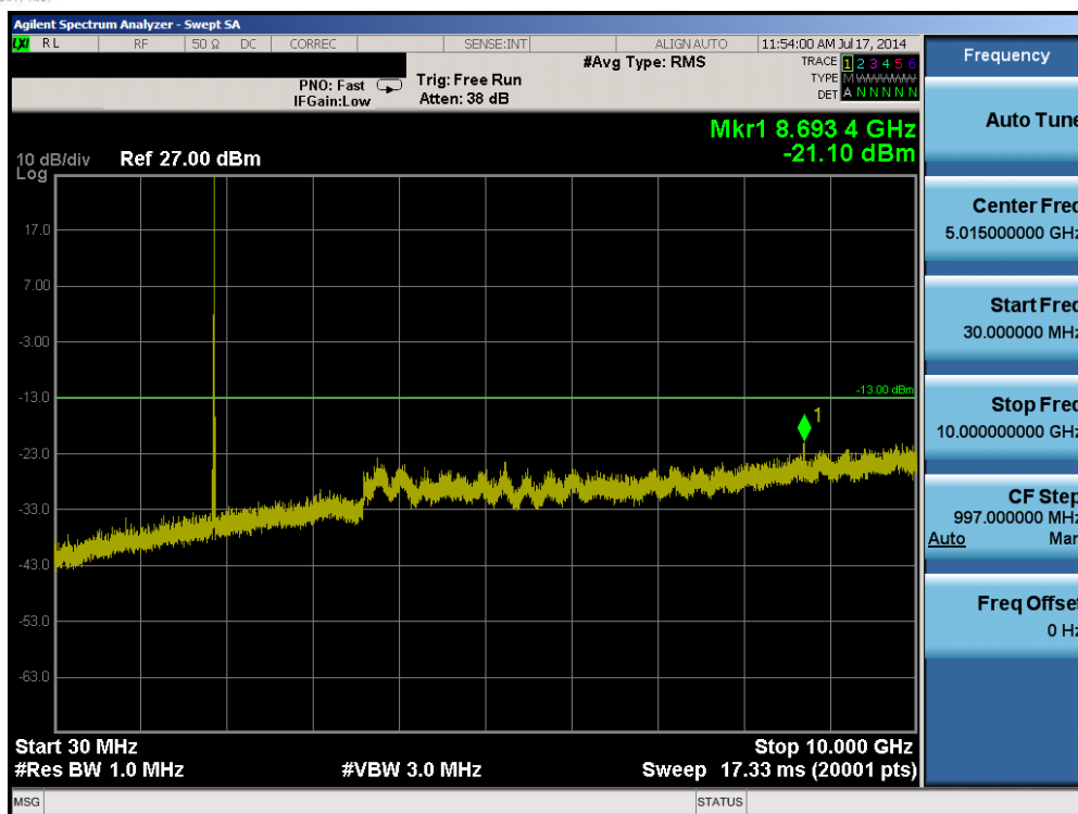
Plot 6-23. Conducted Spurious Plot (Band 2 – 15.0MHz QPSK – RB Size 1, RB Offset 0 – Mid Channel)
