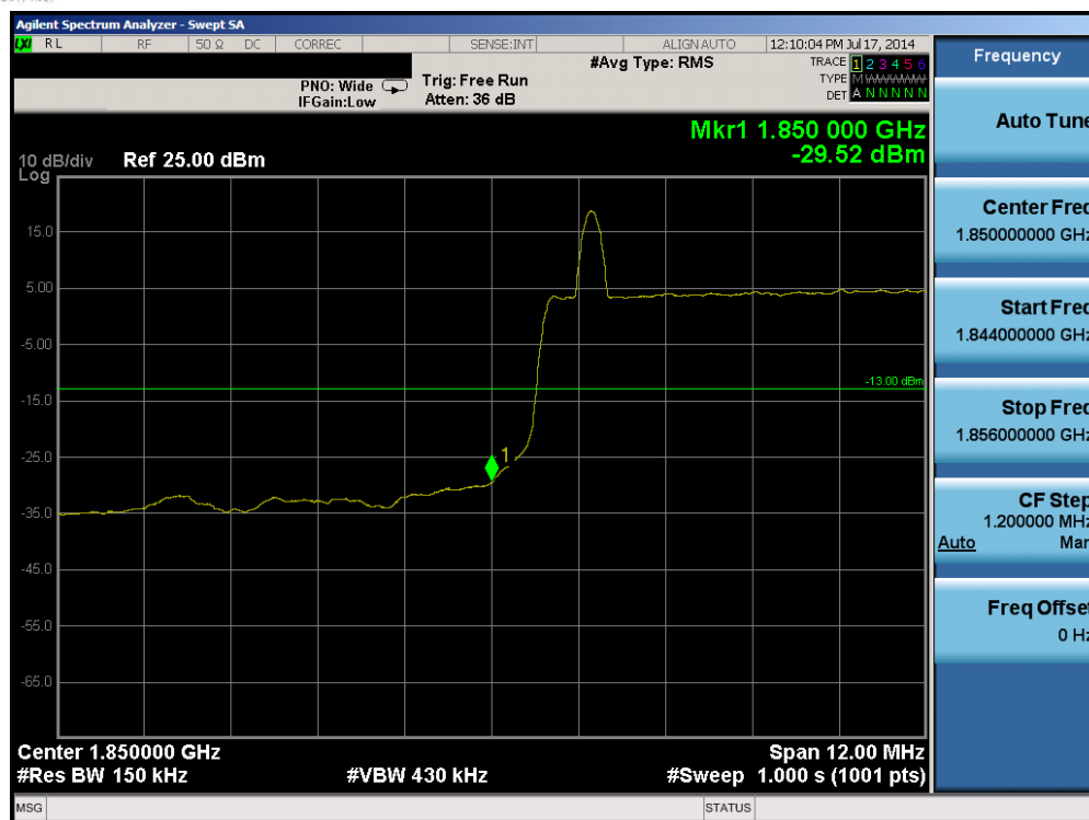
Plot 6-41. Lower Band Edge Plot (Band 2 – 15.0MHz QPSK – RB Size 75)
