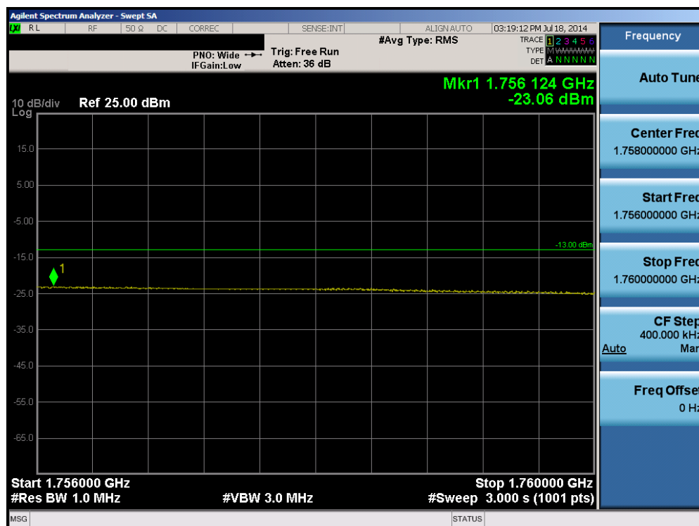
Plot 6-40. Upper Extended Band Edge Plot (Band 4 – 20.0MHz QPSK – RB Size 100)
