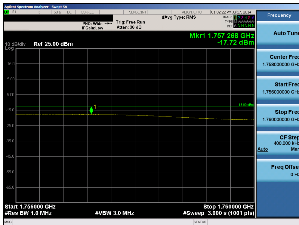
Plot 6-36. Upper Extended Band Edge Plot (Band 4 – 15.0MHz QPSK – RB Size 75)
