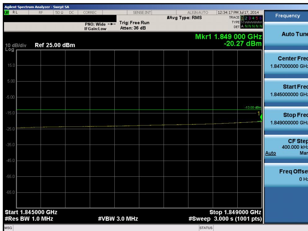
Plot 6-46. Lower Extended Band Edge Plot (Band 2 – 20.0MHz QPSK – RB Size 100)
