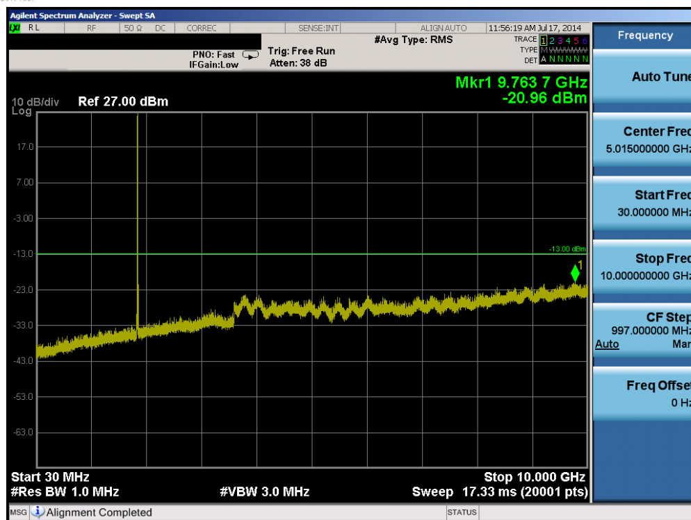
Plot 6-21. Conducted Spurious Plot (Band 2 – 15.0MHz QPSK – RB Size 1, RB Offset 0 – Low Channel)
