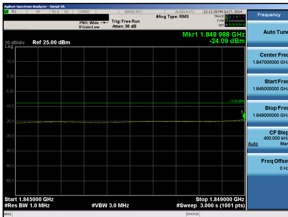
Plot 6-42. Lower Extended Band Edge Plot (Band 2 – 15.0MHz QPSK – RB Size 75)
