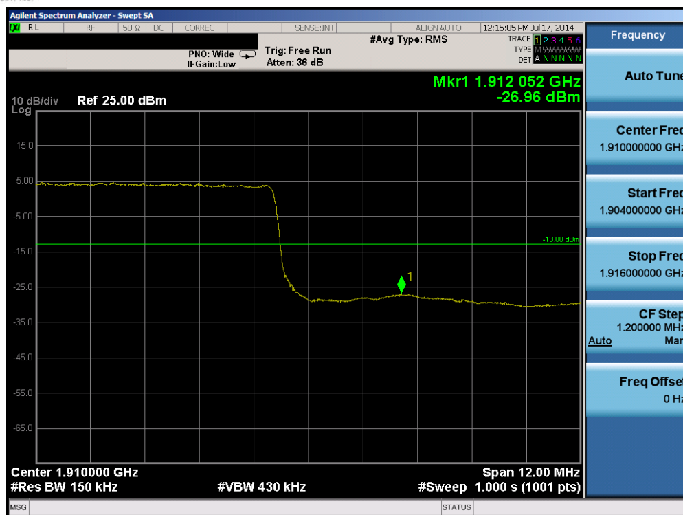
Plot 6-43. Upper Band Edge Plot (Band 2 – 15.0MHz QPSK – RB Size 75)
