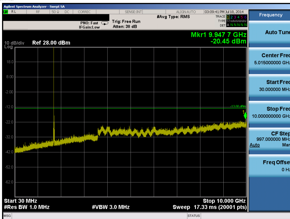
Plot 6-15. Conducted Spurious Plot (Band 4 – 20.0MHz QPSK – RB Size 1, RB Offset 0– Low Channel)
