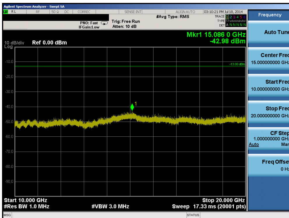
Plot 6-16. Conducted Spurious Plot (Band 4 – 20.0MHz QPSK – RB Size 1, RB Offset 0 – Low Channel)
