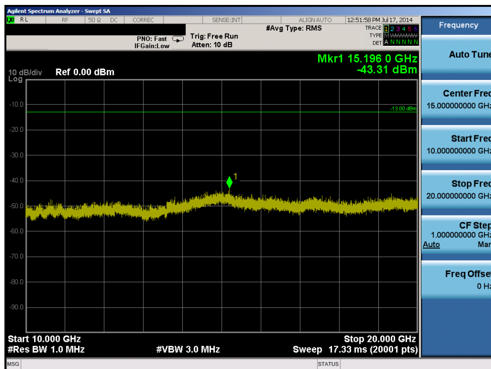
Plot 6-10. Conducted Spurious Plot (Band 4 – 15.0MHz QPSK – RB Size 1, RB Offset 0 – Low Channel)
