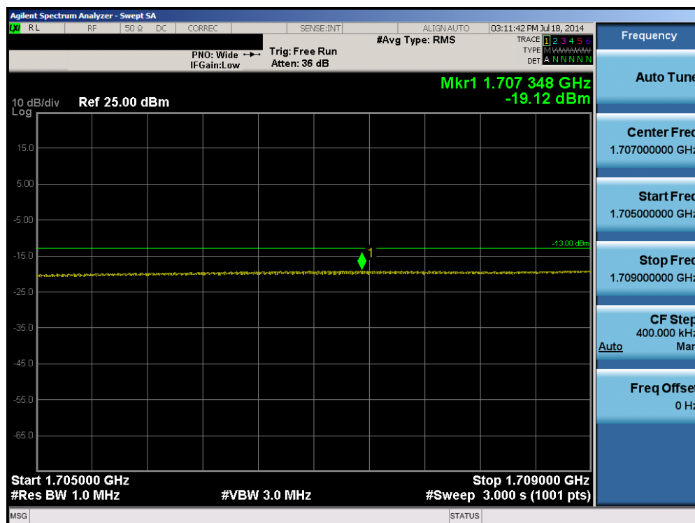
Plot 6-38. Lower Extended Band Edge Plot (Band 4 – 20.0MHz QPSK – RB Size 100)
