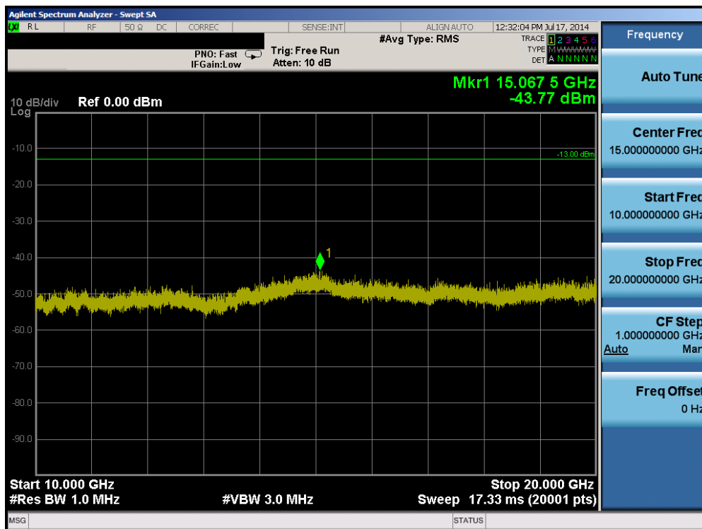
Plot 6-28. Conducted Spurious Plot (Band 2 – 20.0MHz QPSK – RB Size 1, RB Offset 0 – Low Channel)
