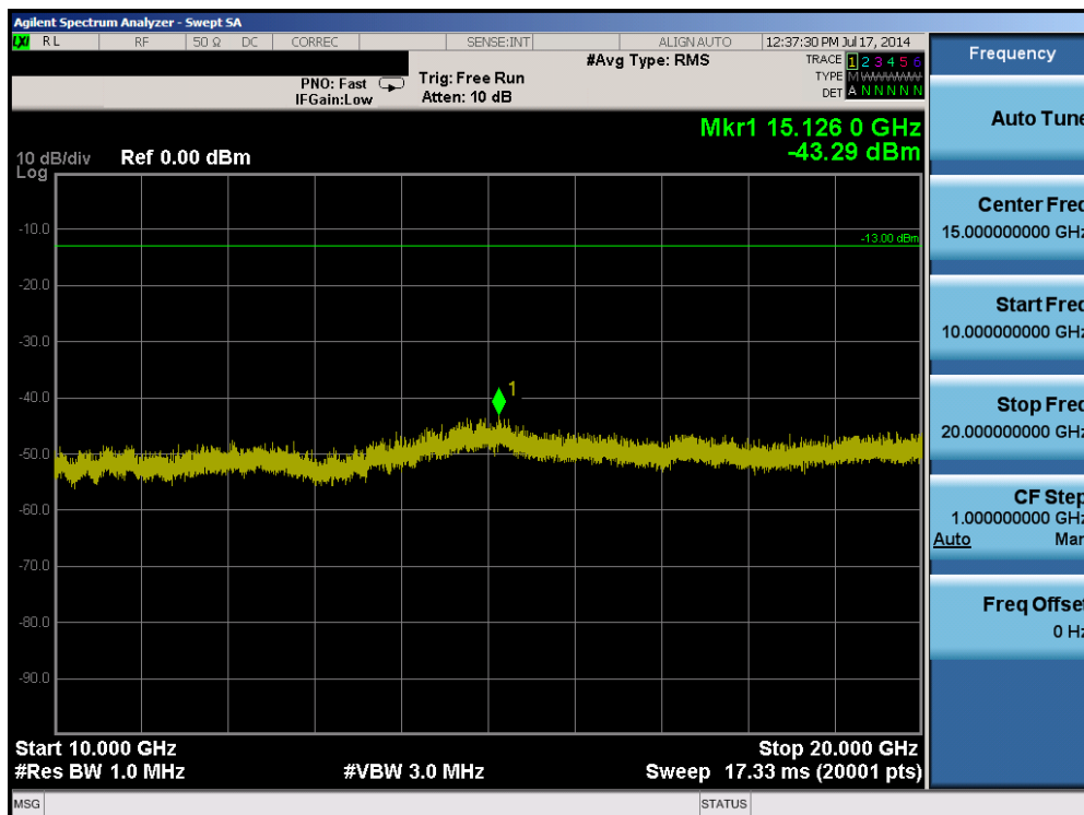
Plot 6-32. Conducted Spurious Plot (Band 2 – 20.0MHz QPSK – RB Size 1, RB Offset 0 – High Channel)
