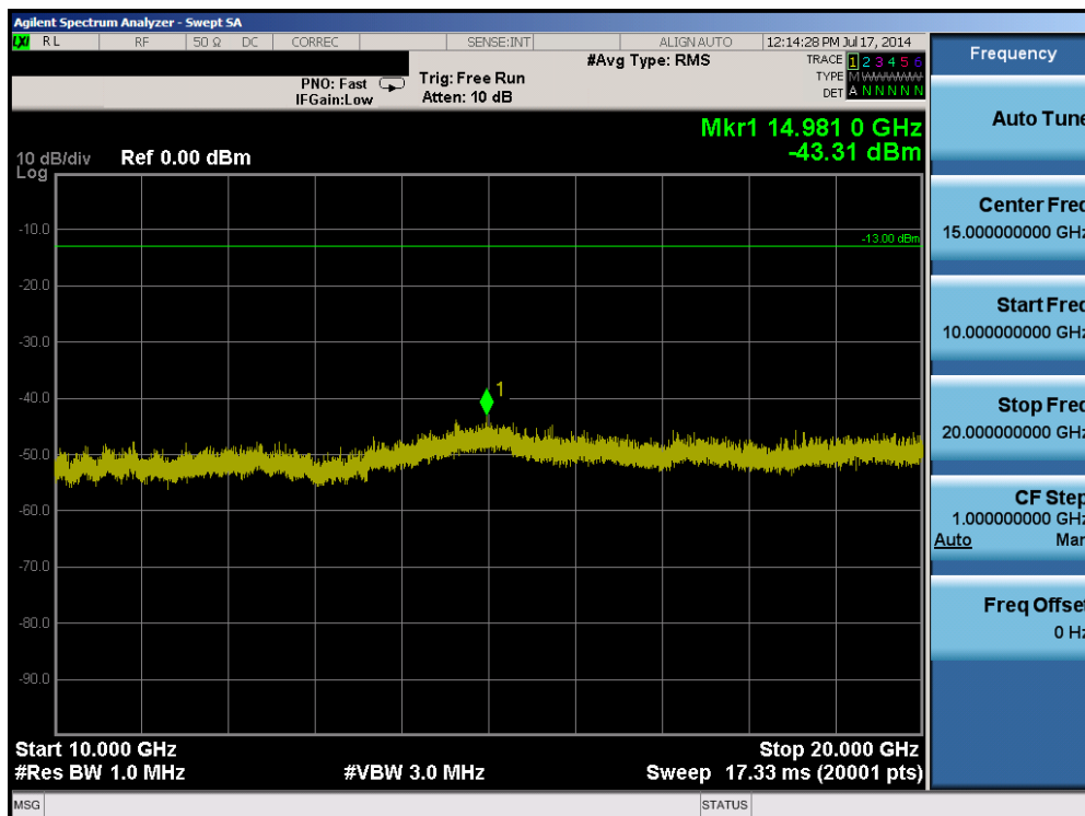
Plot 6-26. Conducted Spurious Plot (Band 2 – 15.0MHz QPSK – RB Size 1, RB Offset 0 – High Channel)
