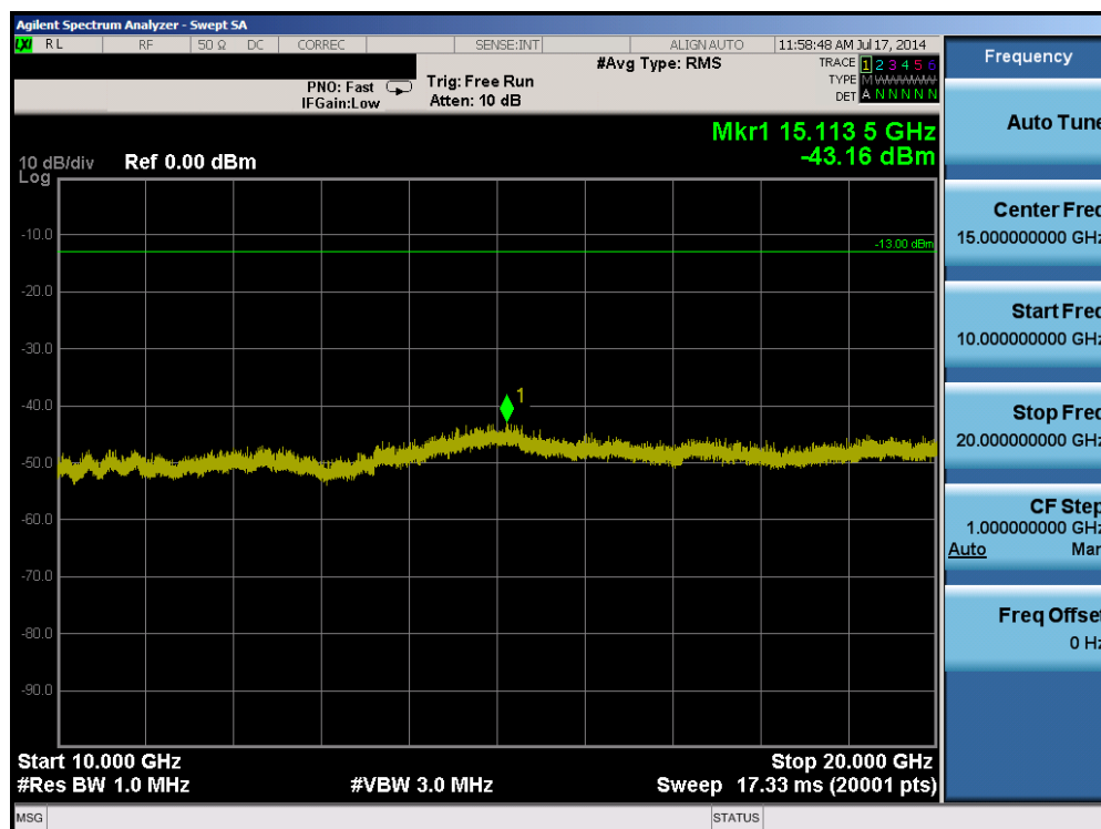
Plot 6-22. Conducted Spurious Plot (Band 2 – 15.0MHz QPSK – RB Size 1, RB Offset 0 – Low Channel)
