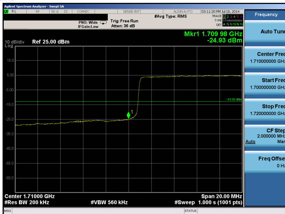
Plot 6-37. Lower Band Edge Plot (Band 4 – 20.0MHz QPSK – RB Size 100)
