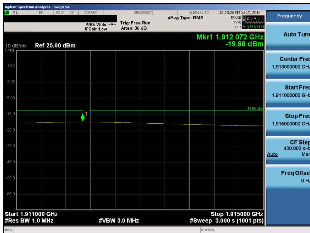
Plot 6-44. Upper Extended Band Edge Plot (Band 2 – 15.0MHz QPSK – RB Size 75)
