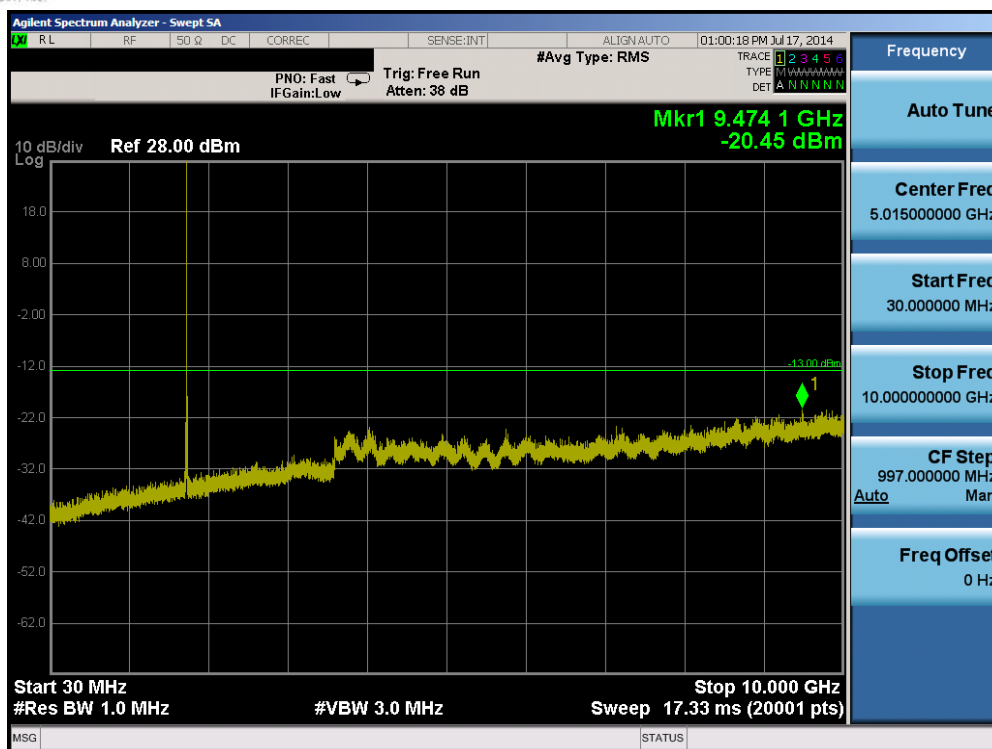
Plot 6-13. Conducted Spurious Plot (Band 4 – 15.0MHz QPSK – RB Size 1, RB Offset 0 – High Channel)
