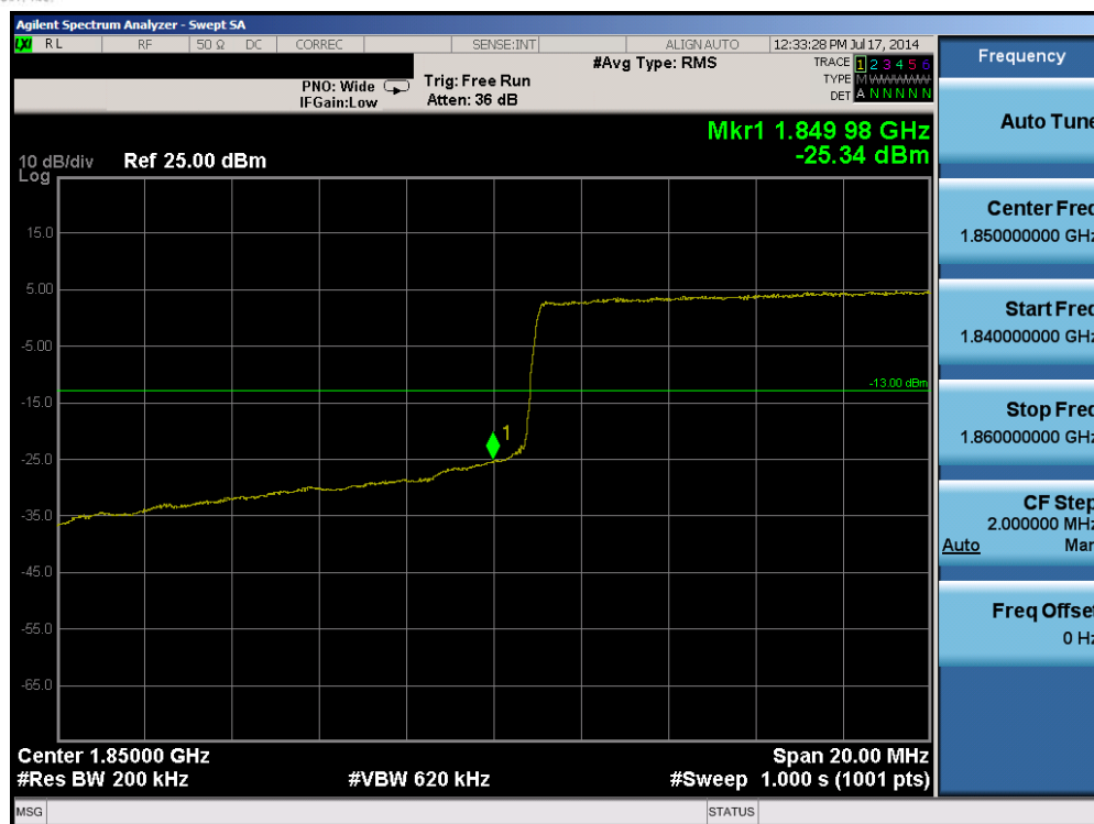
Plot 6-45. Lower Band Edge Plot (Band 2 – 20.0MHz QPSK – RB Size 100)
