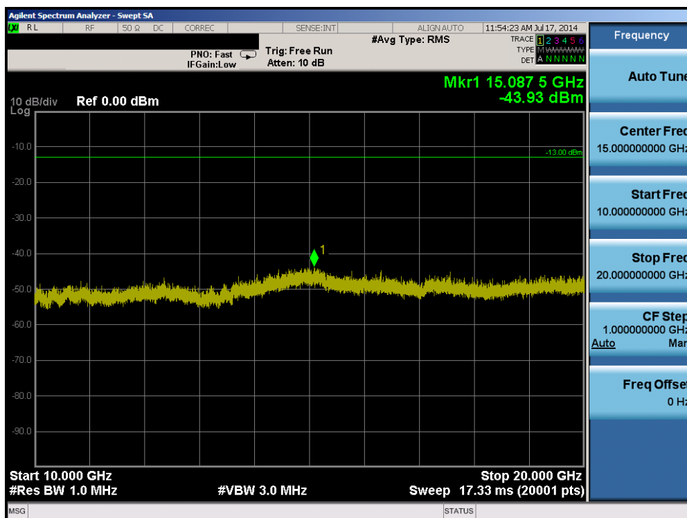
Plot 6-24. Conducted Spurious Plot (Band 2 – 15.0MHz QPSK – RB Size 1, RB Offset 0 – Mid Channel)
