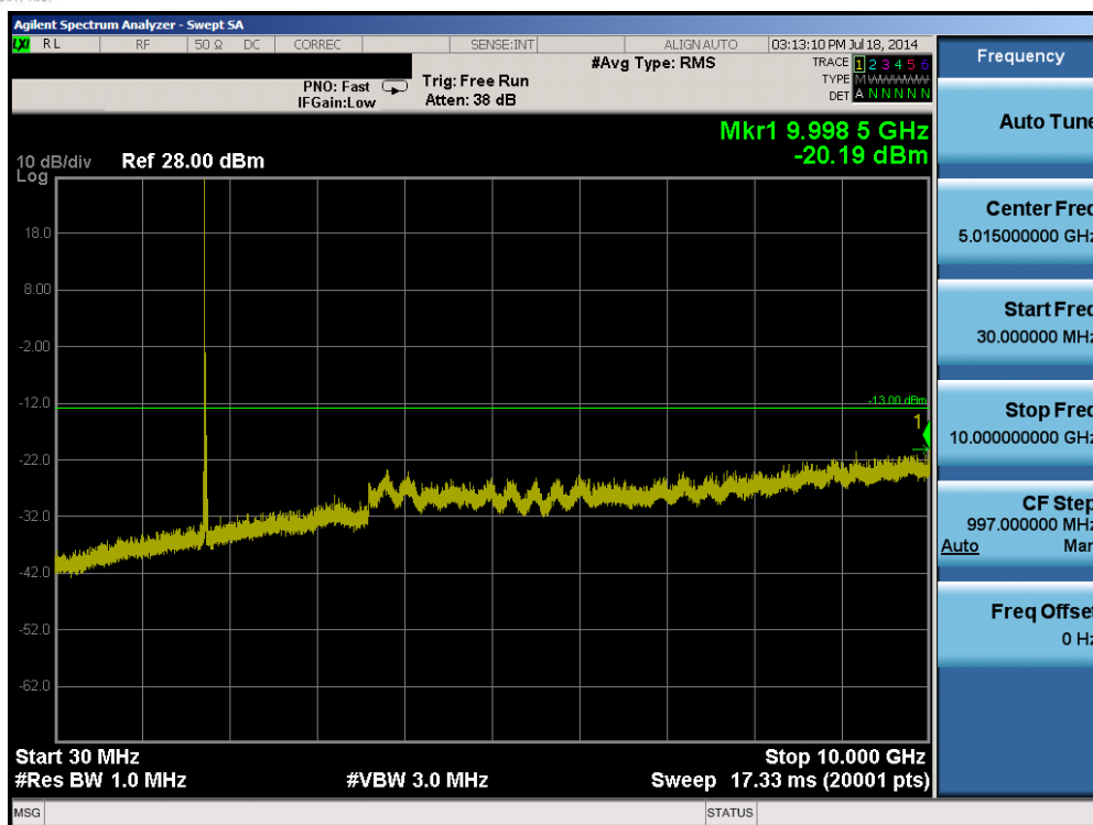
Plot 6-19. Conducted Spurious Plot (Band 4 – 20.0MHz QPSK – RB Size 1, RB Offset 0 – High Channel)
