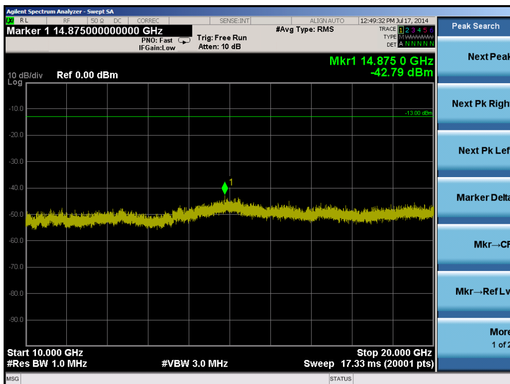
Plot 6-12. Conducted Spurious Plot (Band 4 – 15.0MHz QPSK – RB Size 1, RB Offset 0 – Mid Channel)
