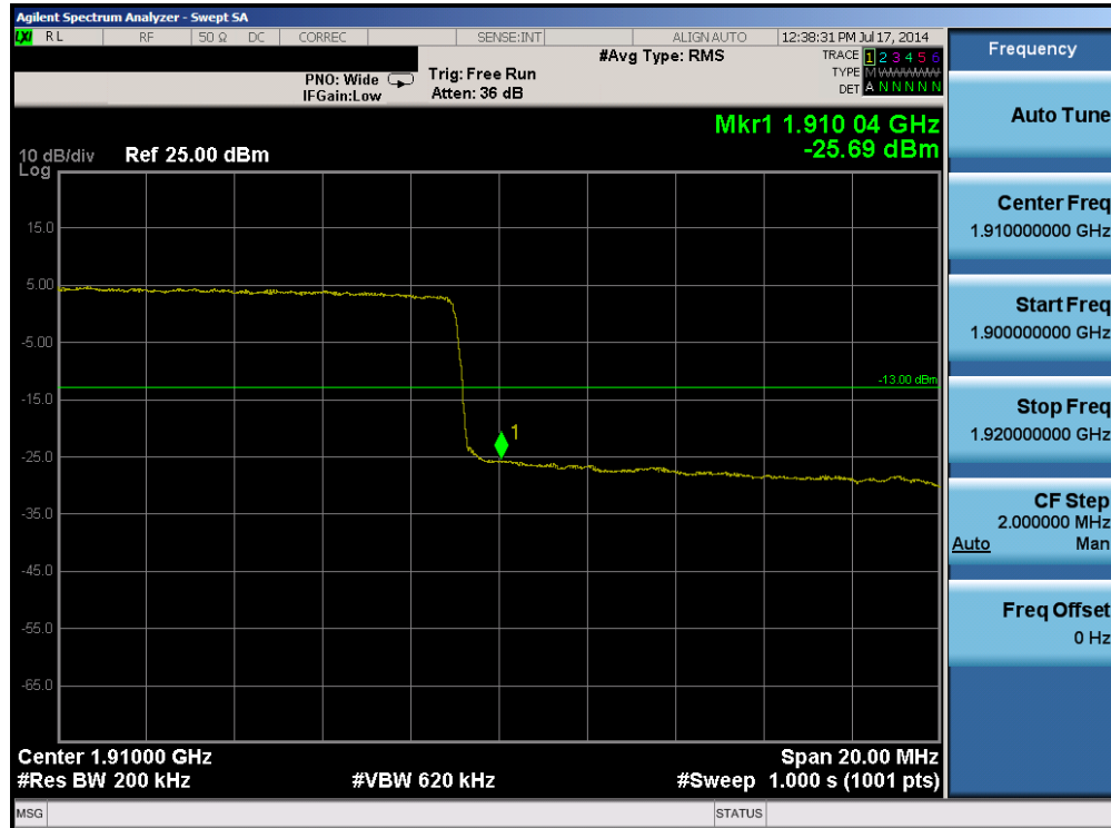
Plot 6-47. Upper Band Edge Plot (Band 2 – 20.0MHz QPSK – RB Size 100)
