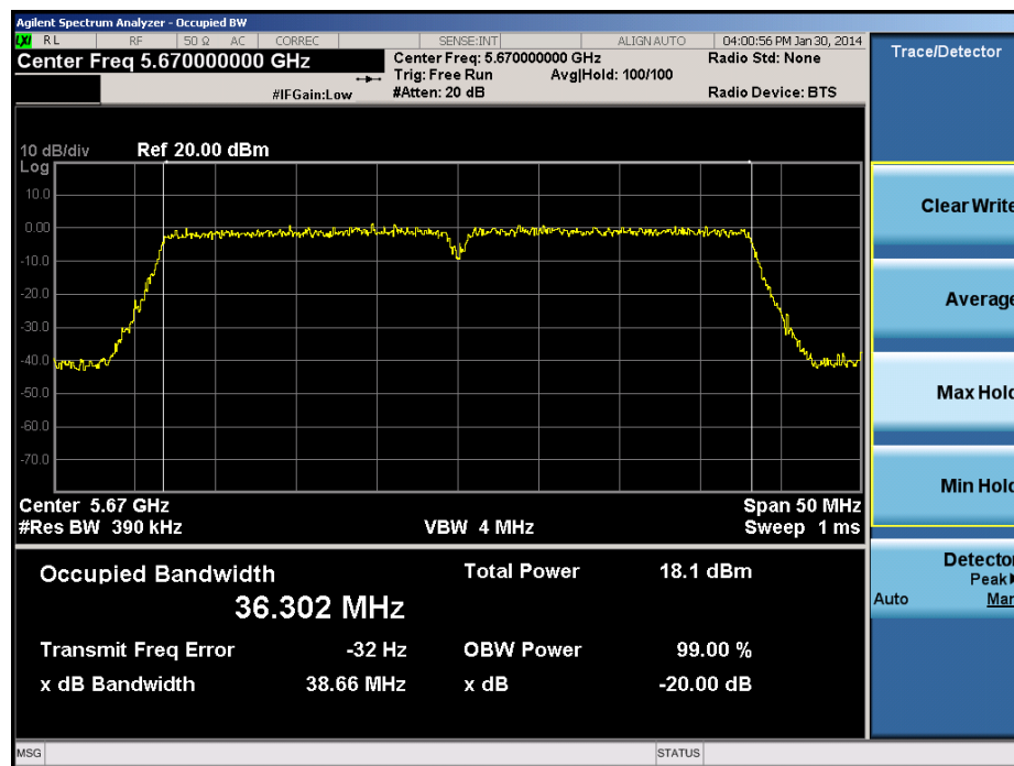
Plot 6-32. 20dB Bandwidth Plot (40MHz BW 802.11n (UNII Band 2C) – Ch. 134)
