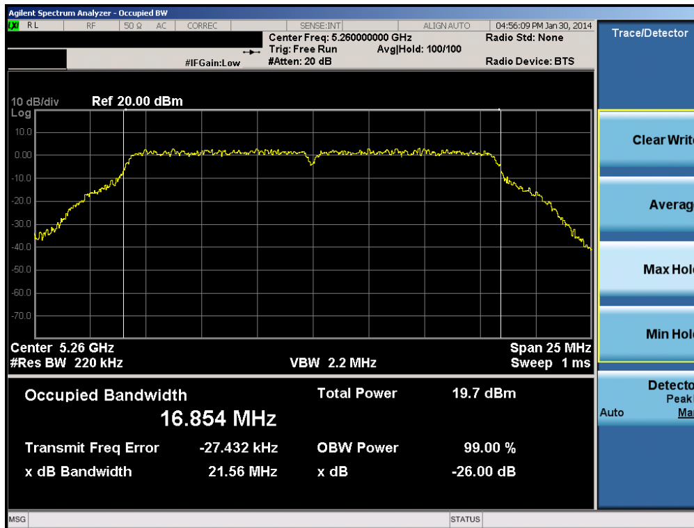
Plot 6-43. 26dB Bandwidth Plot (802.11a (UNII Band 2A) – Ch. 52)
