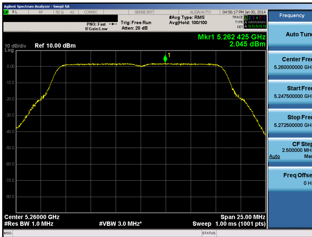
Plot 6-104. Peak Power Spectral Density Plot (802.11a (UNII Band 2A) – Ch. 52)
