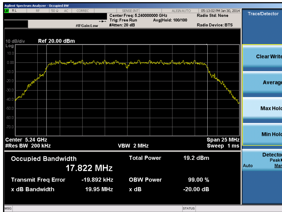
Plot 6-63. 20dB Bandwidth Plot (20MHz BW 802.11n (UNII Band 1) – Ch. 48)
