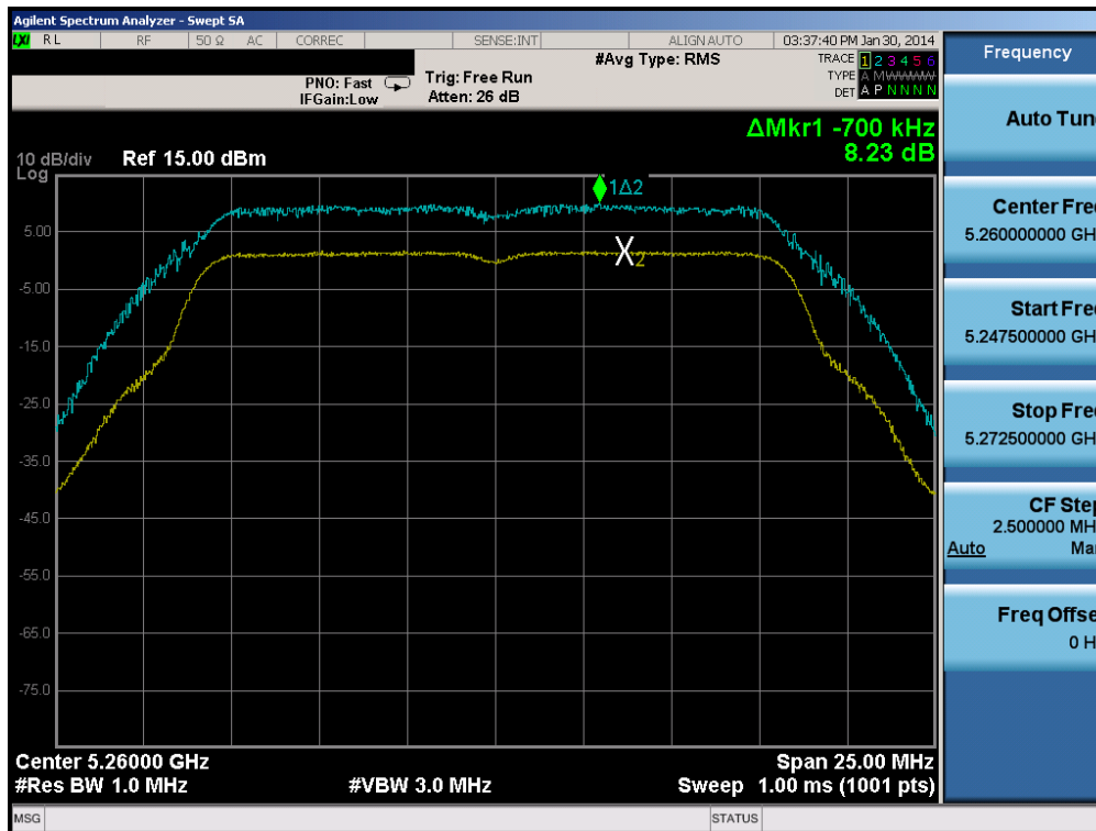
Plot 6-132. Peak Excursion Ratio Plot (802.11a (UNII Band 2A) – Ch. 52)
