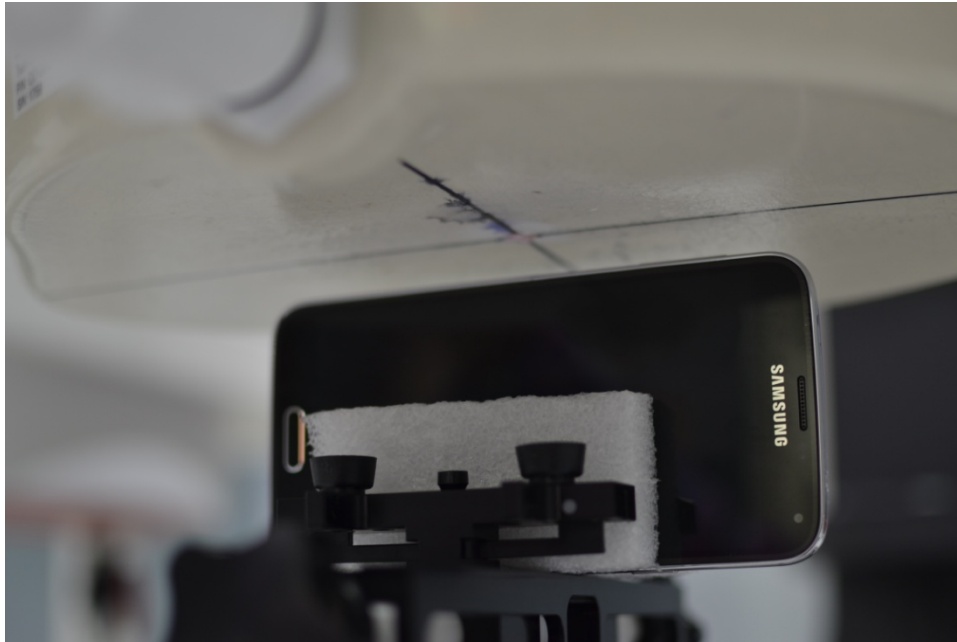
SAR Test Setup Photo 17: Left Edge at 1.0 cm with Standard Cover
