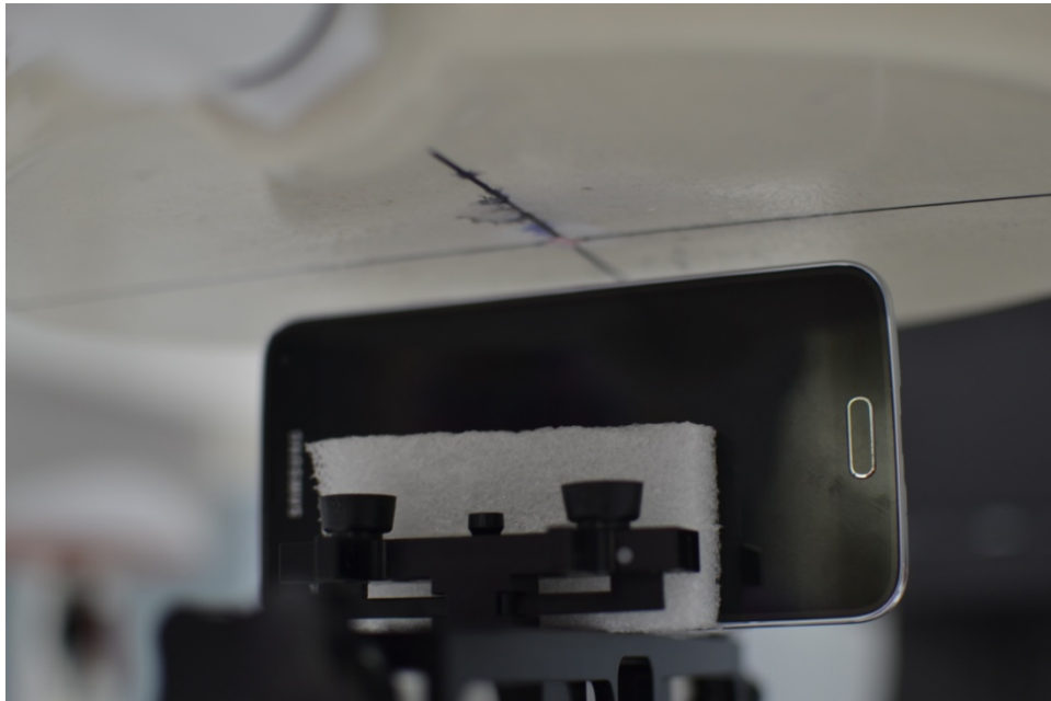
SAR Test Setup Photo 12: Right Edge at 1.0 cm with Standard Cover
