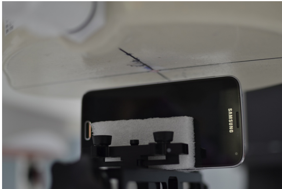
SAR Test Setup Photo 11: Left Edge at 1.0 cm with Standard Cover
