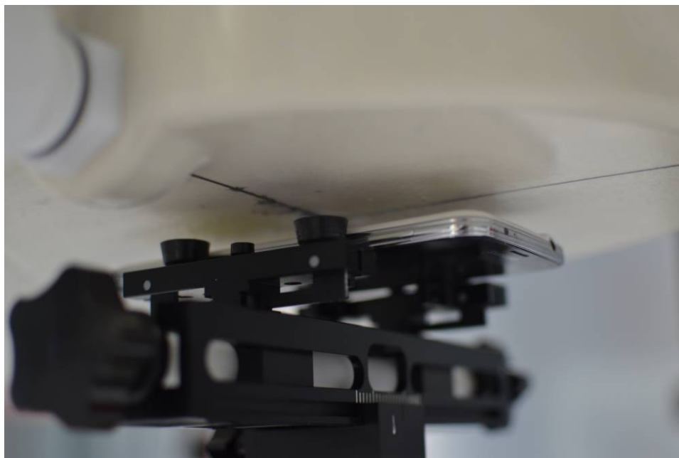
SAR Test Setup Photo 6: Back Side at 1.0 cm with Standard Cover
