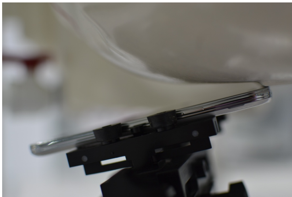
SAR Test Setup Photo 5: Left Tilt with Standard Cover
