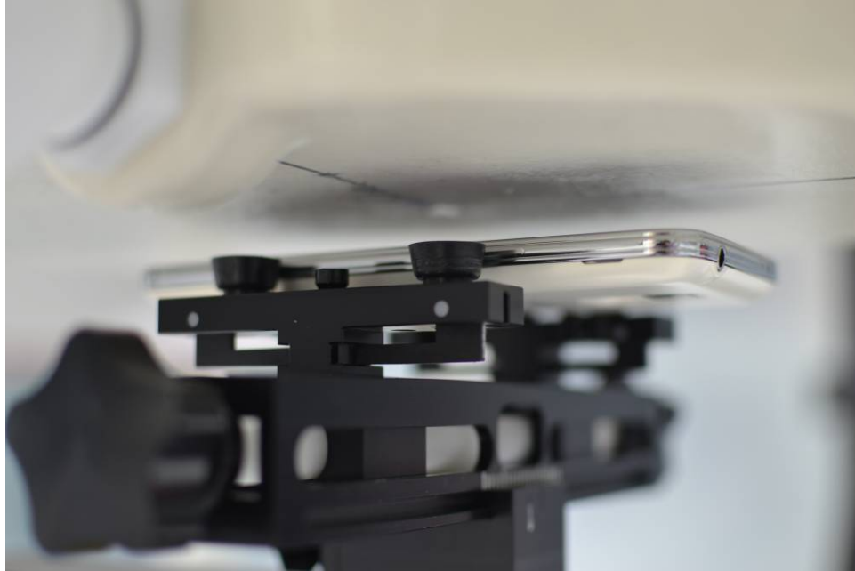
SAR Test Setup Photo 9: Front Side at 1.0 cm with Wireless Charging Cover
