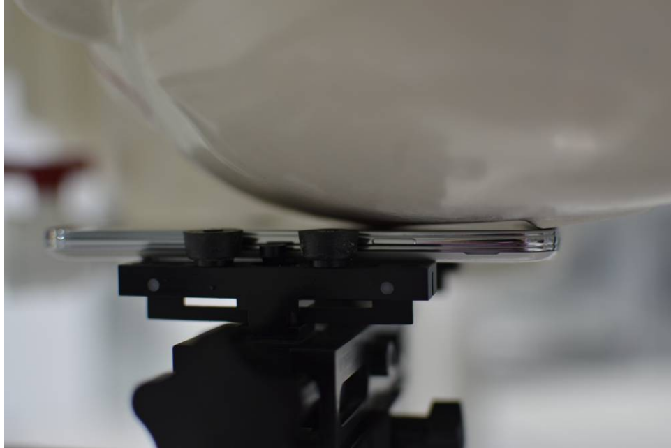
SAR Test Setup Photo 3: Left Cheek with Standard Cover
