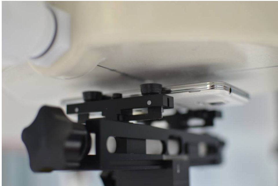
SAR Test Setup Photo 8: Front Side at 1.0 cm with Standard Cover
