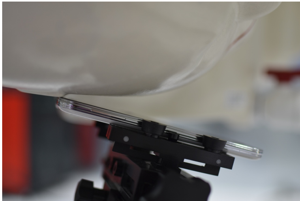
SAR Test Setup Photo 2: Right Tilt with Standard Cover
