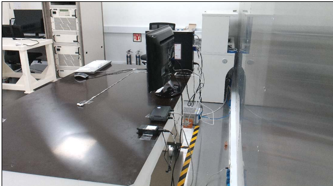
[ Conducted Disturbance – Rear ]
