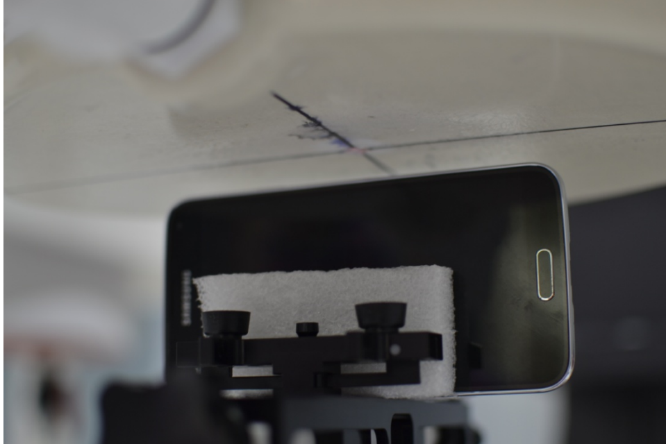
SAR Test Setup Photo 17: Right Edge at 1.0 cm with Standard Cover
