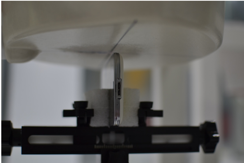
SAR Test Setup Photo 18: Right Edge at 1.0 cm with Wireless Charging Cover
