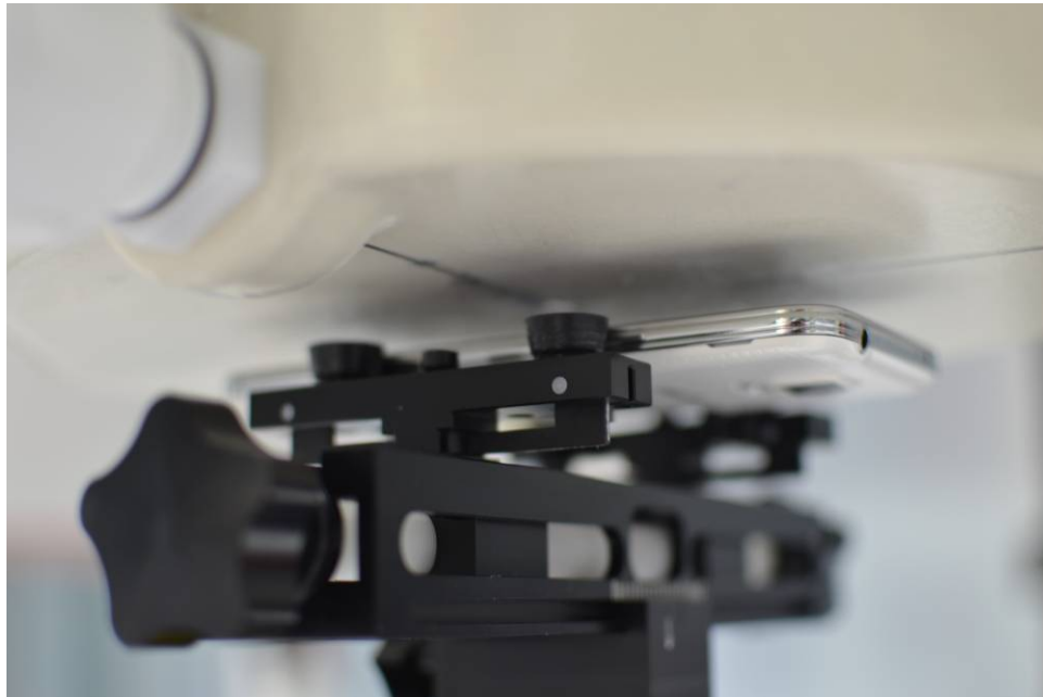
SAR Test Setup Photo 12: Front Side at 1.0 cm with Standard Cover
