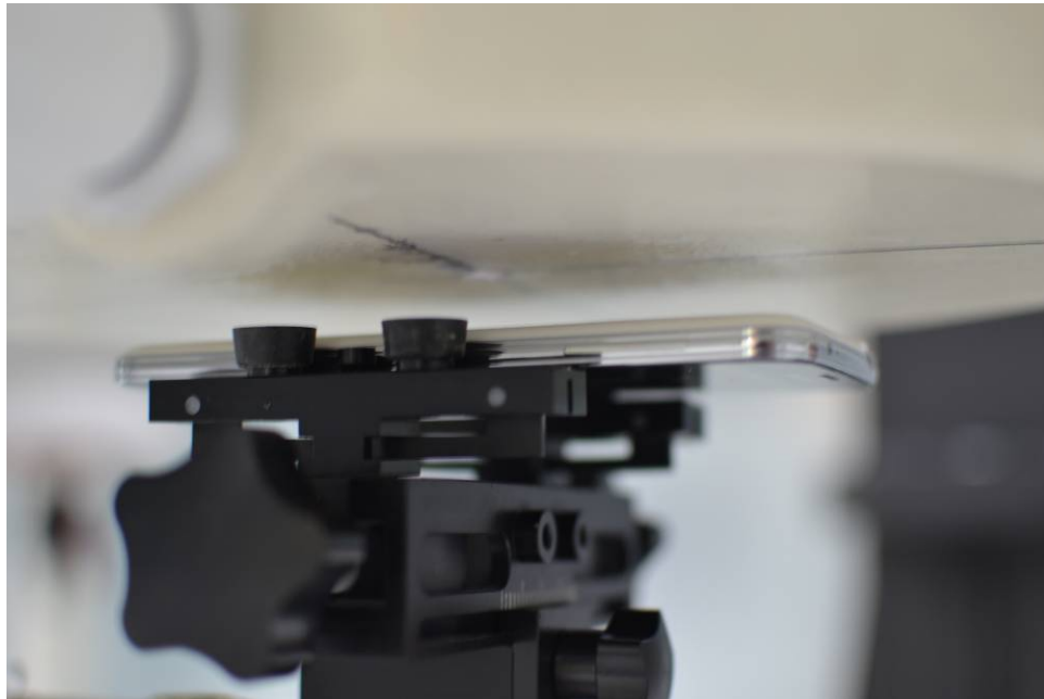
SAR Test Setup Photo 10: Back Side at 1.5 cm with Standard Cover
