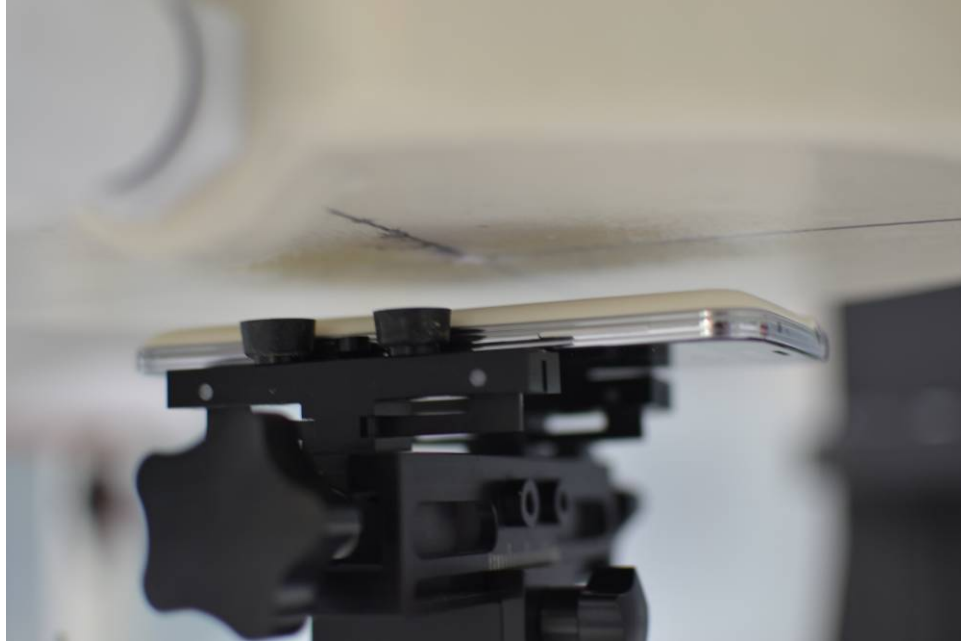
SAR Test Setup Photo 11: Back Side at 1.5 cm with Wireless Charging Cover
