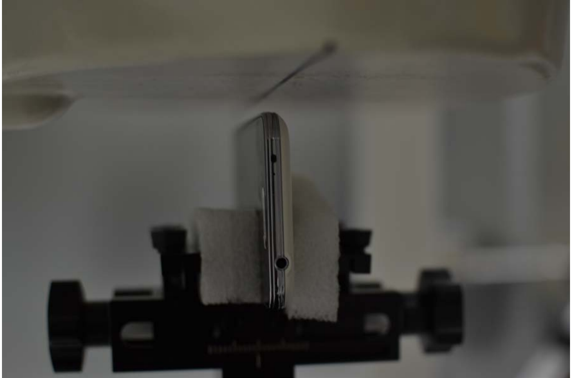
SAR Test Setup Photo 17 – Left Edge, Wireless Charging Cover at 1.0 cm
