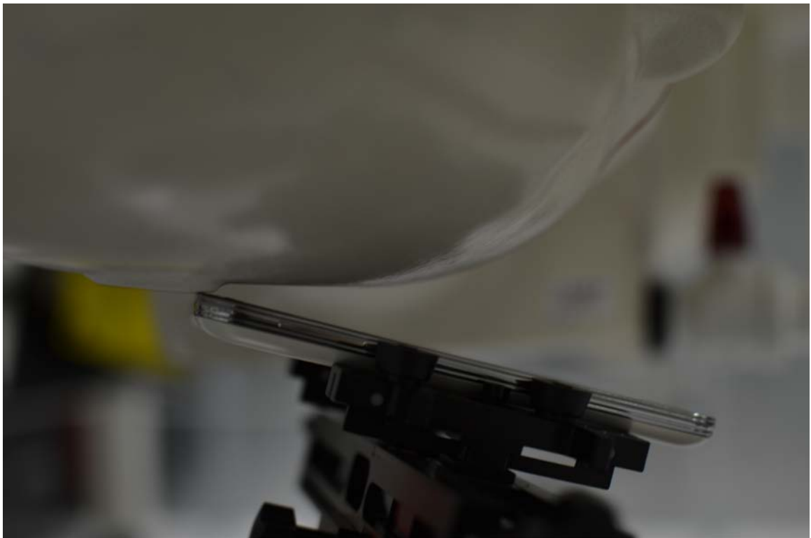
SAR Test Setup Photo 4 – Right Tilt, Wireless Charging Cover
