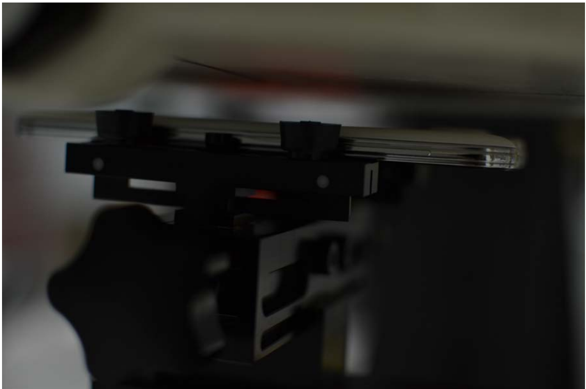
SAR Test Setup Photo 8 – Back Side, Standard Battery Cover at 1.0 cm
