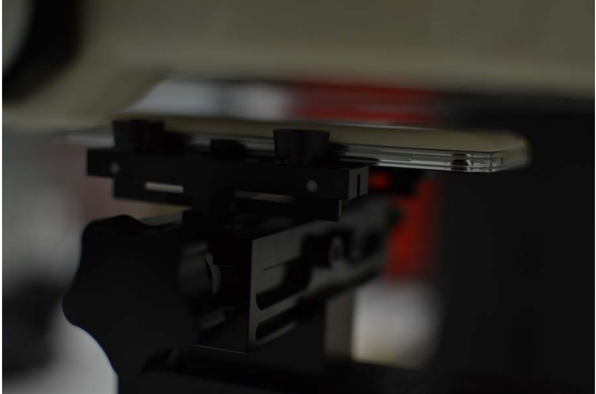
SAR Test Setup Photo 9 – Back Side, Wireless Charging Cover at 1.0 cm
