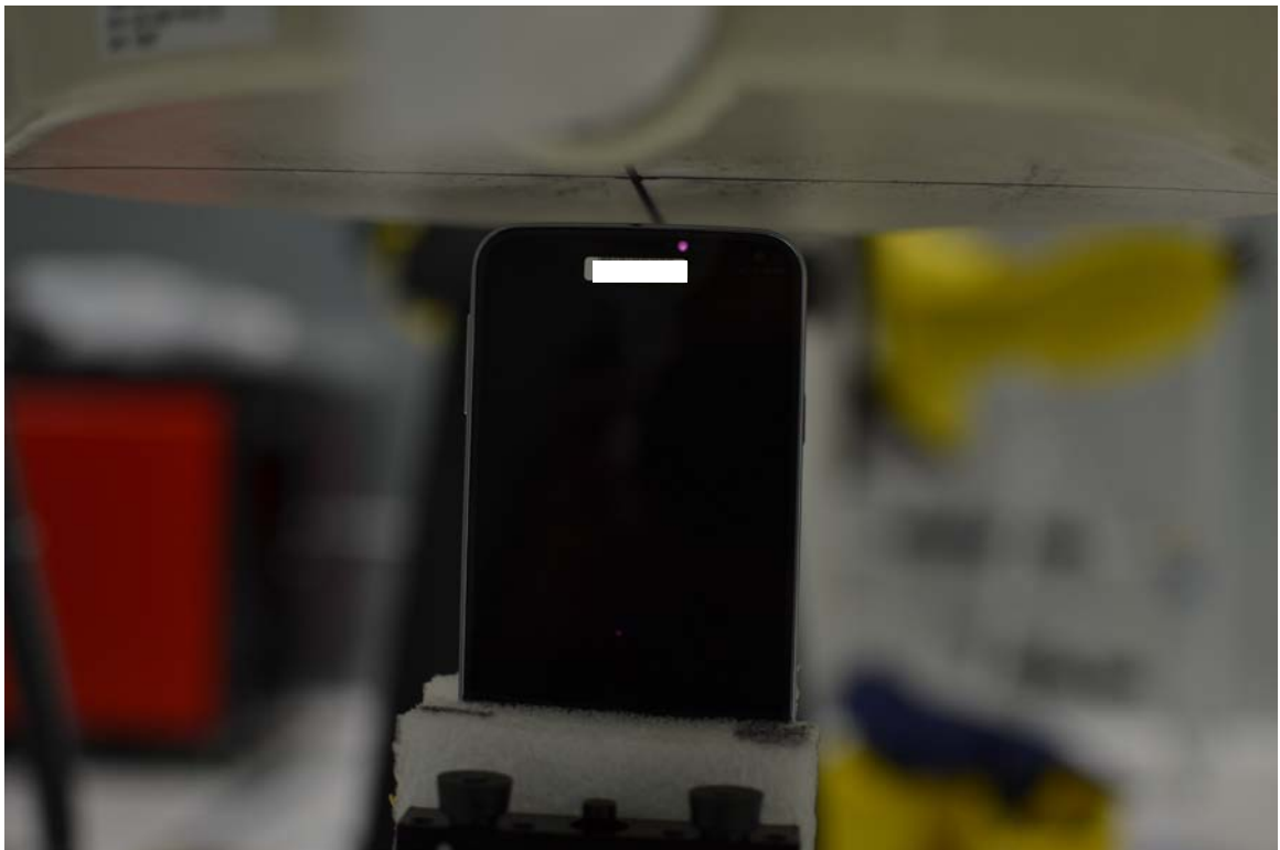
SAR Test Setup Photo 12 – Top Edge, Standard Battery Cover at 1.0 cm
