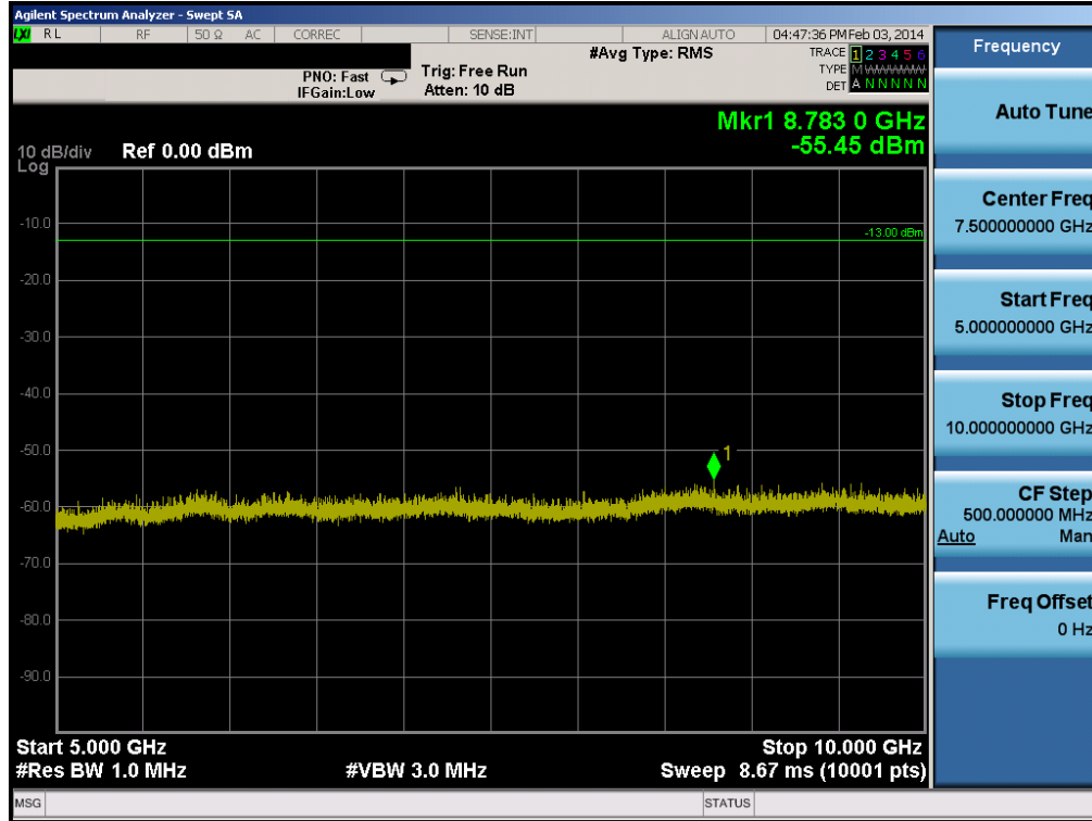
Plot 6-41. Conducted Spurious Plot (Cellular WCDMA Mode – Ch. 4233)
