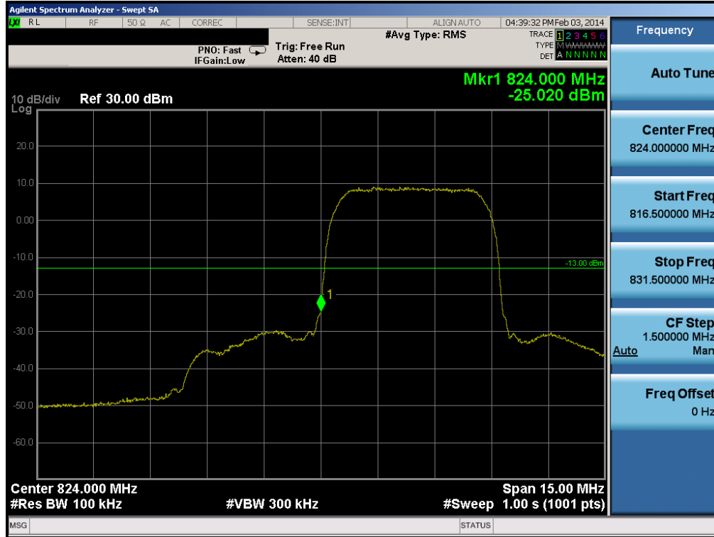
Plot 6-60. Band Edge Plot (Cellular WCDMA Mode – Ch. 4132)
