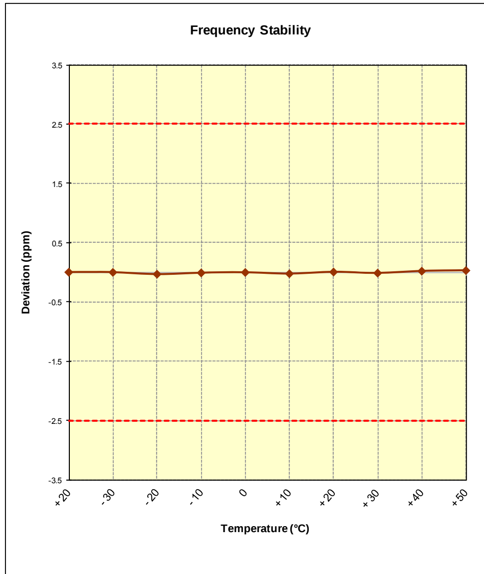
Figure 6-9. Frequency Stability Graph (Cellular WCDMA Mode – Ch. 4183)
