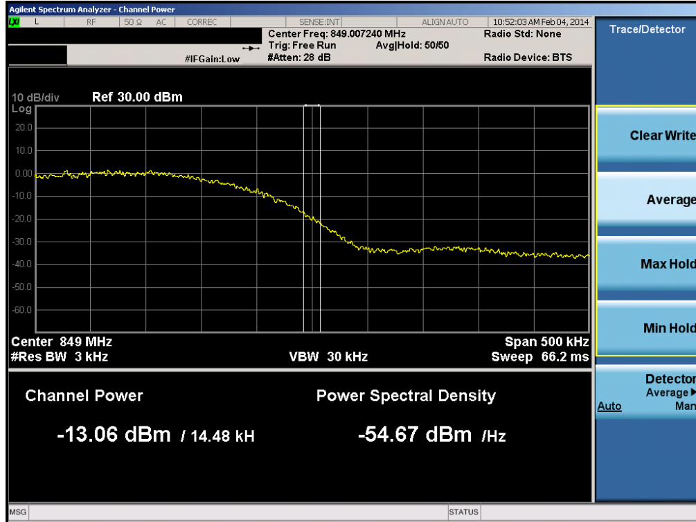
Plot 6-54. Band Edge Plot (Cellular CDMA Mode – Ch. 777)
