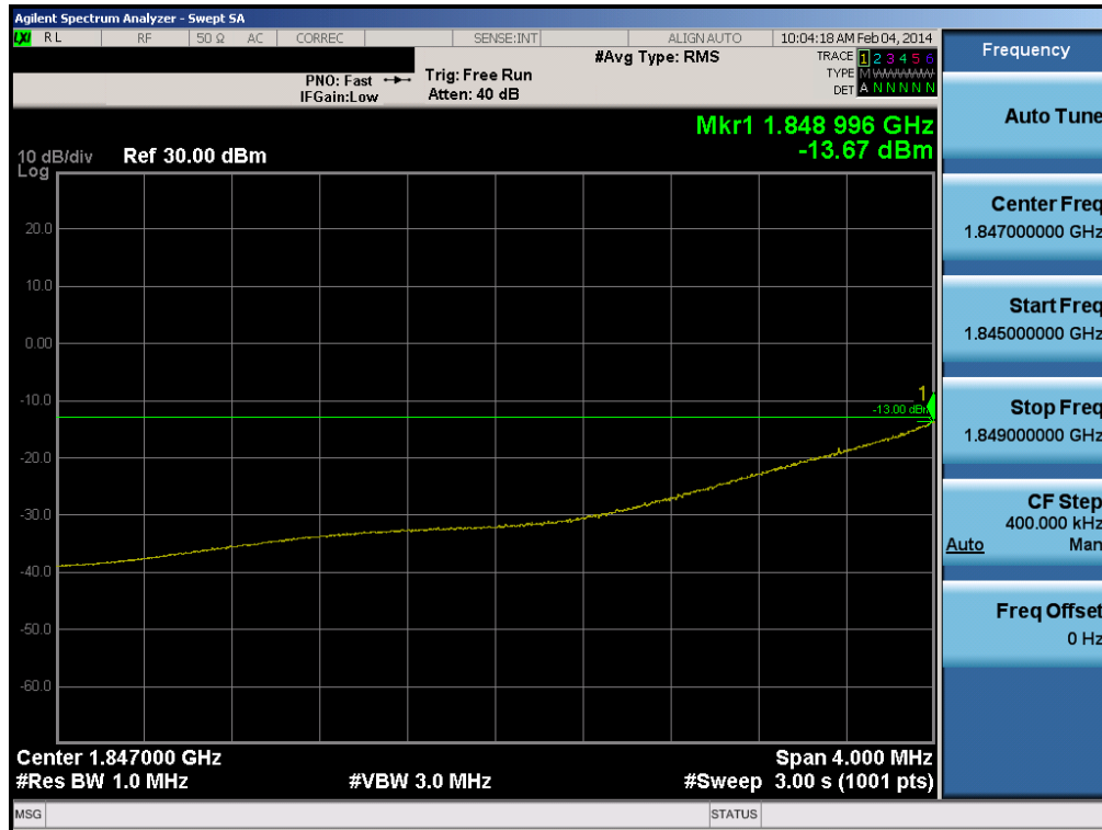
Plot 6-57. 4MHz Span Plot (PCS CDMA Mode – Ch. 25)
