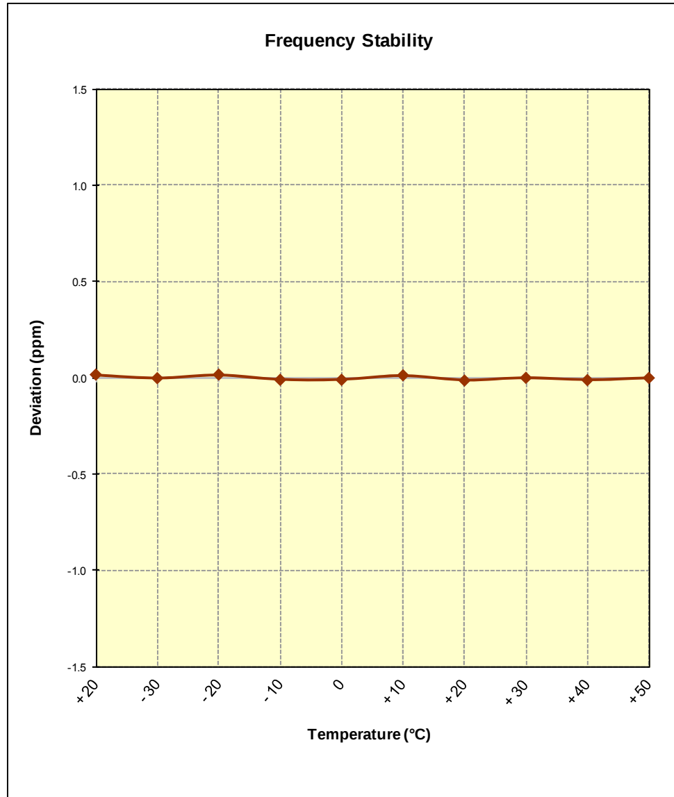
Figure 6-12. Frequency Stability Graph (PCS WCDMA Mode – Ch. 9400)
