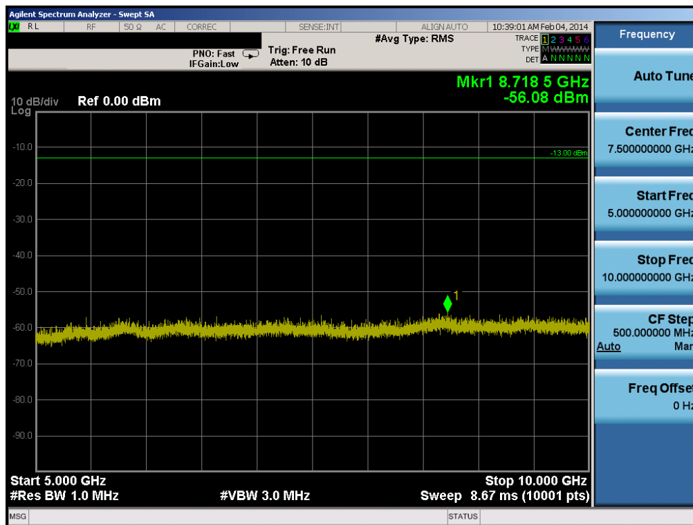
Plot 6-27. Conducted Spurious Plot (Cellular CDMA Mode – Ch. 384)
