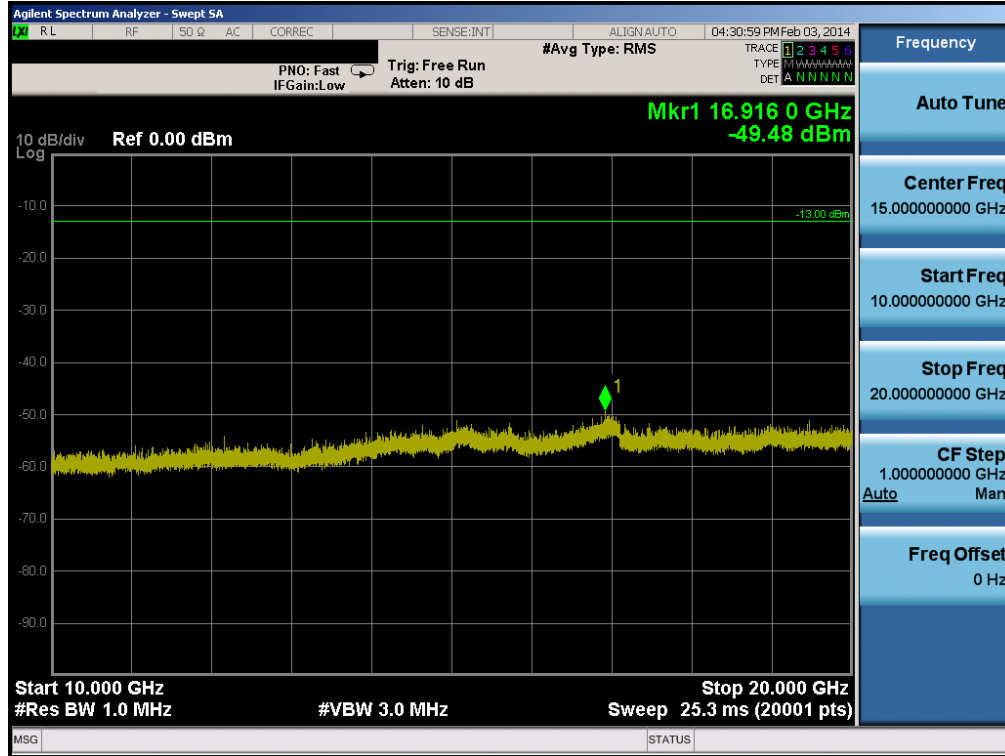
Plot 6-45. Conducted Spurious Plot (PCS WCDMA Mode – Ch. 9400)
