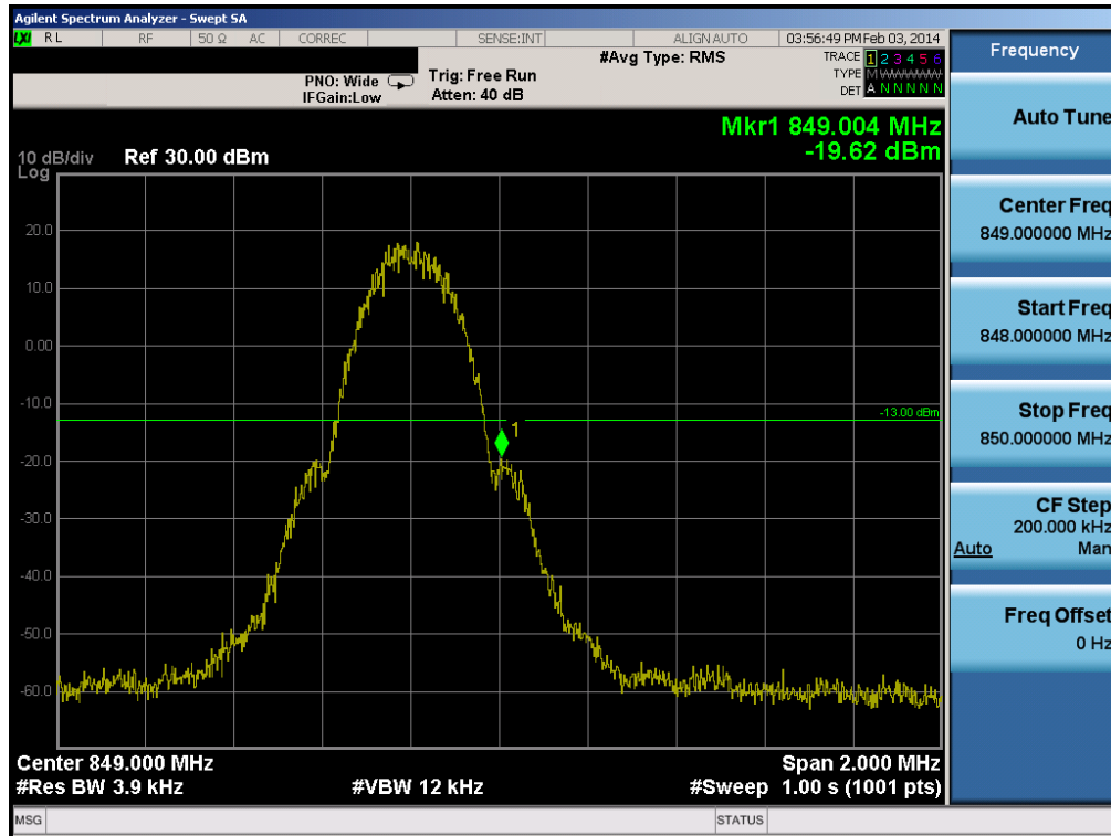
Plot 6-49. Band Edge Plot (Cellular GSM Mode – Ch. 251)
