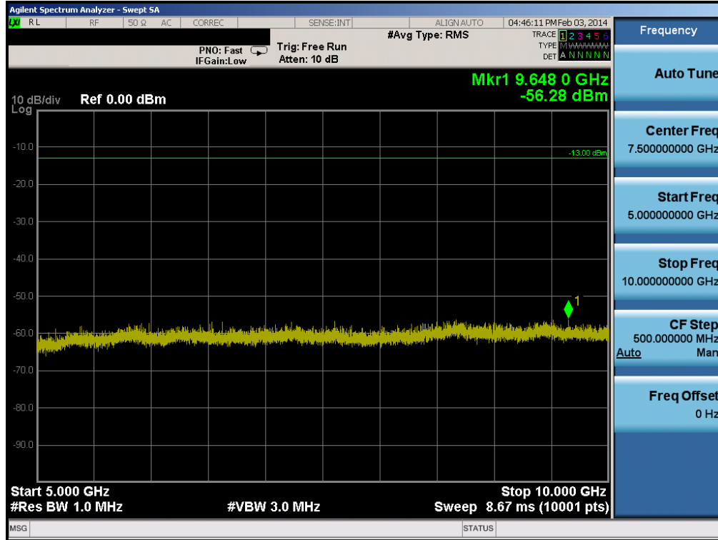
Plot 6-37. Conducted Spurious Plot (Cellular WCDMA Mode – Ch. 4132)
