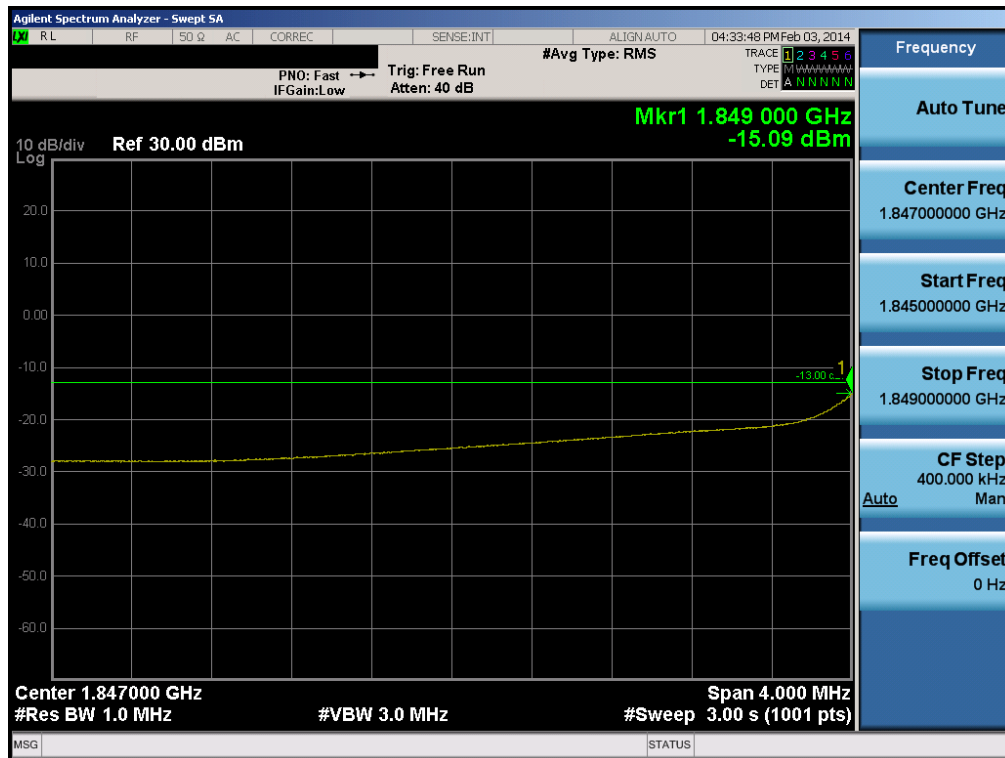
Plot 6-63. 4MHz Span Plot (PCS WCDMA Mode – Ch. 9262)
