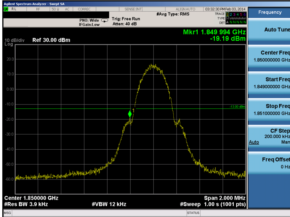
Plot 6-50. Band Edge Plot (PCS GSM Mode – Ch. 512)
