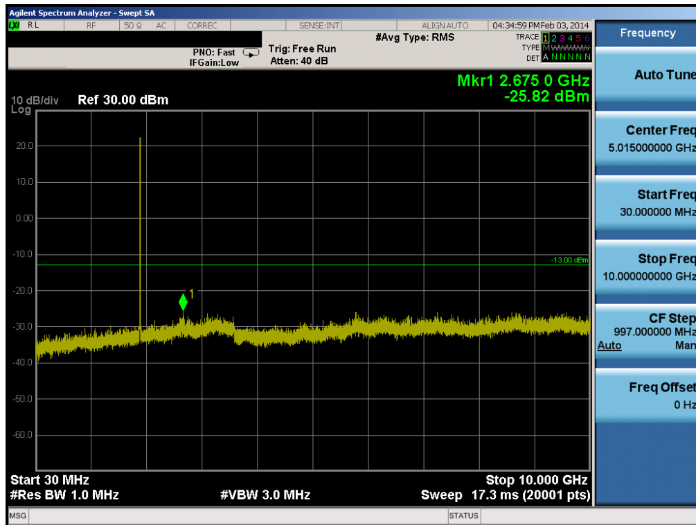
Plot 6-46. Conducted Spurious Plot (PCS WCDMA Mode – Ch. 9538)
