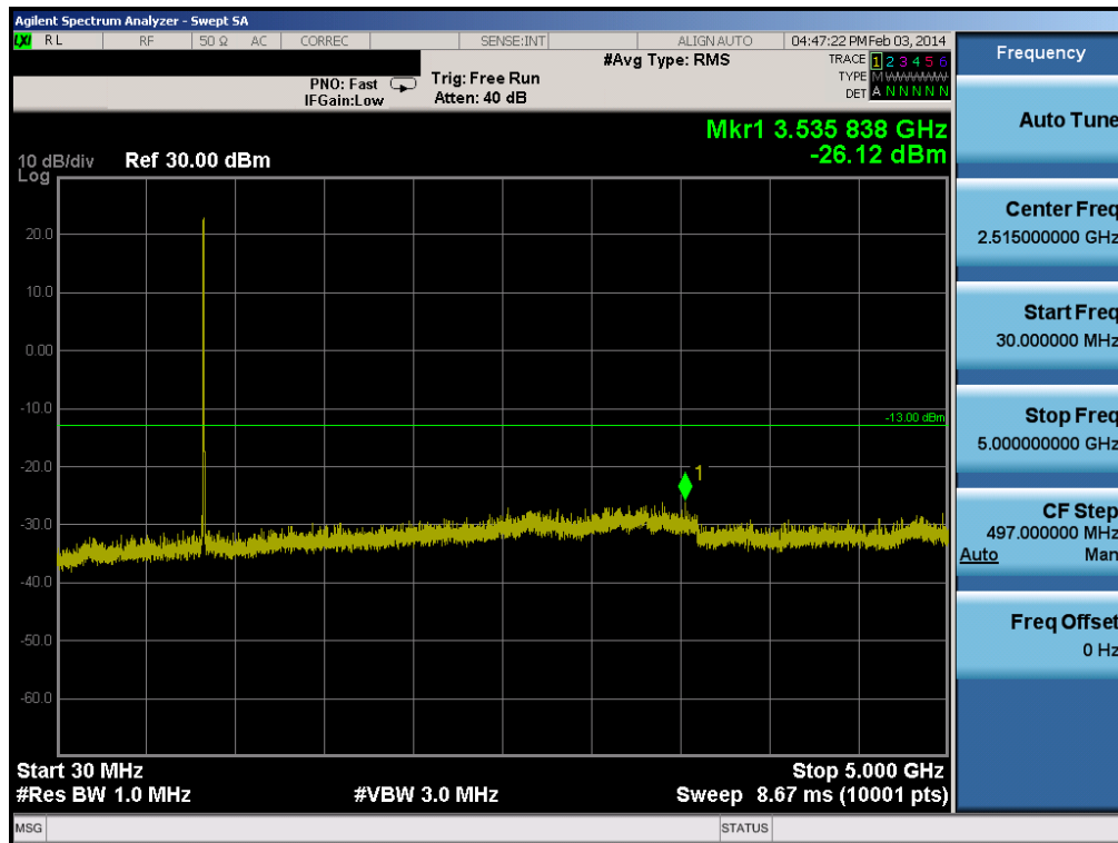
Plot 6-40. Conducted Spurious Plot (Cellular WCDMA Mode – Ch. 4233)
