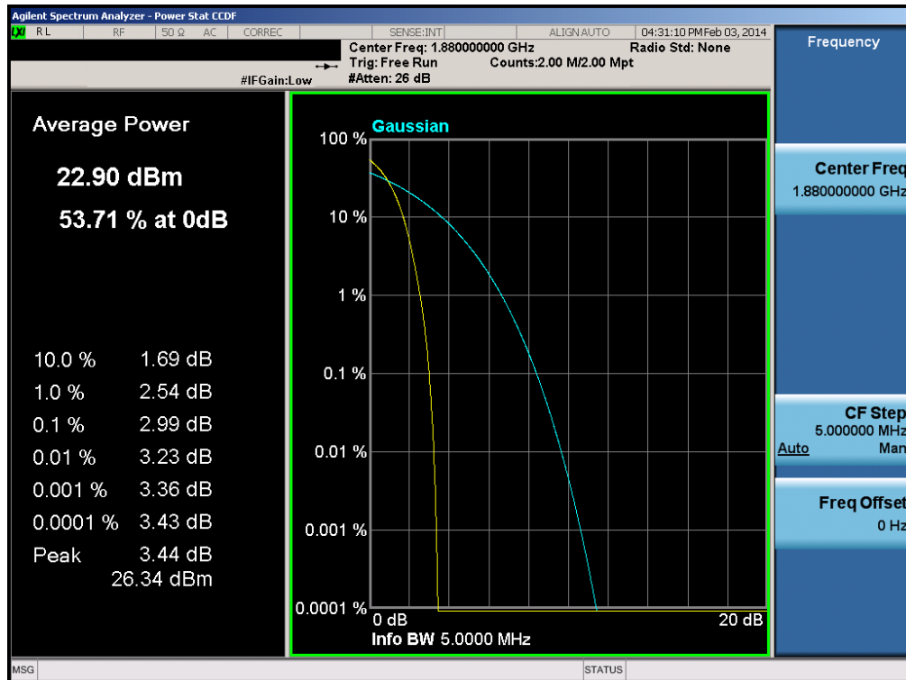
Plot 6-69. Peak-Average Ratio Plot (PCS WCDMA Mode – Ch. 9400)
