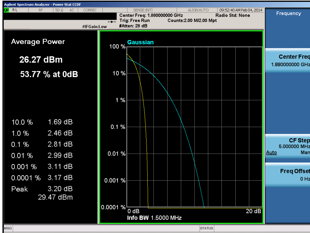
Plot 6-68. Peak-Average Ratio Plot (PCS CDMA Mode – Ch. 600)
