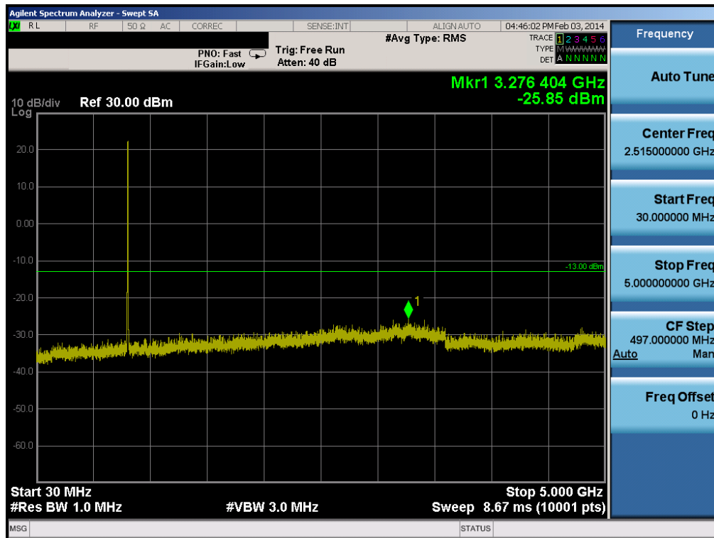
Plot 6-36. Conducted Spurious Plot (Cellular WCDMA Mode – Ch. 4132)
