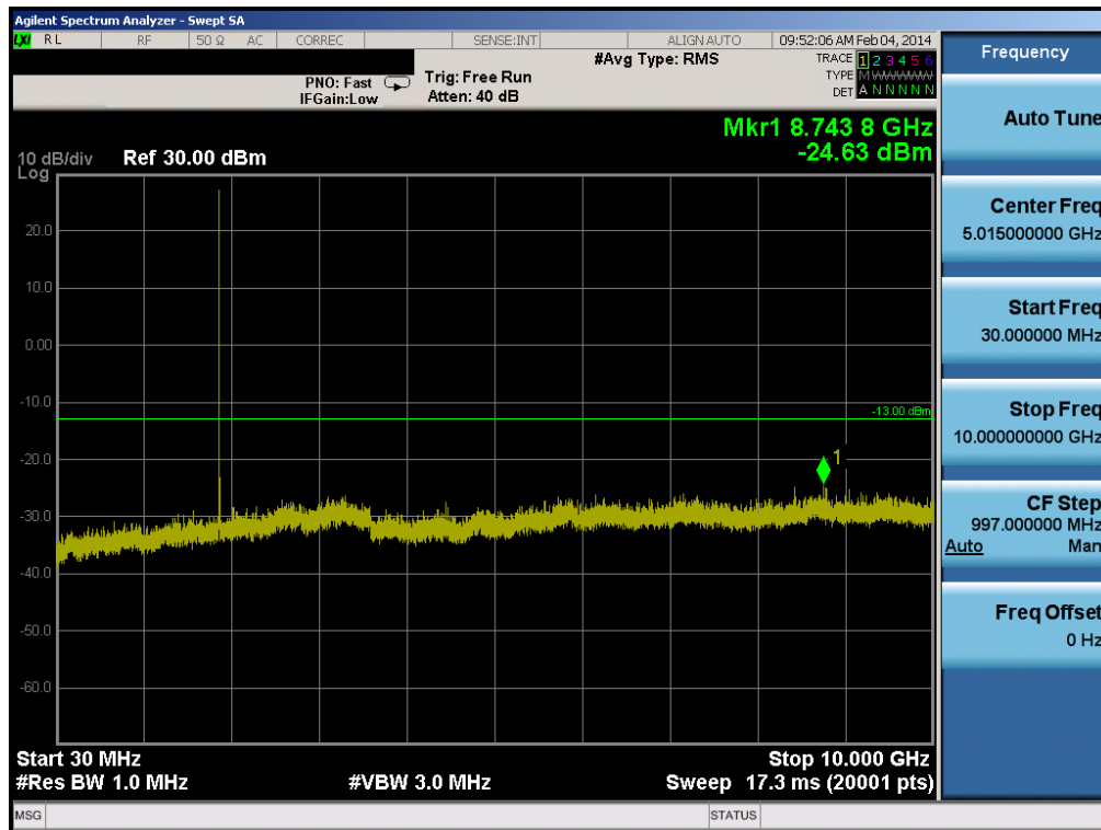
Plot 6-32. Conducted Spurious Plot (PCS CDMA Mode – Ch. 600)
