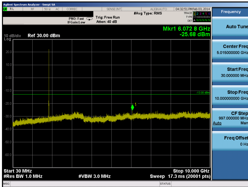
Plot 6-42. Conducted Spurious Plot (PCS WCDMA Mode – Ch. 9262)
