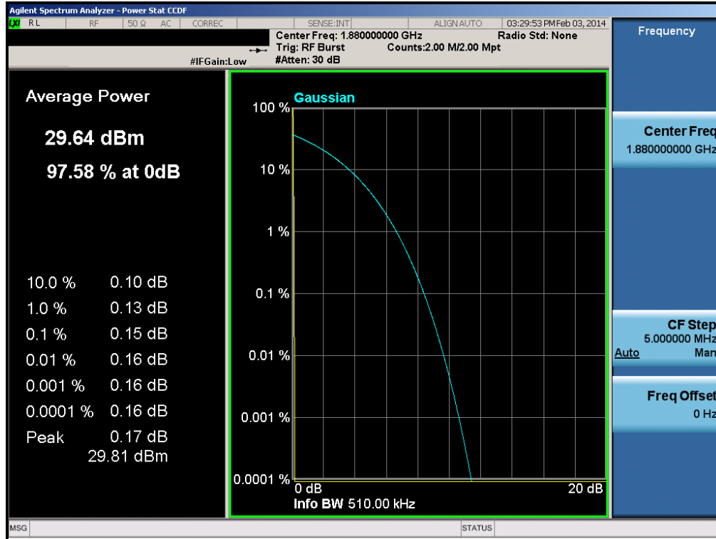
Plot 6-66. Peak-Average Ratio Plot (PCS GSM Mode – Ch. 661)
