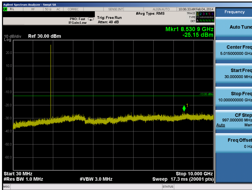
Plot 6-34. Conducted Spurious Plot (PCS CDMA Mode – Ch. 1175)
