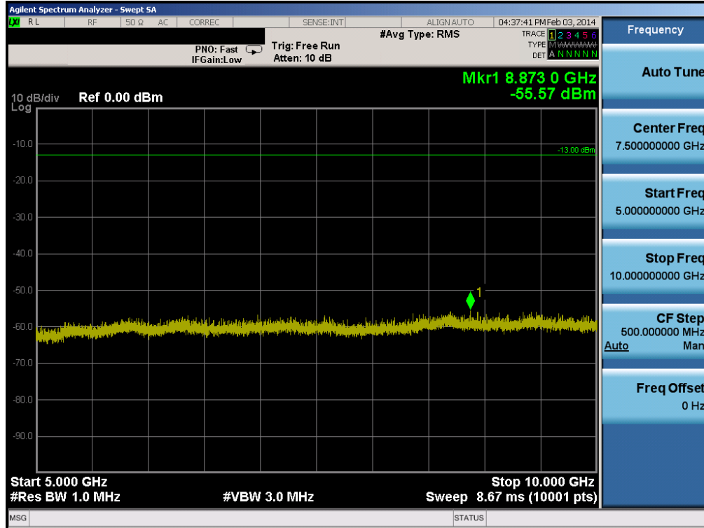
Plot 6-39. Conducted Spurious Plot (Cellular WCDMA Mode – Ch. 4183)
