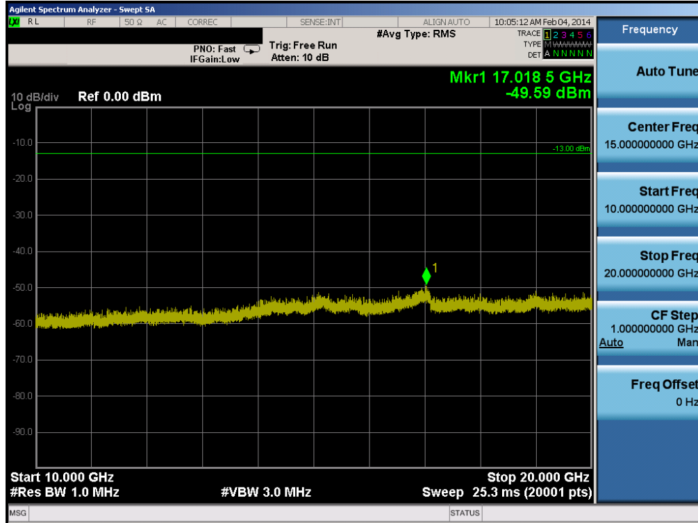
Plot 6-31. Conducted Spurious Plot (PCS CDMA Mode – Ch. 25)
