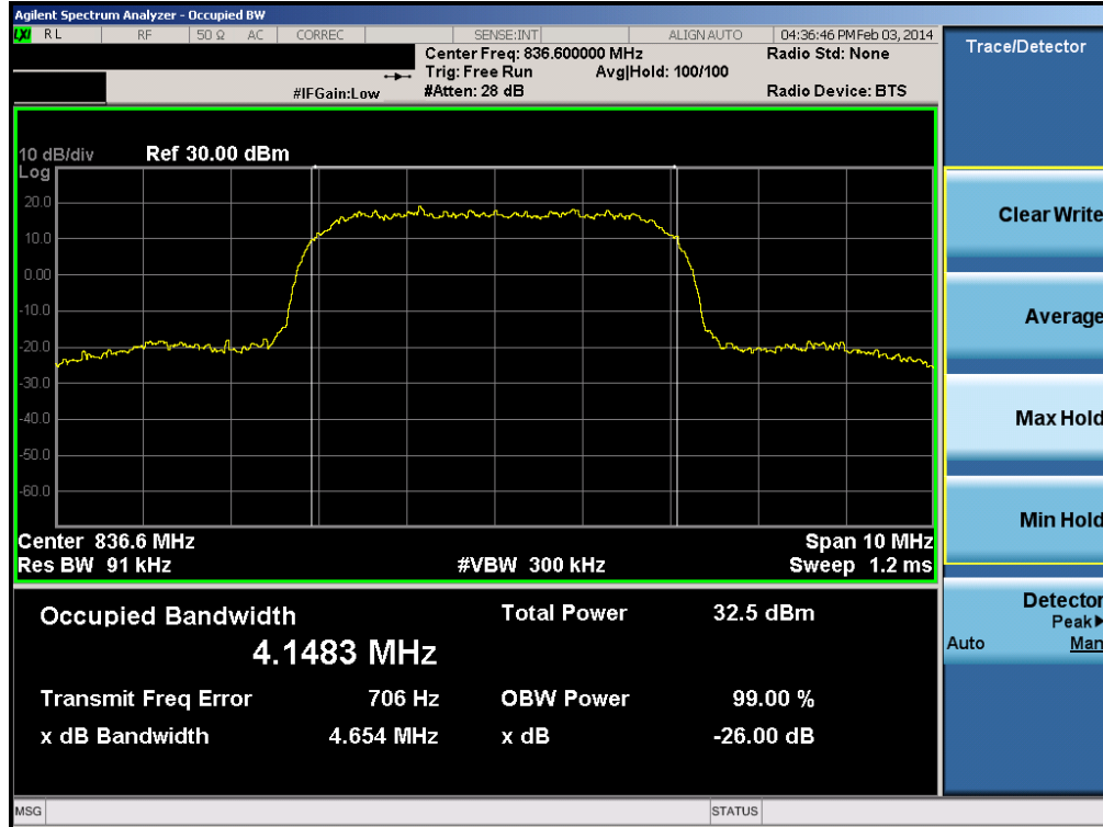
Plot 6-7. Occupied Bandwidth Plot (Cellular WCDMA Mode – Ch. 4183)
