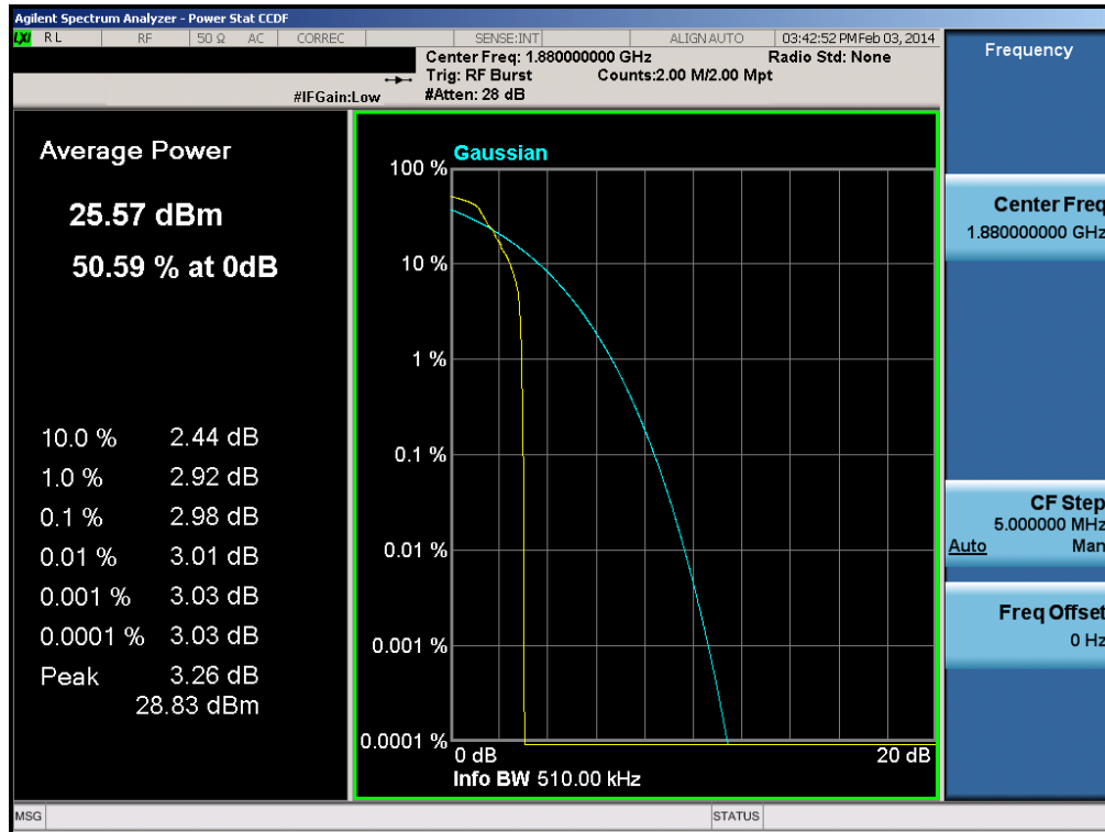
Plot 6-67. Peak-Average Ratio Plot (EDGE1900 Mode – Ch. 661)
