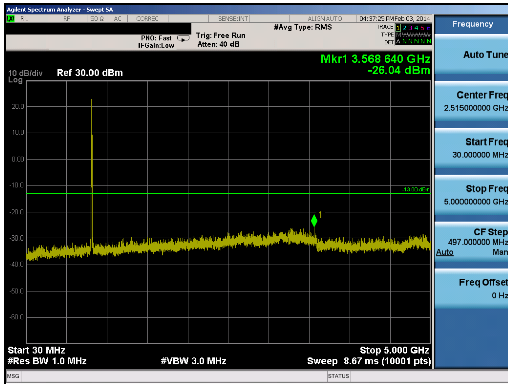
Plot 6-38. Conducted Spurious Plot (Cellular WCDMA Mode – Ch. 4183)
