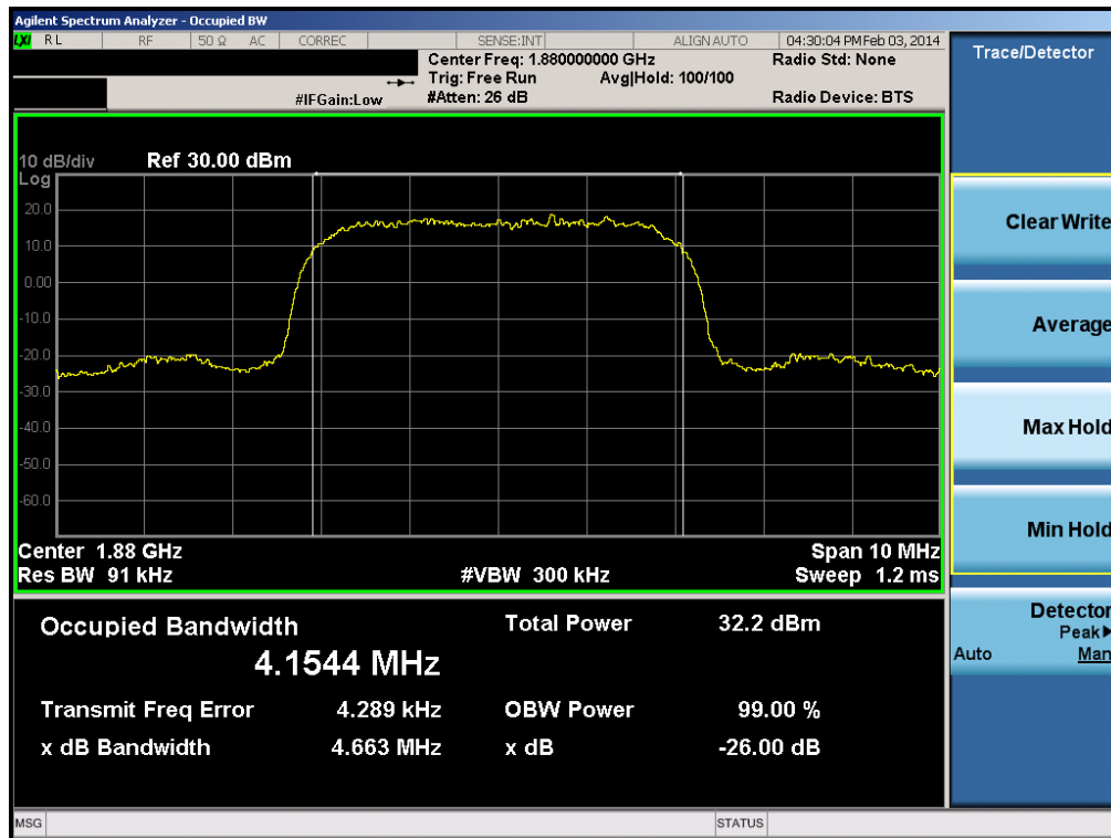
Plot 6-8. Occupied Bandwidth Plot (PCS WCDMA Mode – Ch. 9400)
