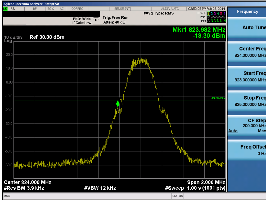
Plot 6-48. Band Edge Plot (Cellular GSM Mode – Ch. 128)
