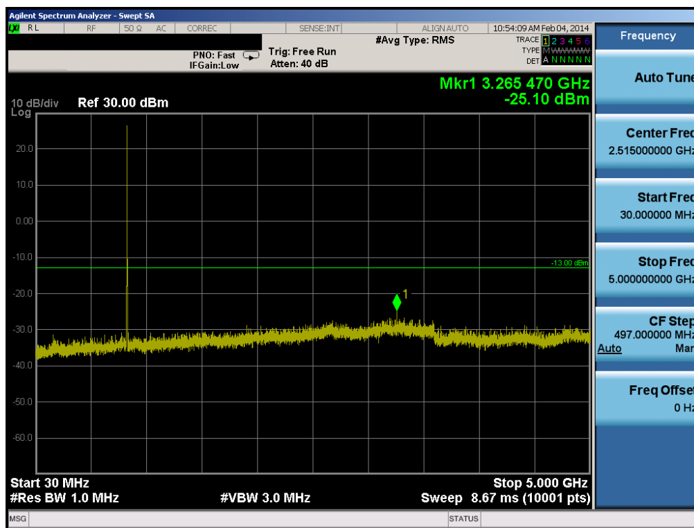
Plot 6-28. Conducted Spurious Plot (Cellular CDMA Mode – Ch. 777)
