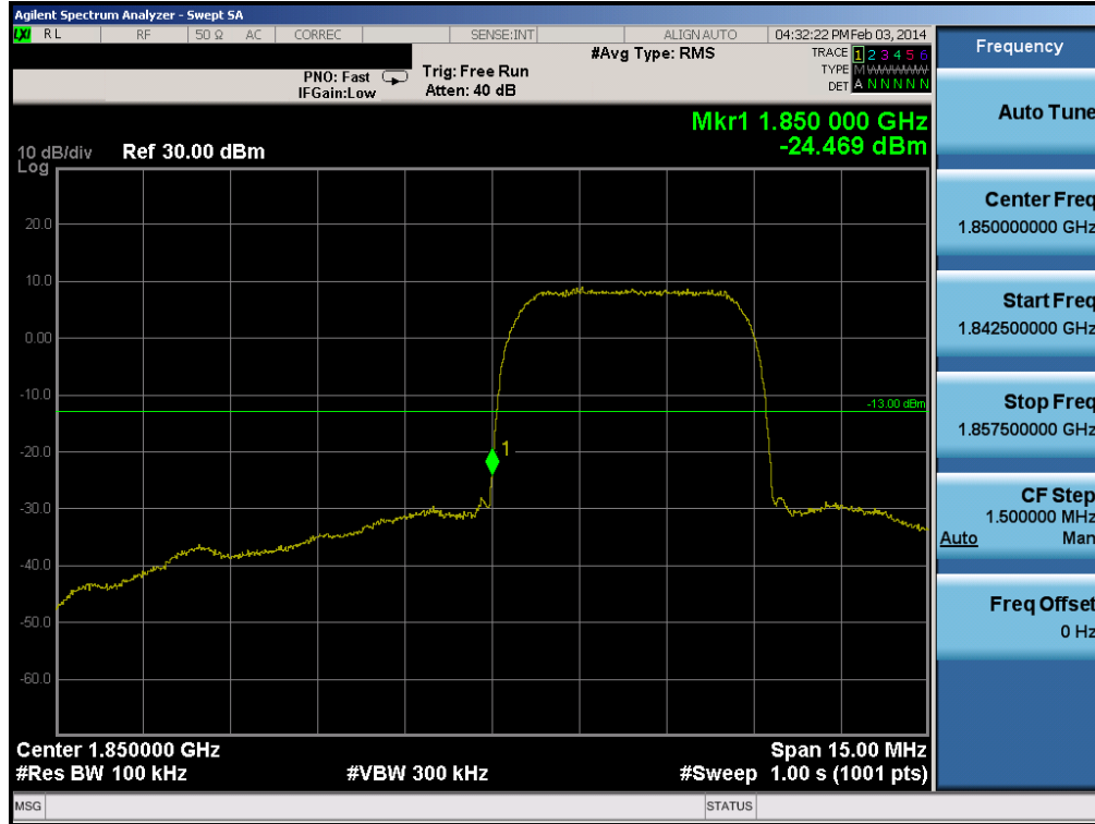
Plot 6-62. Band Edge Plot (PCS WCDMA Mode – Ch. 9262)
