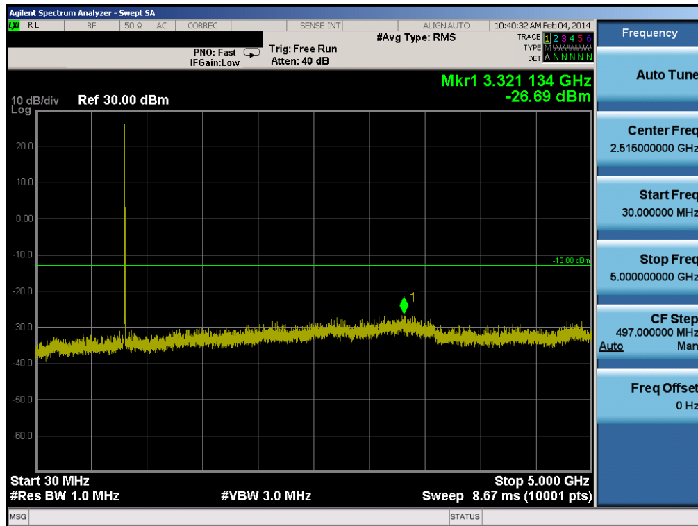
Plot 6-24. Conducted Spurious Plot (Cellular CDMA Mode – Ch. 1013)
