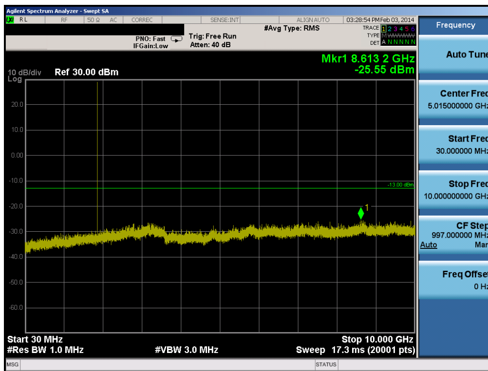
Plot 6-20. Conducted Spurious Plot (PCS GSM Mode – Ch. 661)
