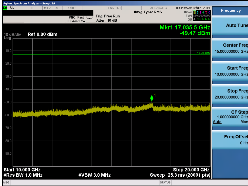
Plot 6-35. Conducted Spurious Plot (PCS CDMA Mode – Ch. 1175)
