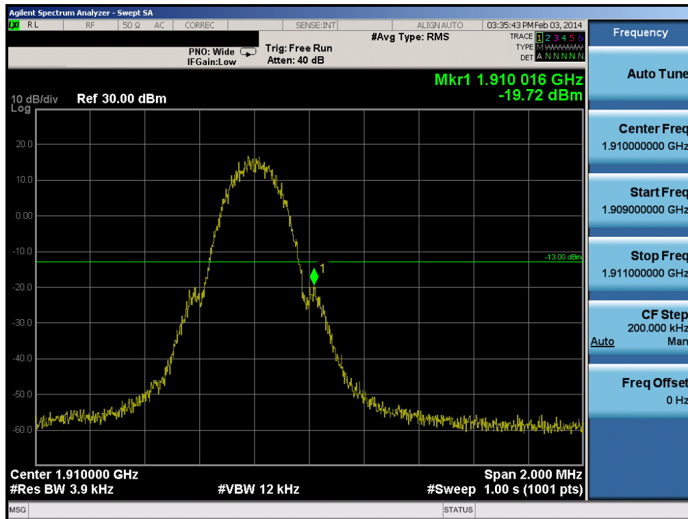
Plot 6-51. Band Edge Plot (PCS GSM Mode – Ch. 810)
