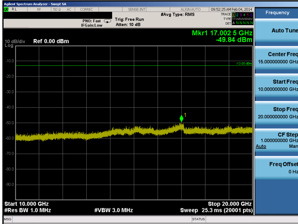
Plot 6-33. Conducted Spurious Plot (PCS CDMA Mode – Ch. 600)
