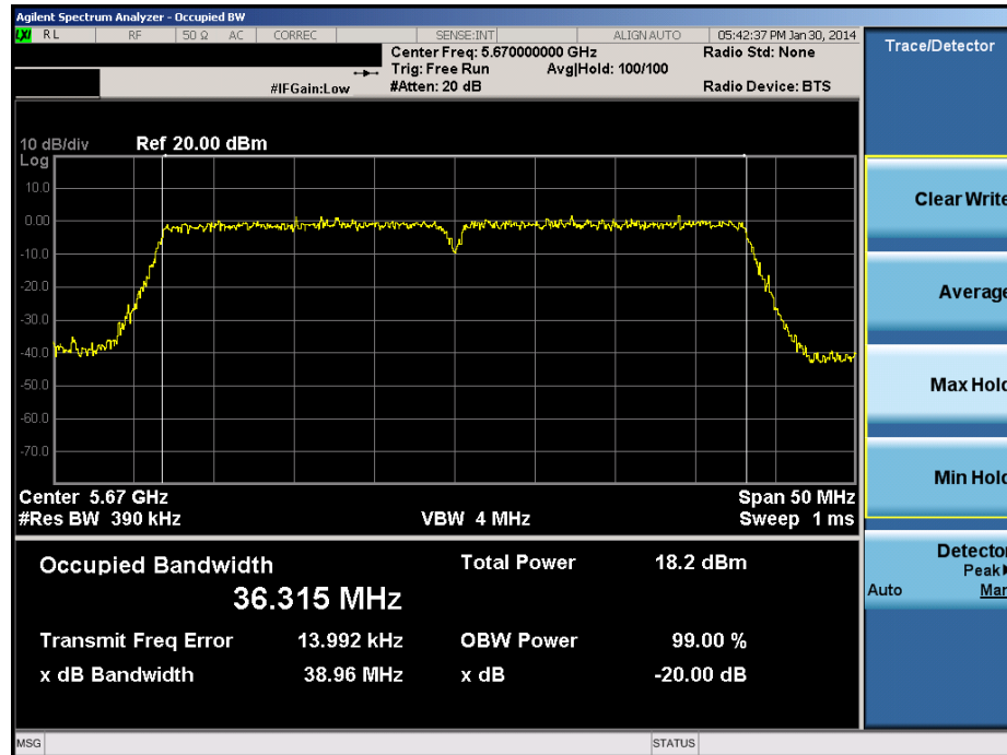
Plot 6-63. 20dB Bandwidth Plot (40MHz BW 802.11n (UNII Band 2C) – Ch. 134)
