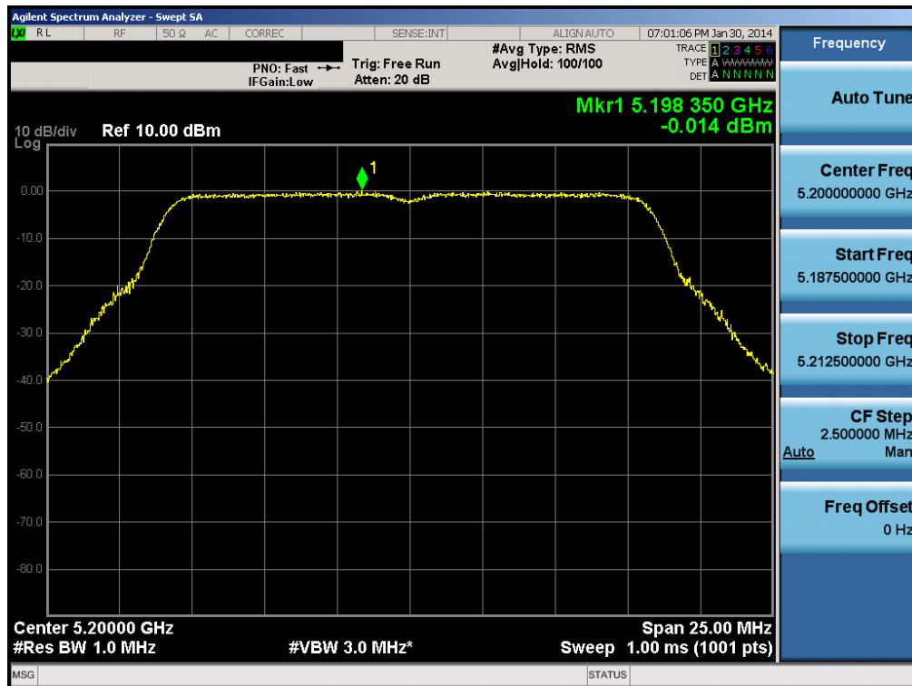
Plot 6-66. Peak Power Spectral Density Plot (802.11a (UNII Band 1) – Ch. 40)
