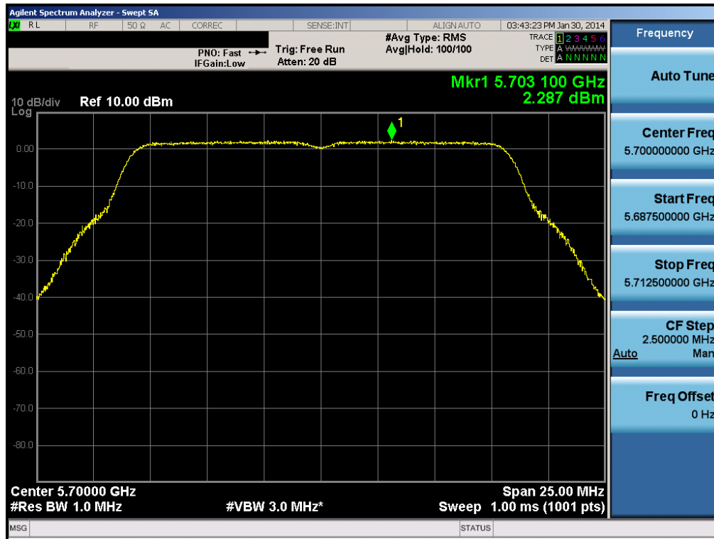
Plot 6-85. Peak Power Spectral Density Plot (802.11a (UNII Band 2C) – Ch. 140)
