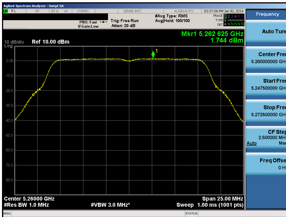
Plot 6-74. Peak Power Spectral Density Plot (802.11a (UNII Band 2A) – Ch. 52)
