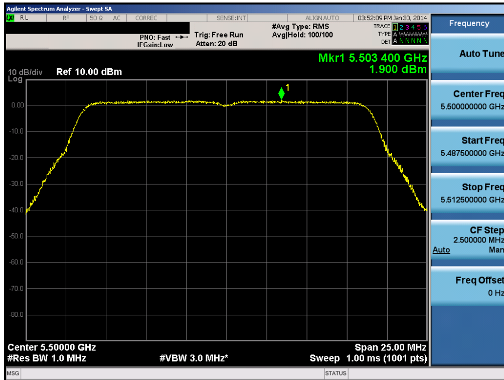
Plot 6-86. Peak Power Spectral Density Plot (20MHz BW 802.11n (UNII Band 2C) – Ch. 100)
