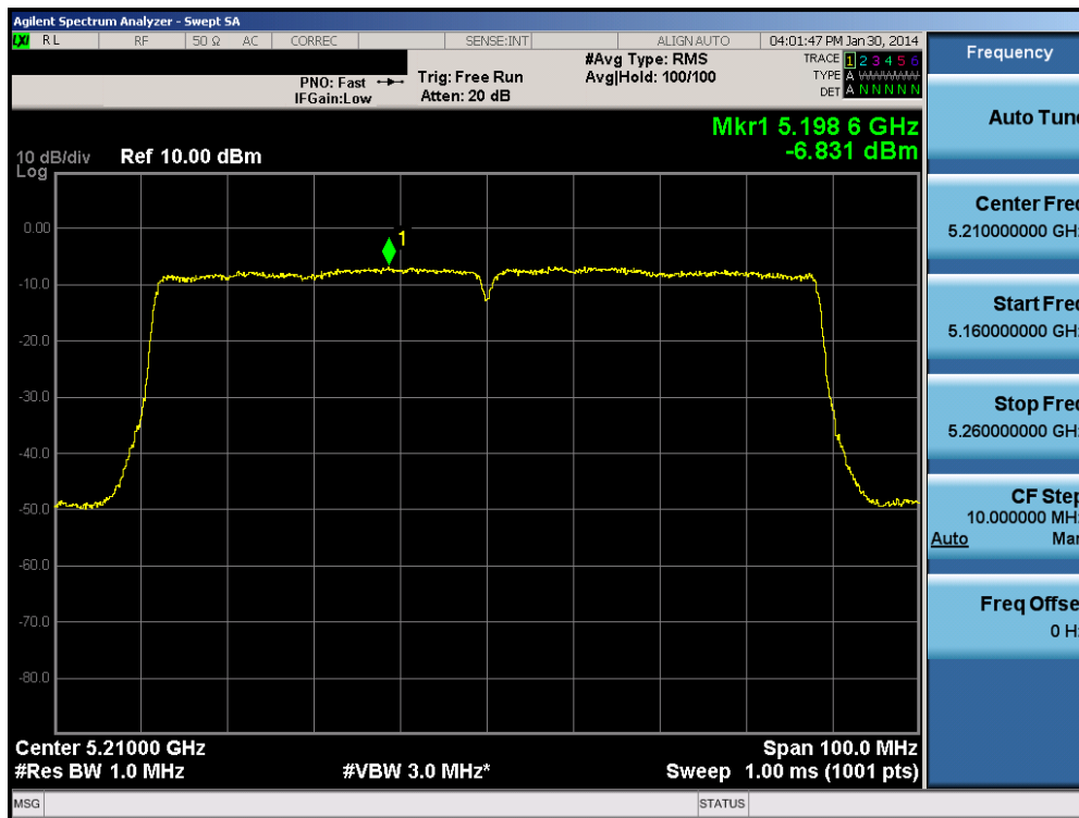
Plot 6-73. Peak Power Spectral Density Plot (80MHz BW 802.11ac (UNII Band 1) – Ch. 42)
