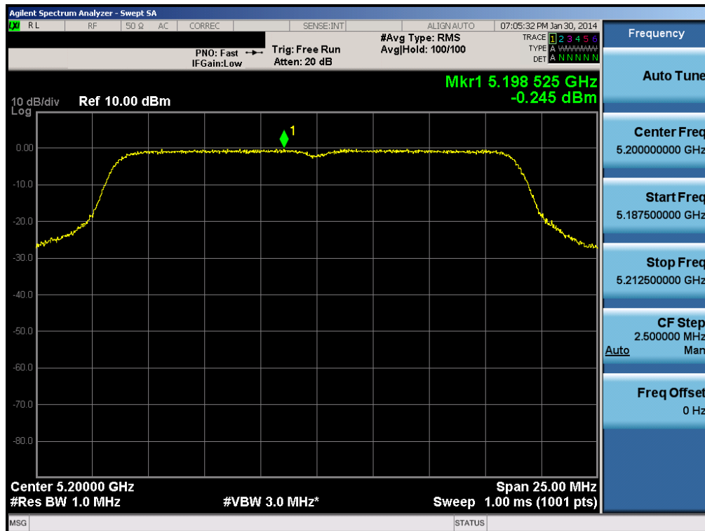
Plot 6-69. Peak Power Spectral Density Plot (20MHz BW 802.11n (UNII Band 1) – Ch. 40)
