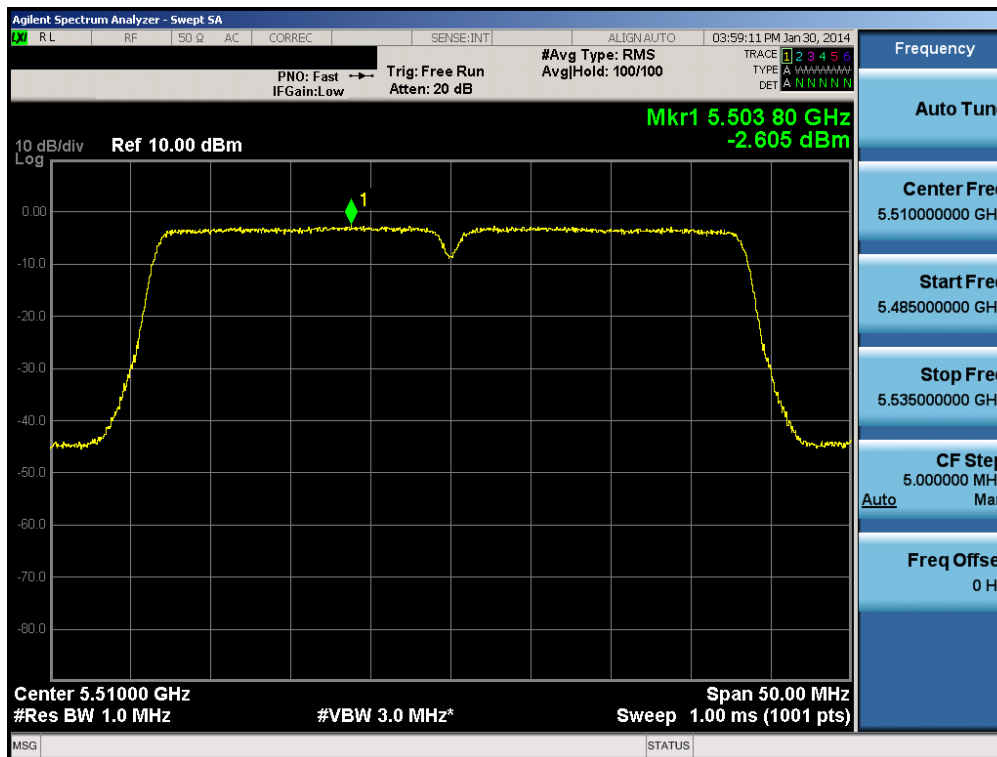
Plot 6-89. Peak Power Spectral Density Plot (40MHz BW 802.11n (UNII Band 2C) – Ch. 102)
