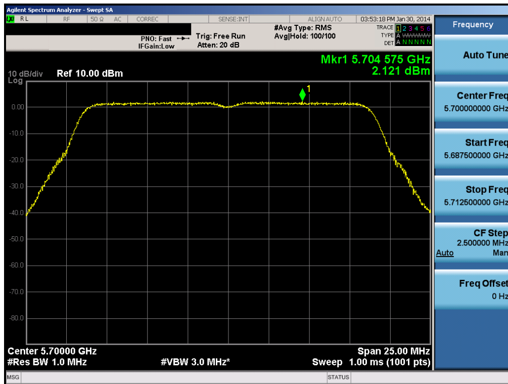
Plot 6-88. Peak Power Spectral Density Plot (20MHz BW 802.11n (UNII Band 2C) – Ch. 140)
