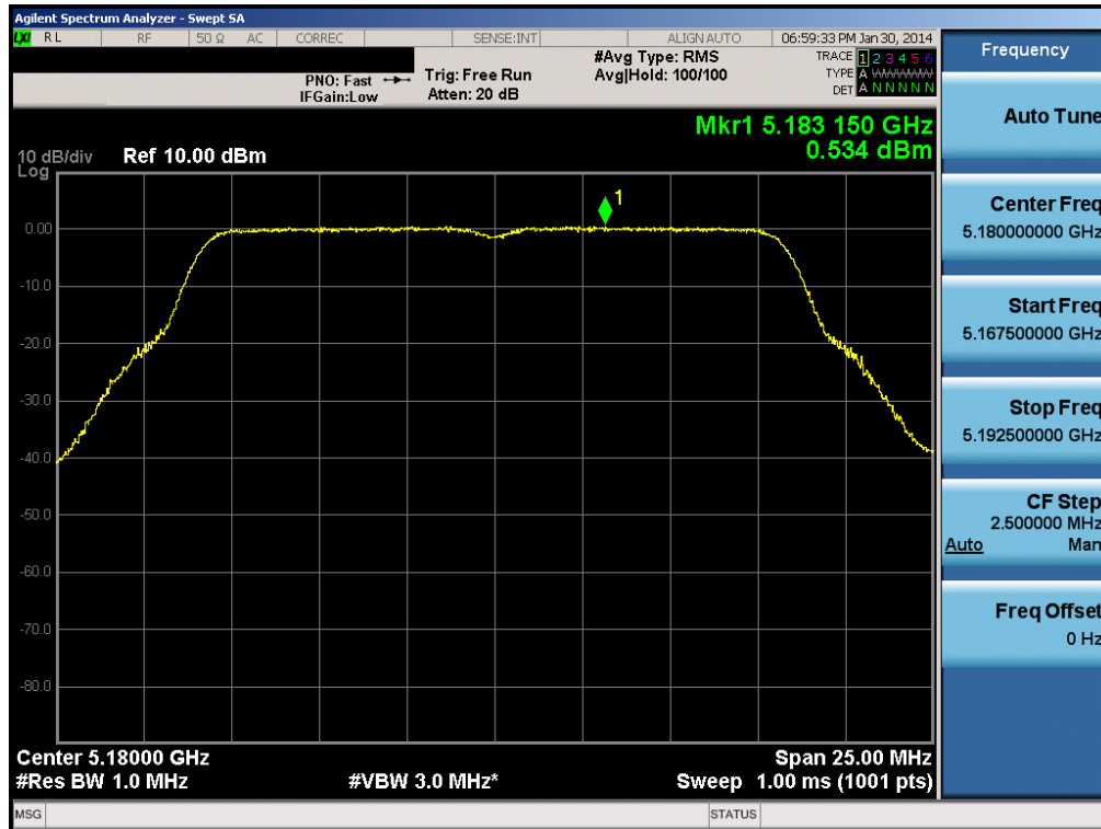
Plot 6-65. Peak Power Spectral Density Plot (802.11a (UNII Band 1) – Ch. 36)
