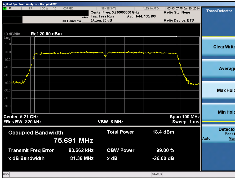
Plot 6-41. 26dB Bandwidth Plot (80MHz BW 802.11ac (UNII Band 1) – Ch. 42)
