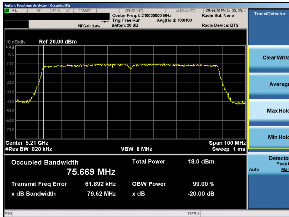
Plot 6-64. 20dB Bandwidth Plot (80MHz BW 802.11ac (UNII Band 1) – Ch. 42)
