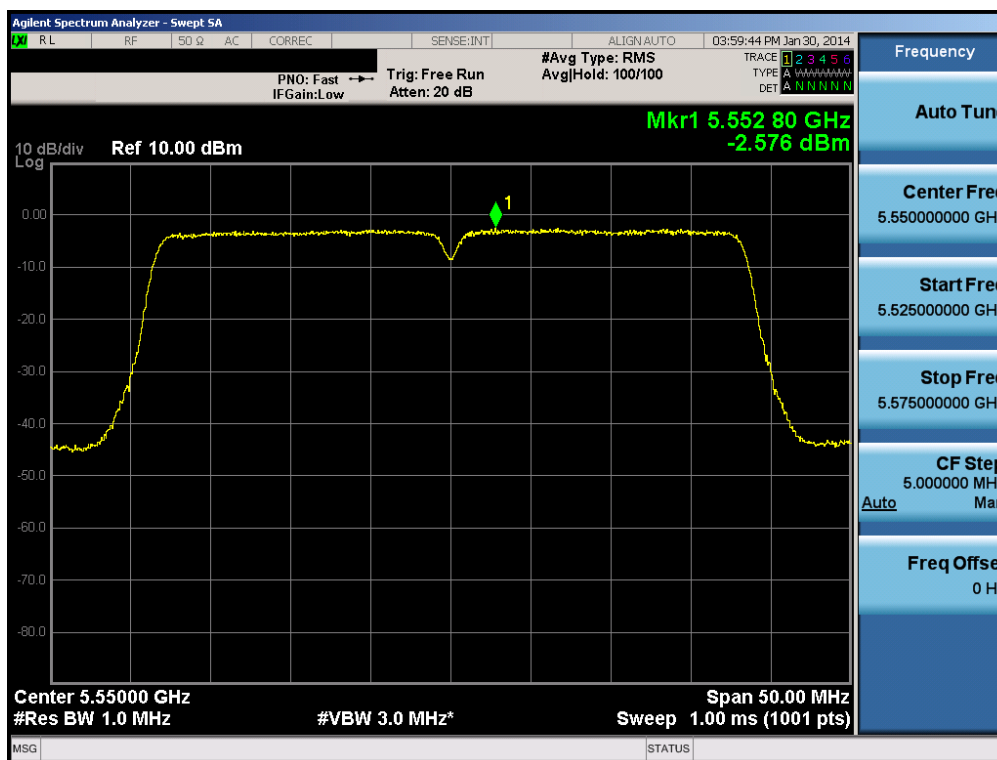
Plot 6-90. Peak Power Spectral Density Plot (40MHz BW 802.11n (UNII Band 2C) – Ch. 110)
