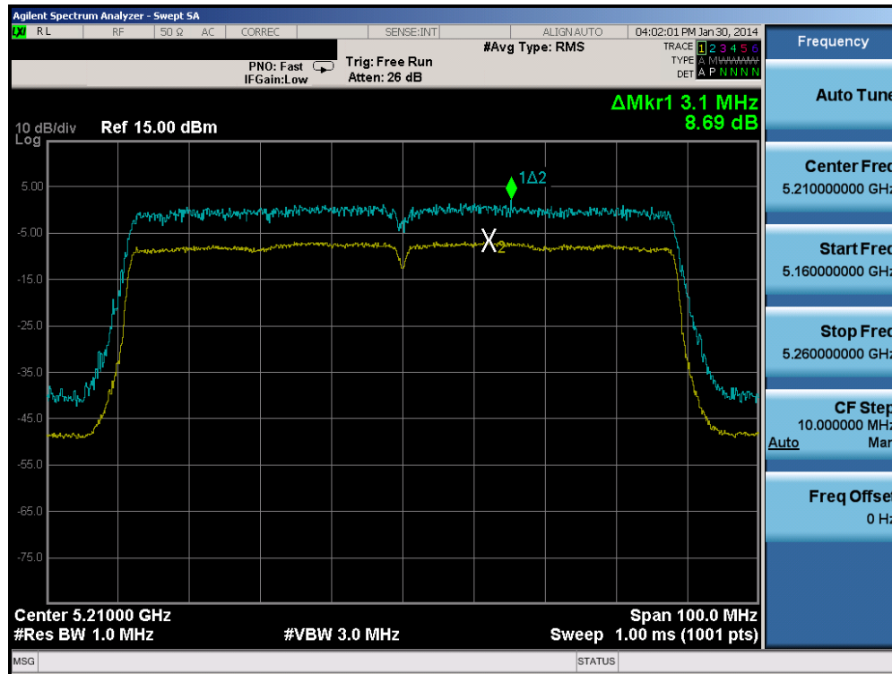
Plot 6-129. Peak Excursion Ratio Plot (80MHz BW 802.11ac (UNII Band 1) – Ch. 42)
