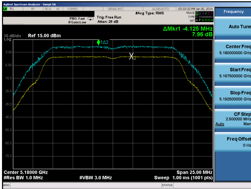
Plot 6-121. Peak Excursion Ratio Plot (802.11a (UNII Band 1) – Ch. 36)
