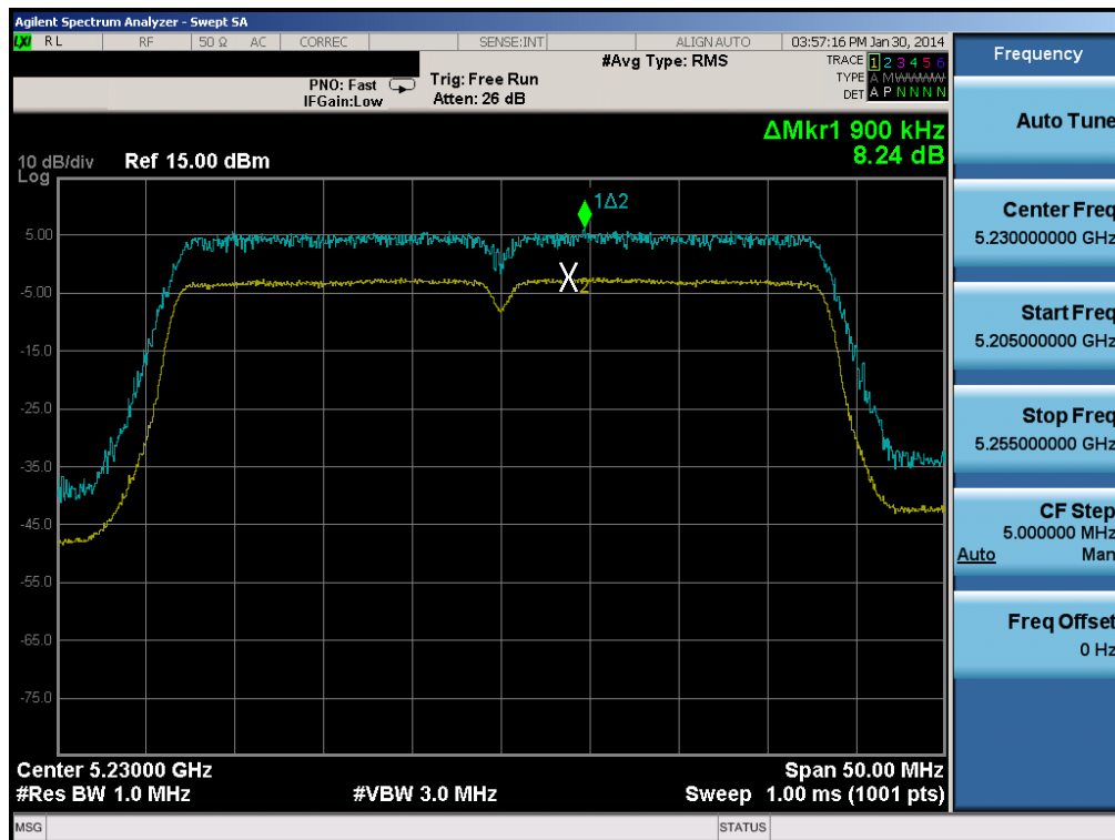
Plot 6-128. Peak Excursion Ratio Plot (40MHz BW 802.11n (UNII Band 1) – Ch. 46)
