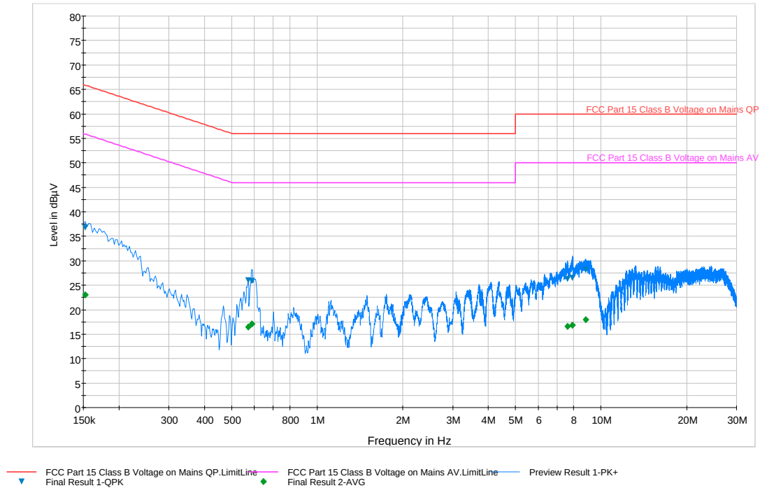
Plot 6-243. Line Conducted Plot with 802.11a UNII Band 1 (N)
