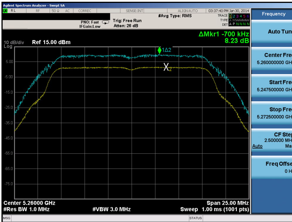
Plot 6-130. Peak Excursion Ratio Plot (802.11a (UNII Band 2A) – Ch. 52)
