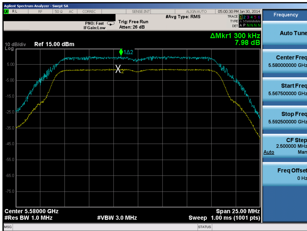
Plot 6-168. Peak Excursion Ratio Plot (802.11a (UNII Band 2C) – Ch. 116)
