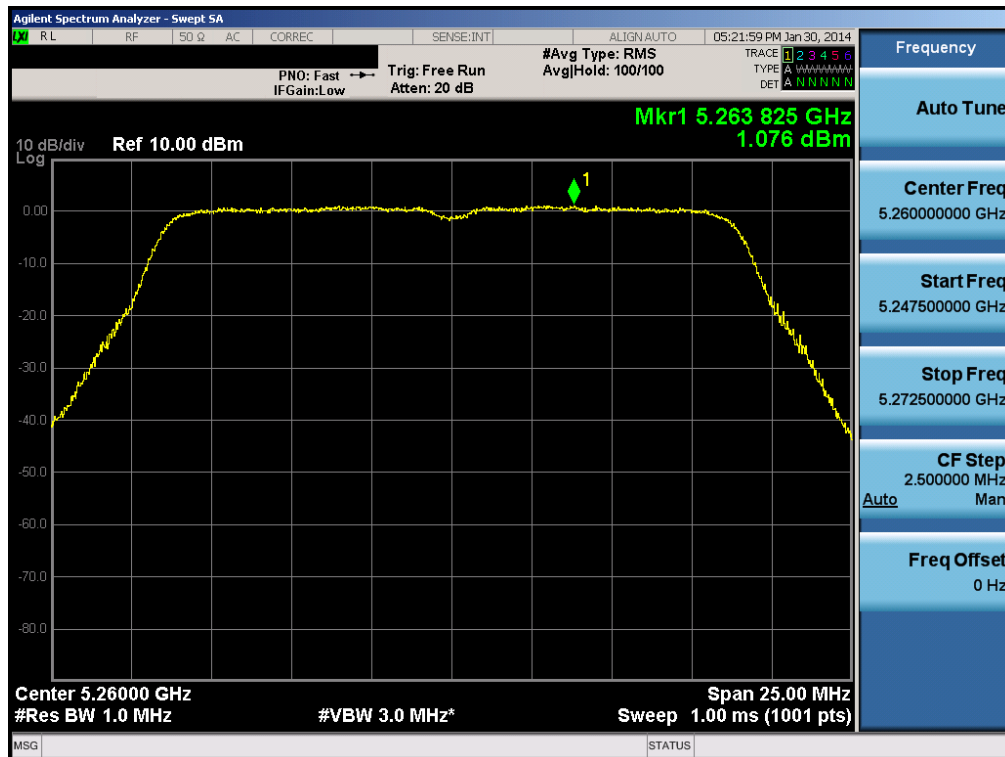
Plot 6-105. Peak Power Spectral Density Plot (20MHz BW 802.11n (UNII Band 2A) – Ch. 52)
