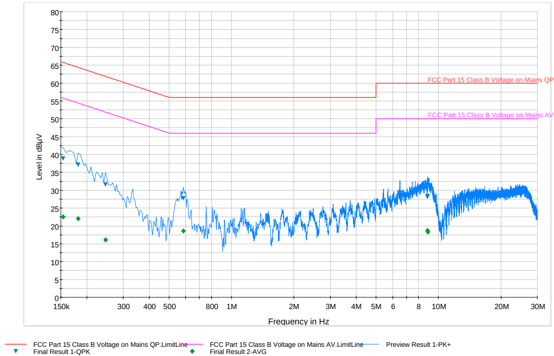
Plot 6-247. Line Conducted Plot with 802.11a UNII Band 2C (N)
