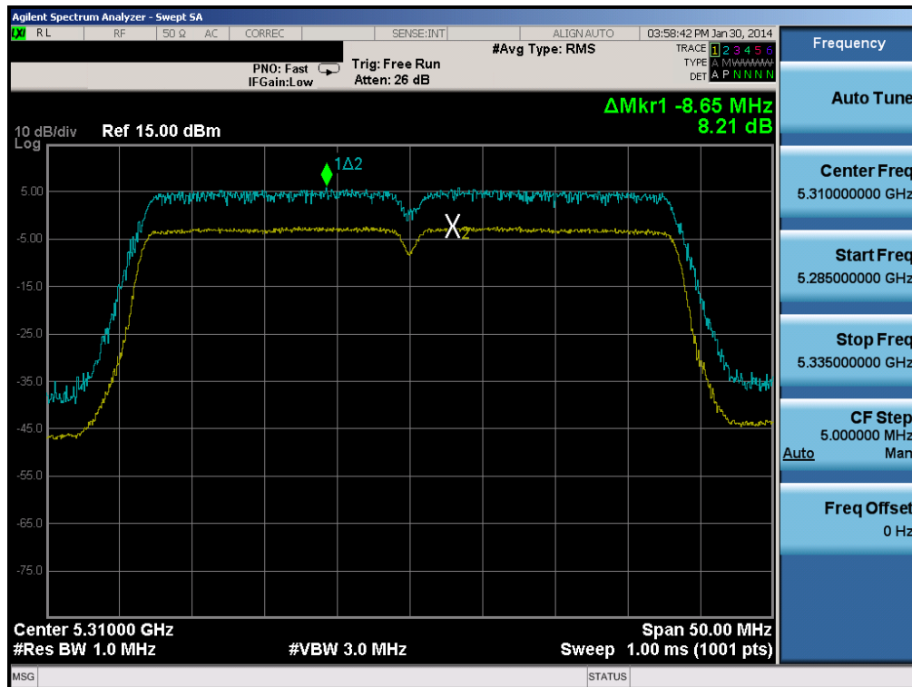
Plot 6-137. Peak Excursion Ratio Plot (40MHz BW 802.11n (UNII Band 2A) – Ch. 62)
