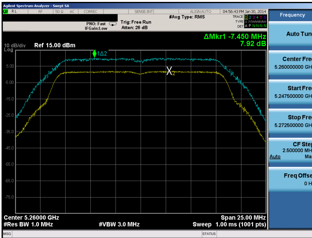
Plot 6-158. Peak Excursion Ratio Plot (802.11a (UNII Band 2A) – Ch. 52)
