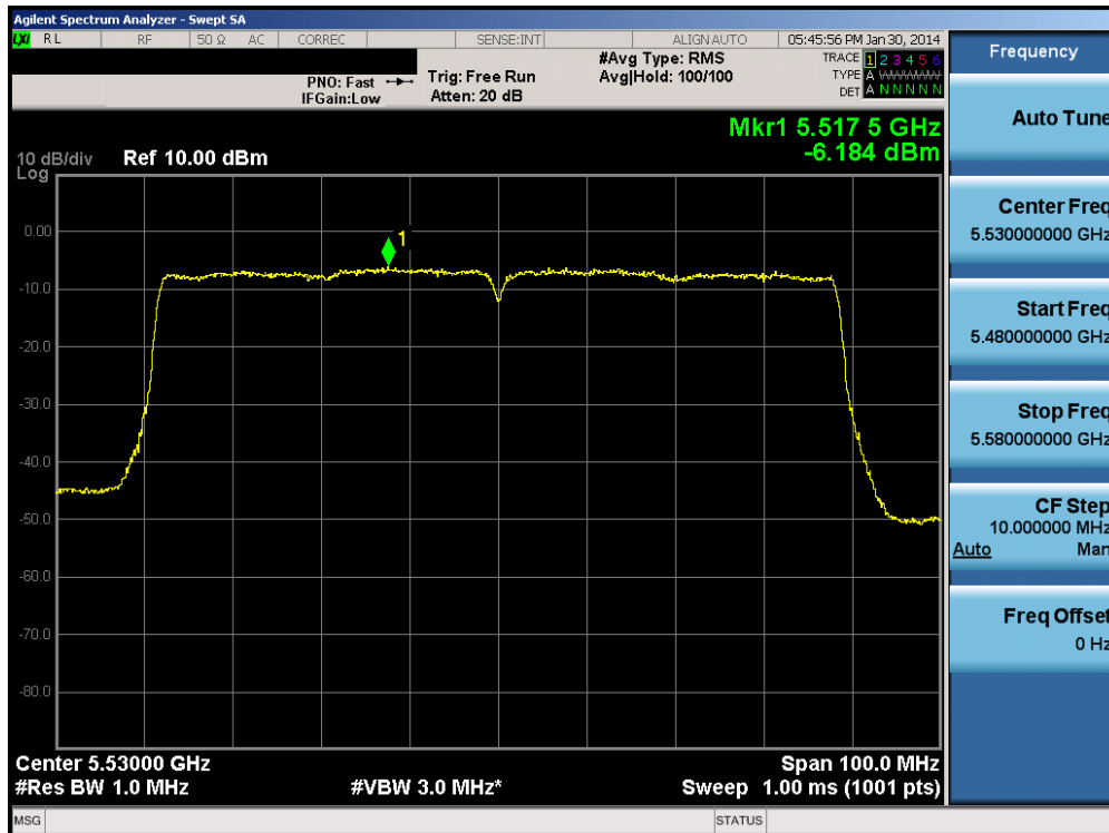
Plot 6-120. Peak Power Spectral Density Plot (80MHz BW 802.11ac (UNII Band 2C) – Ch. 106)
