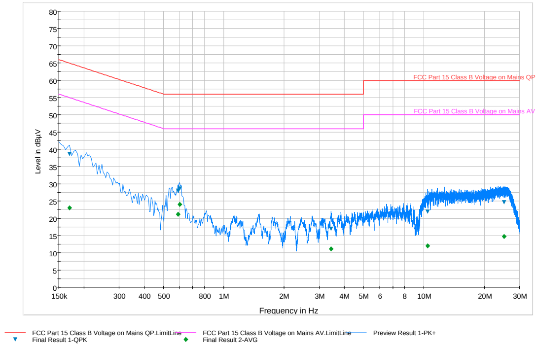
Plot 6-246. Line Conducted Plot with 802.11a UNII Band 2C (L1)
