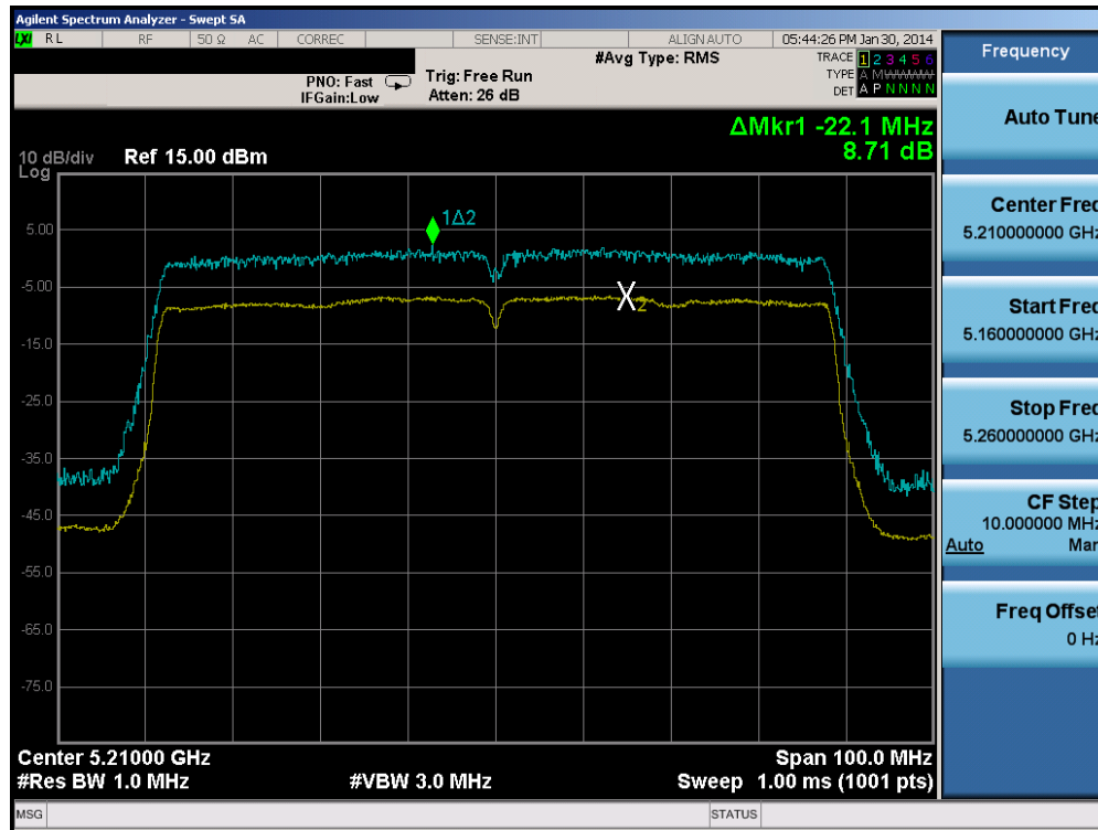
Plot 6-157. Peak Excursion Ratio Plot (80MHz BW 802.11ac (UNII Band 1) – Ch. 42)
