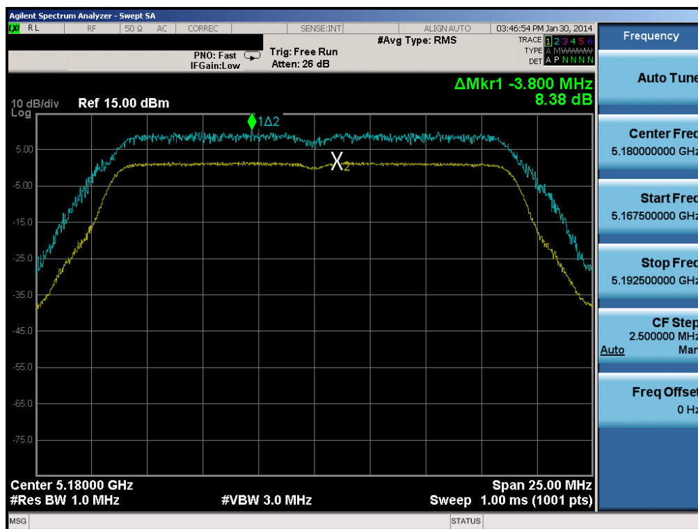
Plot 6-124. Peak Excursion Ratio Plot (20MHz BW 802.11n (UNII Band 1) – Ch. 36)
