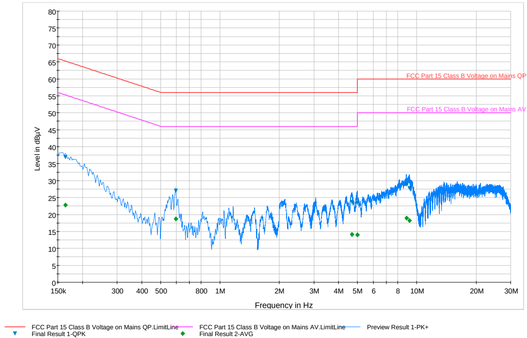
Plot 6-245. Line Conducted Plot with 802.11a UNII Band 2A (N)
