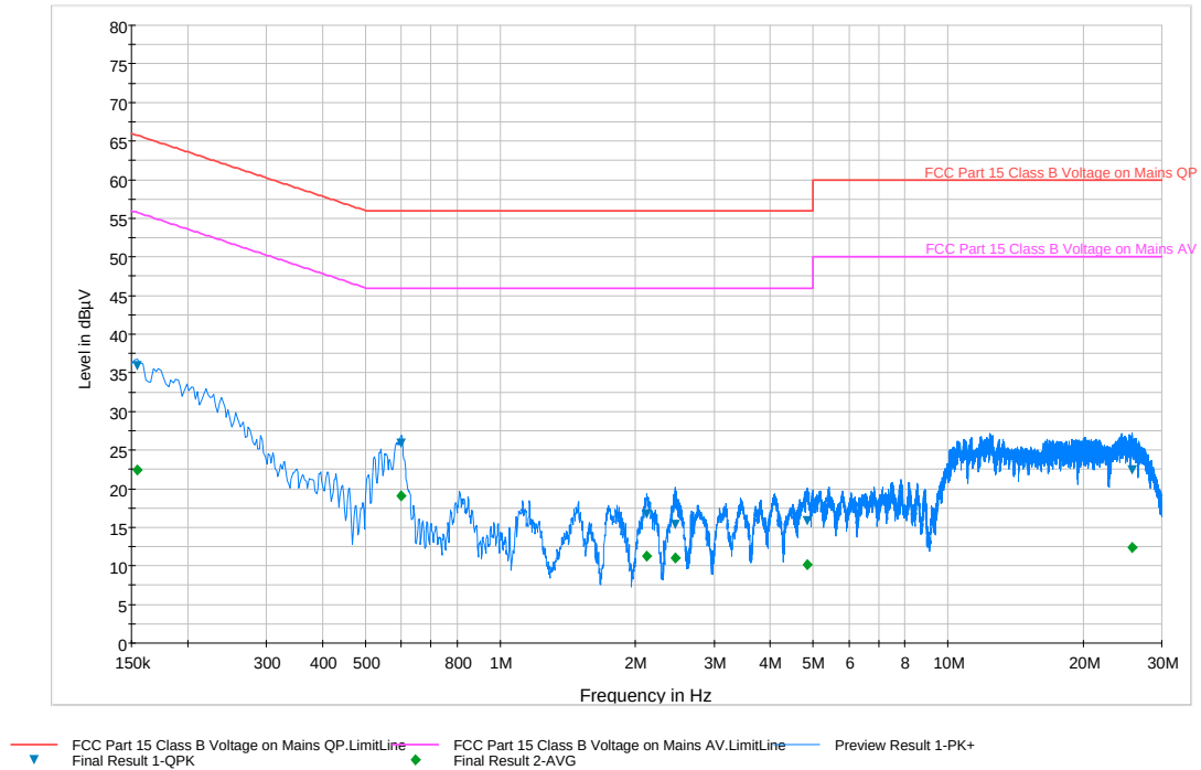
Plot 6-242. Line Conducted Plot with 802.11a UNII Band 1 (L1)
