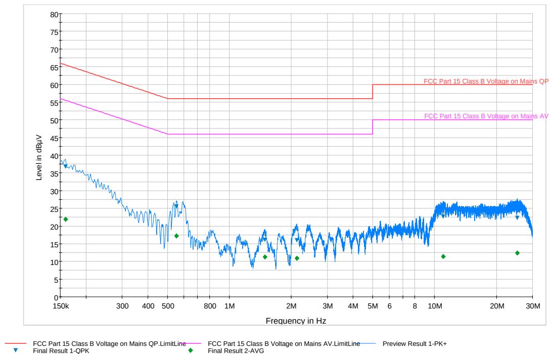
Plot 6-244. Line Conducted Plot with 802.11a UNII Band 2A (L1)
