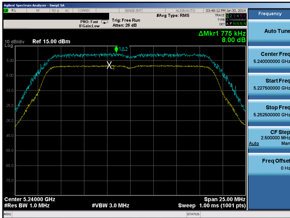
Plot 6-126. Peak Excursion Ratio Plot (20MHz BW 802.11n (UNII Band 1) – Ch. 48)
