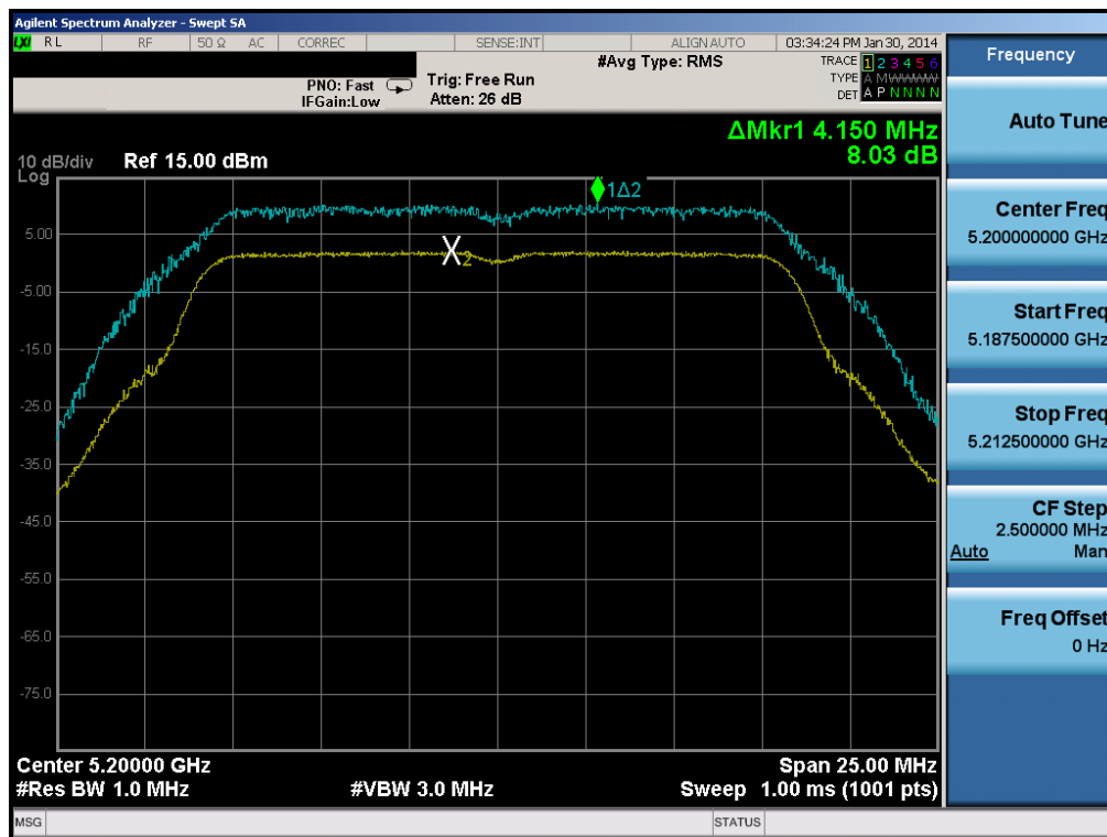
Plot 6-122. Peak Excursion Ratio Plot (802.11a (UNII Band 1) – Ch. 40)
