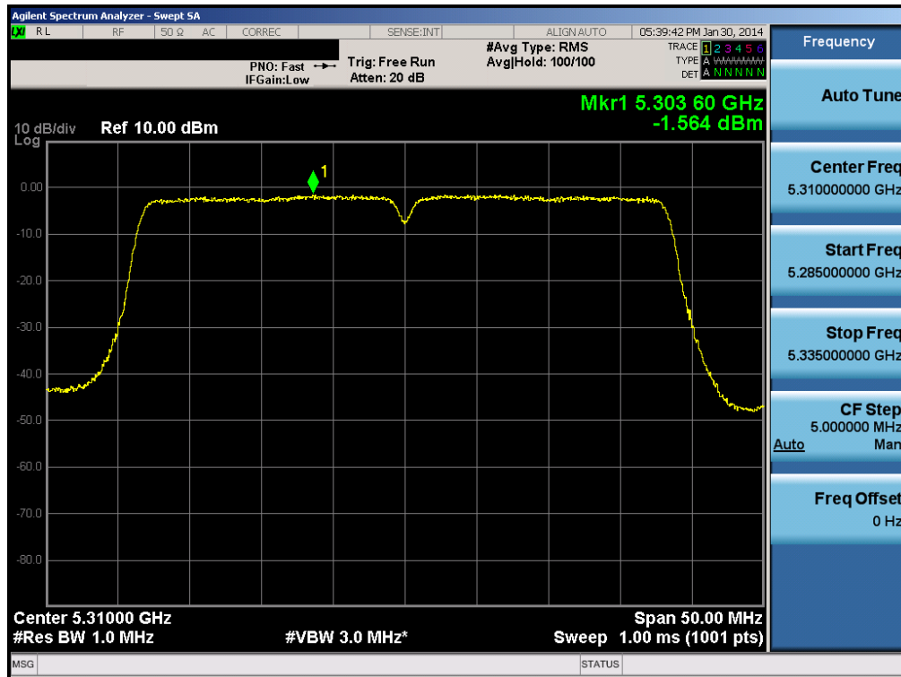
Plot 6-109. Peak Power Spectral Density Plot (40MHz BW 802.11n (UNII Band 2A) – Ch. 62)
