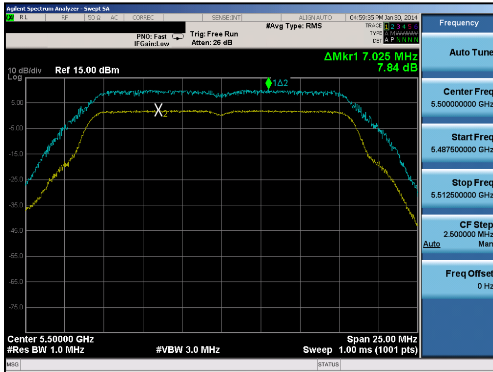
Plot 6-167. Peak Excursion Ratio Plot (802.11a (UNII Band 2C) – Ch. 100)
