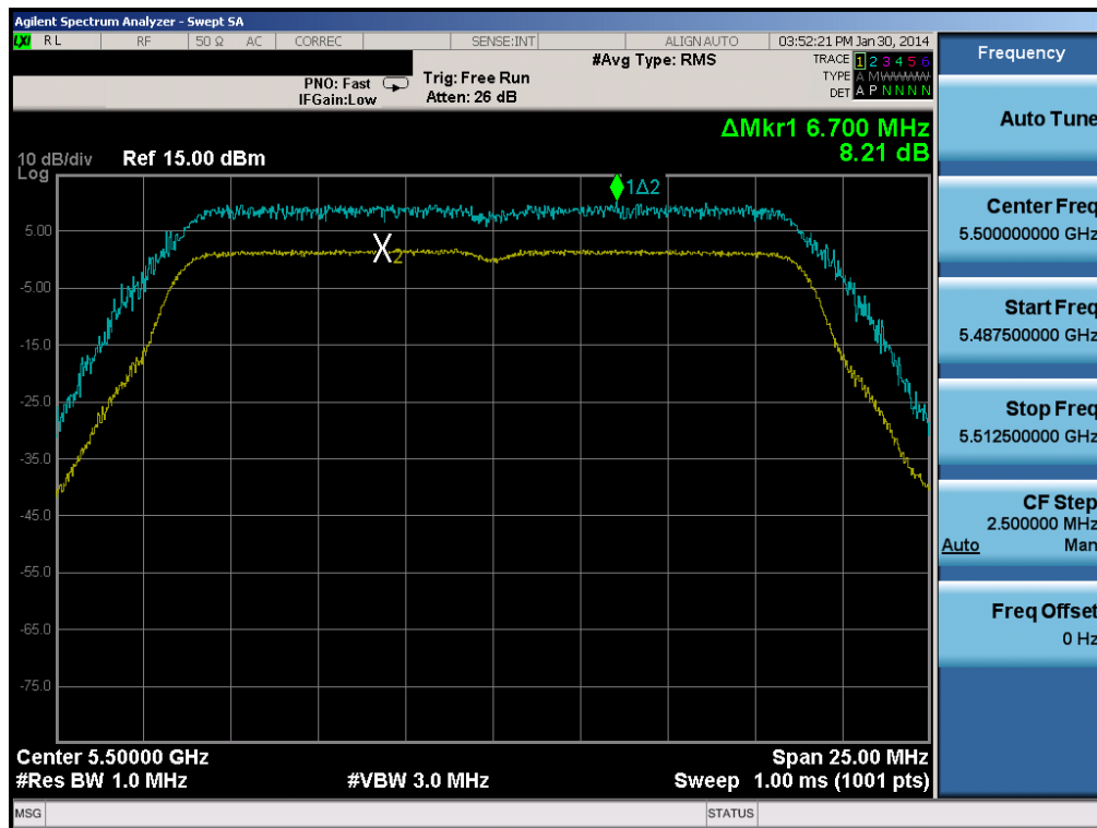
Plot 6-142. Peak Excursion Ratio Plot (20MHz BW 802.11n (UNII Band 2C) – Ch. 100)
