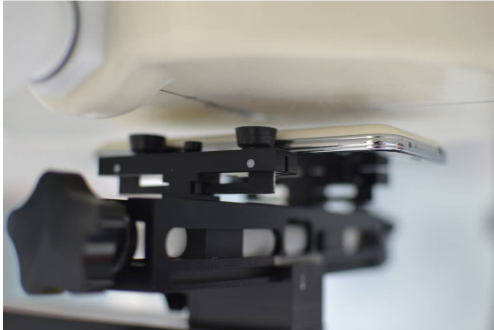
SAR Test Setup Photo 11 – Back Side at 1.0 cm with Wireless Charging Cover
