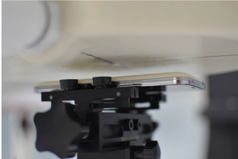
SAR Test Setup Photo 9 – Back Side at 1.5 cm with Wireless Charging Cover
