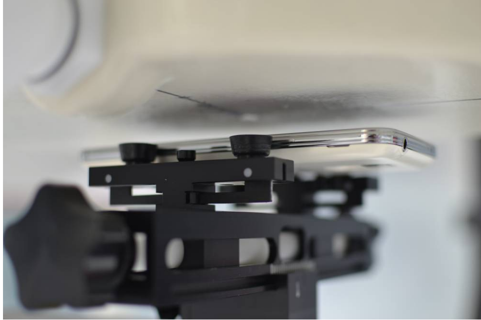
SAR Test Setup Photo 13 – Front Side at 1.0 cm with Wireless Charging Cover
