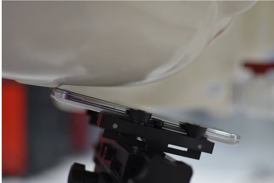
SAR Test Setup Photo 3 – Right Tilt
