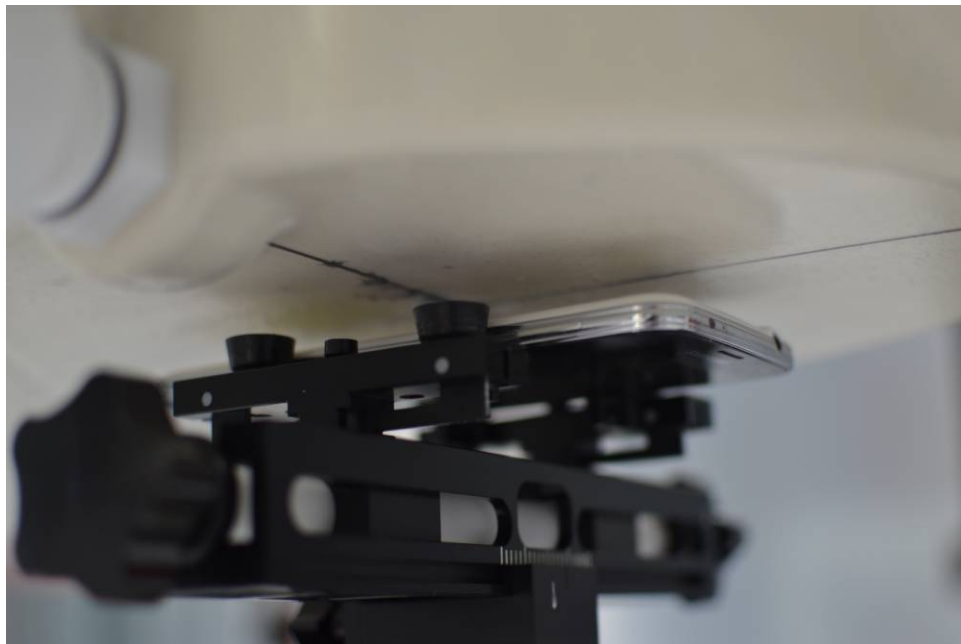
SAR Test Setup Photo 10 – Back Side at 1.0 cm
