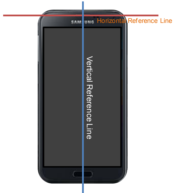
SAR Test Setup Photo 19 – DUT Reference Lines
