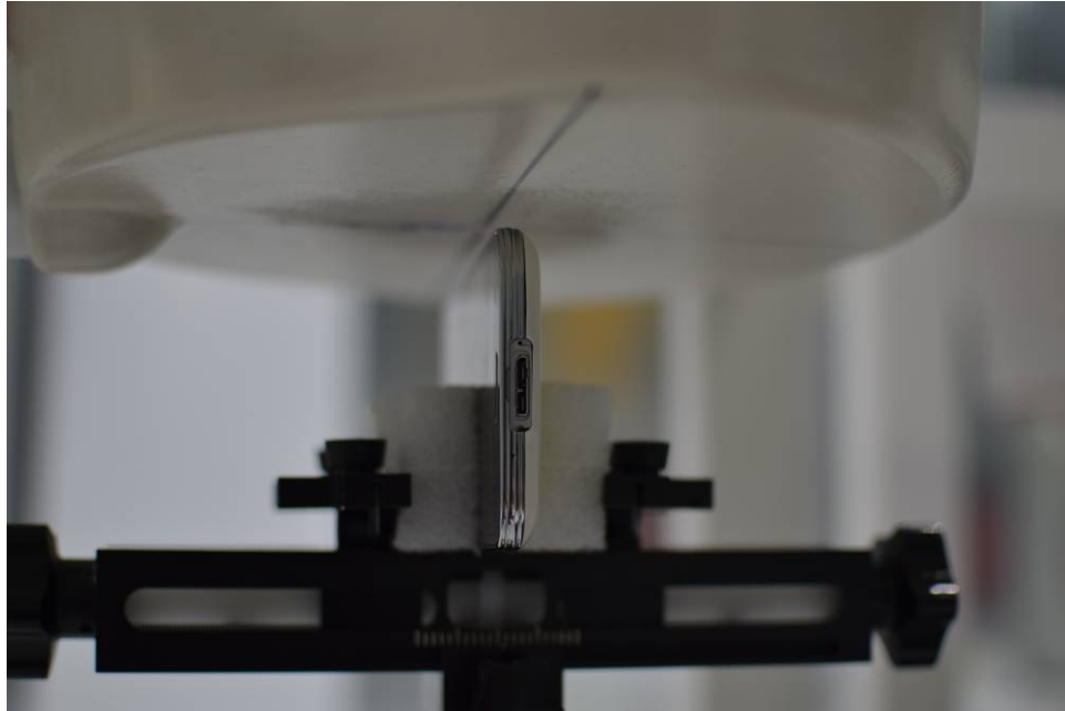
SAR Test Setup Photo 17 – Right Edge at 1.0 cm with Wireless Charging Cover
