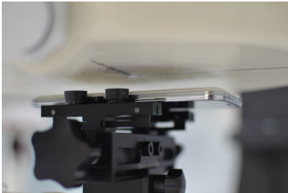
SAR Test Setup Photo 8 – Back Side at 1.5 cm
