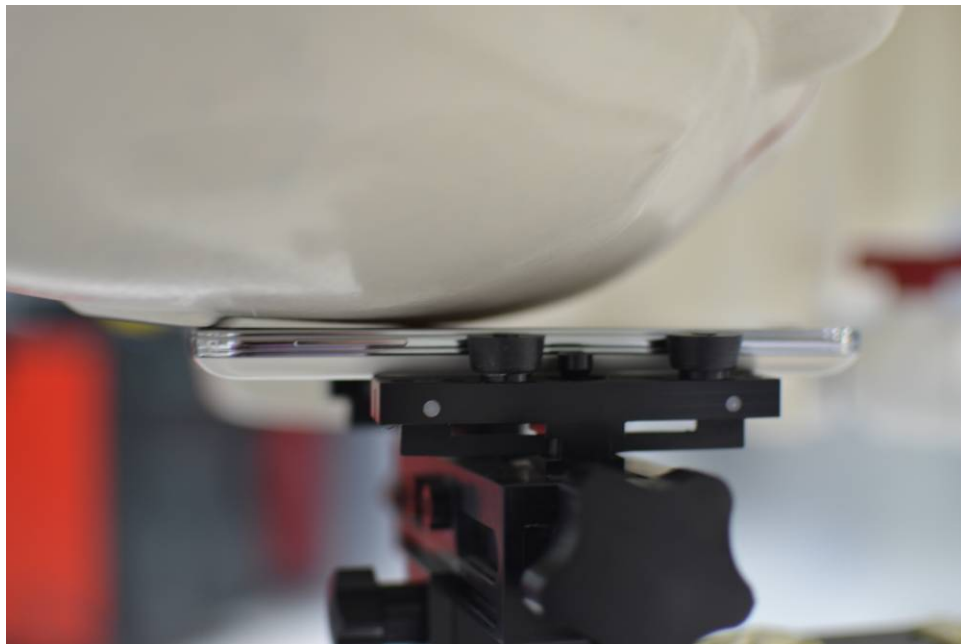
SAR Test Setup Photo 2 – Right Cheek with Wireless Charging Cover
