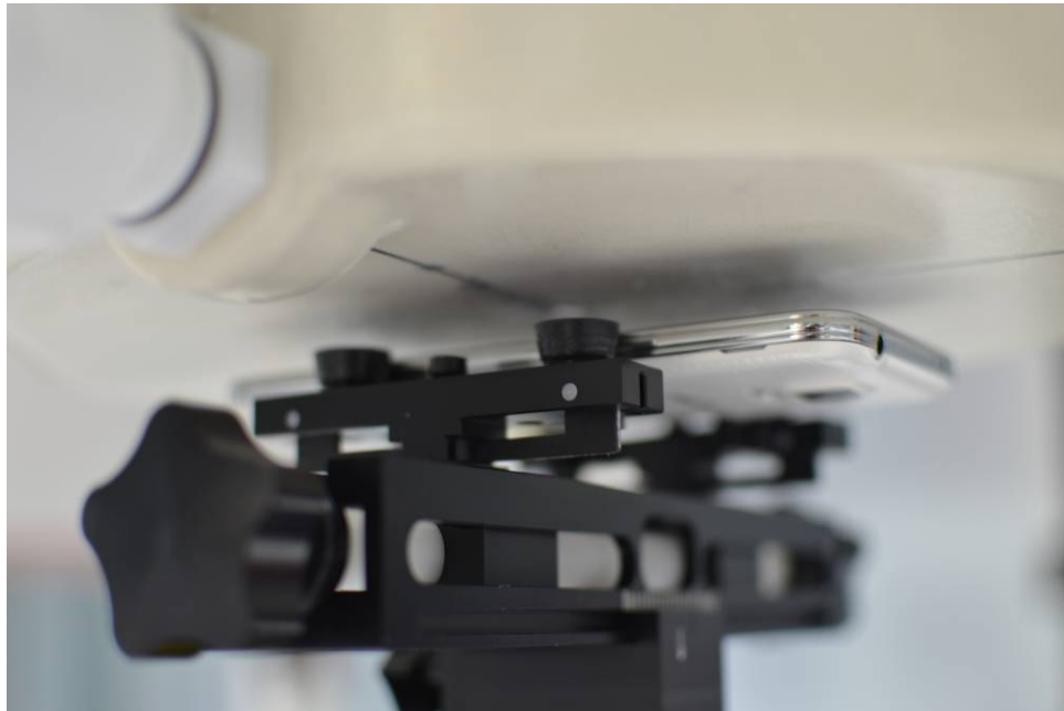
SAR Test Setup Photo 11 – Front Side at 1.0 cm
