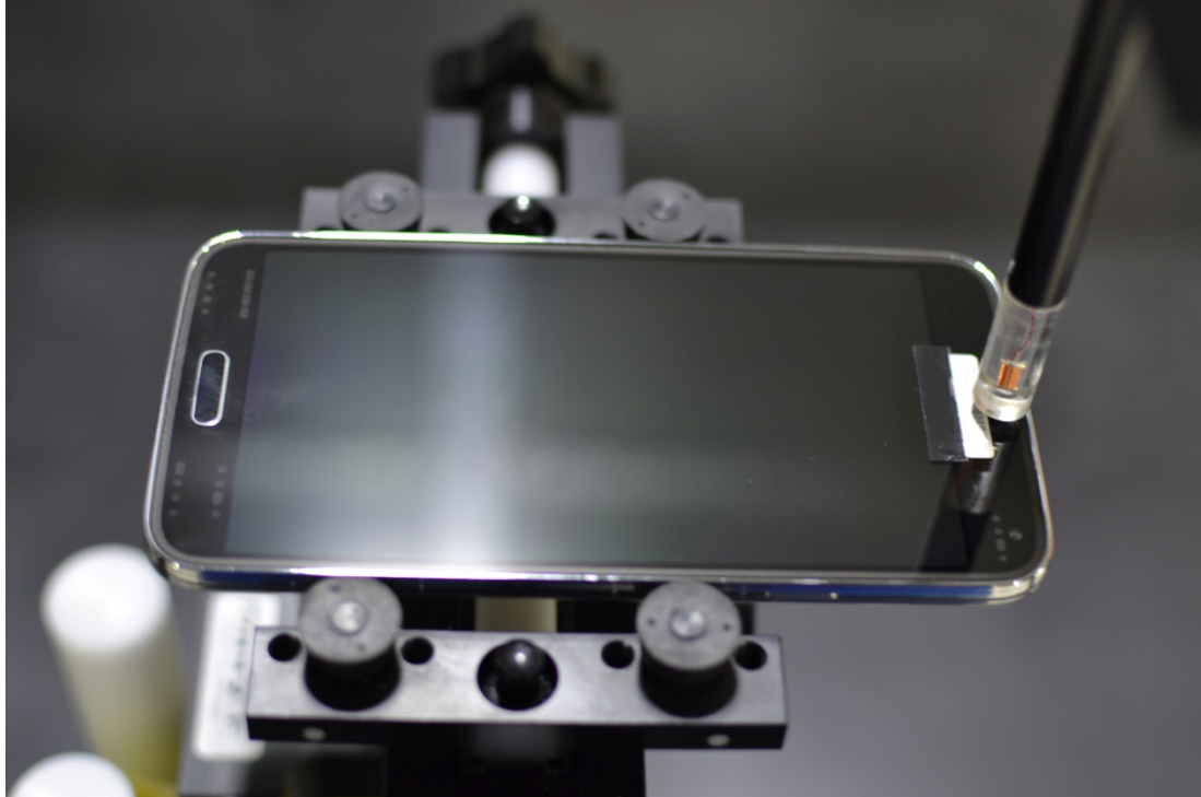
Figure 14-1 Test Setup for Wireless Device
