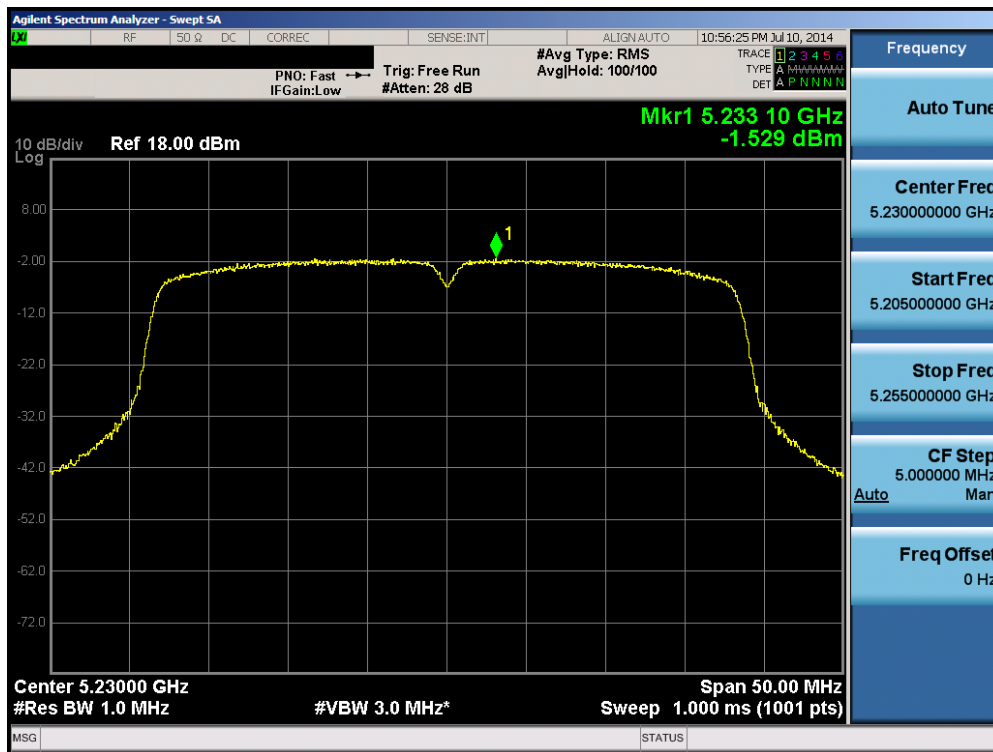
Plot 6-97. Peak Power Spectral Density Plot (40MHz BW 802.11n (UNII Band 1) – Ch. 46)
