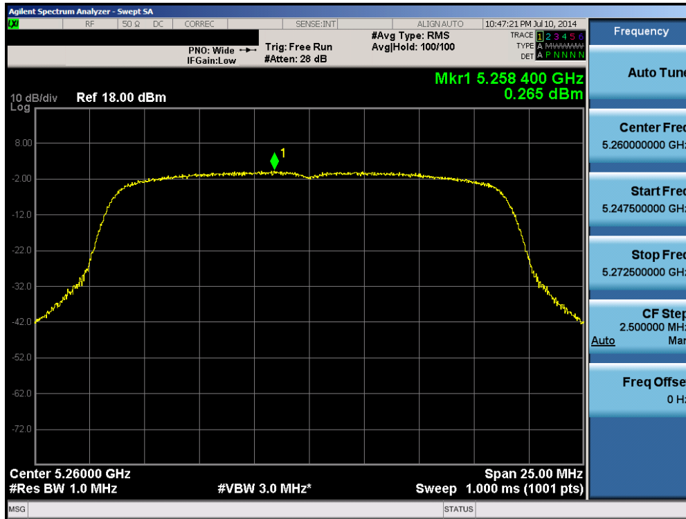
Plot 6-102. Peak Power Spectral Density Plot (20MHz BW 802.11n (UNII Band 2A) – Ch. 52)
