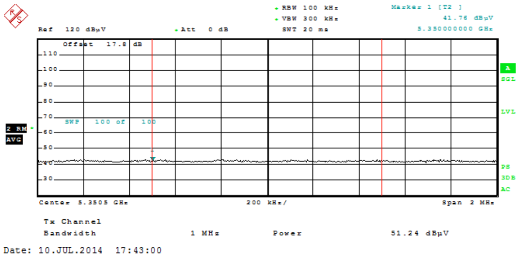
Plot 6-142. Radiated Restricted Upper Band Edge Plot (Average – UNII Band 2A)
