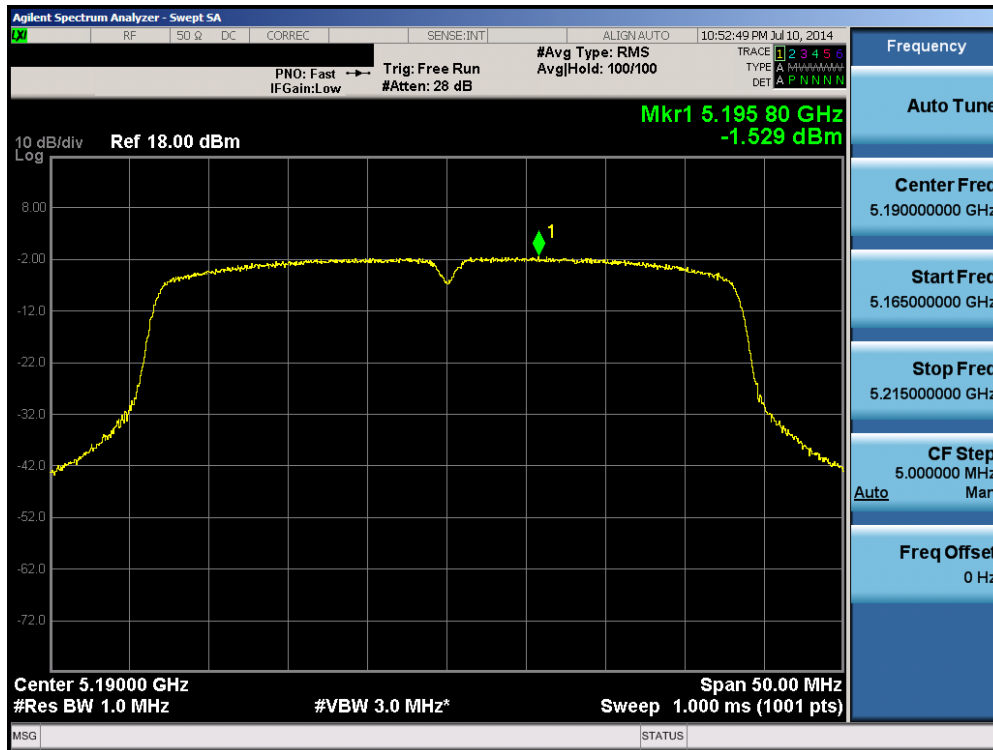
Plot 6-96. Peak Power Spectral Density Plot (40MHz BW 802.11n (UNII Band 1) – Ch. 38)
