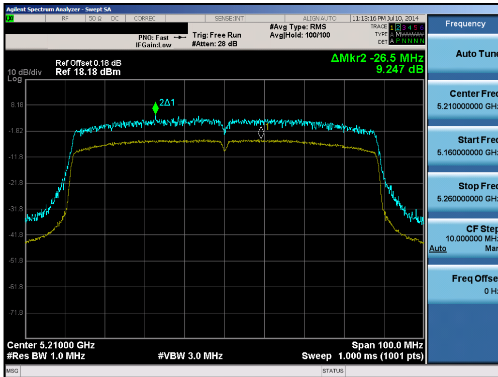
Plot 6-123. Peak Excursion Ratio Plot (80MHz BW 802.11ac (UNII Band 1) – Ch. 42)
