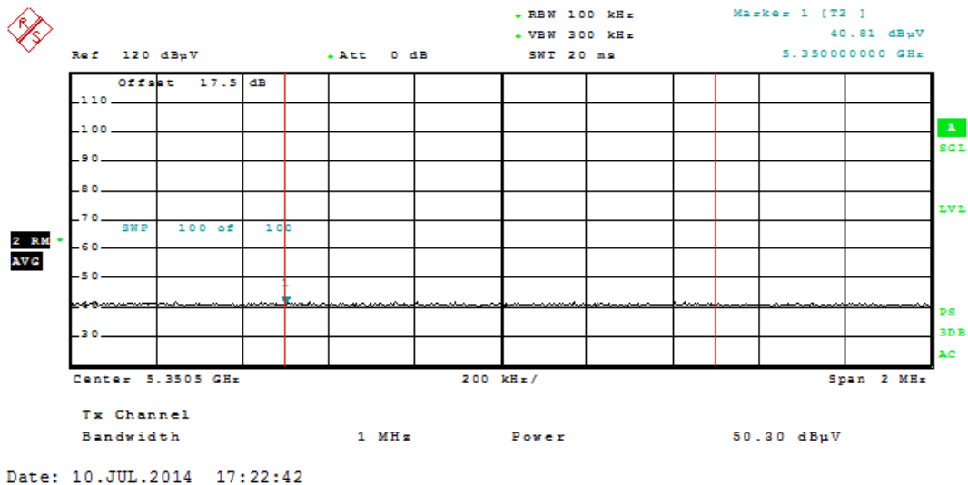
Plot 6-128. Radiated Restricted Upper Band Edge Plot (Average – UNII Band 2A)
