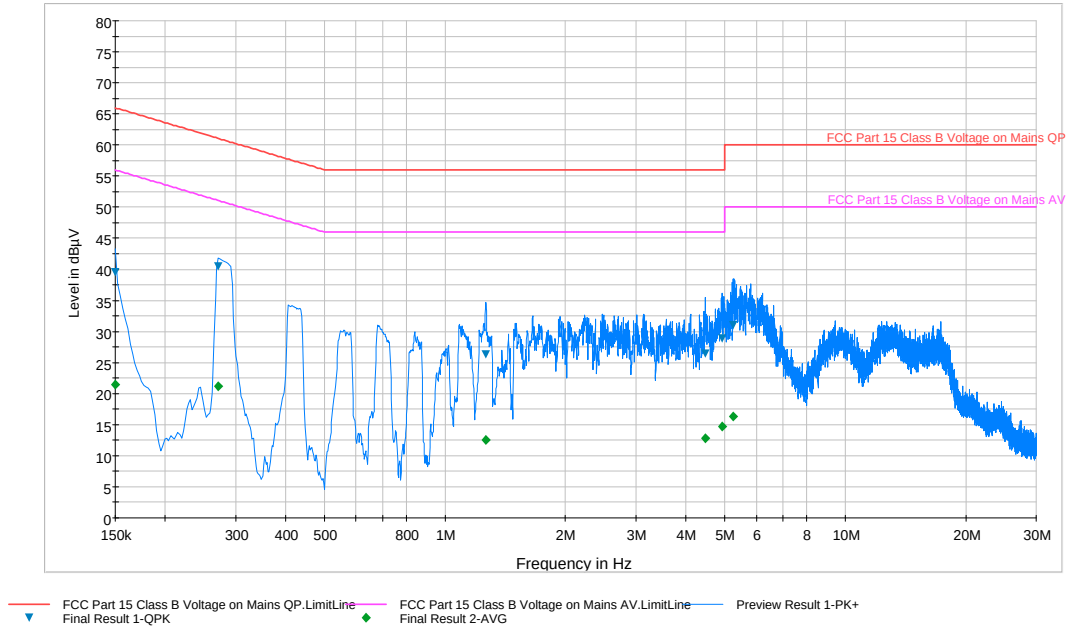
Plot 6-187. Line Conducted Plot with 802.11a UNII Band 1 (L1)
