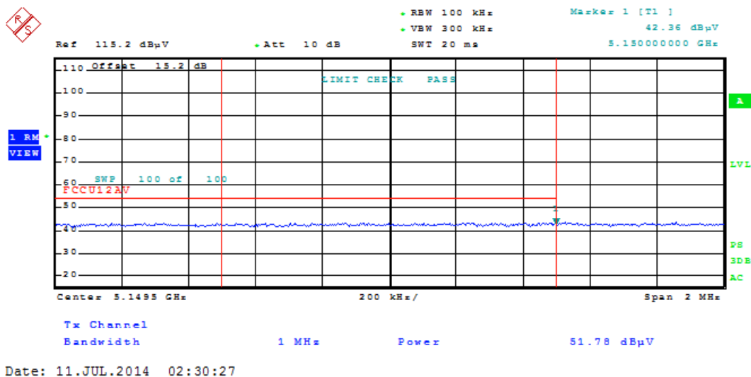
Plot 6-174. Radiated Restricted Lower Band Edge Plot (Average – UNII Band 1)
