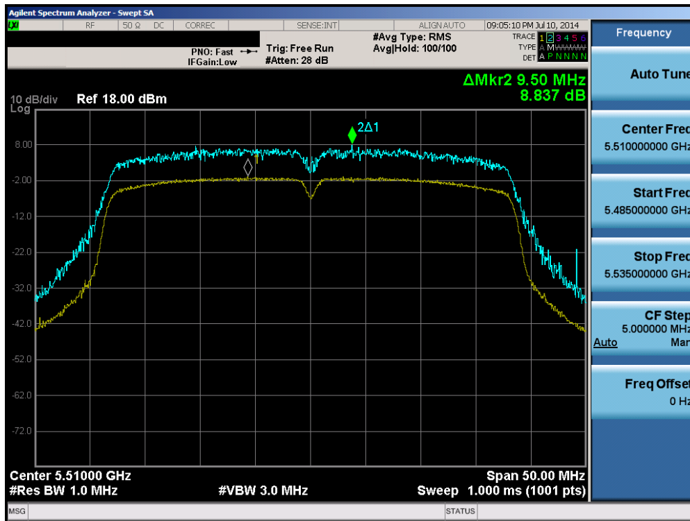
Plot 6-121. Peak Excursion Ratio Plot (40MHz BW 802.11n (UNII Band 2C) – Ch. 102)
