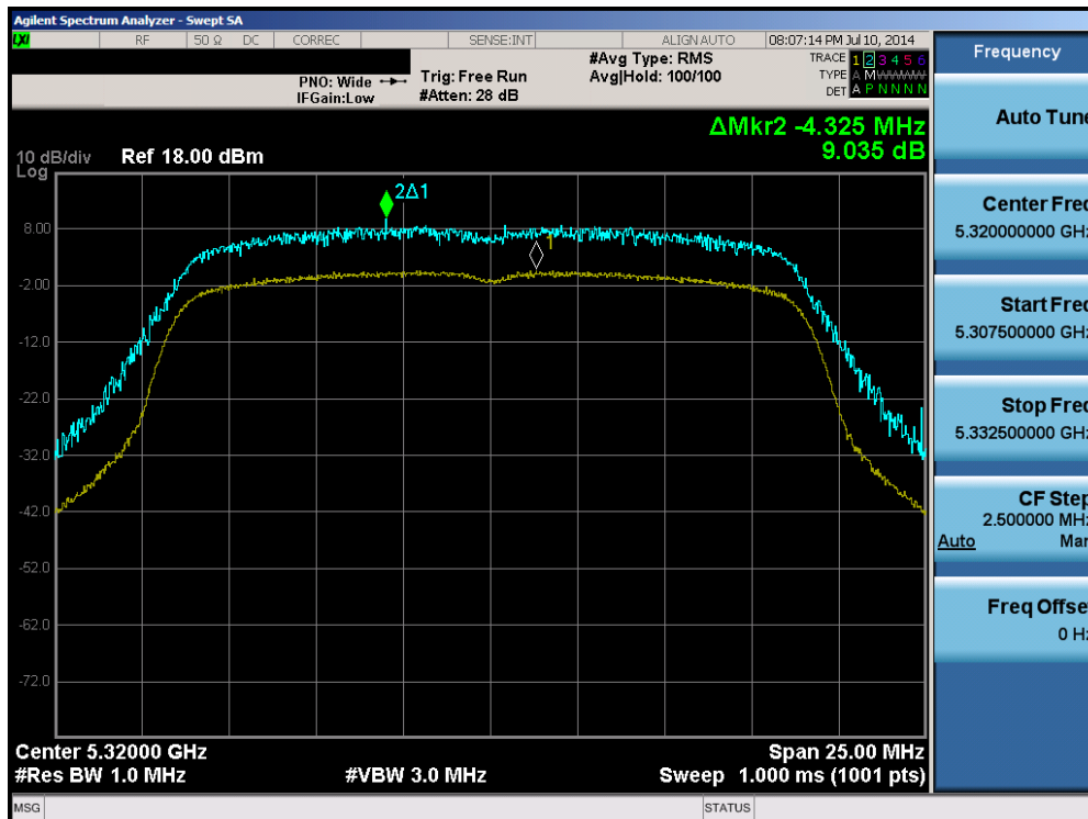
Plot 6-120. Peak Excursion Ratio Plot (20MHz BW 802.11n (UNII Band 2A) – Ch. 64)
