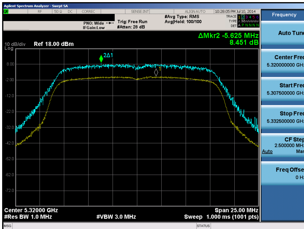
Plot 6-124. Peak Excursion Ratio Plot (802.11a (UNII Band 2A) – Ch. 64)
