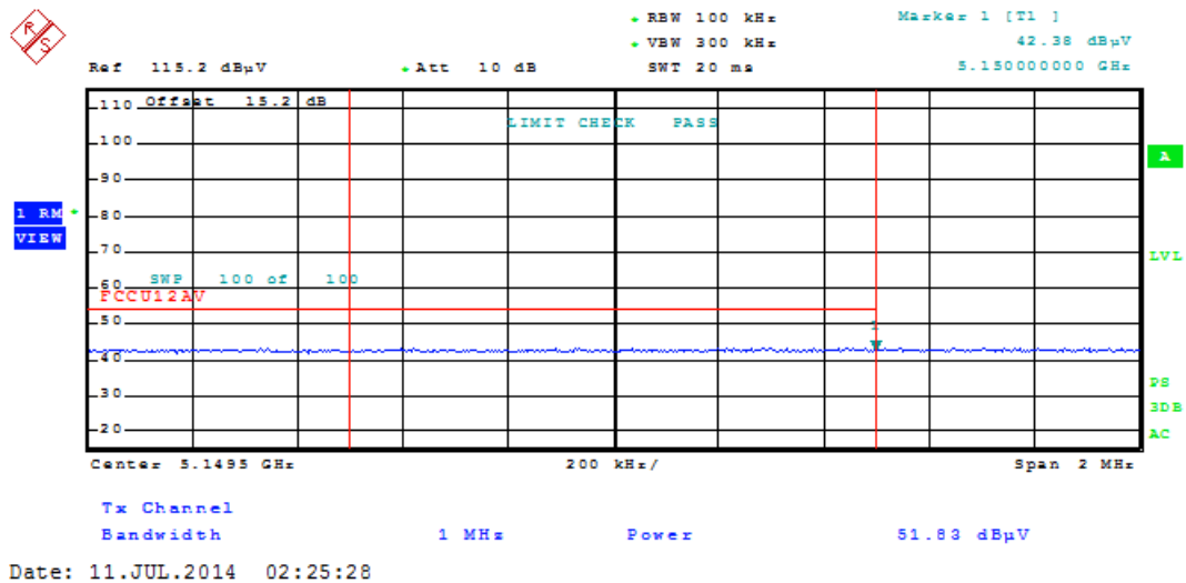
Plot 6-166. Radiated Restricted Lower Band Edge Plot (Average – UNII Band 1)
