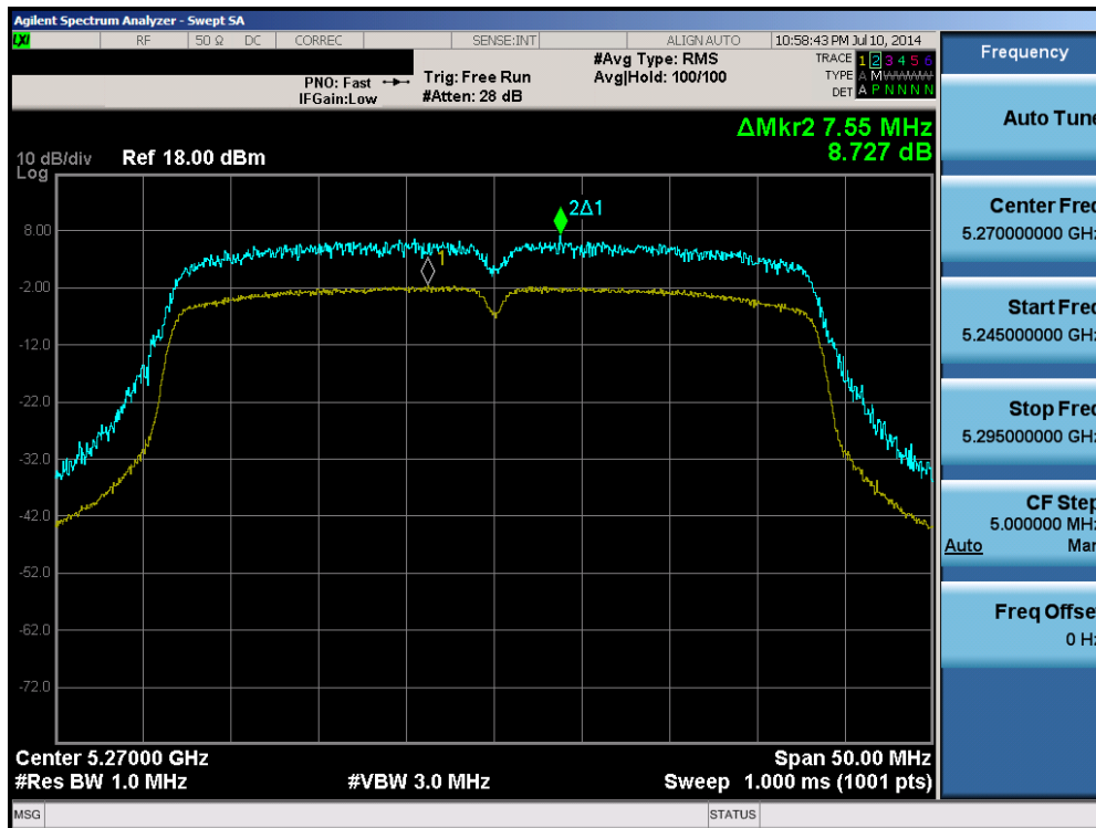
Plot 6-125. Peak Excursion Ratio Plot (40MHz BW 802.11n (UNII Band 2A) – Ch. 54)
