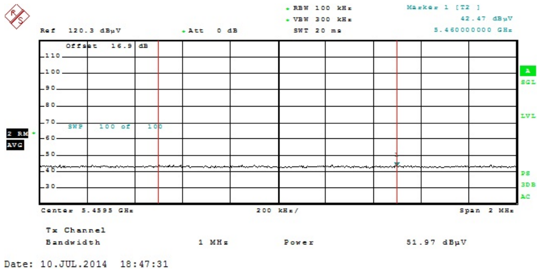
Plot 6-144. Radiated Restricted Lower Band Edge Plot (Average – UNII Band 2C)
