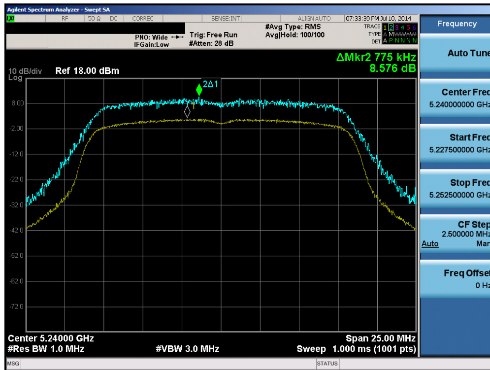
Plot 6-118. Peak Excursion Ratio Plot (802.11a (UNII Band 1) – Ch. 48)
