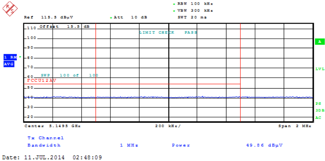
Plot 6-181. Radiated Restricted Lower Band Edge Plot (Average – UNII Band 1)
