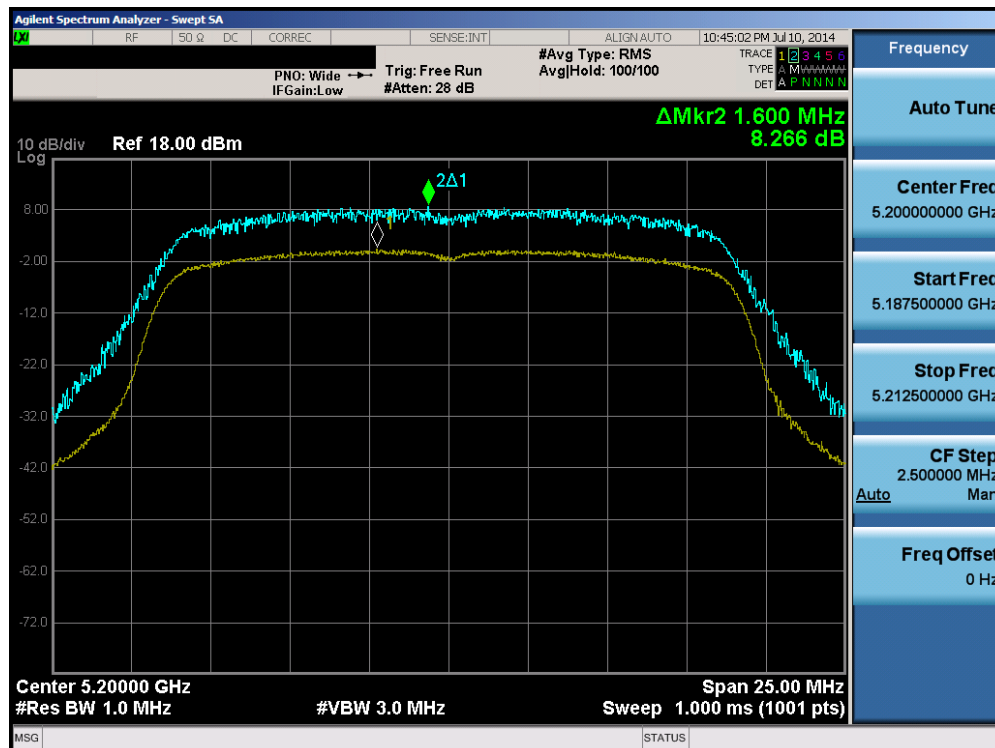
Plot 6-122. Peak Excursion Ratio Plot (20MHz BW 802.11n (UNII Band 1) – Ch. 40)
