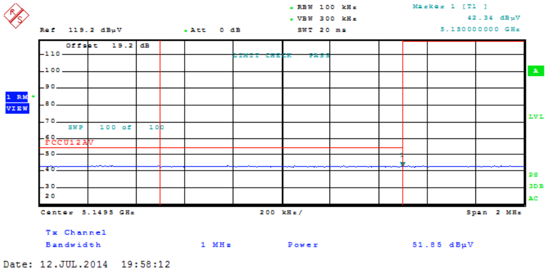
Plot 6-146. Radiated Restricted Lower Band Edge Plot (Average – UNII Band 1)
