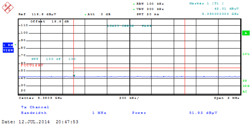
Plot 6-162. Radiated Restricted Upper Band Edge Plot (Average – UNII Band 2A)
