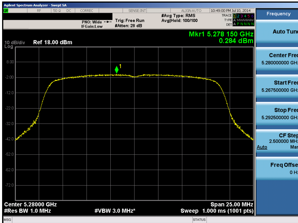
Plot 6-103. Peak Power Spectral Density Plot (20MHz BW 802.11n (UNII Band 2A) – Ch. 56)
