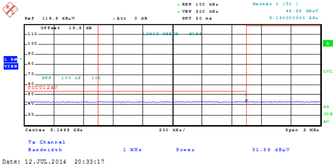
Plot 6-160. Radiated Restricted Lower Band Edge Plot (Average – UNII Band 1)
