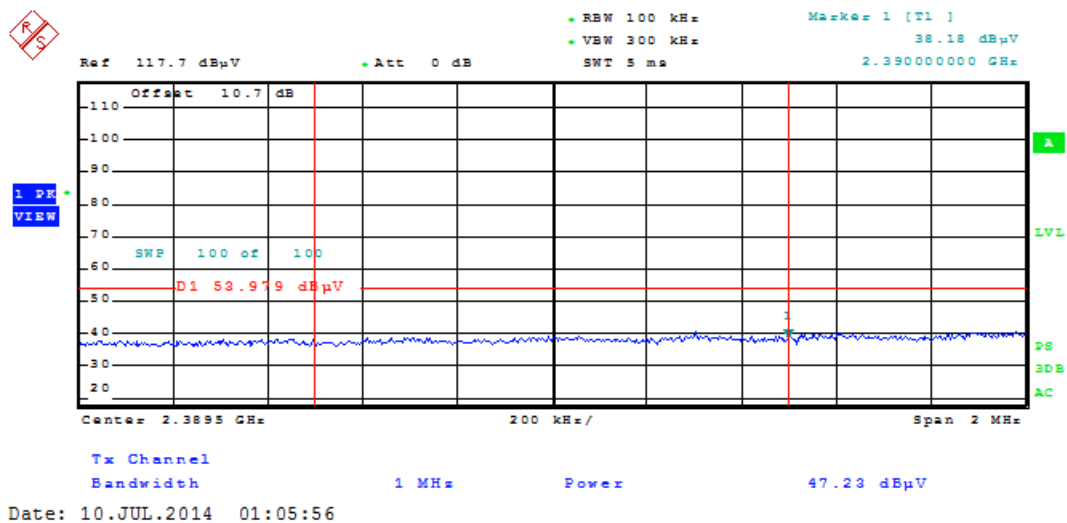
Plot 6-133. Radiated Restricted Lower Band Edge Measurement (Average)
