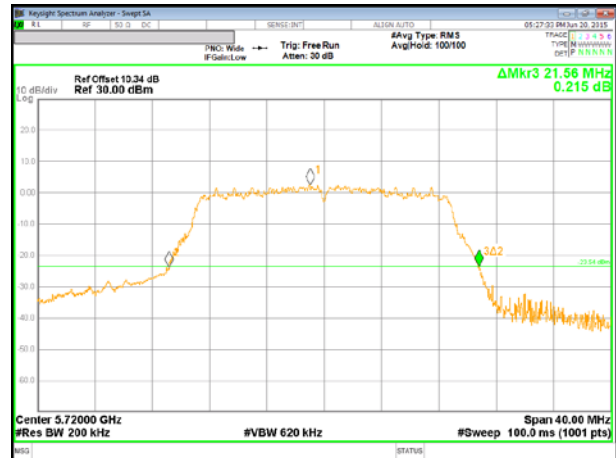
11n Mode Straddle Channel
