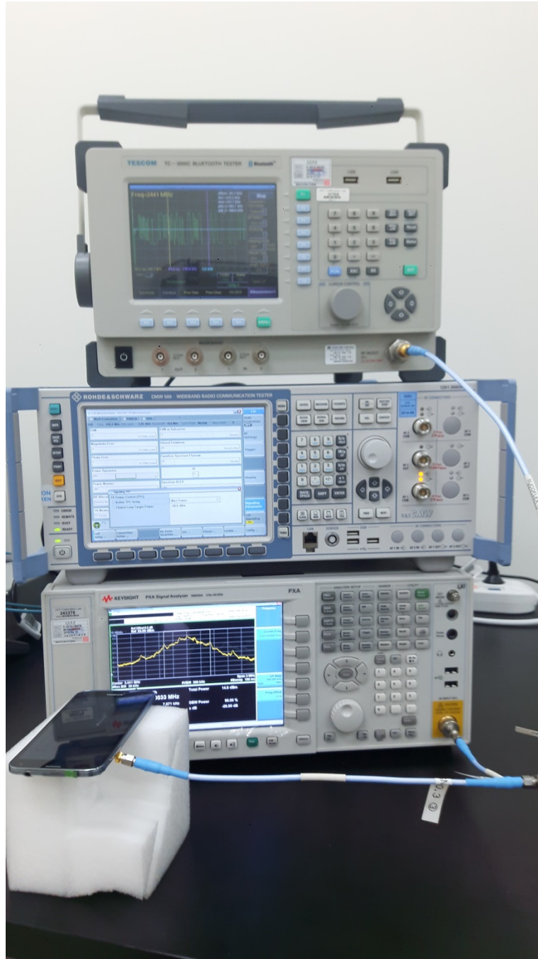
ANTENNA PORT CONDUCTED PHOTO
