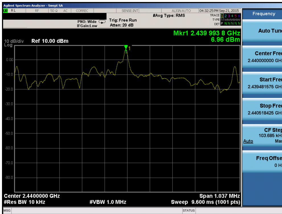
Plot 7-8. Power Spectral Density Plot (Bluetooth (LE) – Ch. 19)
