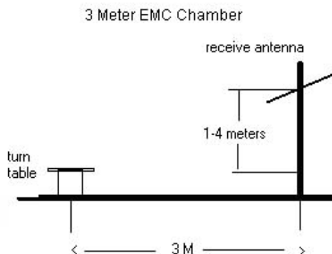
Figure 7-6. Test Instrument & Measurement Setup
