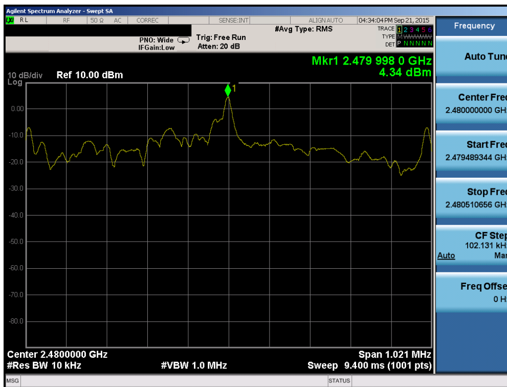
Plot 7-9. Power Spectral Density Plot (Bluetooth (LE) – Ch. 39)
