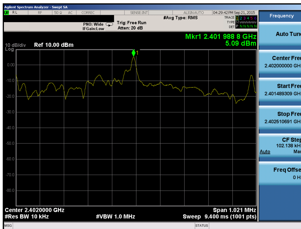
Plot 7-7. Power Spectral Density Plot (Bluetooth (LE) – Ch. 0)
