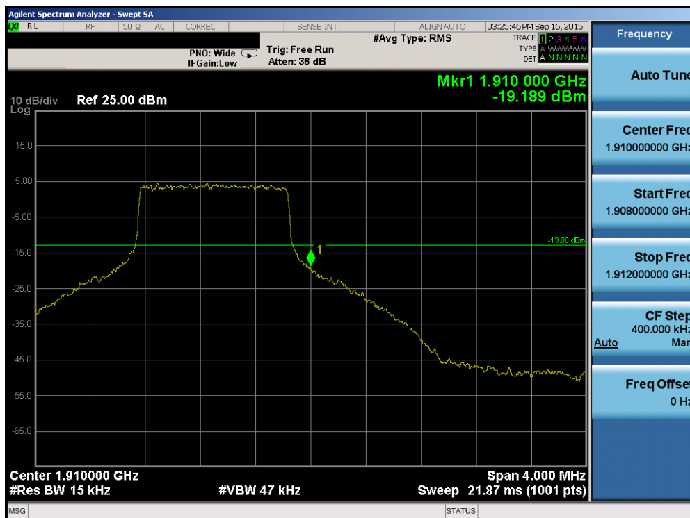
Plot 6-154. Upper Band Edge Plot (Band 2 – 1.4MHz QPSK – RB Size 6)
