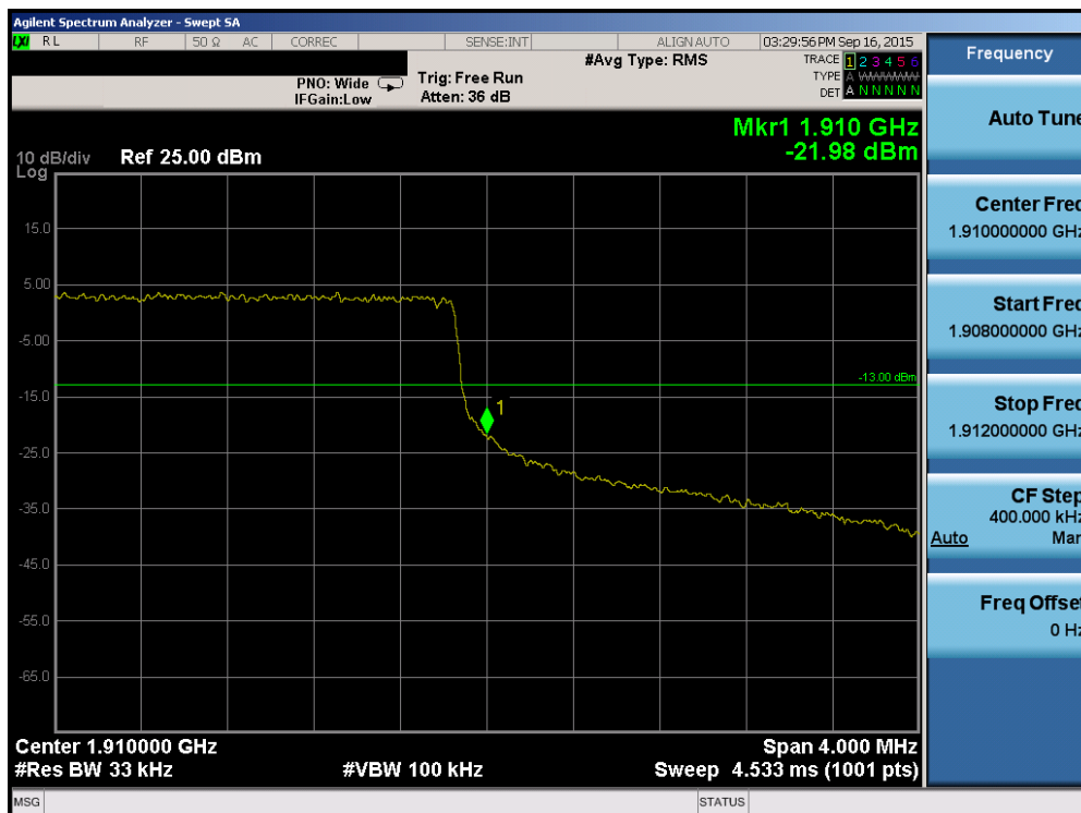
Plot 6-158. Upper Band Edge Plot (Band 2 – 3.0MHz QPSK – RB Size 15)
