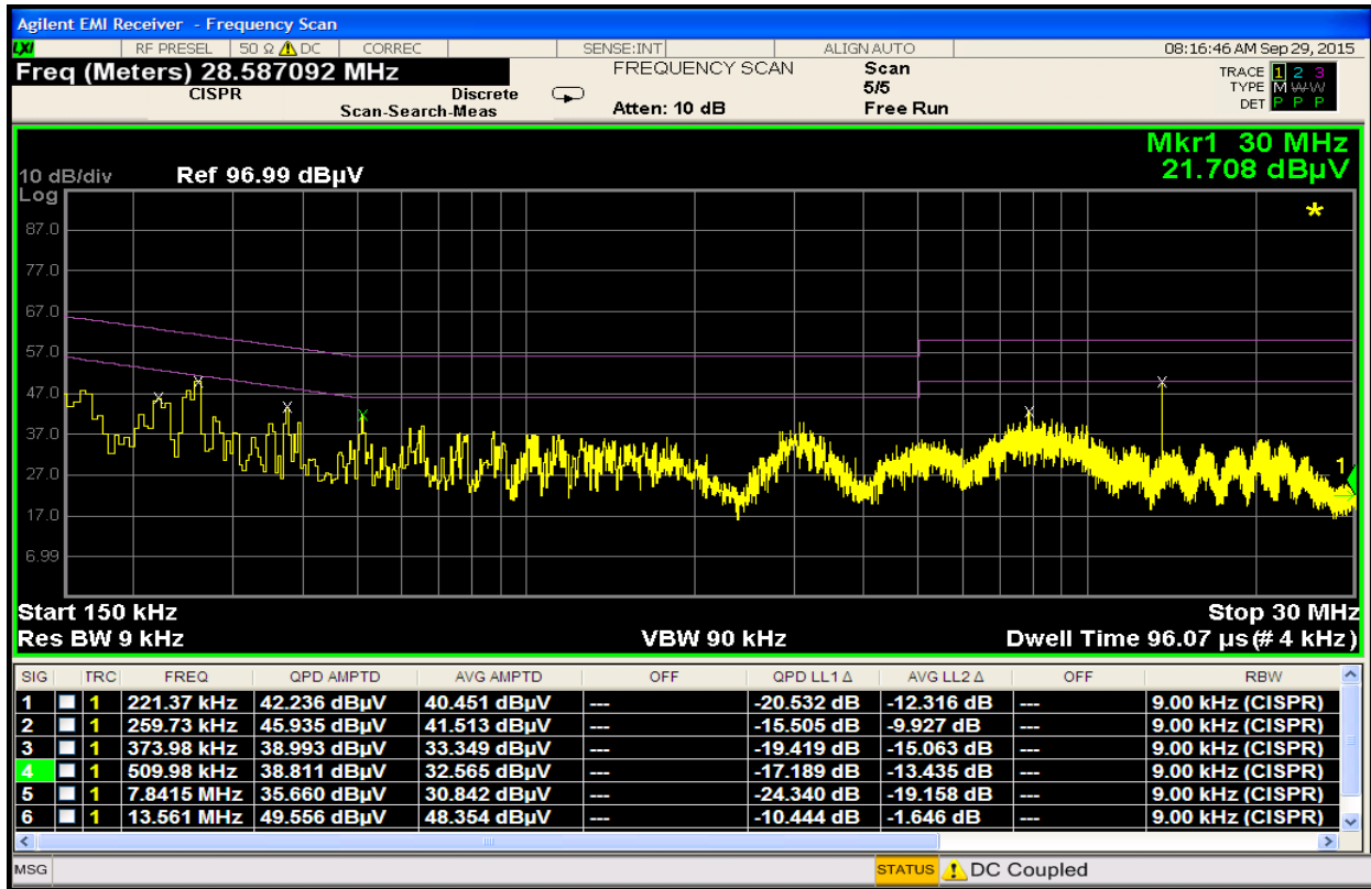
Plot 8-1. Line-Conducted Test Plot (L1)
