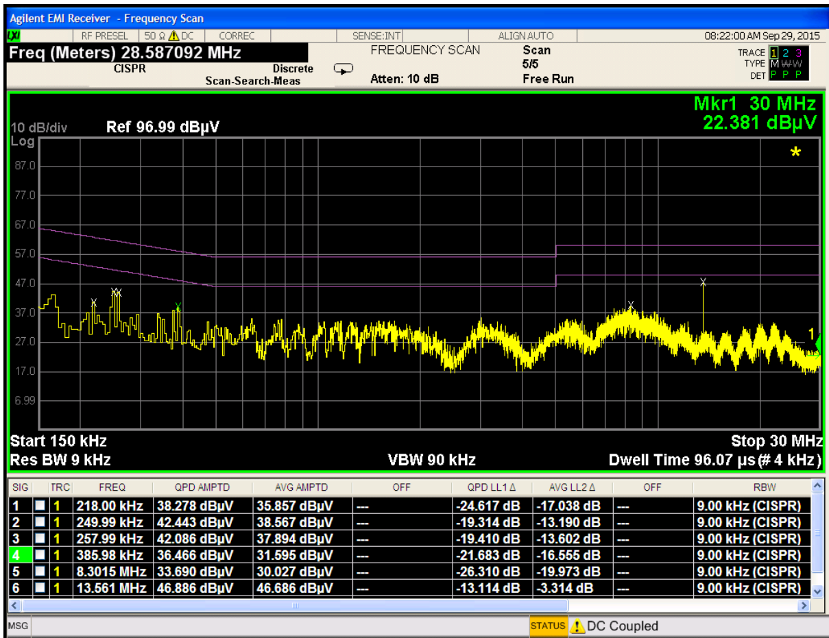
Plot 8-2. Line-Conducted Test Plot (N)
