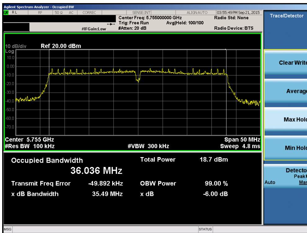
Plot 7-37. 6dB Bandwidth Plot (40MHz BW 802.11n (UNII Band 3) – Ch. 151)
