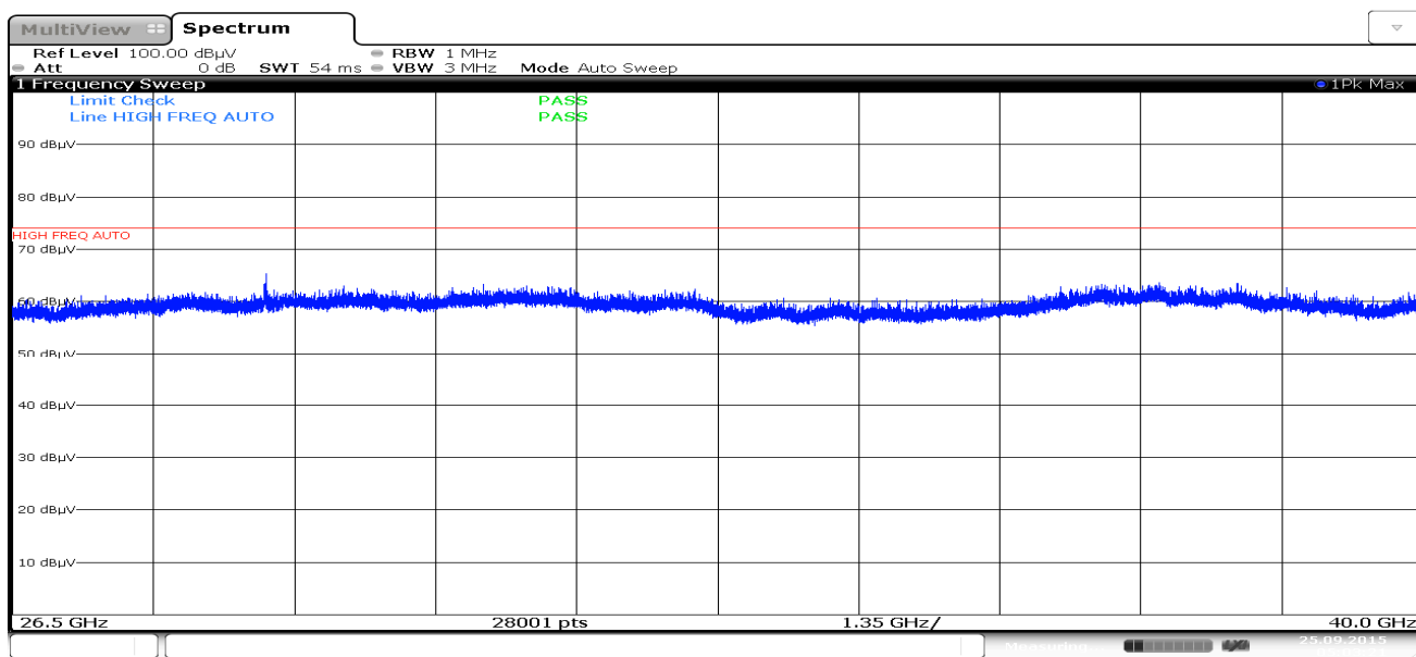
Plot 7-90. Radiated Spurious Plot above 18GHz (802.11a - Ant. Pol. V)
