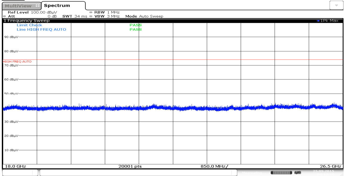
Plot 7-87. Radiated Spurious Plot above 18GHz (802.11a – Ant. Pol. H)
