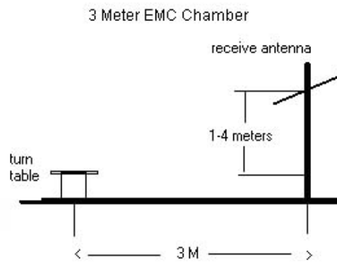
Figure 7-5. Test Instrument & Measurement Setup
