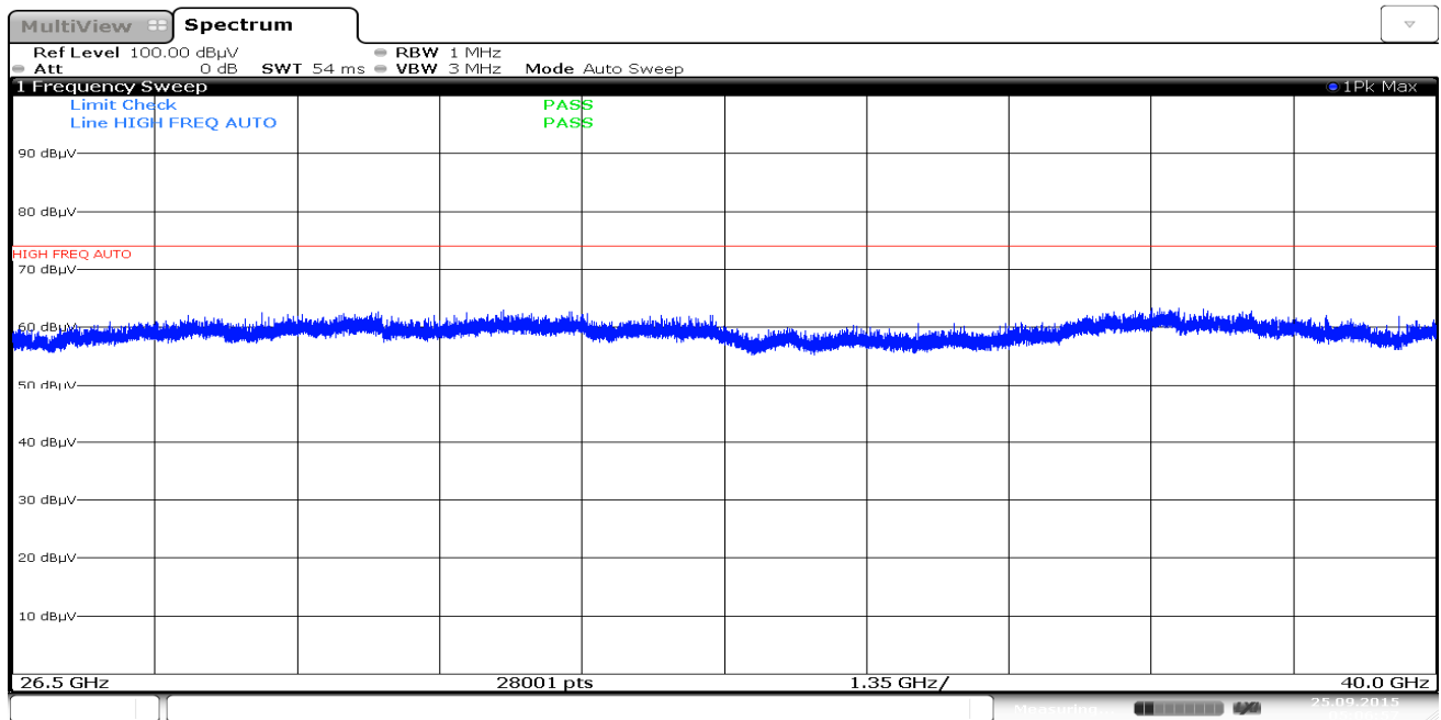
Plot 7-88. Radiated Spurious Plot above 18GHz (802.11a - Ant. Pol.H)
