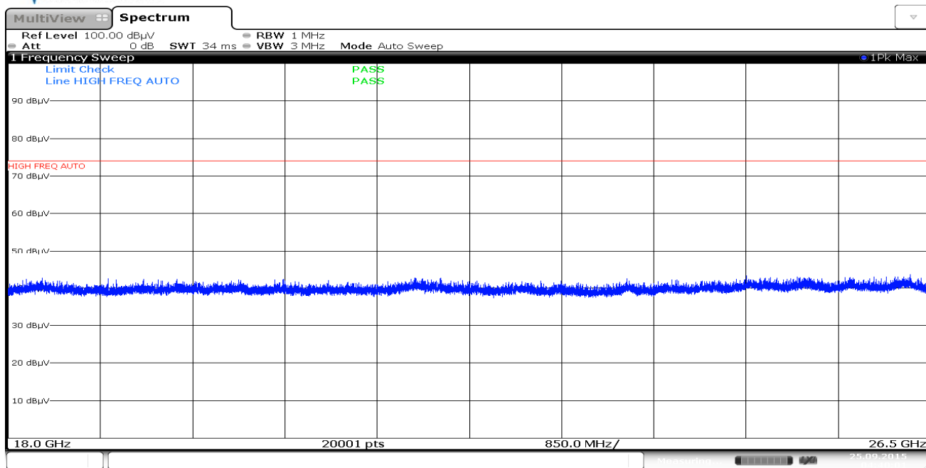
Plot 7-89. Radiated Spurious Plot above 18GHz (802.11a – Ant. Pol. V)
