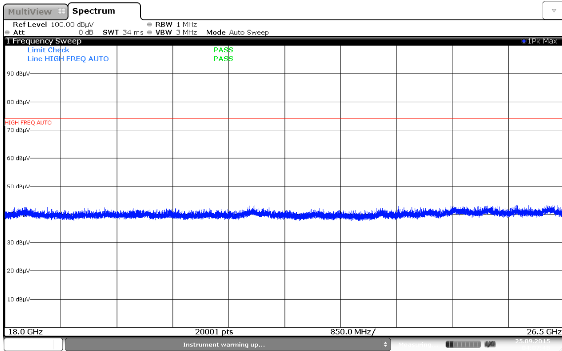
Plot 7-44. Radiated Spurious Plot above 18GHz (Pol. V)
