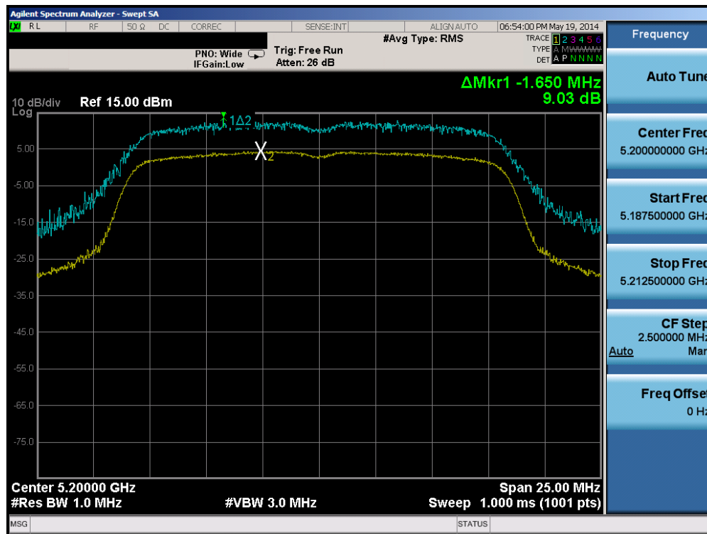
Plot 6-125. Peak Excursion Ratio Plot (802.11a (UNII Band 1) – Ch. 40)
