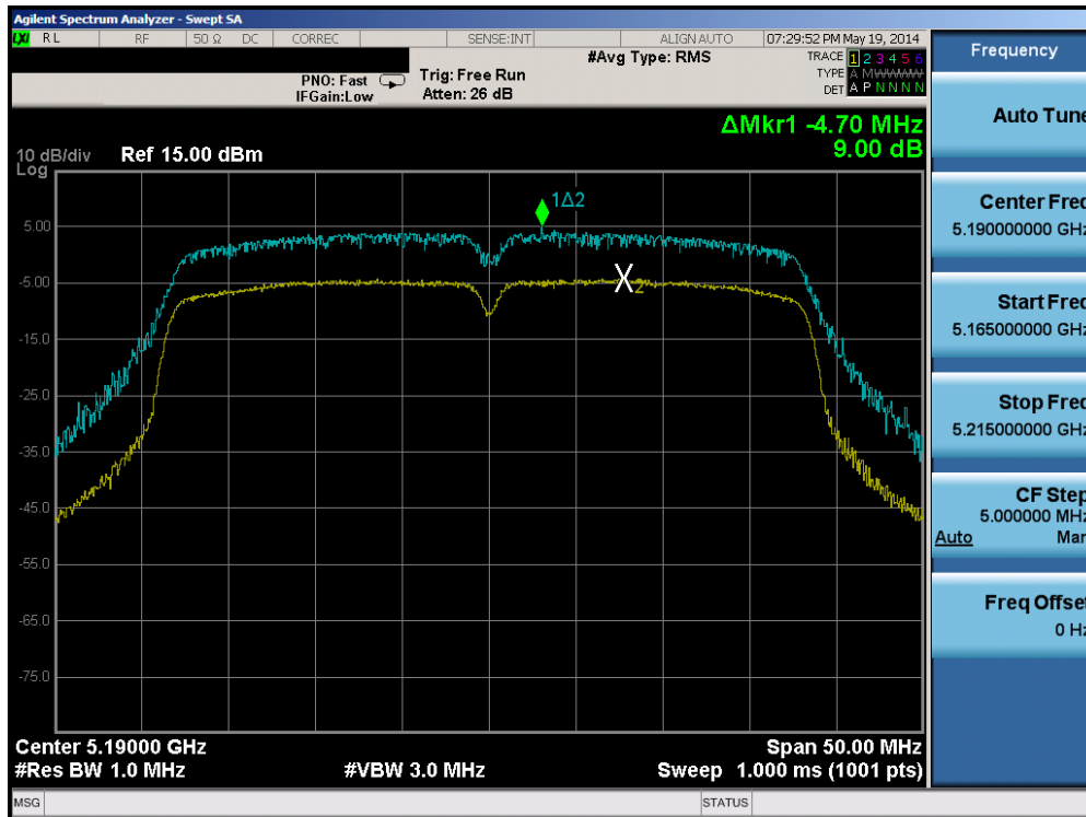
Plot 6-126. Peak Excursion Ratio Plot (40MHz BW 802.11n (UNII Band 1) – Ch. 38)
