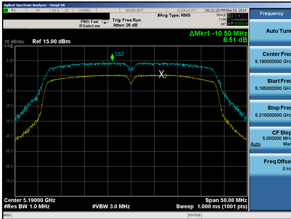
Plot 6-130. Peak Excursion Ratio Plot (40MHz BW 802.11n (UNII Band 1) – Ch. 38)
