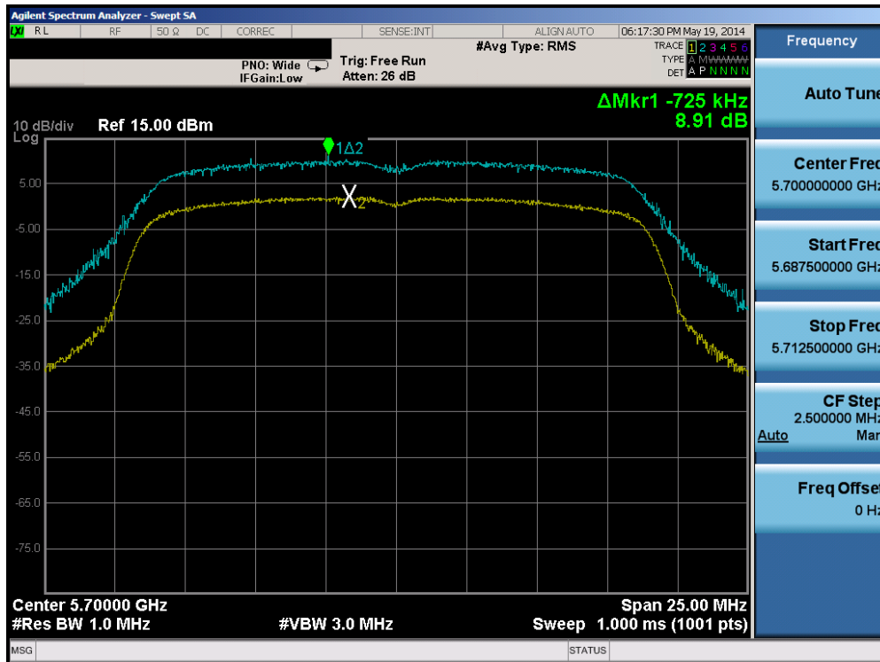
Plot 6-132. Peak Excursion Ratio Plot (20MHz BW 802.11n (UNII Band 2C) – Ch. 140)
