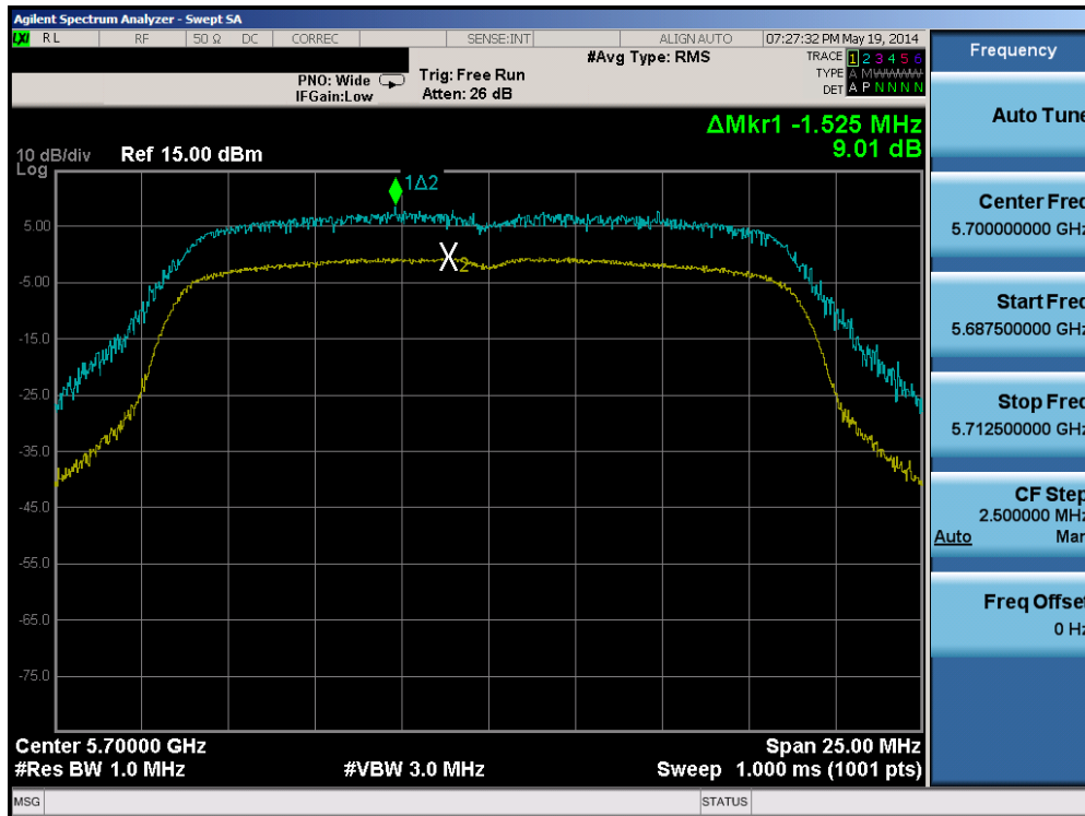
Plot 6-128. Peak Excursion Ratio Plot (20MHz BW 802.11n (UNII Band 2C) – Ch. 140)
