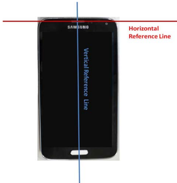
SAR Test Setup Photo 11 – Vertical and Horizontal Reference Lines
