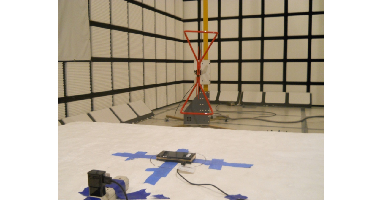
RADIATED BACK PHOTO (BELOW 1 GHz)
