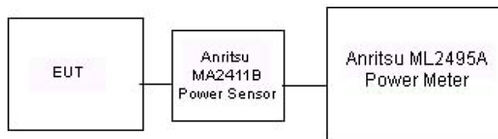
Figure 9-3 Power Measurement Setup < 50MHz Bandwidth
