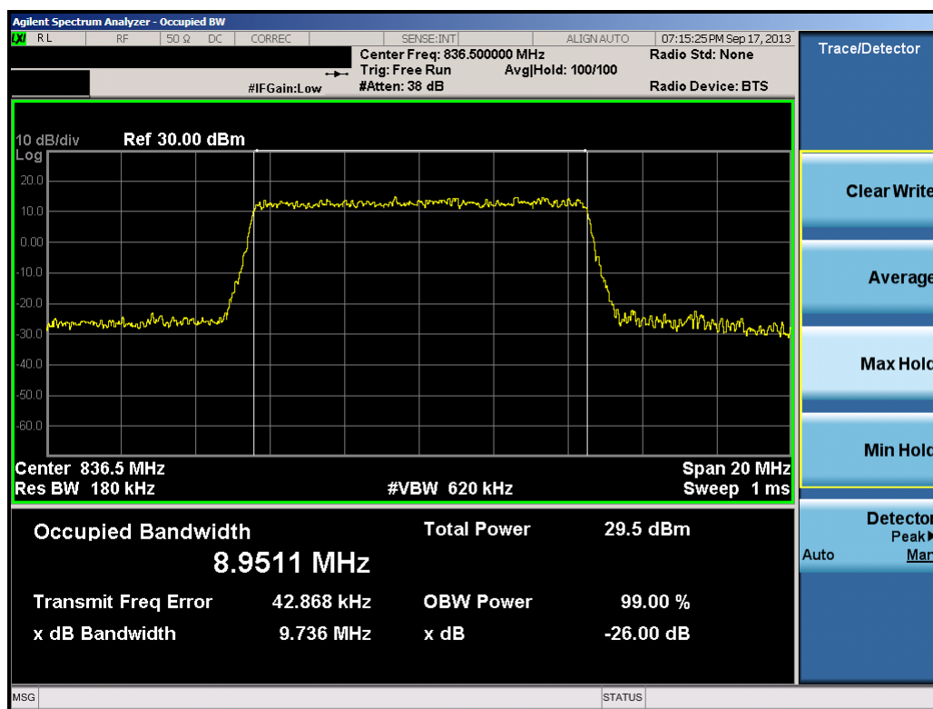
Plot 7-7. Occupied Bandwidth Plot (10.0MHz 16-QAM – RB Size 50)
