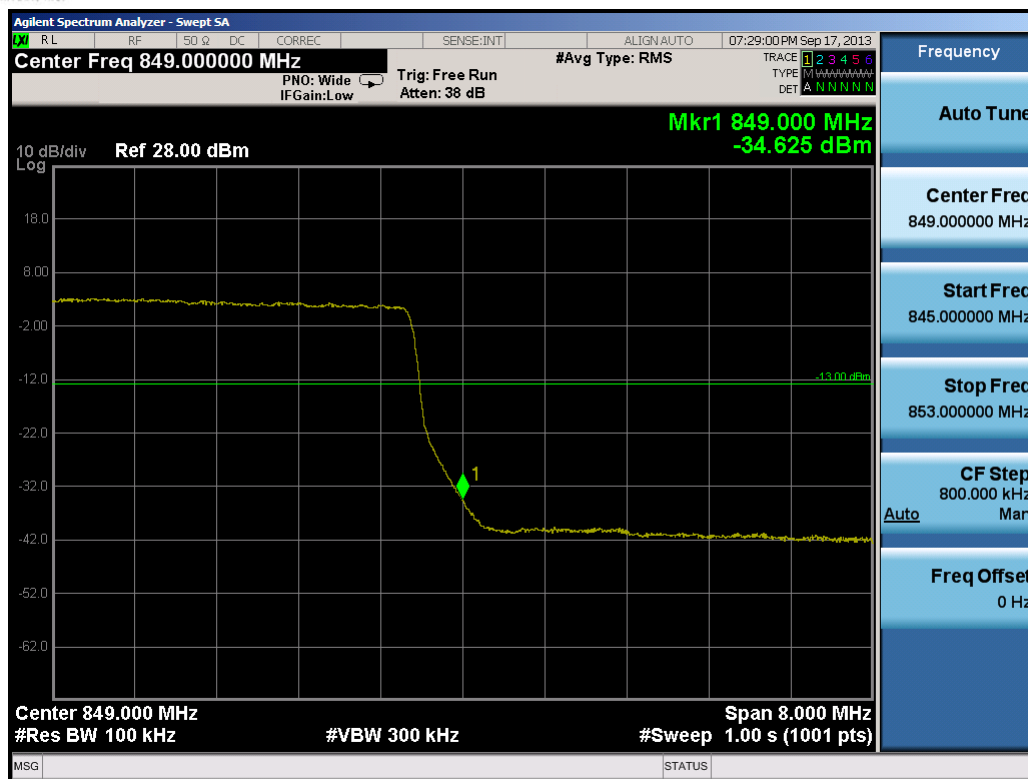
Plot 7-14. Upper Band Edge Plot (10.0MHz QPSK – RB Size 50)
