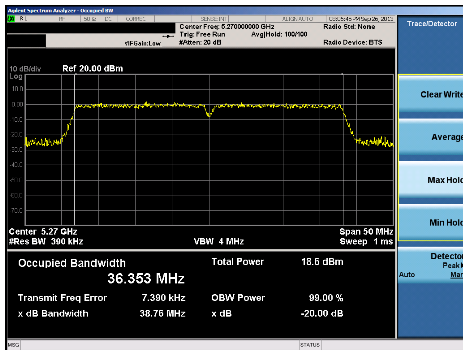
Plot 6-30. 20dB Bandwidth Plot (40MHz BW 802.11n (UNII Band 2) – Ch. 54)
