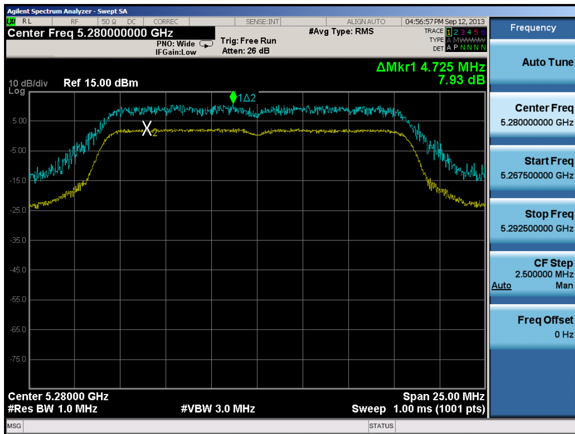
Plot 6-59. Peak Excursion Ratio Plot (802.11a)
