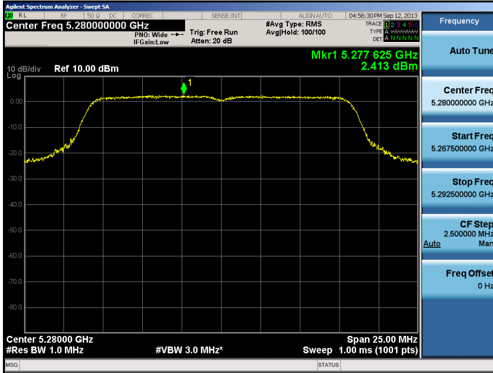
Plot 6-41. Peak Power Spectral Density Plot (802.11a (UNII Band 2) – Ch. 56)
