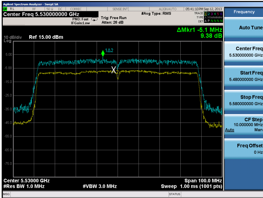
Plot 6-62. Peak Excursion Ratio Plot (80MHz BW 802.11ac)
