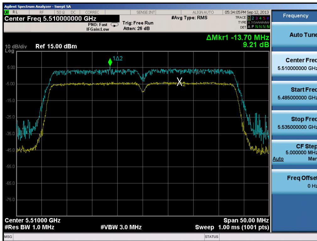
Plot 6-61. Peak Excursion Ratio Plot (40MHz BW 802.11n)
