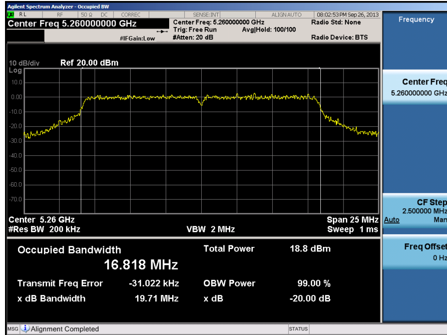
Plot 6-29. 20dB Bandwidth Plot (20MHz BW 802.11n (UNII Band 2) – Ch. 52)
