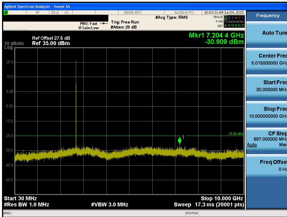
BAND 41. Conducted Spurious Plot 1 (5 MHz Ch.41565 QPSK RB 1, Offset 0)
