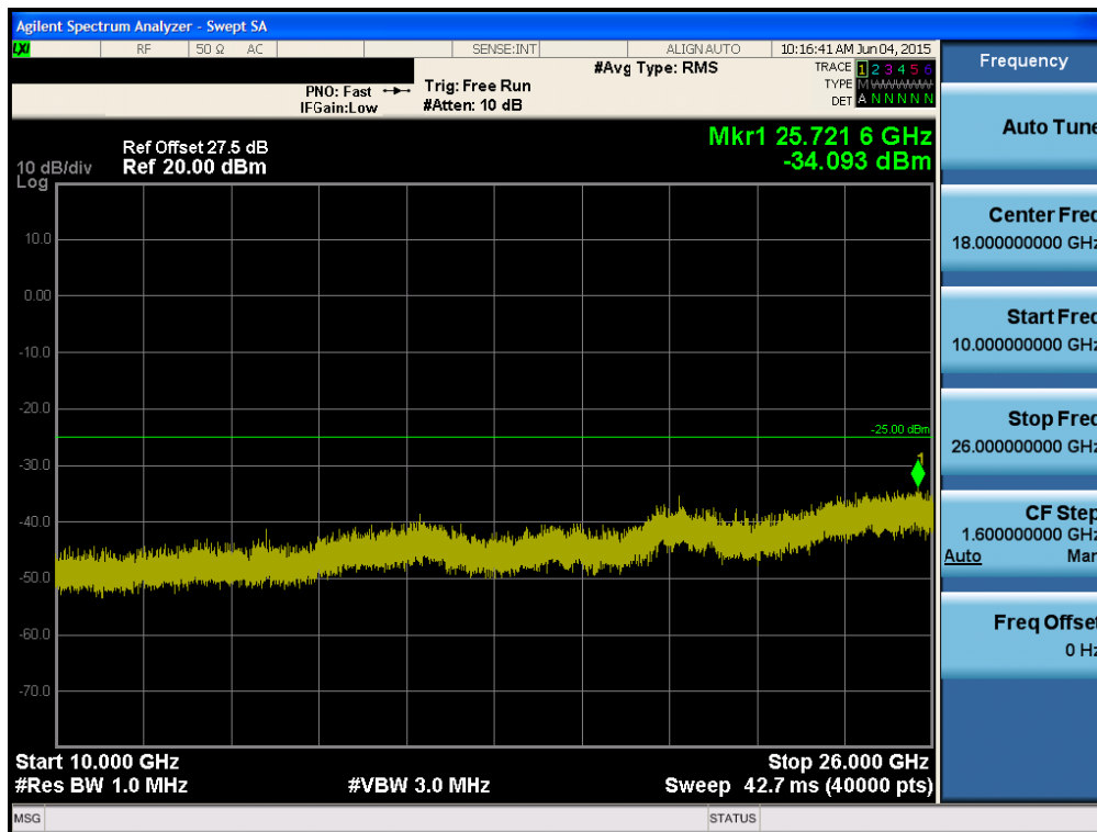
BAND 41. Conducted Spurious Plot 2 (5 MHz Ch. 41565 QPSK RB 1, Offset 0)
