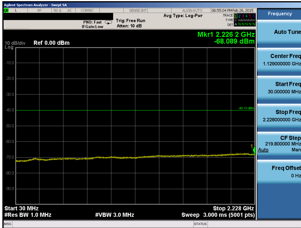
Plot 6-87. Conducted Spurious Plot (Band 30 – 5.0MHz QPSK – RB Size 1, RB Offset 0 – High Channel)
