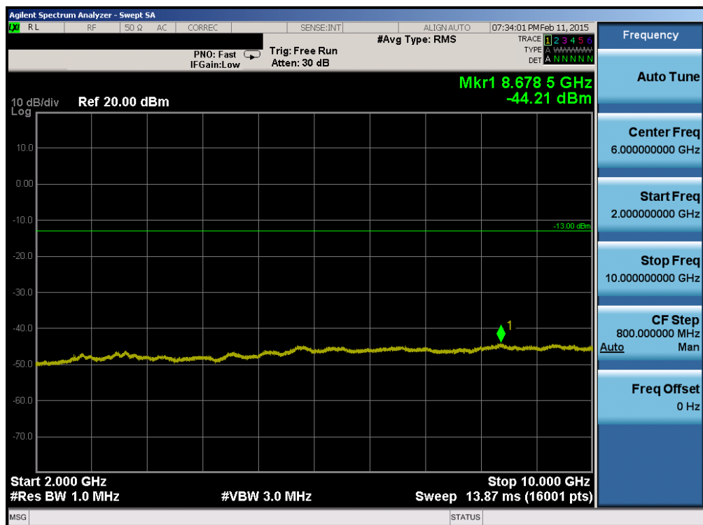
Plot 6-62. Conducted Spurious Plot (Band 5 – 3.0MHz QPSK – RB Size 1, RB Offset 0 – High Channel)
