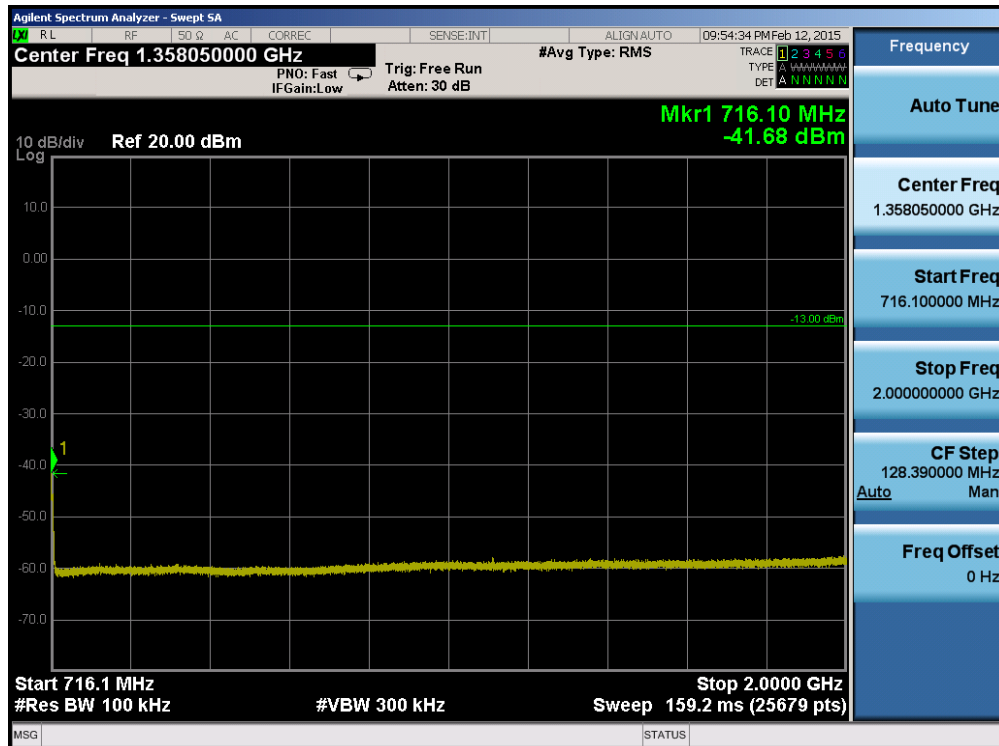
Plot 6-52. Conducted Spurious Plot (Band 12 – 5.0MHz QPSK – RB Size 1, RB Offset 0 – High Channel)
