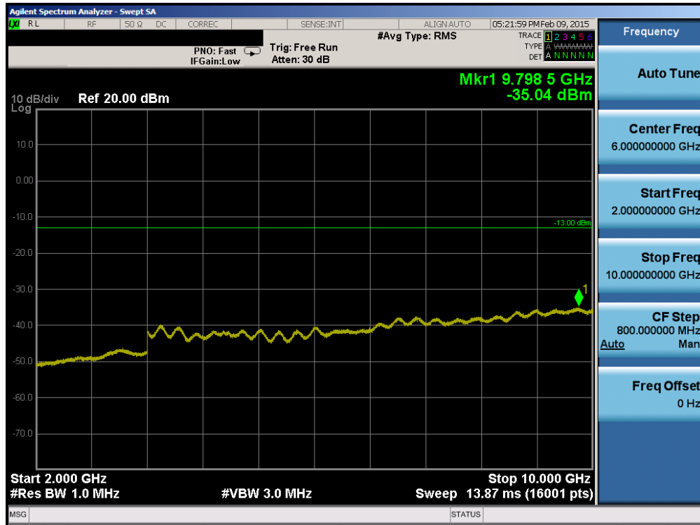
Plot 6-59. Conducted Spurious Plot (Band 5 – 3.0MHz QPSK – RB Size 1, RB Offset 0 – Mid Channel)
