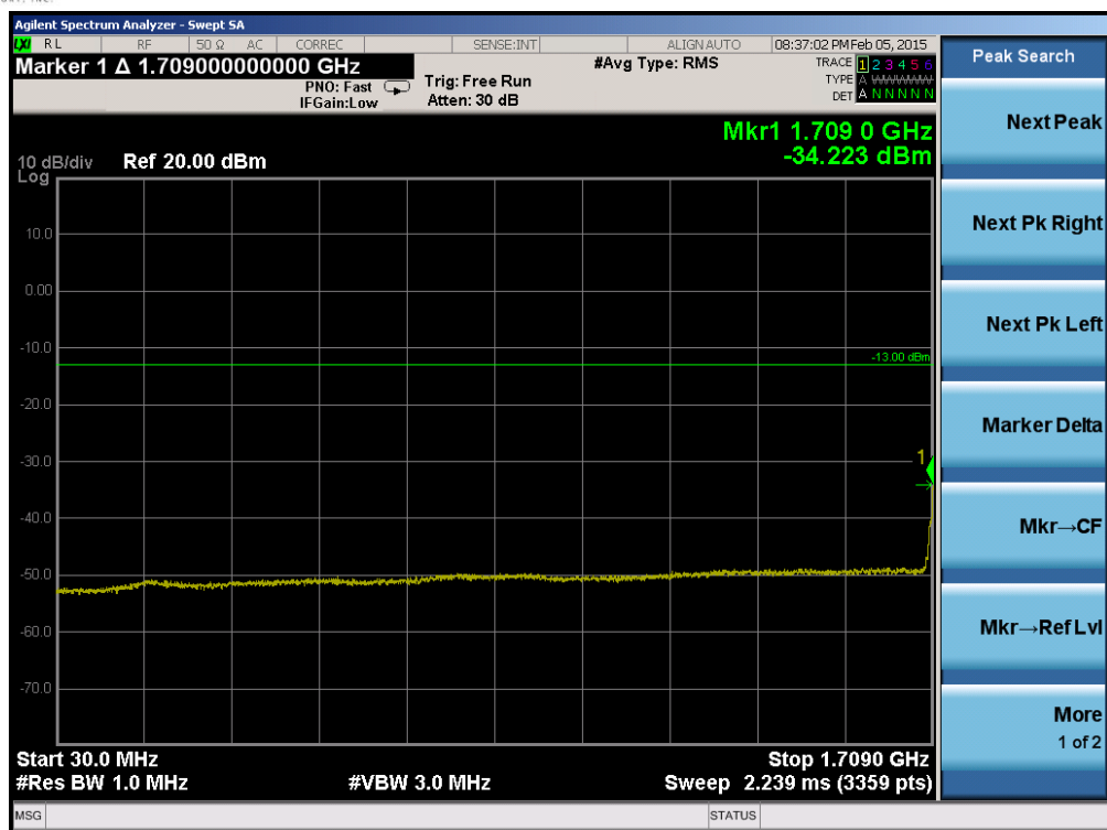
Plot 6-63. Conducted Spurious Plot (Band 4 – 5.0MHz QPSK – RB Size 1, RB Offset 0 – Low Channel)
