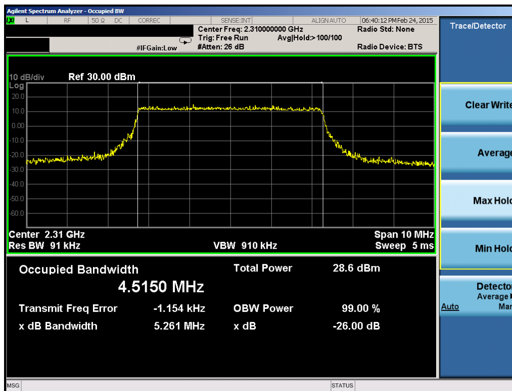
Plot 6-42. Occupied Bandwidth Plot (Band 30 – 5.0MHz 16-QAM – RB Size 25)
