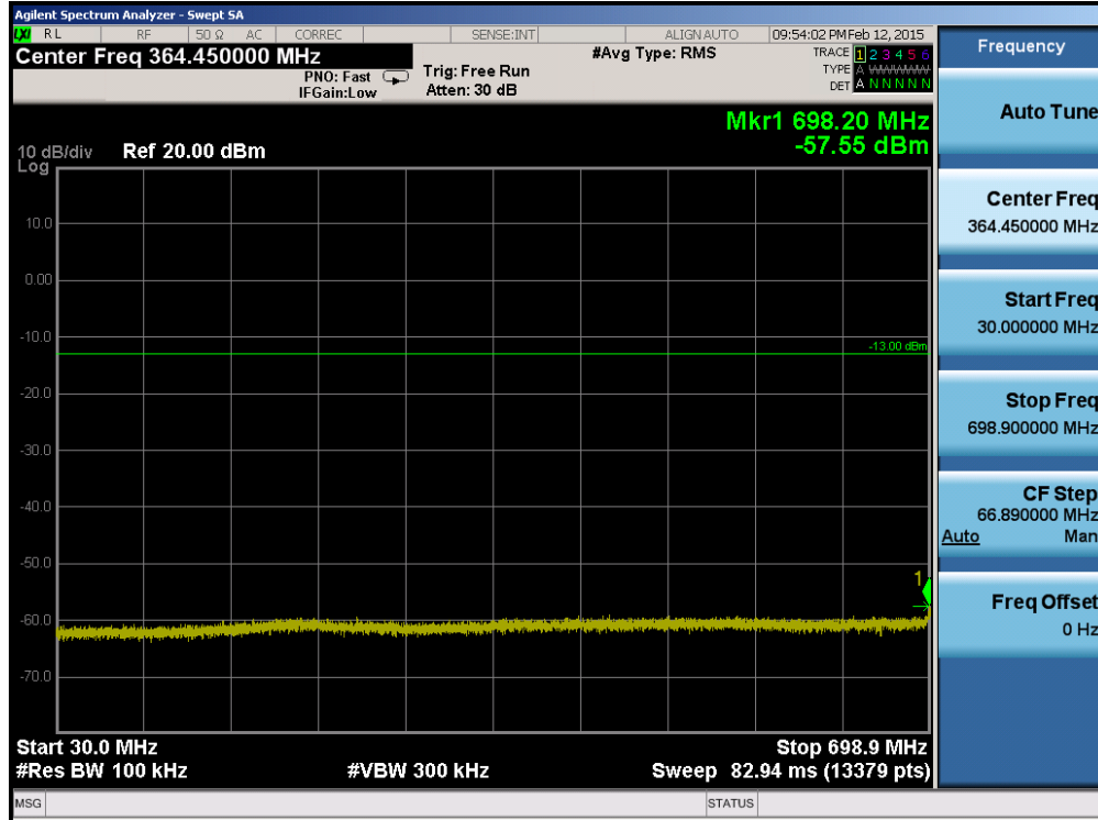
Plot 6-51. Conducted Spurious Plot (Band 12 – 5.0MHz QPSK – RB Size 1, RB Offset 0 – High Channel)
