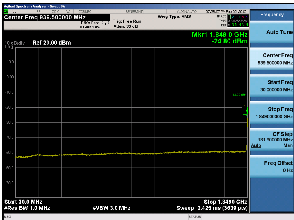
Plot 6-72. Conducted Spurious Plot (Band 2 – 5.0MHz QPSK – RB Size 1, RB Offset 0 – Low Channel)
