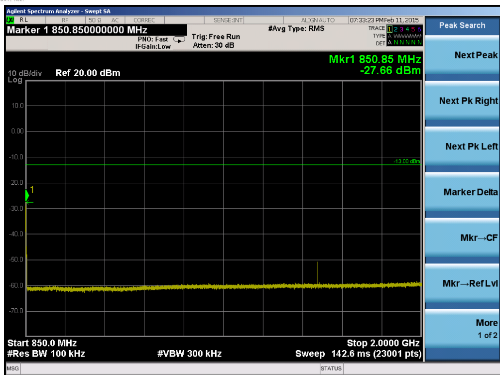
Plot 6-61. Conducted Spurious Plot (Band 5 – 3.0MHz QPSK – RB Size 1, RB Offset 0 – High Channel)
