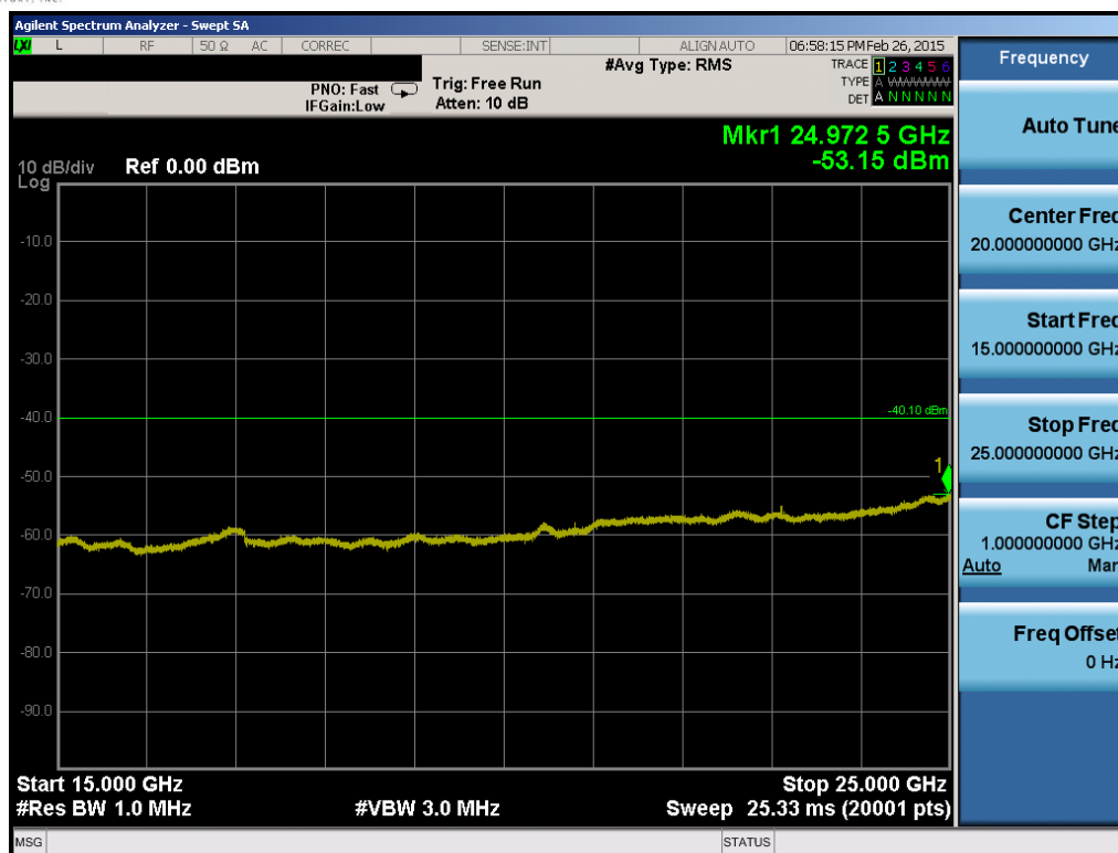
Plot 6-89. Conducted Spurious Plot (Band 30 – 5.0MHz QPSK – RB Size 1, RB Offset 0 – High Channel)
