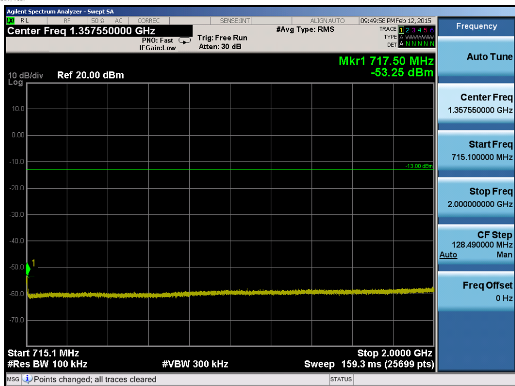
Plot 6-49. Conducted Spurious Plot (Band 12 – 5.0MHz QPSK – RB Size 1, RB Offset 0 – Mid Channel)
