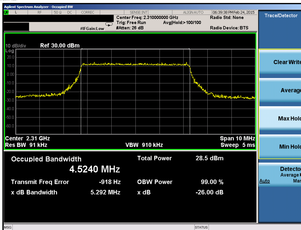
Plot 6-41. Occupied Bandwidth Plot (Band 30 – 5.0MHz QPSK – RB Size 25)
