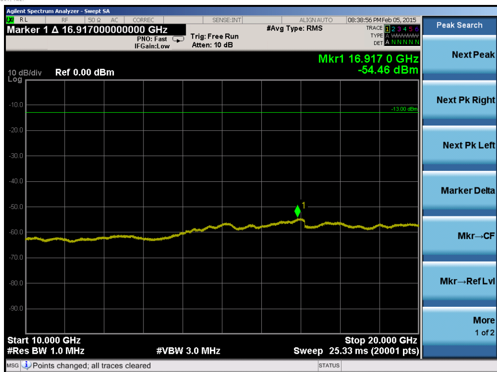
Plot 6-65. Conducted Spurious Plot (Band 4 – 5.0MHz QPSK – RB Size 1, RB Offset 0 – Low Channel)
