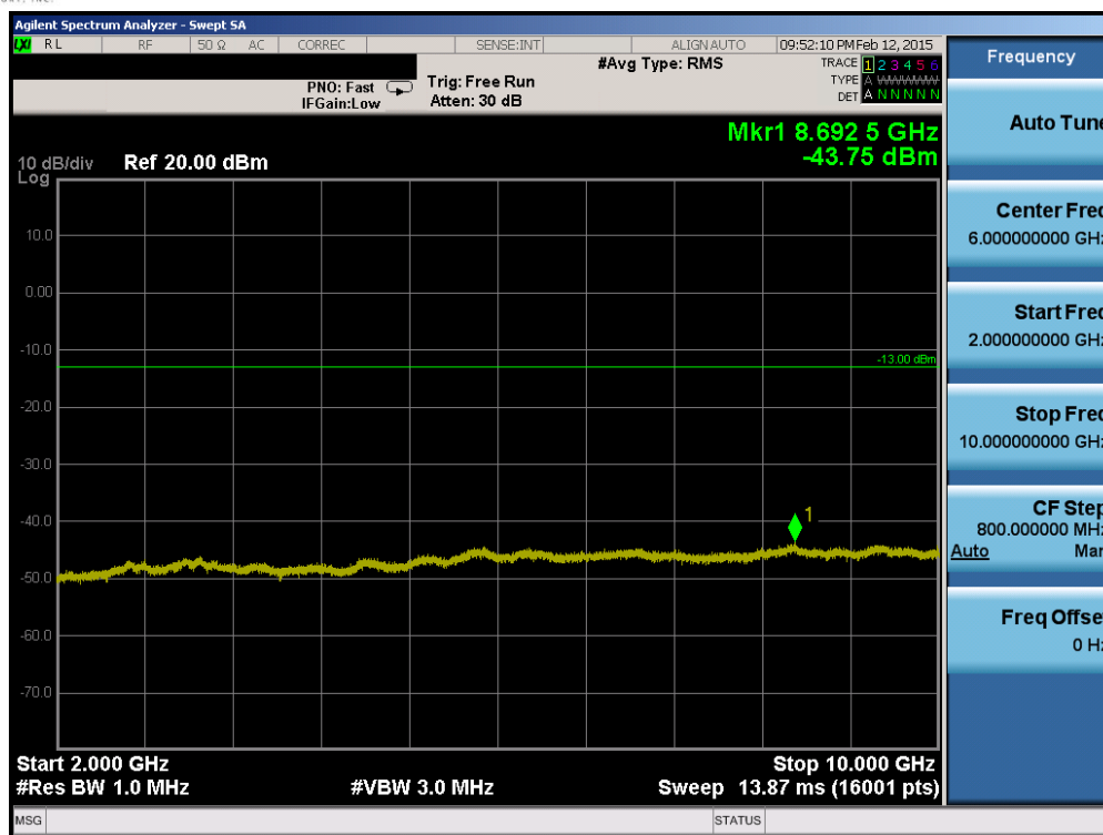
Plot 6-47. Conducted Spurious Plot (Band 12 – 5.0MHz QPSK – RB Size 1, RB Offset 0 – Low Channel)
