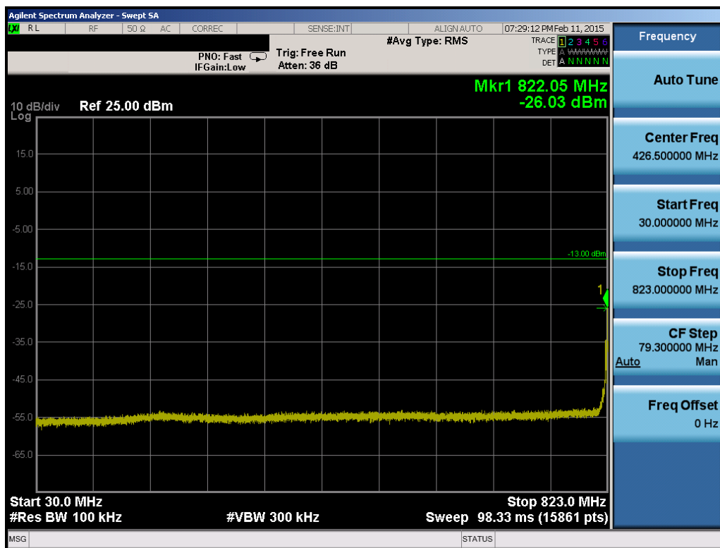
Plot 6-54. Conducted Spurious Plot (Band 5 – 3.0MHz QPSK – RB Size 1, RB Offset 0 – Low Channel)
