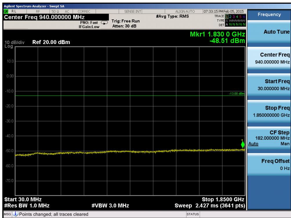
Plot 6-78. Conducted Spurious Plot (Band 2 – 5.0MHz QPSK – RB Size 1, RB Offset 0 – High Channel)
