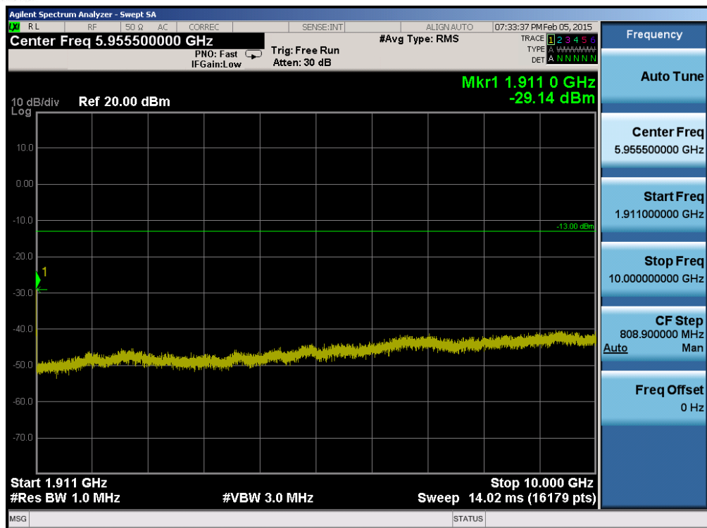
Plot 6-79. Conducted Spurious Plot (Band 2 – 5.0MHz QPSK – RB Size 1, RB Offset 0 – High Channel)
