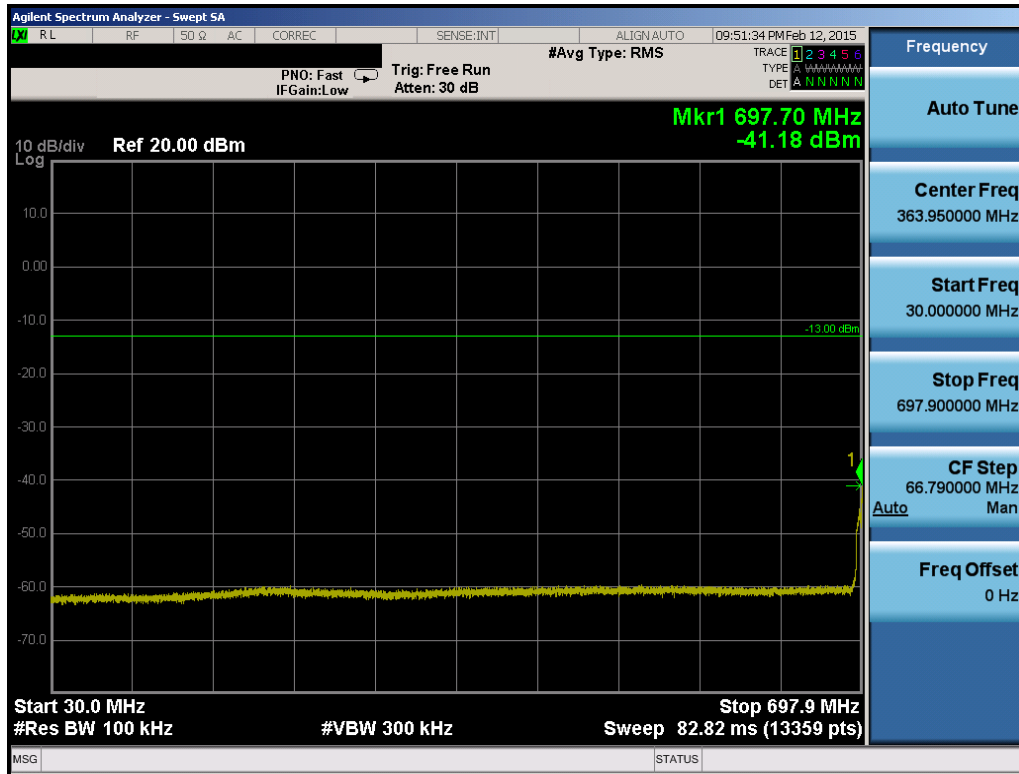
Plot 6-45. Conducted Spurious Plot (Band 12 – 5.0MHz QPSK – RB Size 1, RB Offset 0 – Low Channel)
