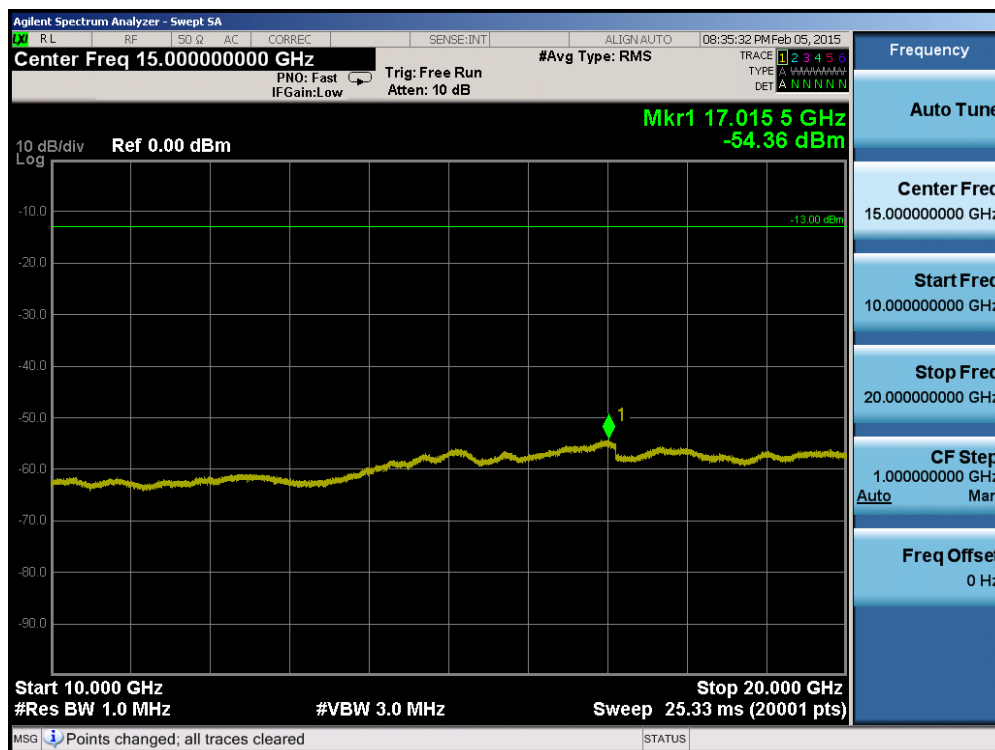
Plot 6-68. Conducted Spurious Plot (Band 4 – 5.0MHz QPSK – RB Size 1, RB Offset 0 – Mid Channel)
