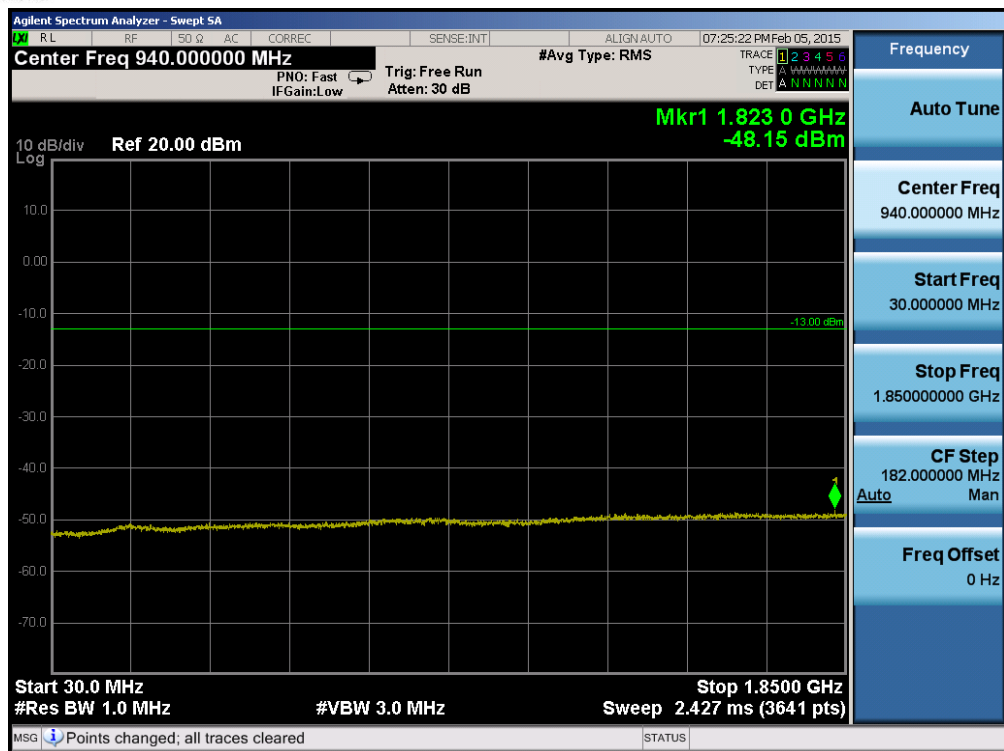
Plot 6-75. Conducted Spurious Plot (Band 2 – 5.0MHz QPSK – RB Size 1, RB Offset 0 – Mid Channel)
