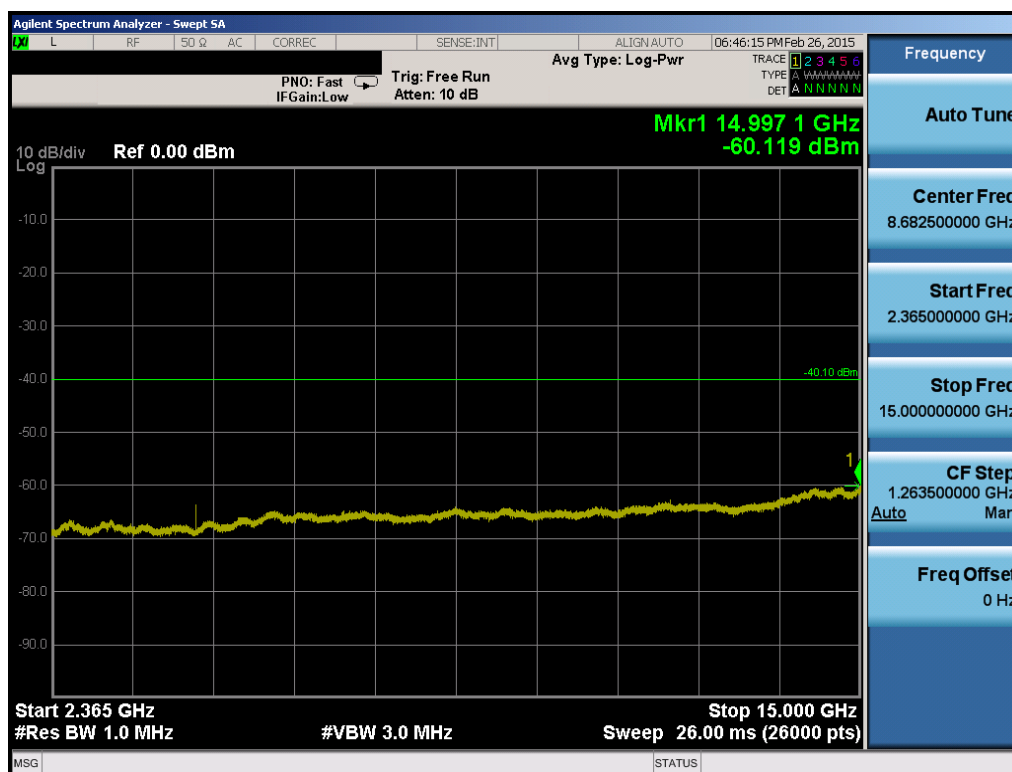
Plot 6-82. Conducted Spurious Plot (Band 30 – 5.0MHz QPSK – RB Size 1, RB Offset 0 – Low Channel)
