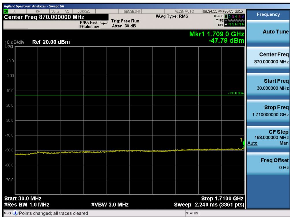
Plot 6-66. Conducted Spurious Plot (Band 4 – 5.0MHz QPSK – RB Size 1, RB Offset 0 – Mid Channel)
