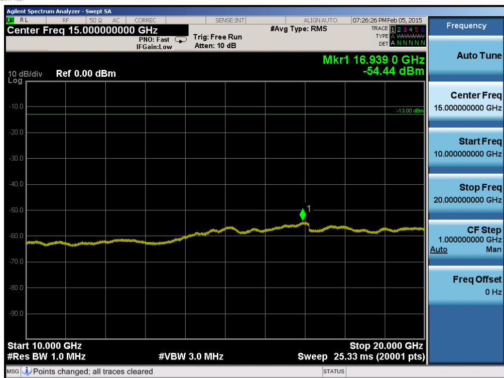
Plot 6-77. Conducted Spurious Plot (Band 2 – 5.0MHz QPSK – RB Size 1, RB Offset 0 – Mid Channel)
