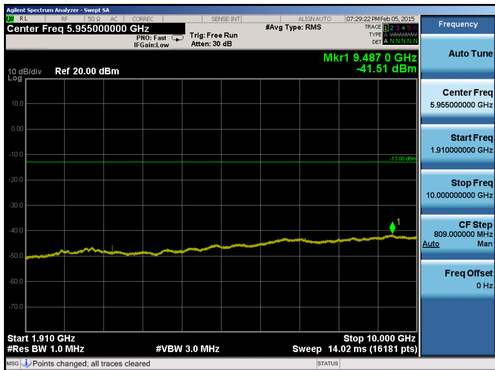
Plot 6-73. Conducted Spurious Plot (Band 2 – 5.0MHz QPSK – RB Size 1, RB Offset 0 – Low Channel)
