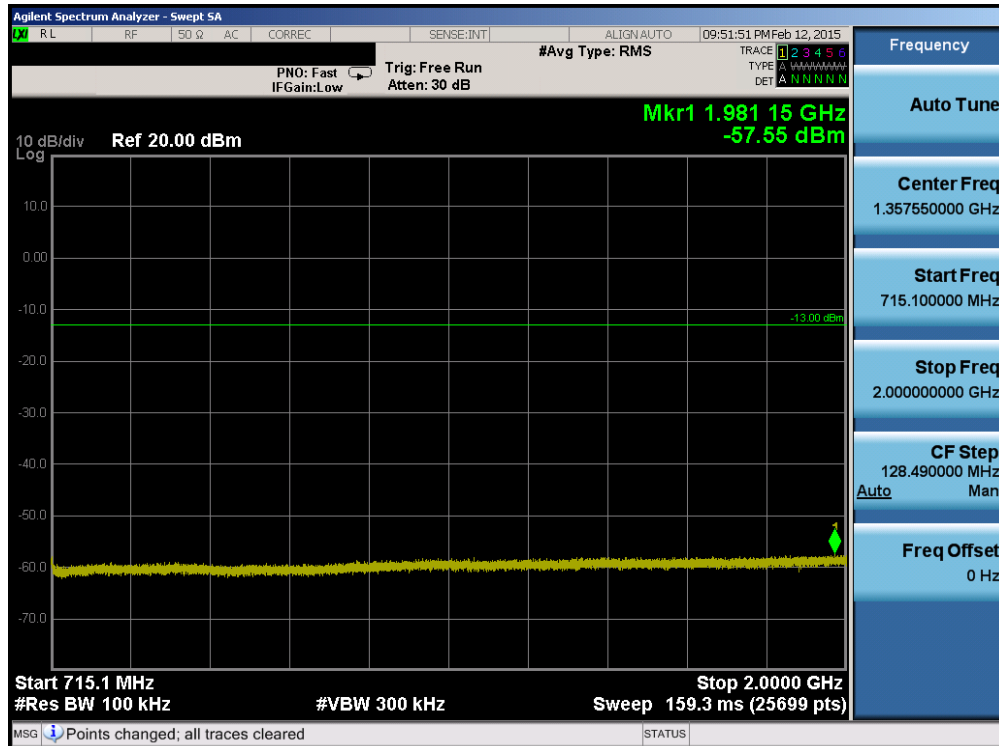
Plot 6-46. Conducted Spurious Plot (Band 12 – 5.0MHz QPSK – RB Size 1, RB Offset 0 – Low Channel)
