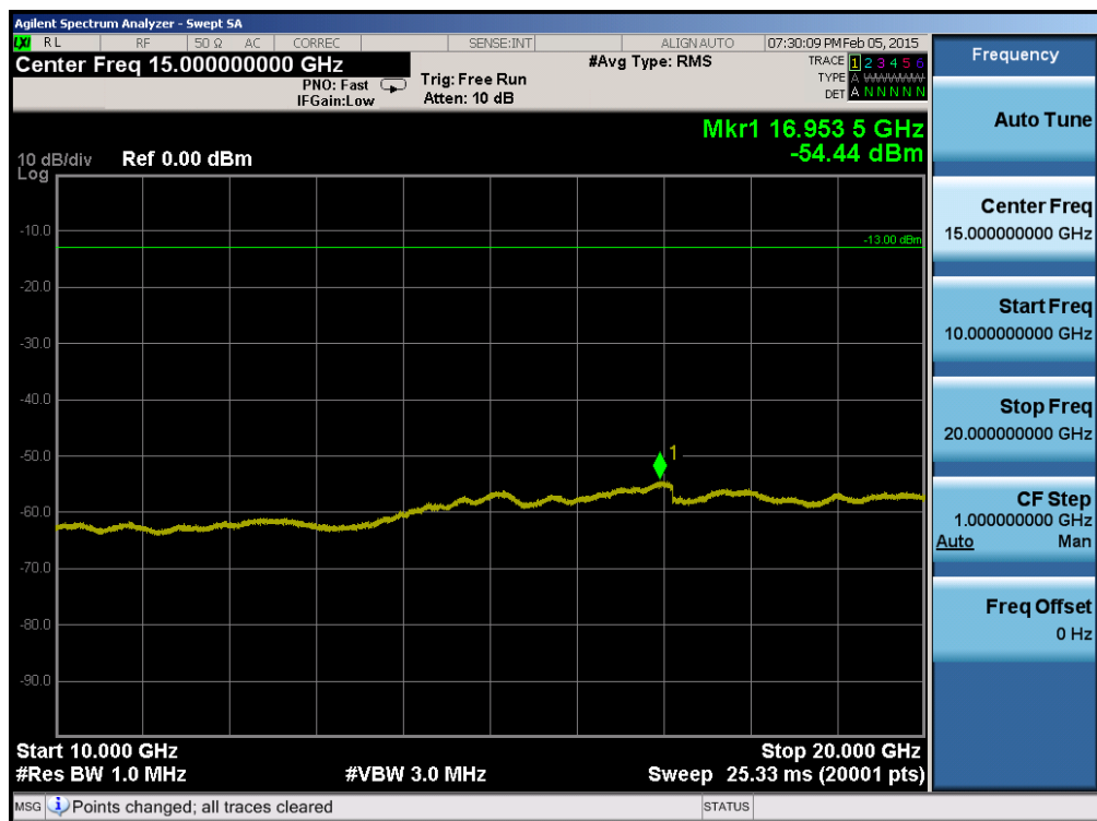
Plot 6-74. Conducted Spurious Plot (Band 2 – 5.0MHz QPSK – RB Size 1, RB Offset 0 – Low Channel)
