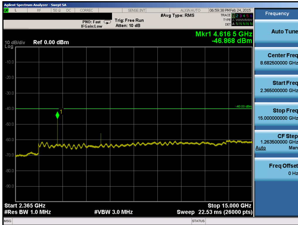
Plot 6-85. Conducted Spurious Plot (Band 30 – 5.0MHz QPSK – RB Size 1, RB Offset 0 – Mid Channel)
