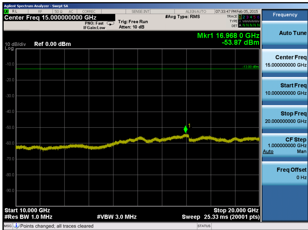
Plot 6-80. Conducted Spurious Plot (Band 2 – 5.0MHz QPSK – RB Size 1, RB Offset 0 – High Channel)
