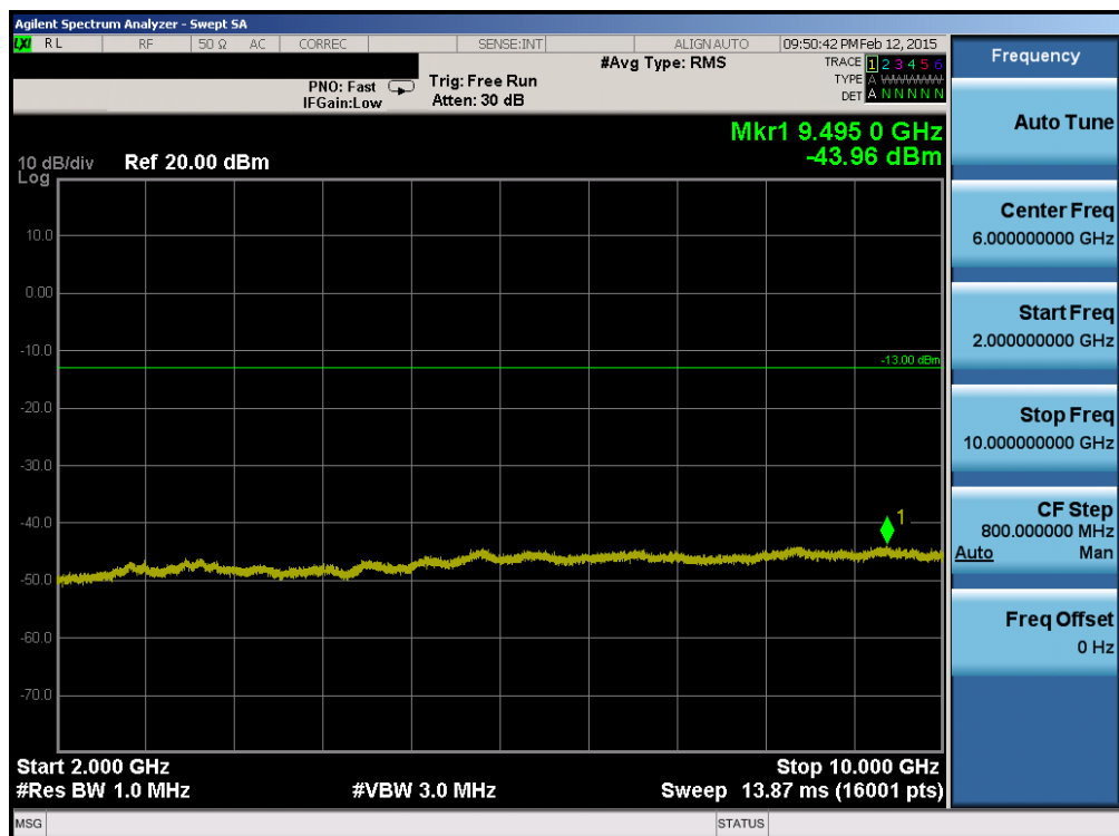
Plot 6-50. Conducted Spurious Plot (Band 12 – 5.0MHz QPSK – RB Size 1, RB Offset 0 – Mid Channel)
