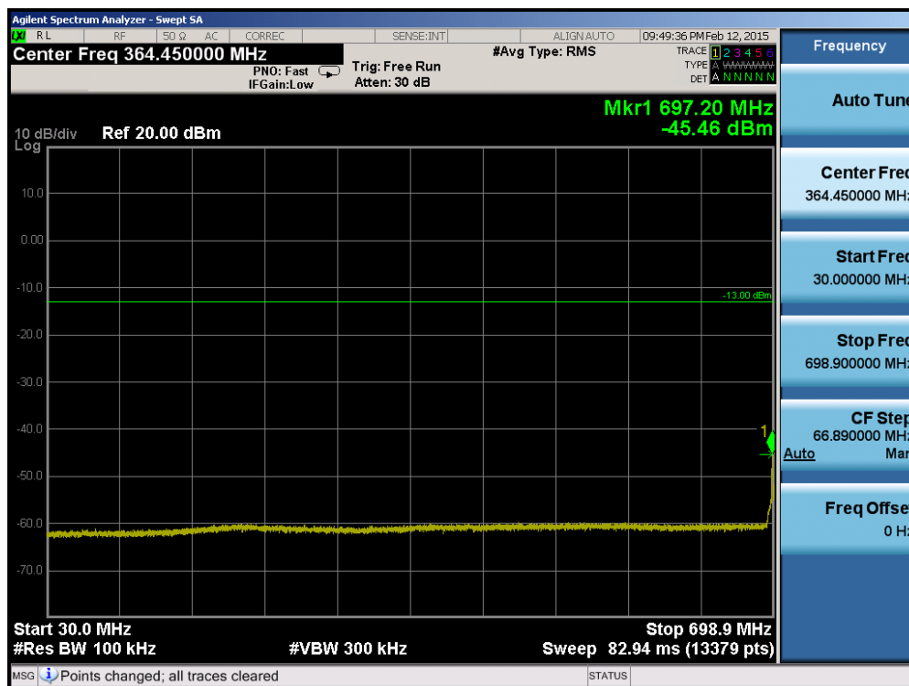
Plot 6-48. Conducted Spurious Plot (Band 12 – 5.0MHz QPSK – RB Size 1, RB Offset 0 – Mid Channel)
