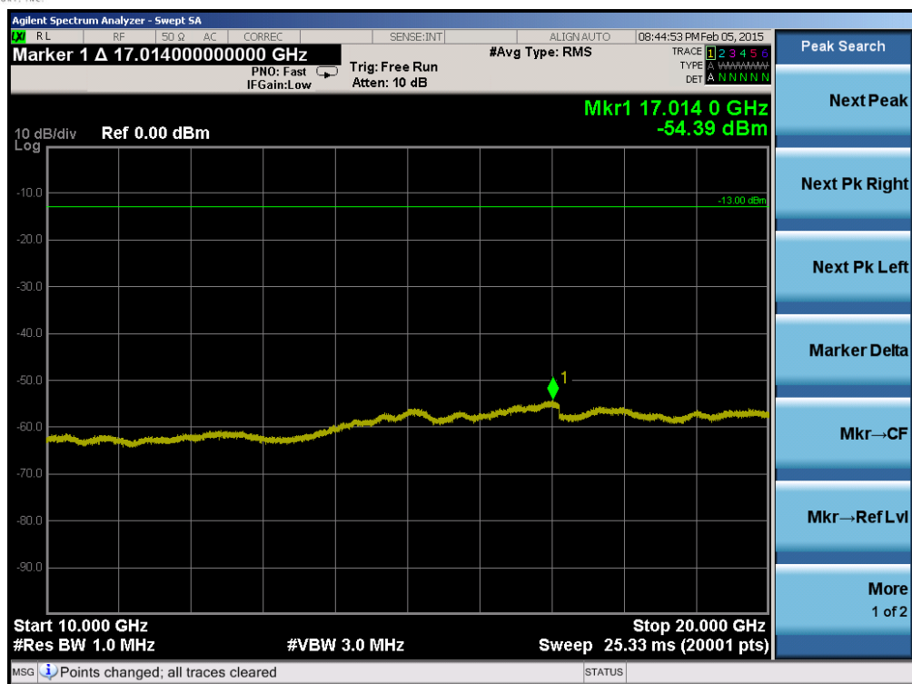
Plot 6-71. Conducted Spurious Plot (Band 4 – 5.0MHz QPSK – RB Size 1, RB Offset 0 – High Channel)
