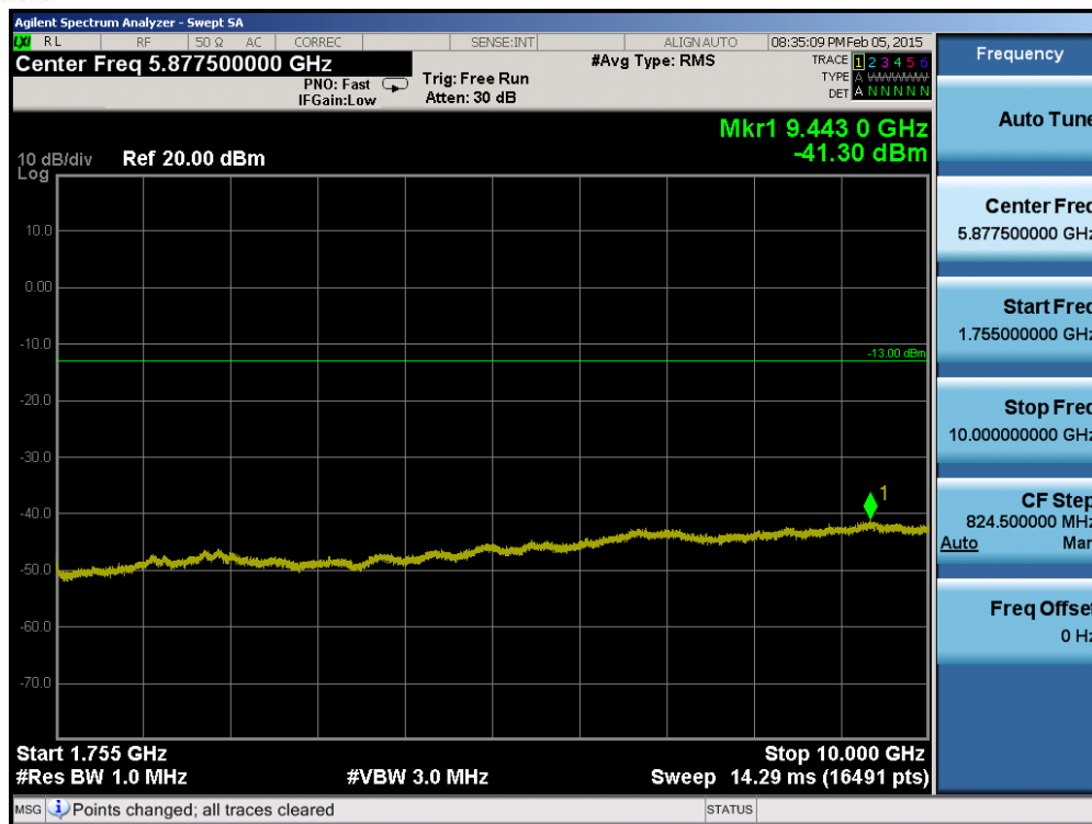
Plot 6-67. Conducted Spurious Plot (Band 4 – 5.0MHz QPSK – RB Size 1, RB Offset 0 – Mid Channel)
