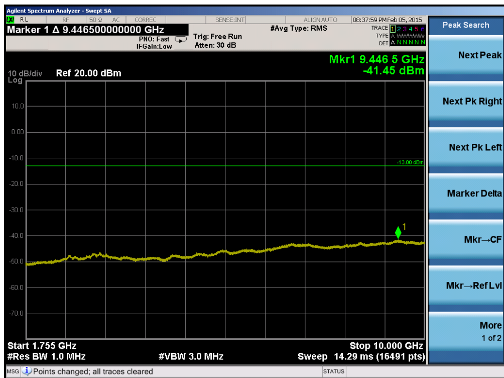
Plot 6-64. Conducted Spurious Plot (Band 4 – 5.0MHz QPSK – RB Size 1, RB Offset 0 – Low Channel)
