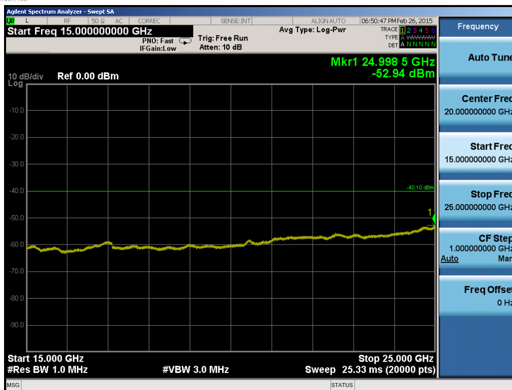
Plot 6-83. Conducted Spurious Plot (Band 30 – 5.0MHz QPSK – RB Size 1, RB Offset 0 – Low Channel)
