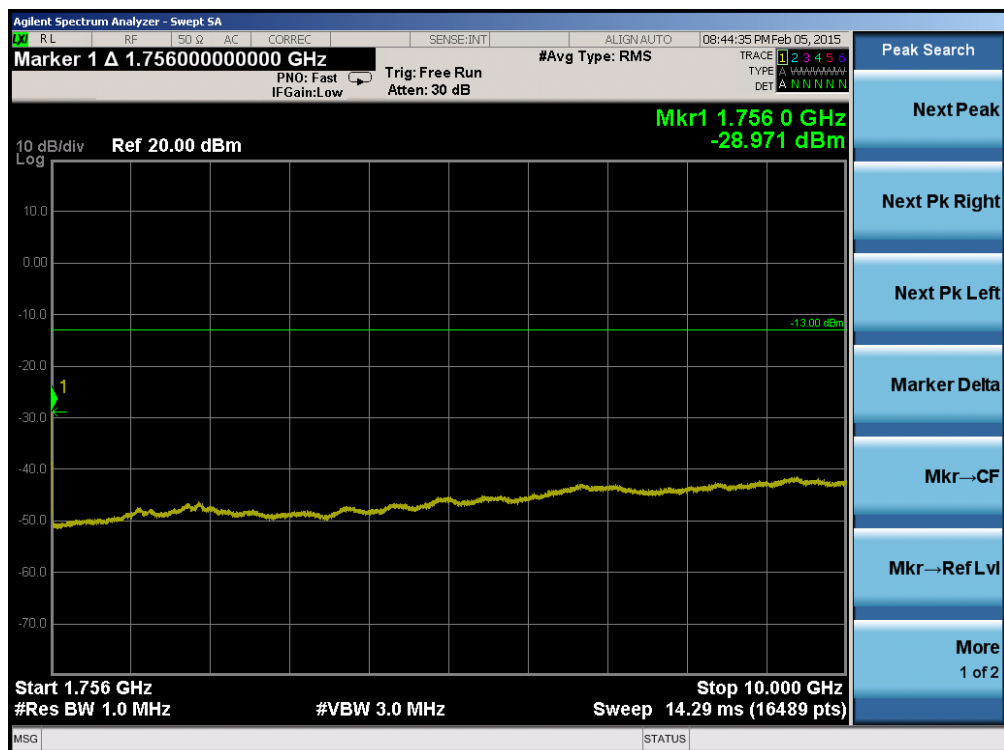
Plot 6-70. Conducted Spurious Plot (Band 4 – 5.0MHz QPSK – RB Size 1, RB Offset 0 – High Channel)
