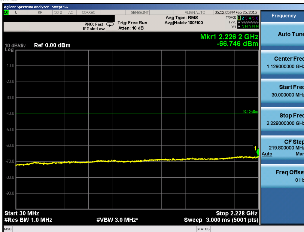
Plot 6-81. Conducted Spurious Plot (Band 30 – 5.0MHz QPSK – RB Size 1, RB Offset 0 – Low Channel)
