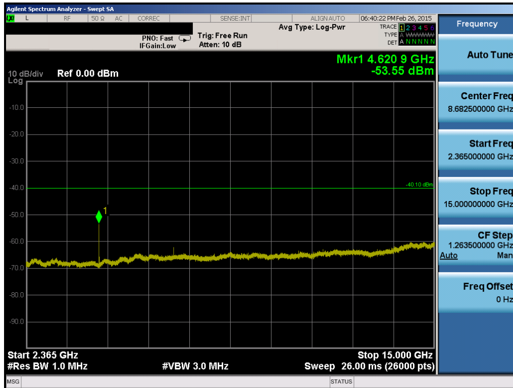
Plot 6-88. Conducted Spurious Plot (Band 30 – 5.0MHz QPSK – RB Size 1, RB Offset 0 – High Channel)
