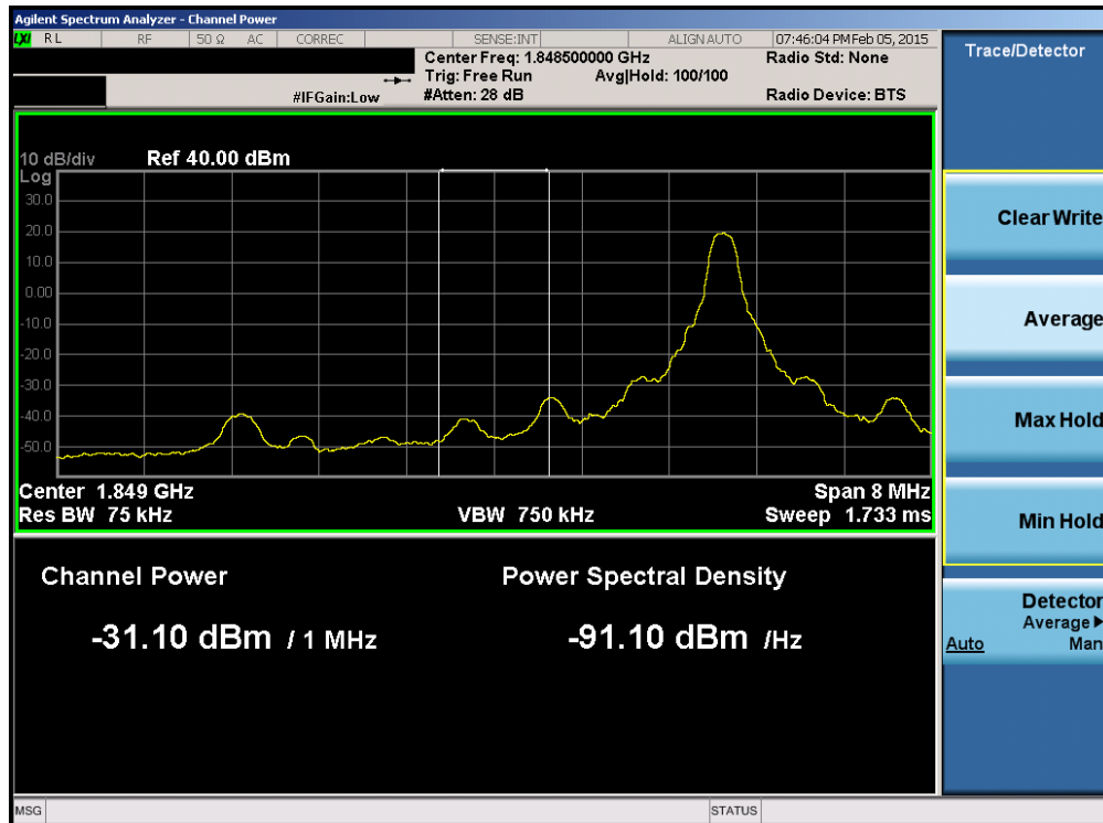
Plot 6-155. Lower Extended Band Edge Plot (Band 2 – 10.0MHz QPSK – RB Size 1)
