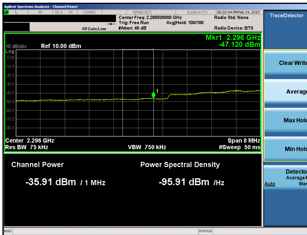
Plot 6-173. Lower Extended Band Edge Plot (Band 30 – 10MHz QPSK – RB Size 50)
