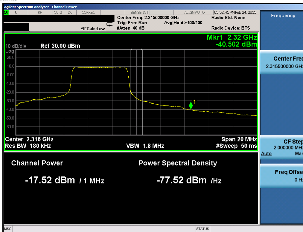
Plot 6-168. Upper Band Edge Plot (Band 30 – 5MHz QPSK – RB Size 25)
