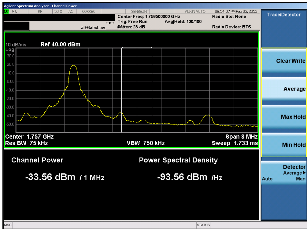
Plot 6-133. Upper Extended Band Edge Plot (Band 4 – 10.0MHz QPSK – RB Size 1)
