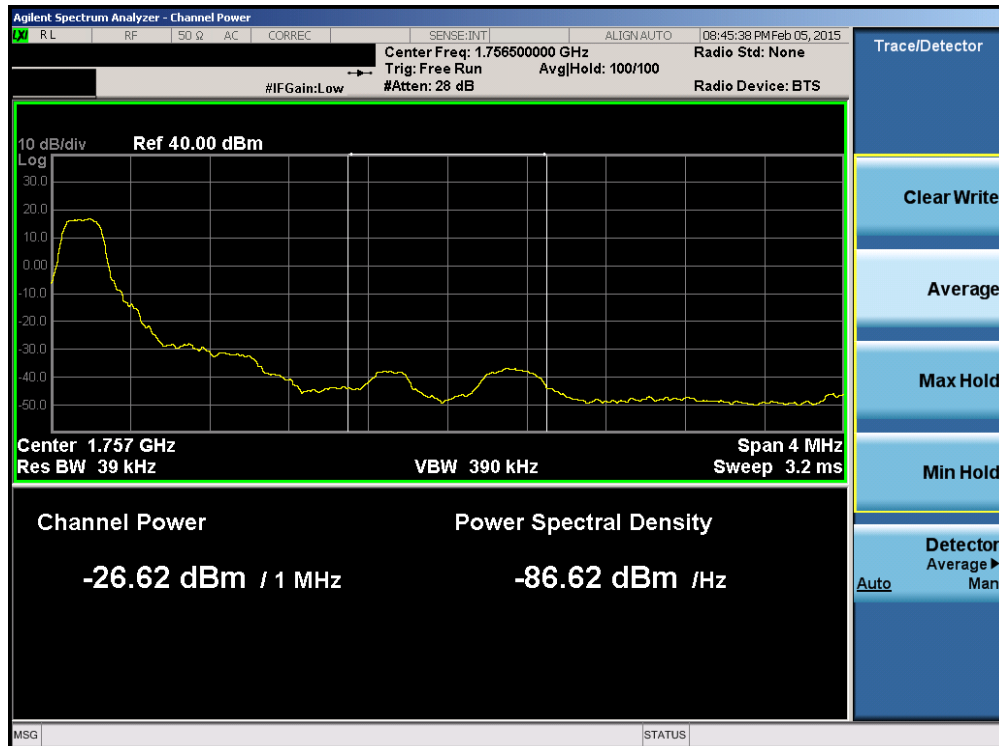
Plot 6-129. Upper Extended Band Edge Plot (Band 4 – 5.0MHz QPSK – RB Size 1)
