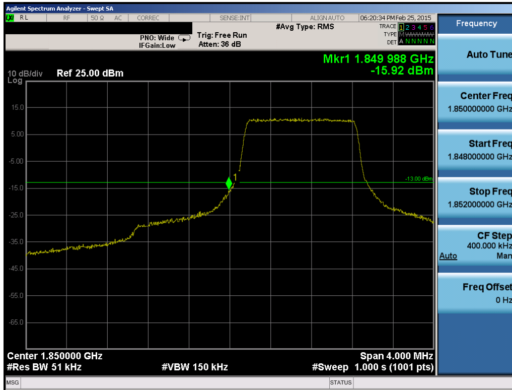
Plot 6-142. Lower Band Edge Plot (Band 2 – 1.4MHz QPSK – RB Size 6)
