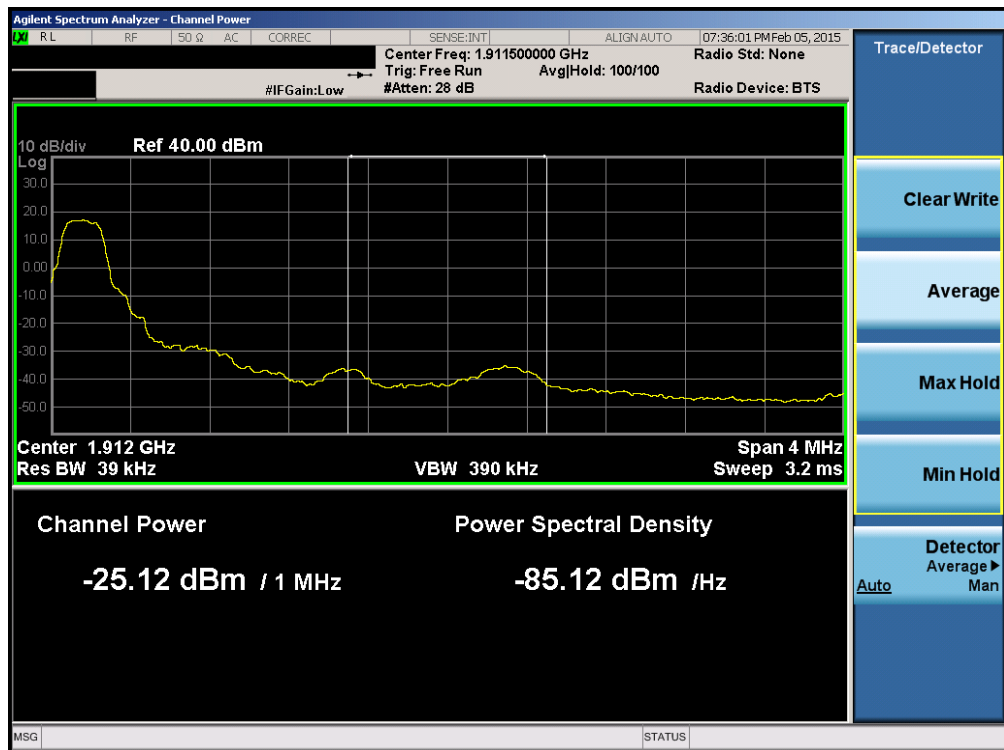
Plot 6-153. Upper Extended Band Edge Plot (Band 2 – 5.0MHz QPSK – RB Size 1)
