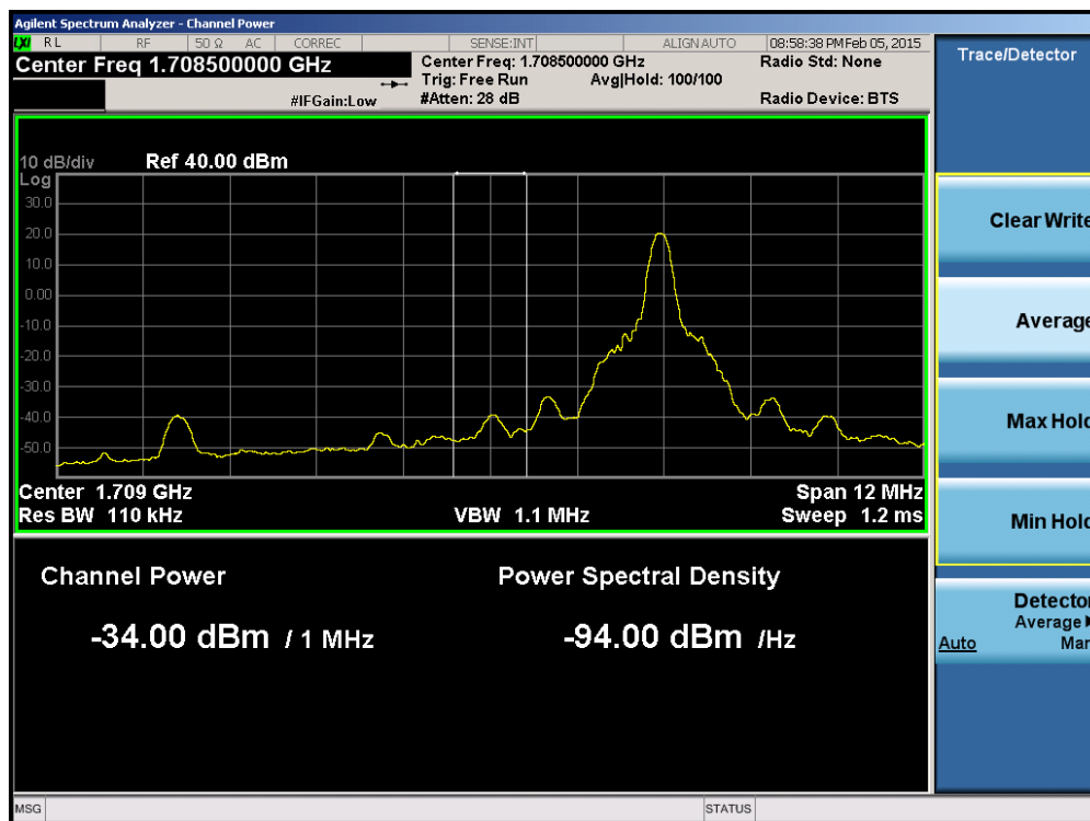
Plot 6-135. Lower Extended Band Edge Plot (Band 4 – 15.0MHz QPSK – RB Size 1)
