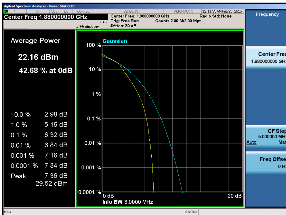
Plot 6-180. PAR Plot (Band 2 – 3.0MHz 16-QAM – RB Size 15)
