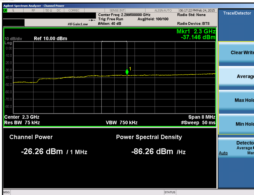
Plot 6-172. Lower Extended Band Edge Plot (Band 30 – 10MHz QPSK – RB Size 50)
