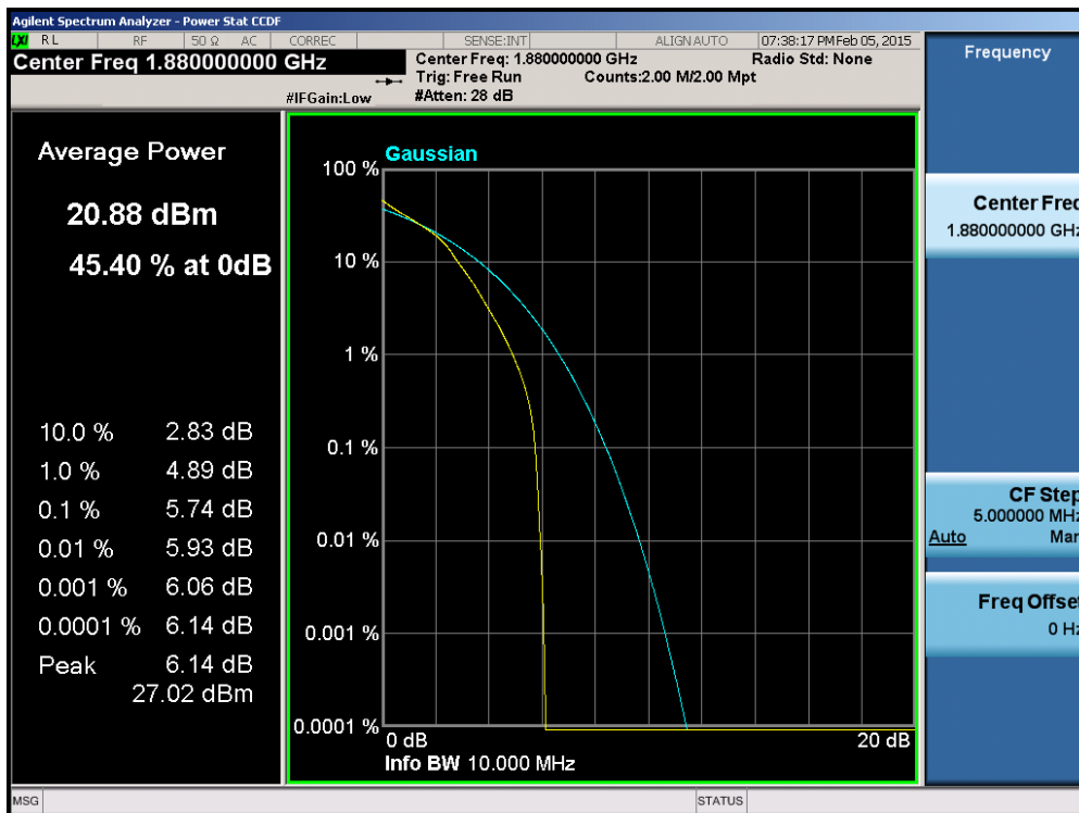
Plot 6-184. PAR Plot (Band 2 – 10.0MHz 16-QAM – RB Size 50)
