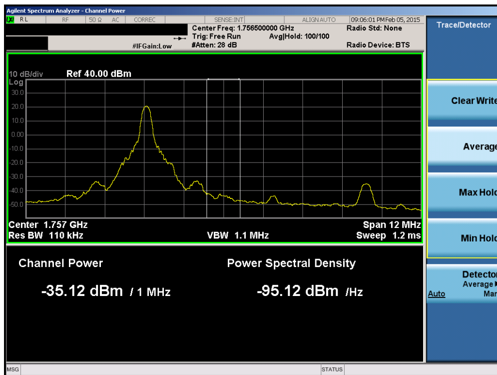
Plot 6-137. Upper Extended Band Edge Plot (Band 4 – 15.0MHz QPSK – RB Size 1)
