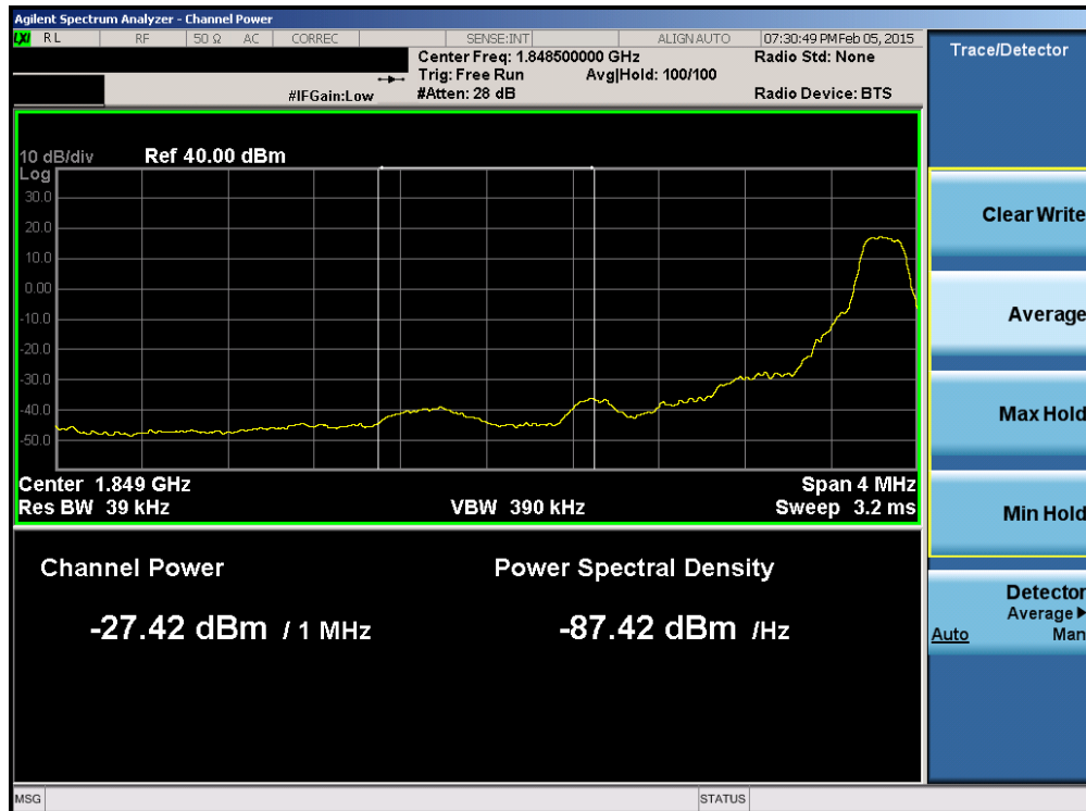
Plot 6-151. Lower Extended Band Edge Plot (Band 2 – 5.0MHz QPSK – RB Size 1)
