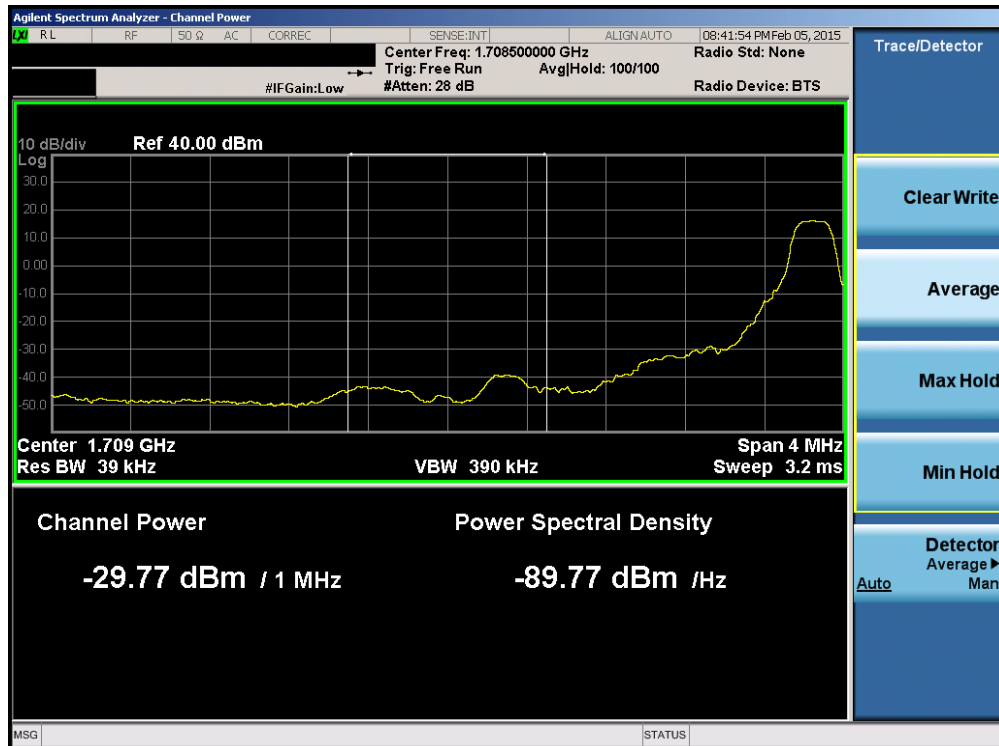
Plot 6-127. Lower Extended Band Edge Plot (Band 4 – 5.0MHz QPSK – RB Size 1)
