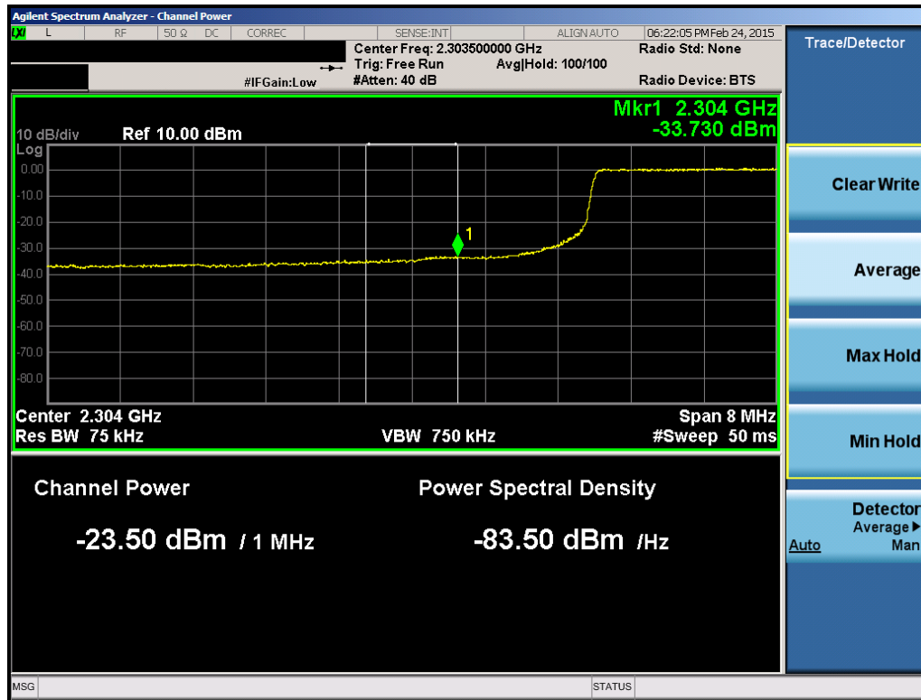
Plot 6-171. Lower Extended Band Edge Plot (Band 30 – 10MHz QPSK – RB Size 50)
