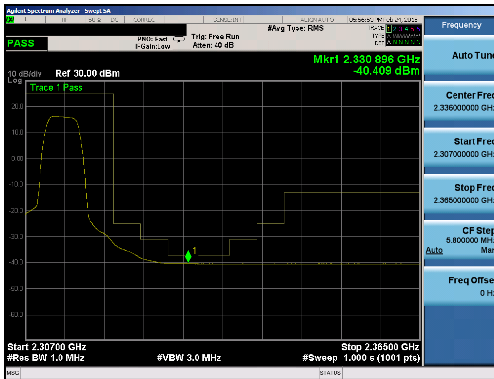
Plot 6-169. Upper Extended Band Edge Plot (Band 30 – 5MHz QPSK – RB Size 25)
