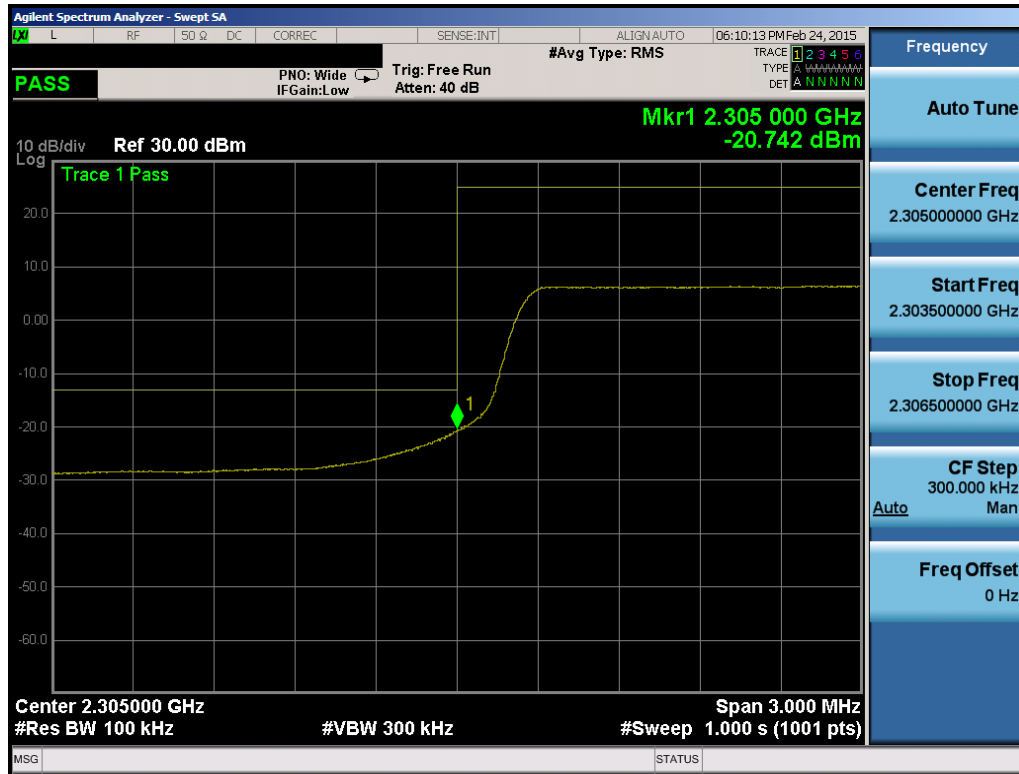
Plot 6-166. Lower Band Edge Plot (Band 30 – 5MHz QPSK – RB Size 25)
