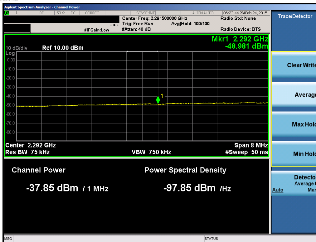
Plot 6-174. Lower Extended Band Edge Plot (Band 30 – 10MHz QPSK – RB Size 50)
