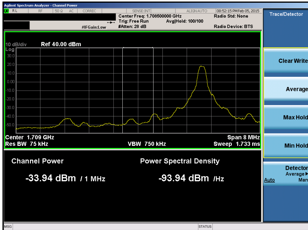
Plot 6-131. Lower Extended Band Edge Plot (Band 4 – 10.0MHz QPSK – RB Size 1)
