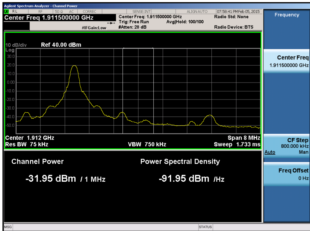
Plot 6-157. Upper Extended Band Edge Plot (Band 2 – 10.0MHz QPSK – RB Size 1)
