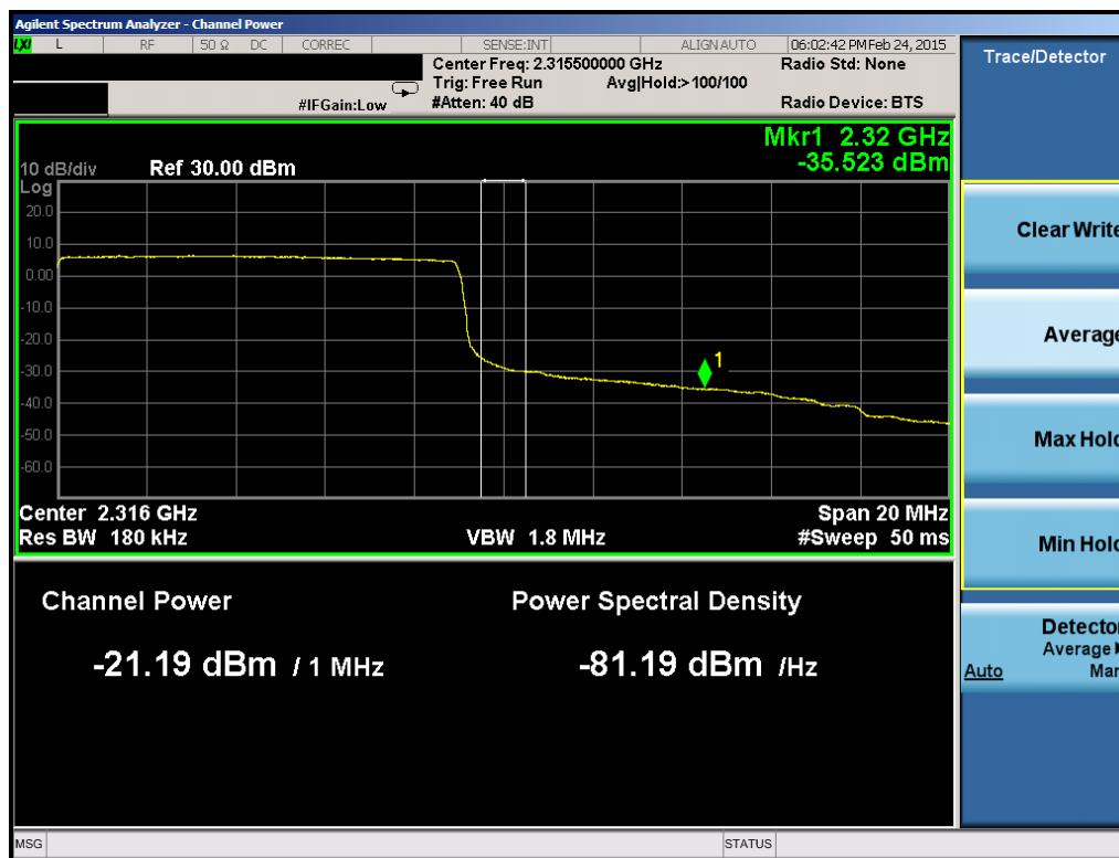
Plot 6-175. Upper Band Edge Plot (Band 30 – 10MHz QPSK – RB Size 50)
