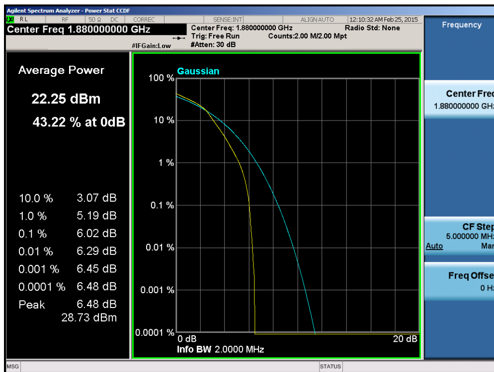
Plot 6-178. PAR Plot (Band 2 – 1.4MHz 16-QAM – RB Size 6)
